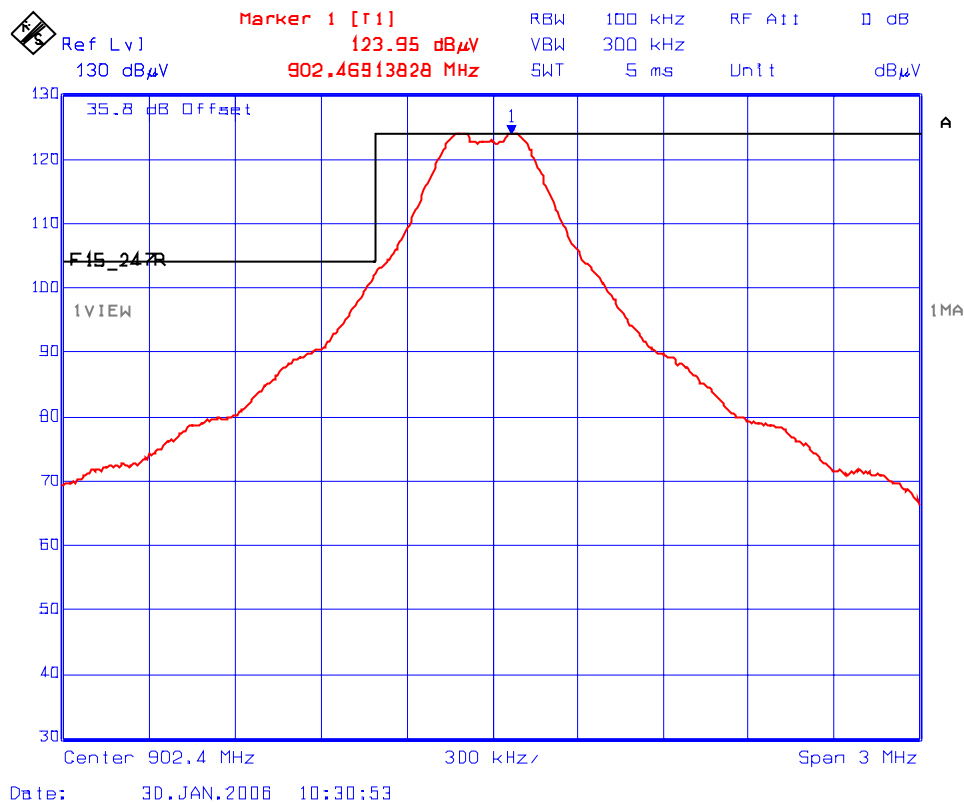
Plot 6.12.5.1.2: FHSS - Band-Edge RF Radiated Emissions @ 3 meters Low End of Frequency Band Test Configuration 1: EUT with \frac{1}{4} Wave Antenna (1.5 dBi Gain) Rx Antenna Orientation: Horizontal
