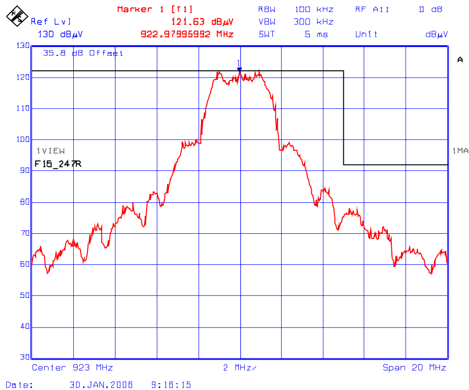
Plot 6.12.5.1.11: DTS - Band-Edge RF Radiated Emissions @ 3 meters Upper End of Frequency Band (923 MHz at Data Rate 11) Test Configuration 1: EUT with ¼ Wave Antenna (1.5 dBi Gain) Rx Antenna Orientation: Vertical
