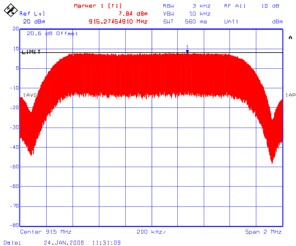
Plot 6.13.5.5 Power Spectral Density Frequency: 915 MHz at Data Rate 9
