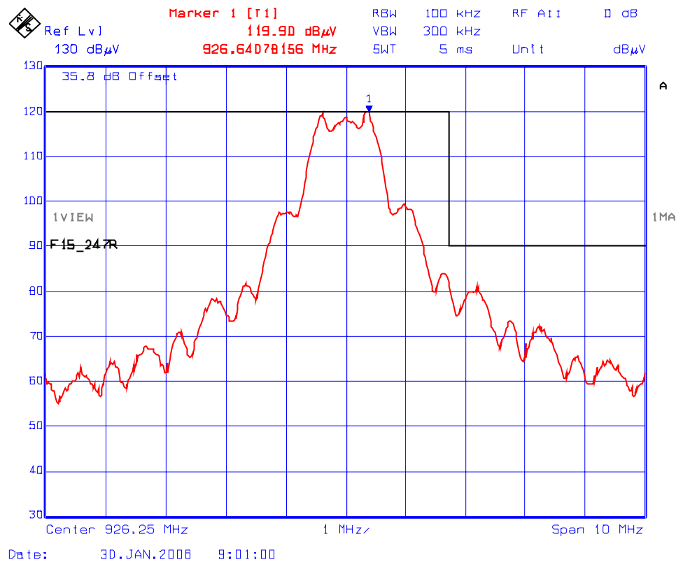
Plot 6.12.5.1.10: DTS - Band-Edge RF Radiated Emissions @ 3 meters Upper End of Frequency Band (926.25 MHz at Data Rate 8) Test Configuration 1: EUT with ¼ Wave Antenna (1.5 dBi Gain) Rx Antenna Orientation: Horizontal
