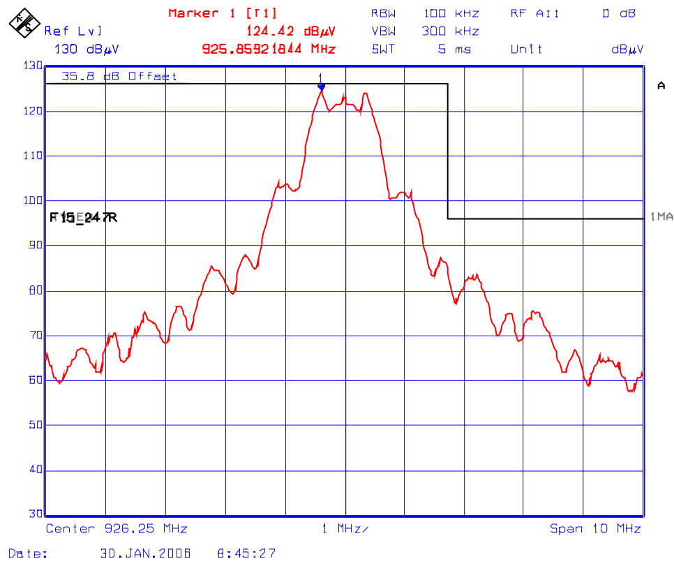
Plot 6.12.5.1.9: DTS - Band-Edge RF Radiated Emissions @ 3 meters Upper End of Frequency Band (926.25 MHz at Data Rate 8) Test Configuration 1: EUT with ¼ Wave Antenna (1.5 dBi Gain) Rx Antenna Orientation: Vertical
