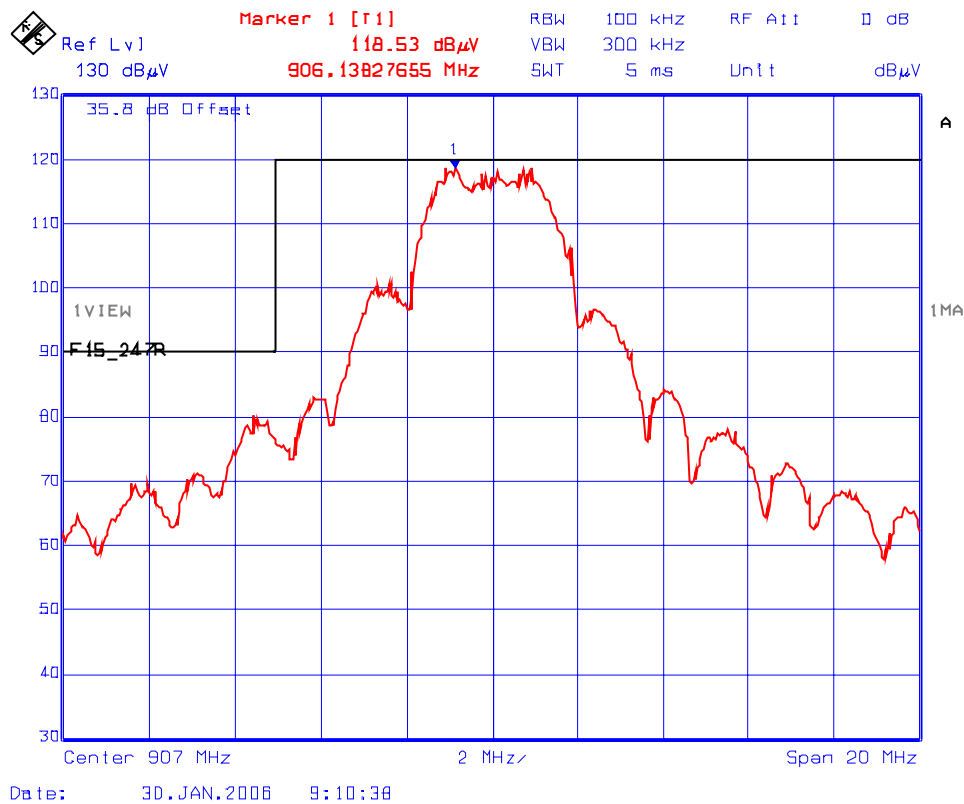
Plot 6.12.5.1.6: DTS - Band-Edge RF Radiated Emissions @ 3 meters Low End of Frequency Band (907 MHz at Data Rate 11) Test Configuration 1: EUT with ¼ Wave Antenna (1.5 dBi Gain) Rx Antenna Orientation: Horizontal
