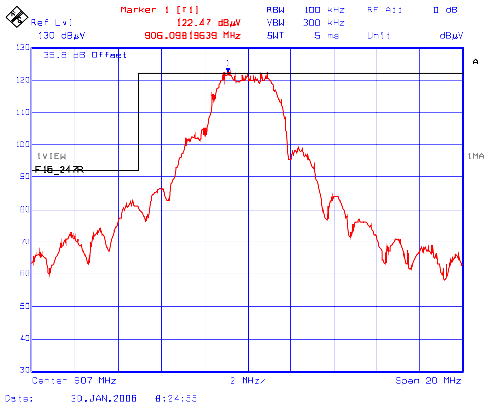
Plot 6.12.5.1.5: DTS - Band-Edge RF Radiated Emissions @ 3 meters Low End of Frequency Band (907 MHz at Data Rate 11) Test Configuration 1: EUT with ¼ Wave Antenna (1.5 dBi Gain) Rx Antenna Orientation: Vertical
