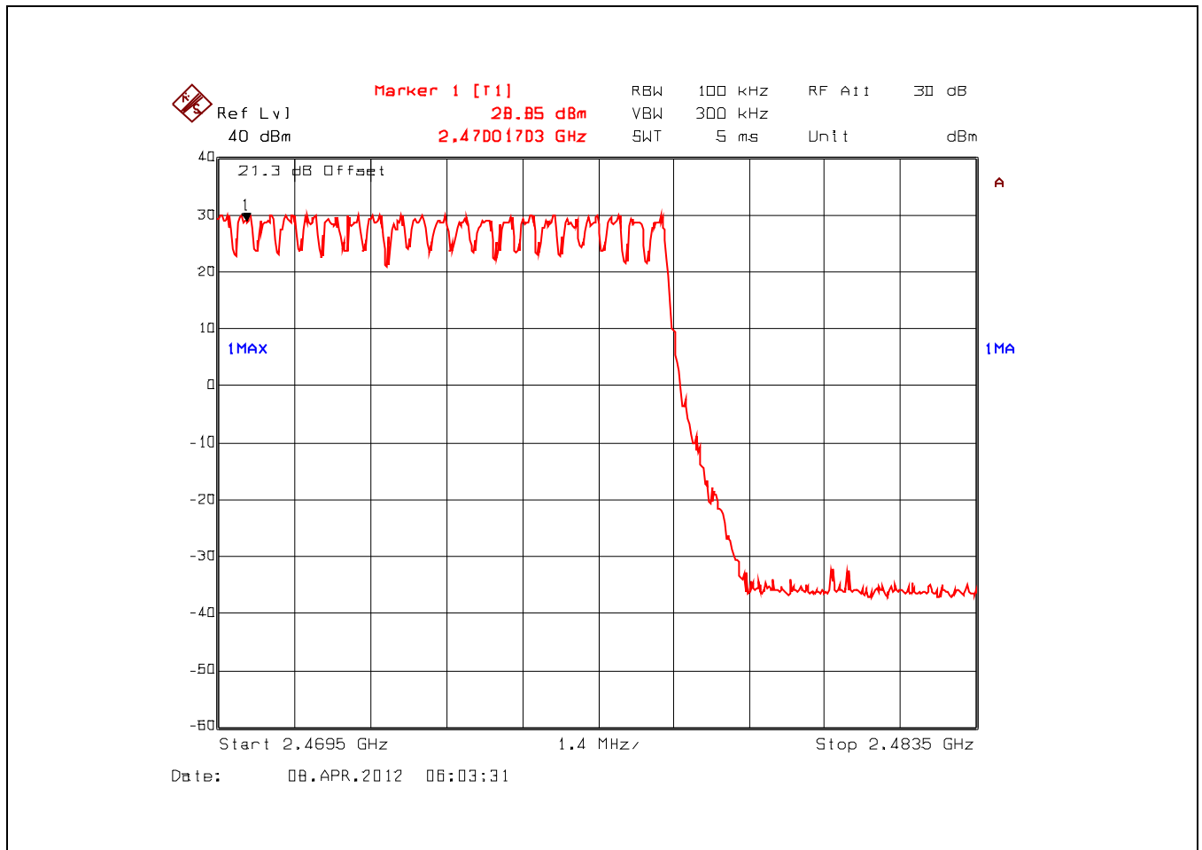
Plot 5.3.4.10. Number of Hopping Frequencies, Data Rate 5 20 Hopping Channels from 2469.5 - 2483.5 MHz
