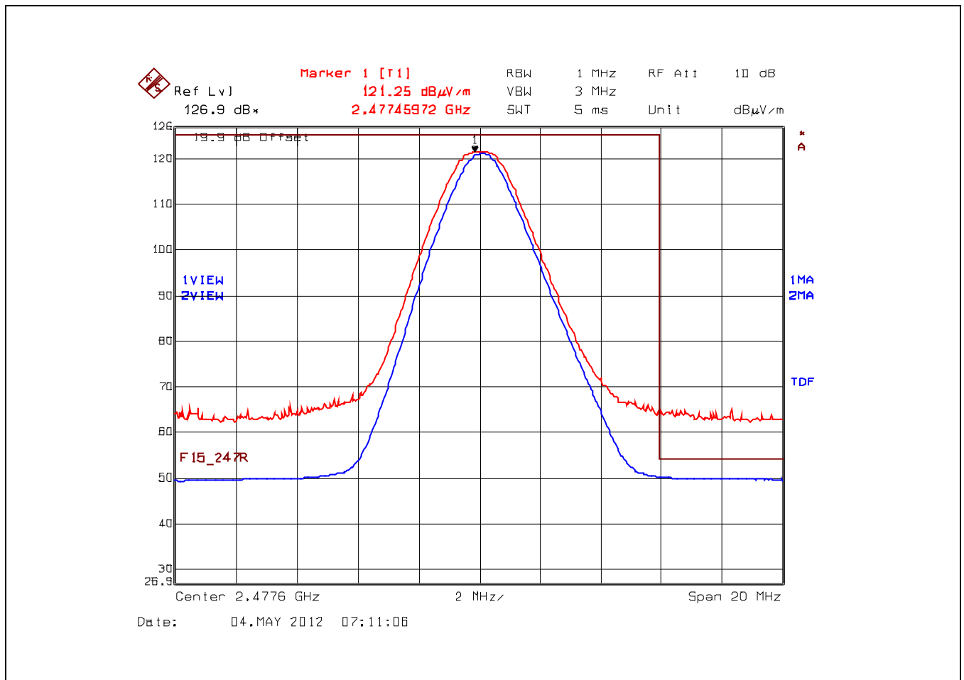
Plot 5.6.4.3.2.7. Band-Edge RF Radiated Emissions at 3 m, Vertical Polarization High End of Frequency Band, 2477.6 MHz, Power Setting 38, Data Rate 5
