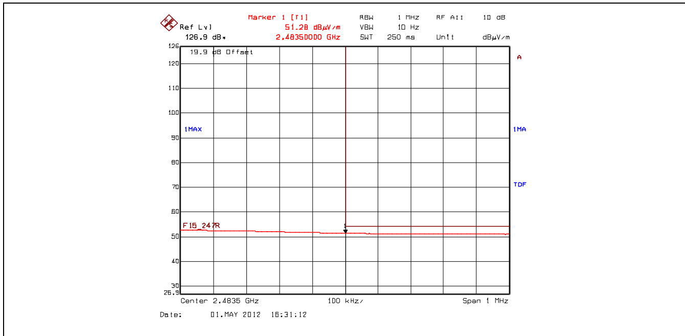
Plot 5.6.4.1.2.6. Band-Edge RF Radiated Emissions at 3 m, Horizontal Polarization High End of Frequency Band, 2477.6 MHz, Power Setting 50, Data Rate 5
