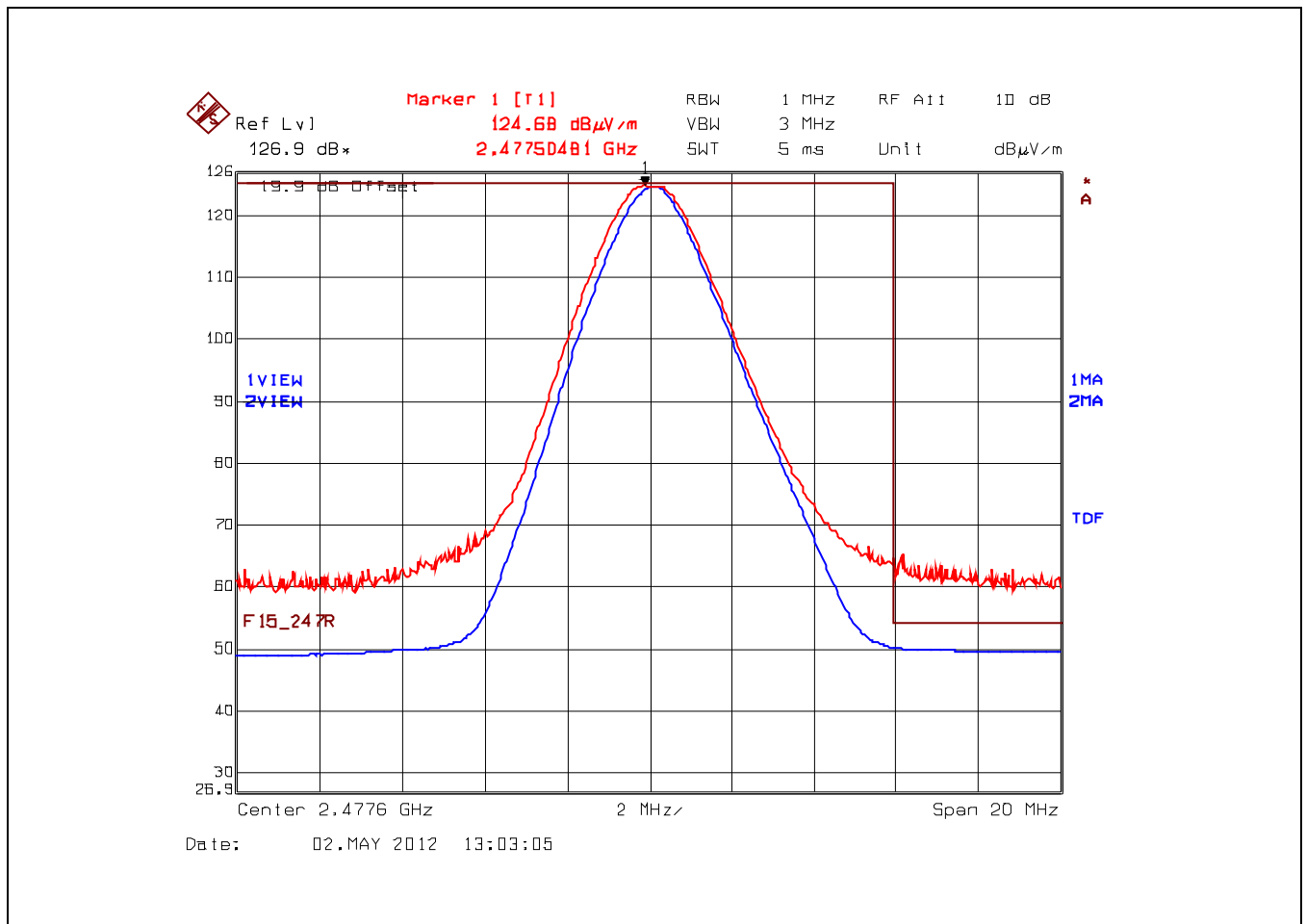
Plot 5.6.4.4.2.7. Band-Edge RF Radiated Emissions at 3 m, Vertical Polarization High End of Frequency Band, 2477.6 MHz, Power Setting 40, Data Rate 5
