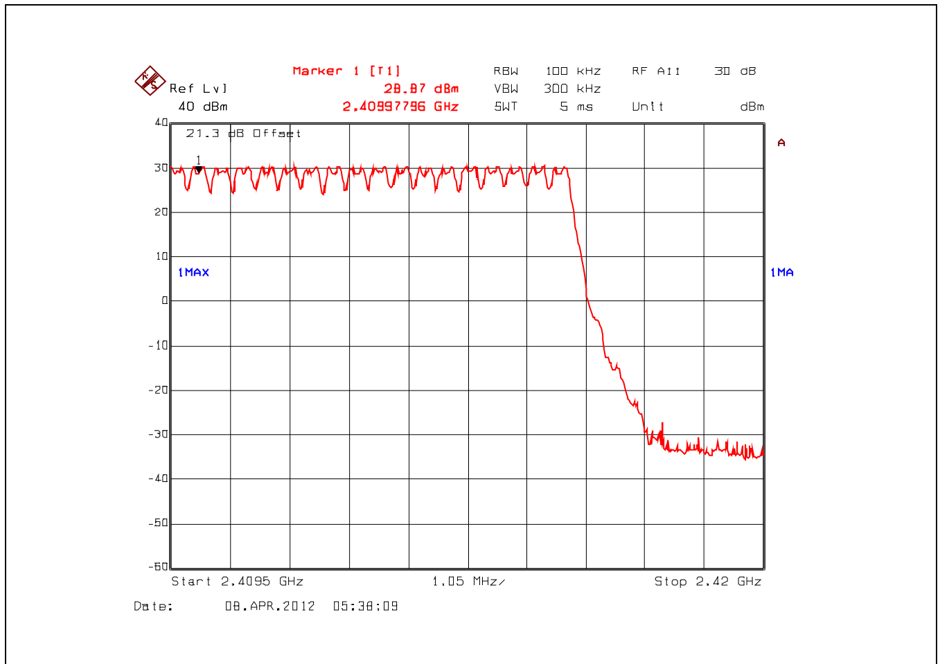
Plot 5.3.4.7. Number of Hopping Frequencies, Data Rate 5 17 Hopping Channels from 2409.5 - 2420 MHz
