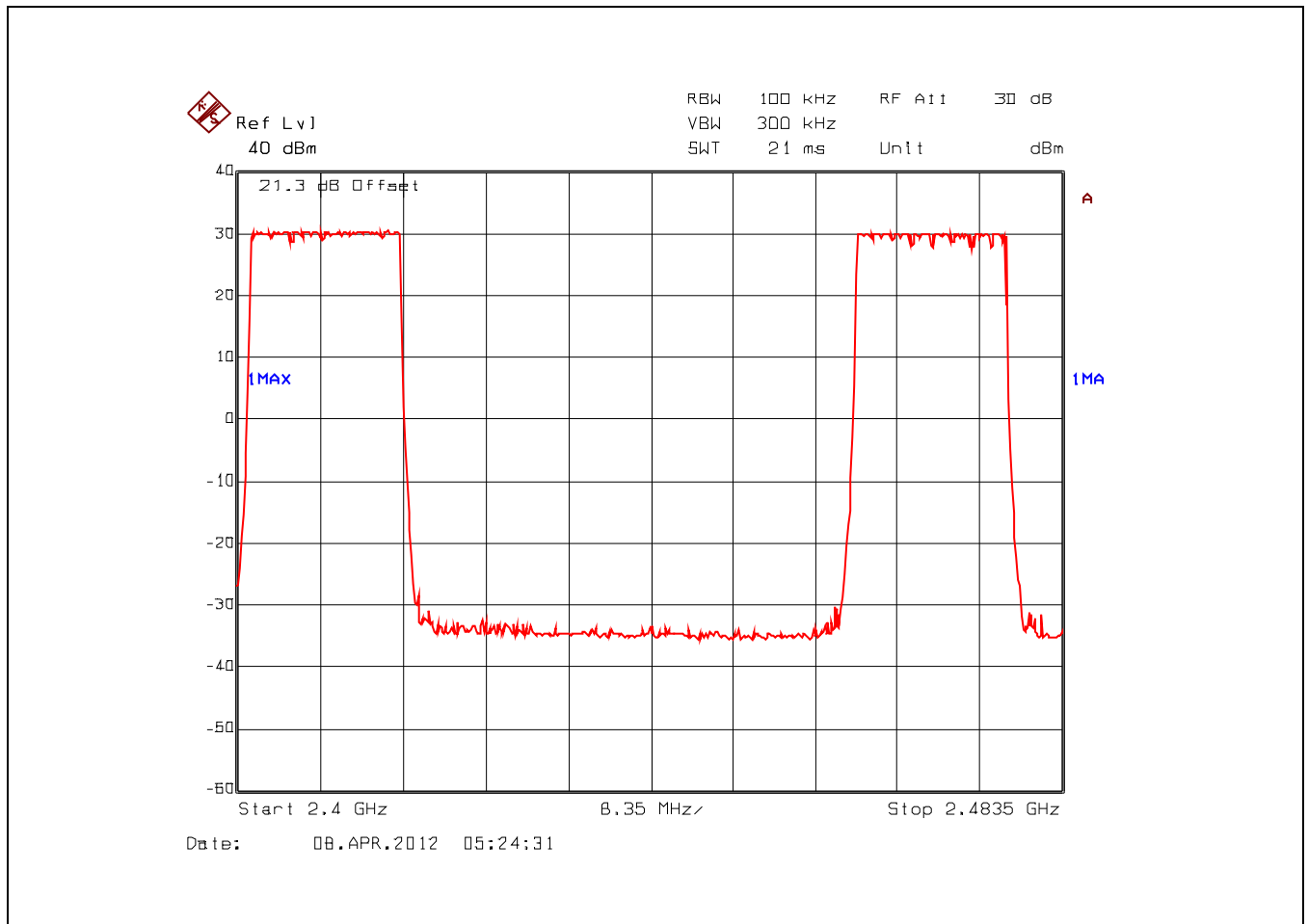
Plot 5.3.4.5. Number of Hopping Frequencies, Data Rate 5 76 Hopping Channels from 2400-2483.5 MHz
