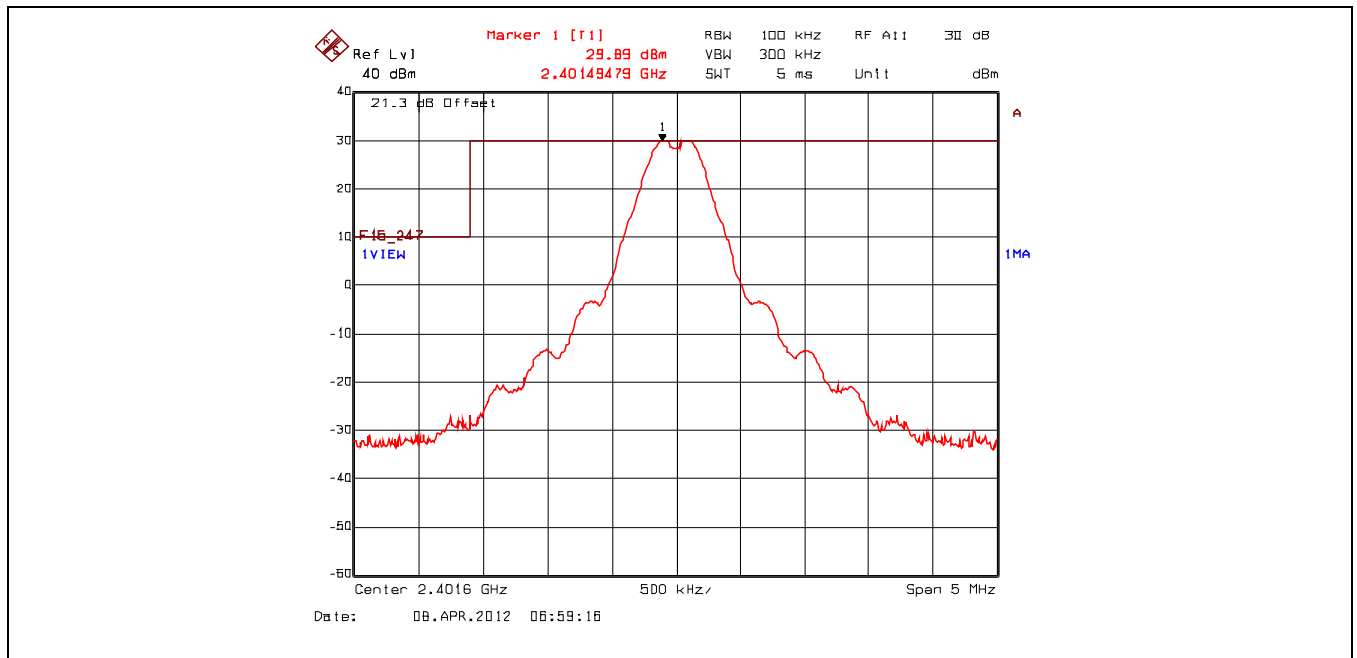
Plot 5.5.4.1.1. Band-Edge RF Conducted Emissions Single Frequency Mode, Low End of Frequency Band, 2401.6 MHz
