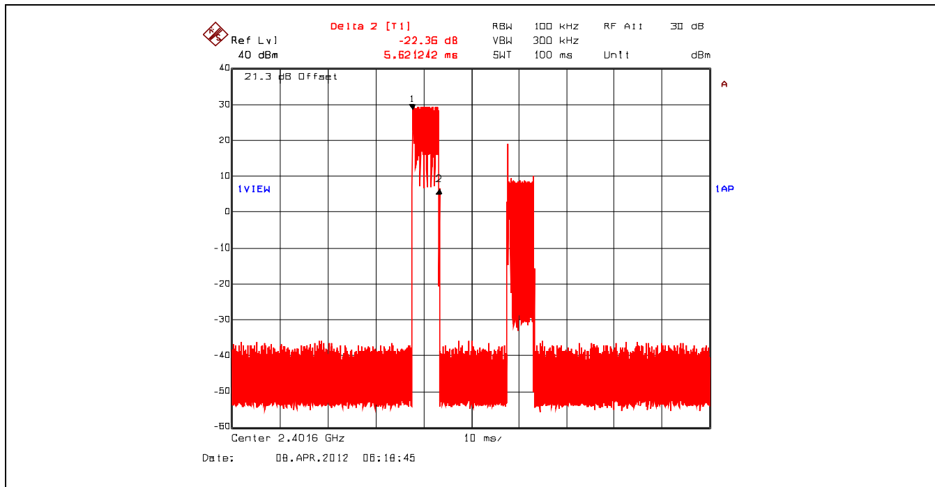
Plot 5.3.4.11. Time of Occupancy, 2401.6 MHz at Data Rate 5 Dwell Time @ 2401.6 MHz = 5.621242 ms
