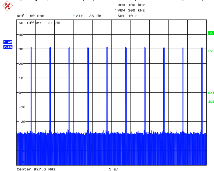
Plot 5.3.5.15. Time of Occupancy, 927.6 MHz, Data Rate 5, High Power, Raw Power setting 235 (0-255) Average time of occupancy = (Dwell Time) x (number of hops within a 10s period) = 17.31 ms x 10 = 173.1 ms
