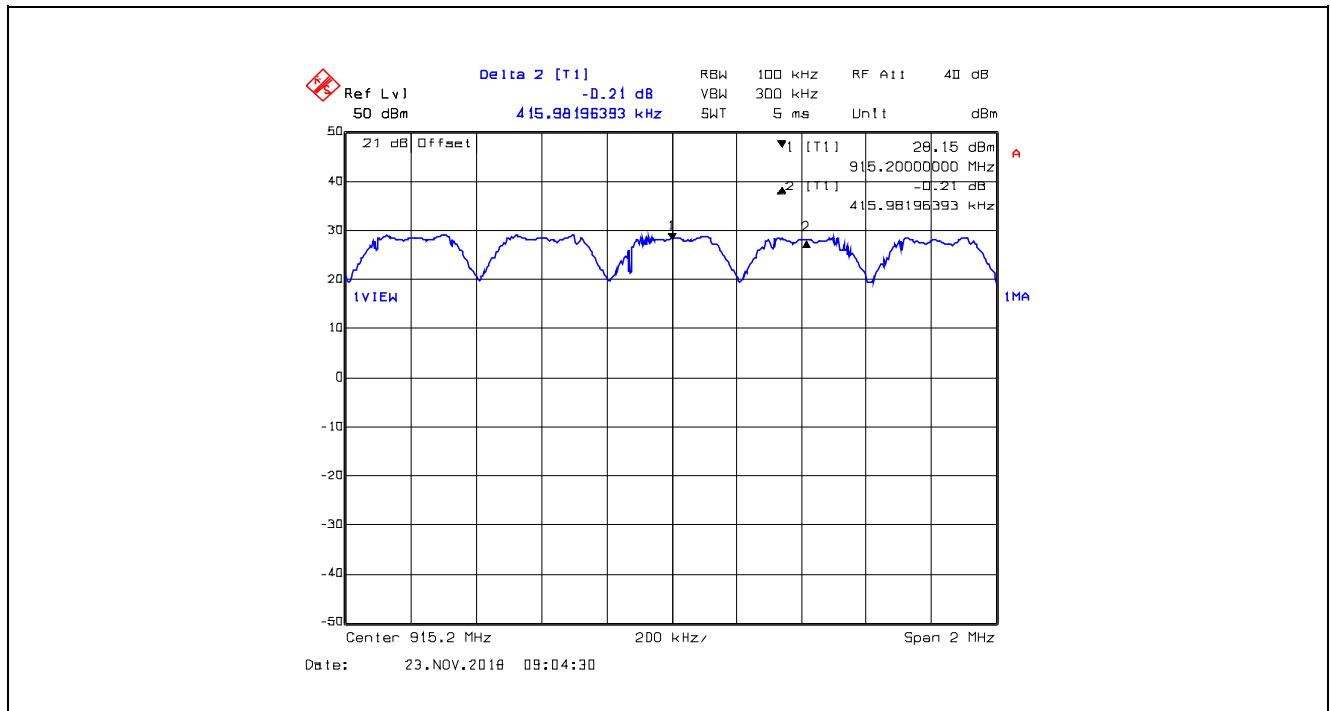
Plot 5.3.4.12. Carrier Frequency Separation, 915 MHz, High Data Rate, 400 kHz CS
