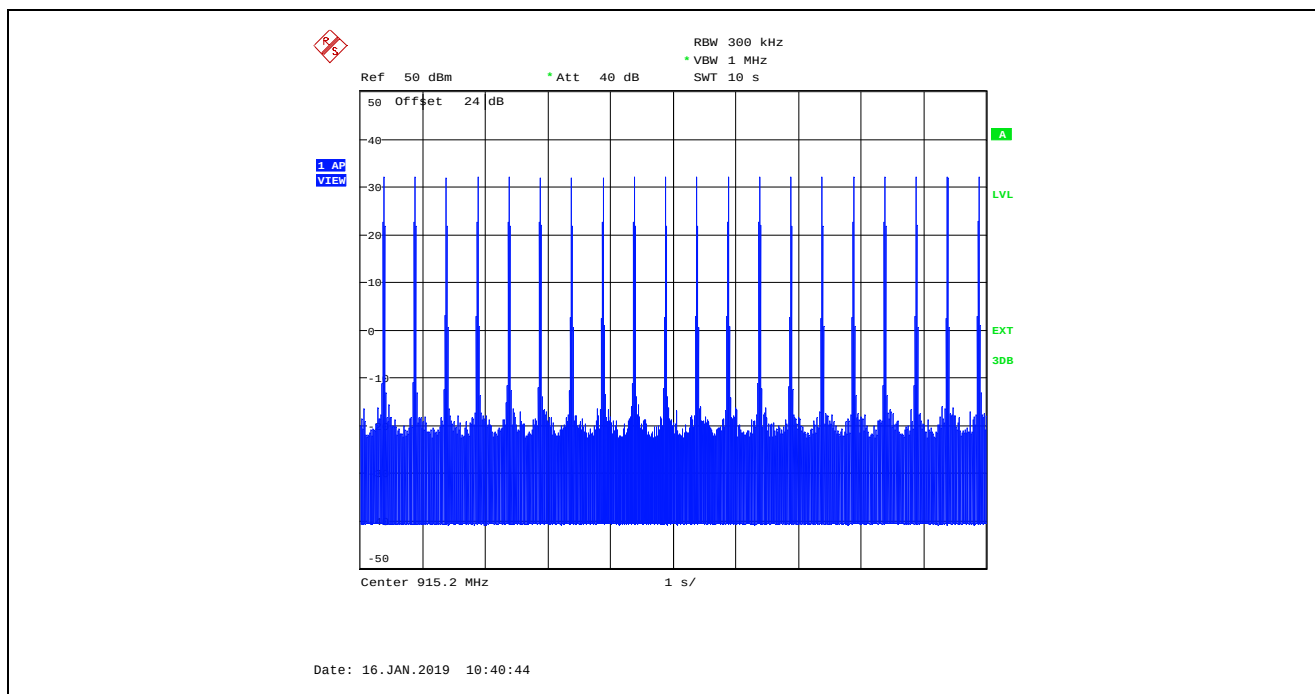
Plot 5.3.4.43. Time of Occupancy, 915.2 MHz, High Data Rate, 400 kHz CS Average time of occupancy = (Dwell Time) x (number of hops within a 10s period) = 975.96 \mu s x 20 = 19.52 ms
