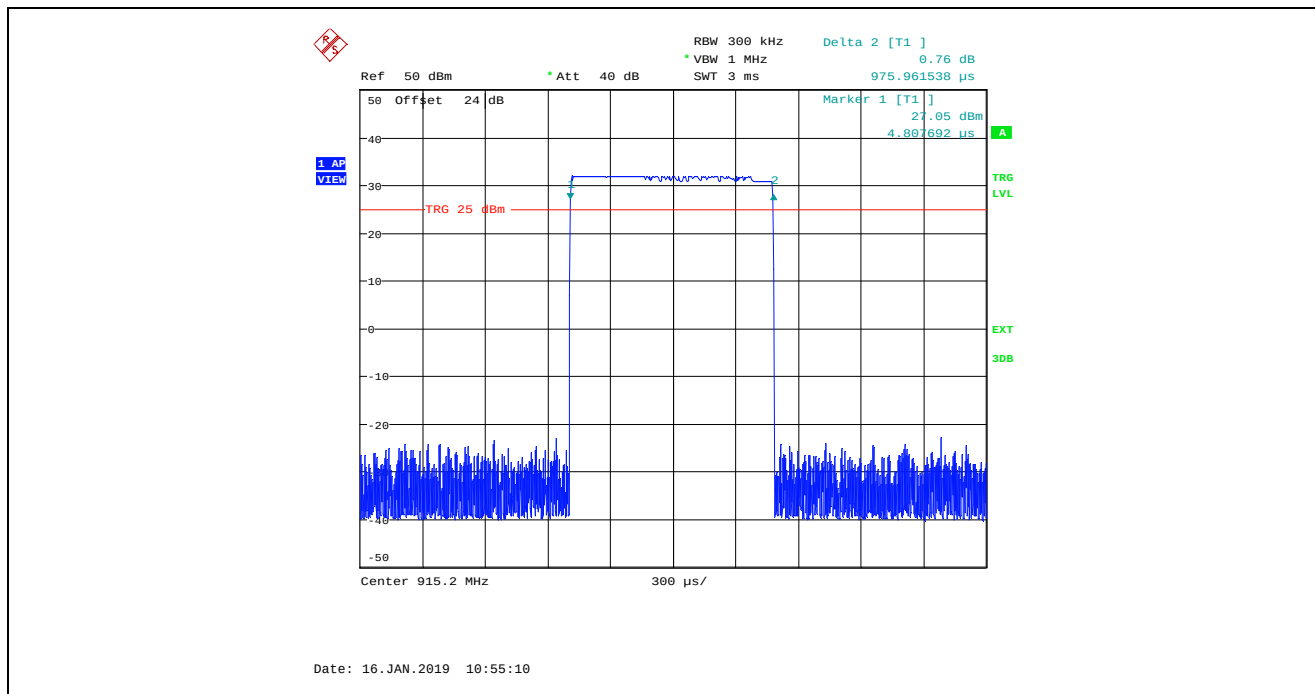
Plot 5.3.4.42. Time of Occupancy, 915.2 MHz, High Data Rate, 400 kHz CS Dwell Time @ 915.2 MHz = 975.96 \mu s
