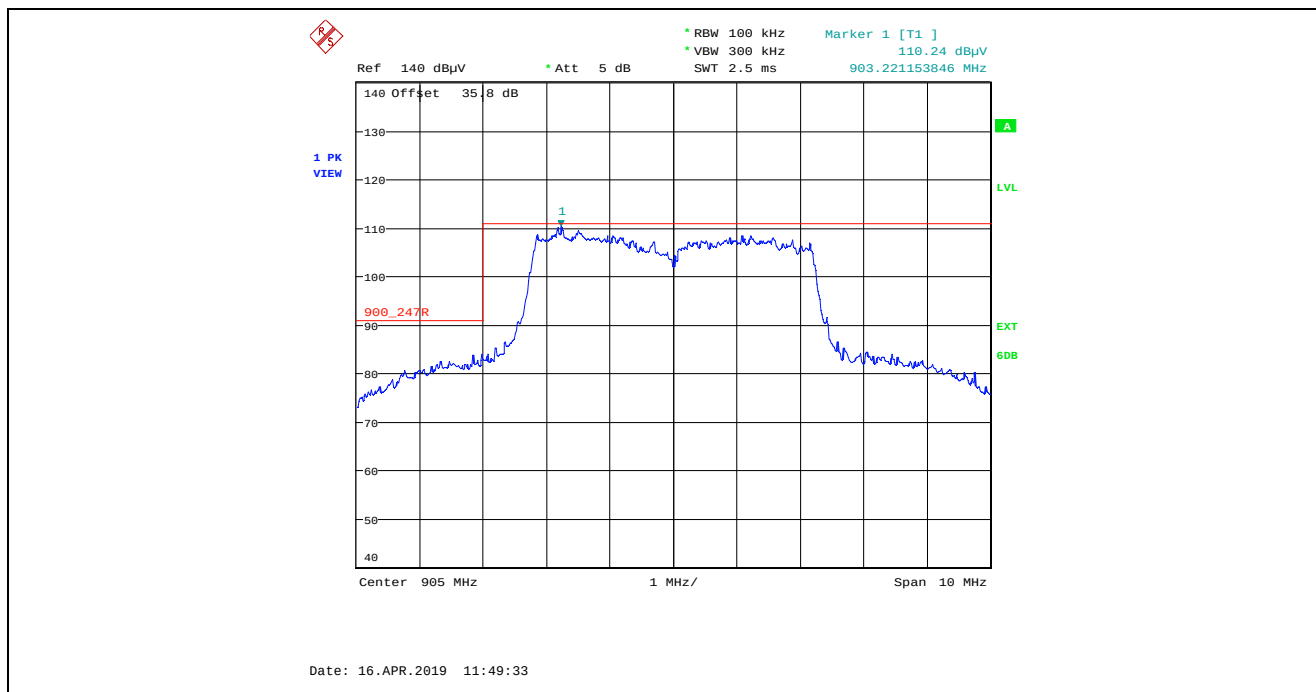
Plot 5.4.4.2.6. Band-Edge RF Radiated Emissions at 3 m, Vertical Polarization Low End of Frequency Band, 4 MHz BW, Tx Gain Setting 23, Data Rate 7
