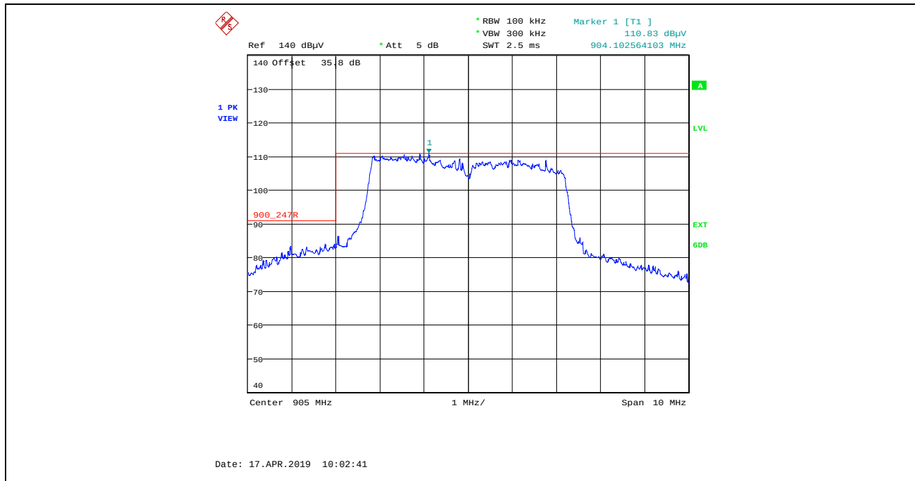
Plot 5.4.4.2.5. Band-Edge RF Radiated Emissions at 3 m, Horizontal Polarization Low End of Frequency Band, 4 MHz BW, Tx Gain Setting 23, Data Rate 7
