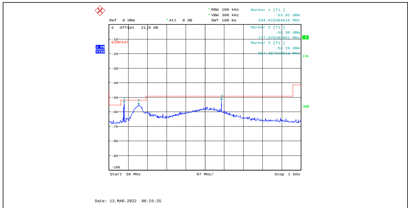
Plot C.2.75. Conducted Spurious Emissions in Restricted Frequency Bands, Chain 1 20 MHz Channel Bandwidth, Data Rate 7, Raw Power Setting 23, 2437 MHz, 30 MHz - 1 GHz, Peak Detector
