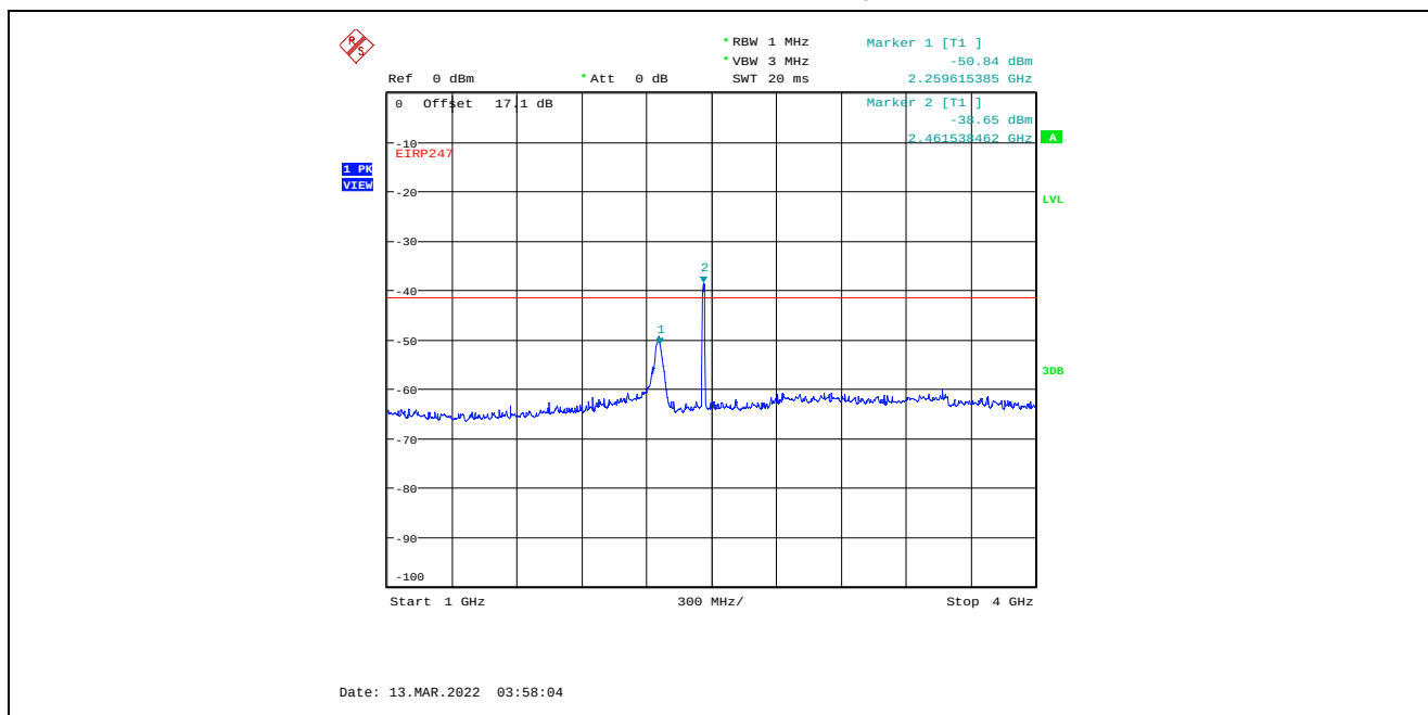
Plot C.1.87. Conducted Spurious Emissions in Restricted Frequency Bands, Chain 1 20 MHz Channel Bandwidth, Data Rate 3, Raw Power Setting 26, 2462 MHz, 1 GHz – 4 GHz, Peak Detector Marker 2 is Fundamental Signal
