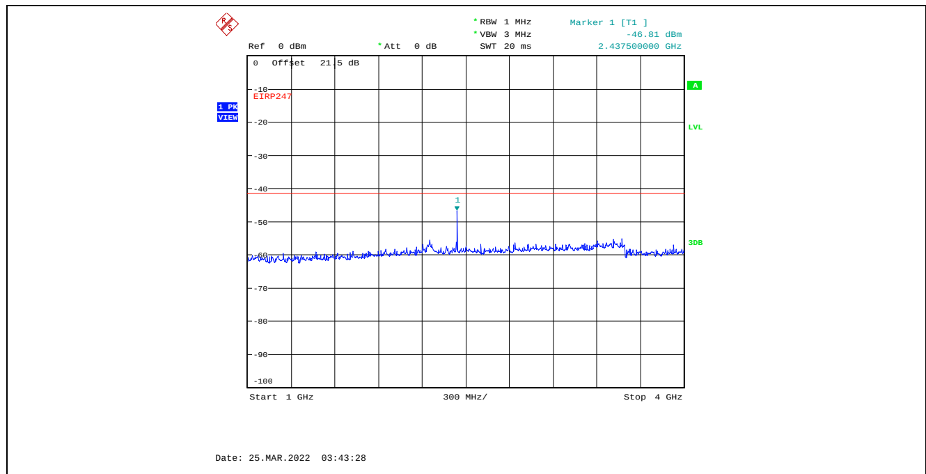
Plot C.3.17. Conducted Spurious Emissions in Restricted Frequency Bands, Chain 1 4 MHz Channel Bandwidth, Data Rate 3, Raw Power Setting 8, 2437 MHz, 1 GHz – 4 GHz, Peak Detector
