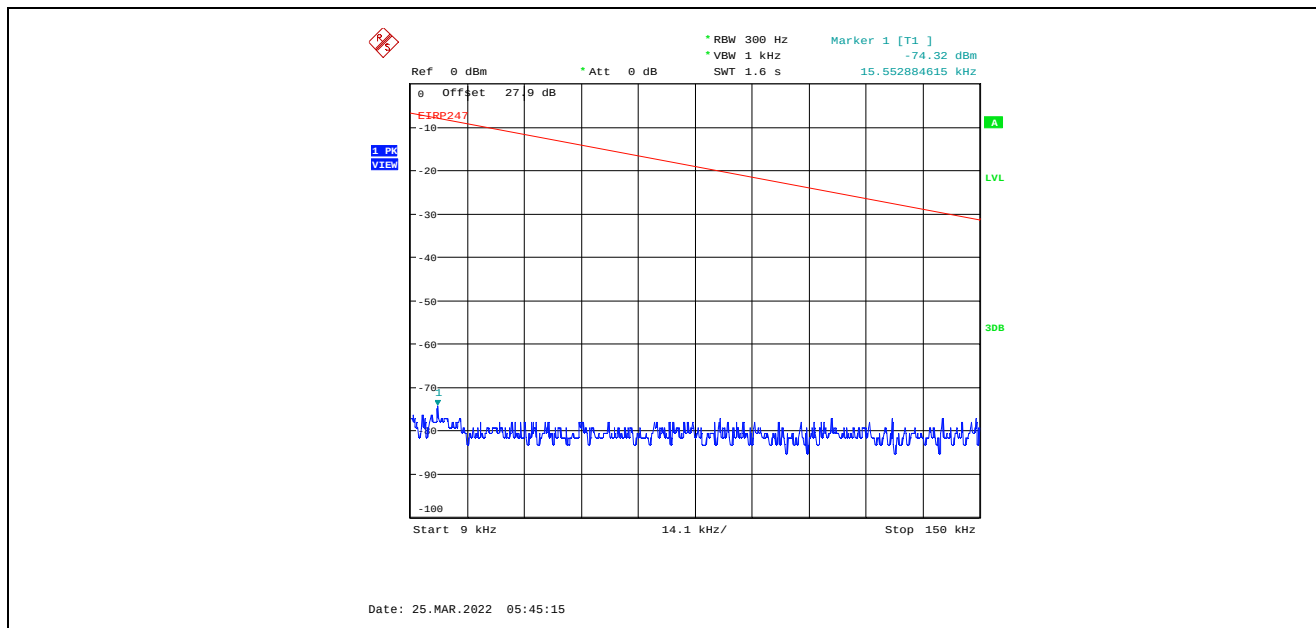
Plot C.4.1. Conducted Spurious Emissions in Restricted Frequency Bands, Chain 1 4 MHz Channel Bandwidth, Data Rate 7, Raw Power Setting 0, 2405 MHz, 9 kHz - 150 kHz, Peak Detector
