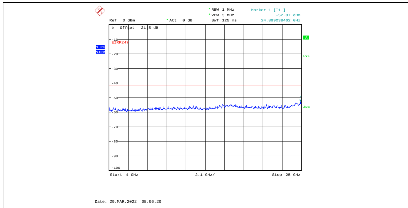
Plot C.3.70. Conducted Spurious Emissions in Restricted Frequency Bands, Chain 2 20 MHz Channel Bandwidth, Data Rate 3, Raw Power Setting 7, 2412 MHz, 4 GHz - 25 GHz, Peak Detector
