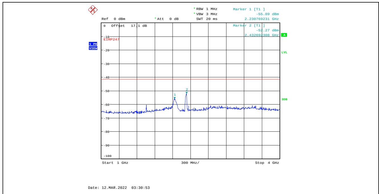
Plot C.1.97. Conducted Spurious Emissions in Restricted Frequency Bands, Chain 1 40 MHz Channel Bandwidth, Data Rate 3, Raw Power Setting 13, 2422 MHz, 1 GHz – 4 GHz, Peak Detector
