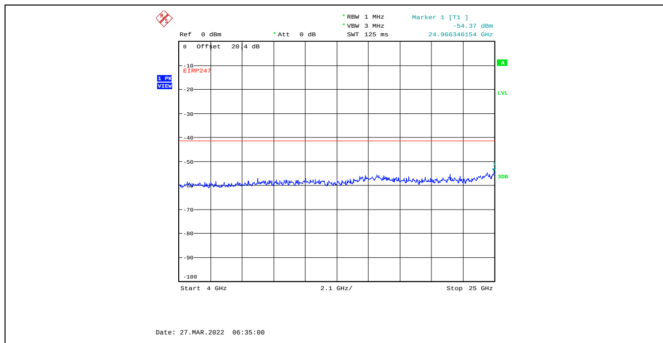
Plot C.3.39. Conducted Spurious Emissions in Restricted Frequency Bands, Chain 1 8 MHz Channel Bandwidth, Data Rate 3, Raw Power Setting 6, 2407 MHz, 4 GHz - 25 GHz, Peak Detector
