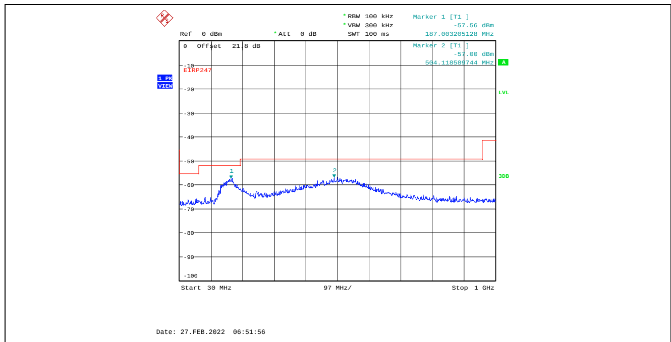
Plot C.1.46. Conducted Spurious Emissions in Restricted Frequency Bands, Chain 2 8 MHz Channel Bandwidth, Data Rate 3, Raw Power Setting 21, 2437 MHz, 30 MHz - 1 GHz, Peak Detector
