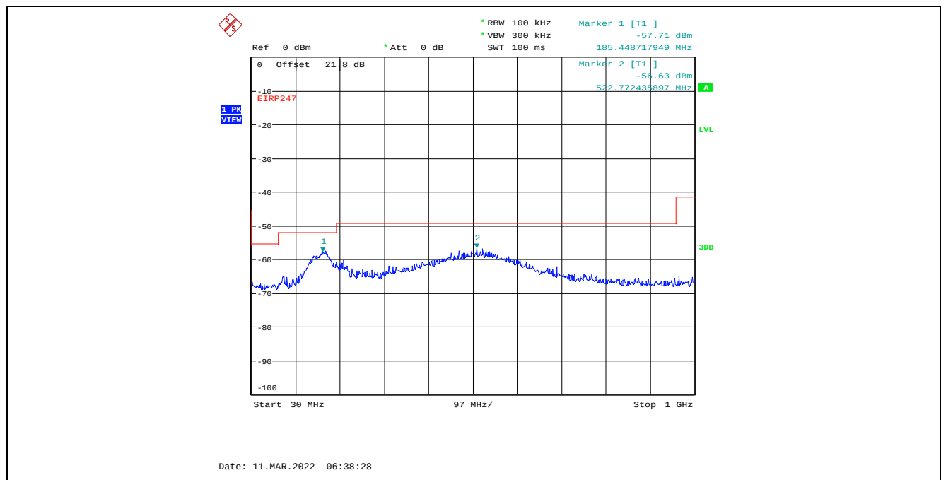
Plot C.1.106. Conducted Spurious Emissions in Restricted Frequency Bands, Chain 2 40 MHz Channel Bandwidth, Data Rate 3, Raw Power Setting 22, 2437 MHz, 30 MHz - 1 GHz, Peak Detector
