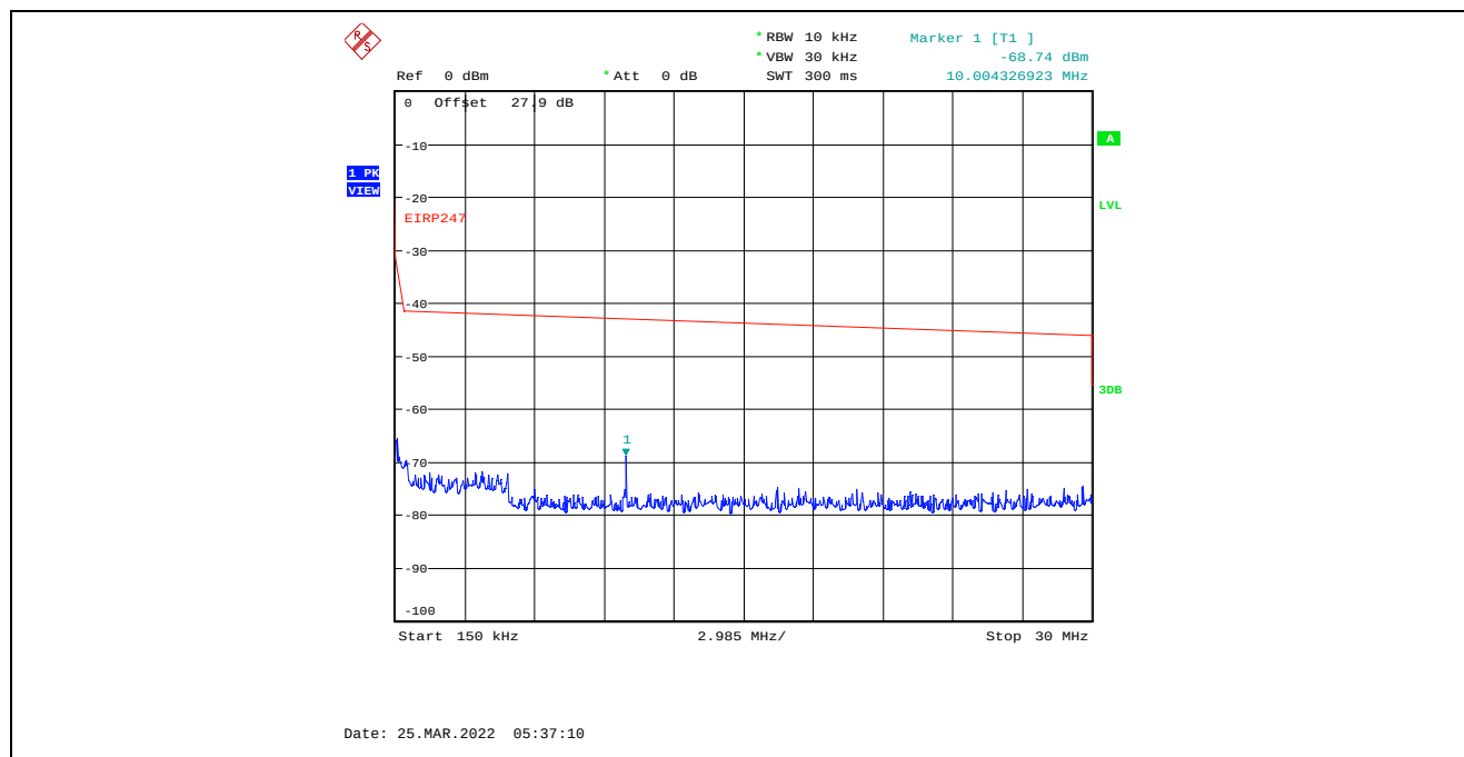
Plot C.4.4. Conducted Spurious Emissions in Restricted Frequency Bands, Chain 2 4 MHz Channel Bandwidth, Data Rate 7, Raw Power Setting 0, 2405 MHz, 150 kHz – 30 MHz, Peak Detector
