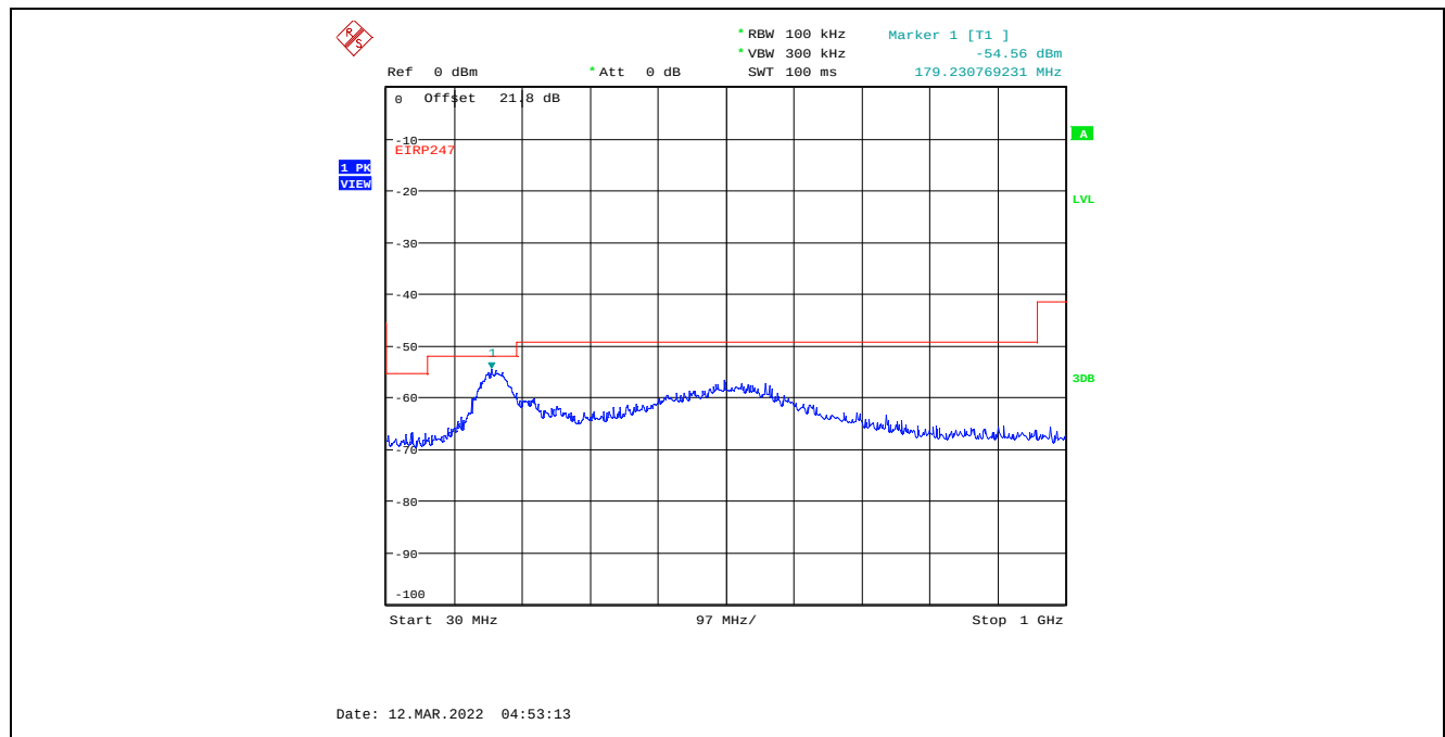
Plot C.2.116. Conducted Spurious Emissions in Restricted Frequency Bands, Chain 2 40 MHz Channel Bandwidth, Data Rate 7, Raw Power Setting 22, 2452 MHz, 30 MHz - 1 GHz, Peak Detector
