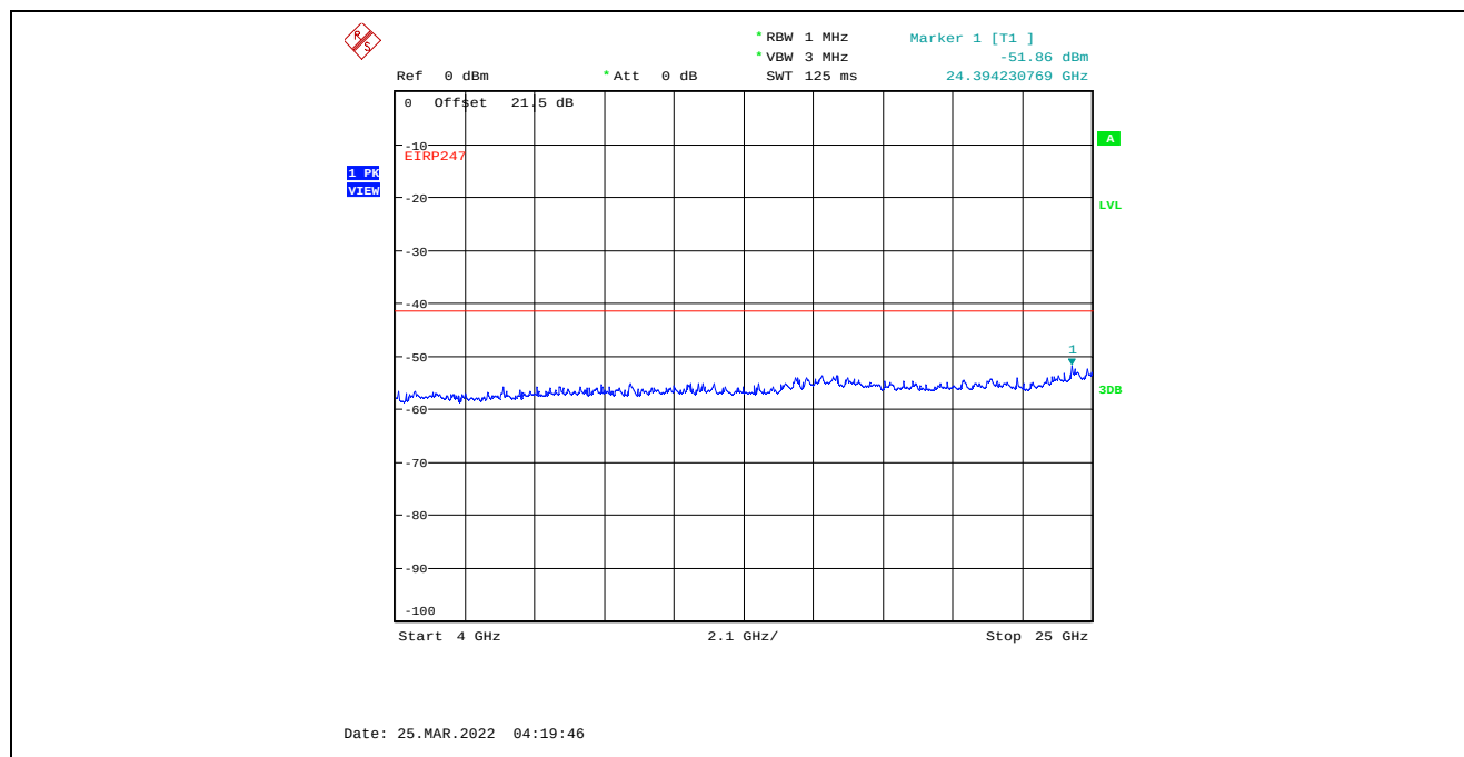
Plot C.4.10. Conducted Spurious Emissions in Restricted Frequency Bands, Chain 2 4 MHz Channel Bandwidth, Data Rate 7, Raw Power Setting 0, 2405 MHz, 4 GHz - 25 GHz, Peak Detector
