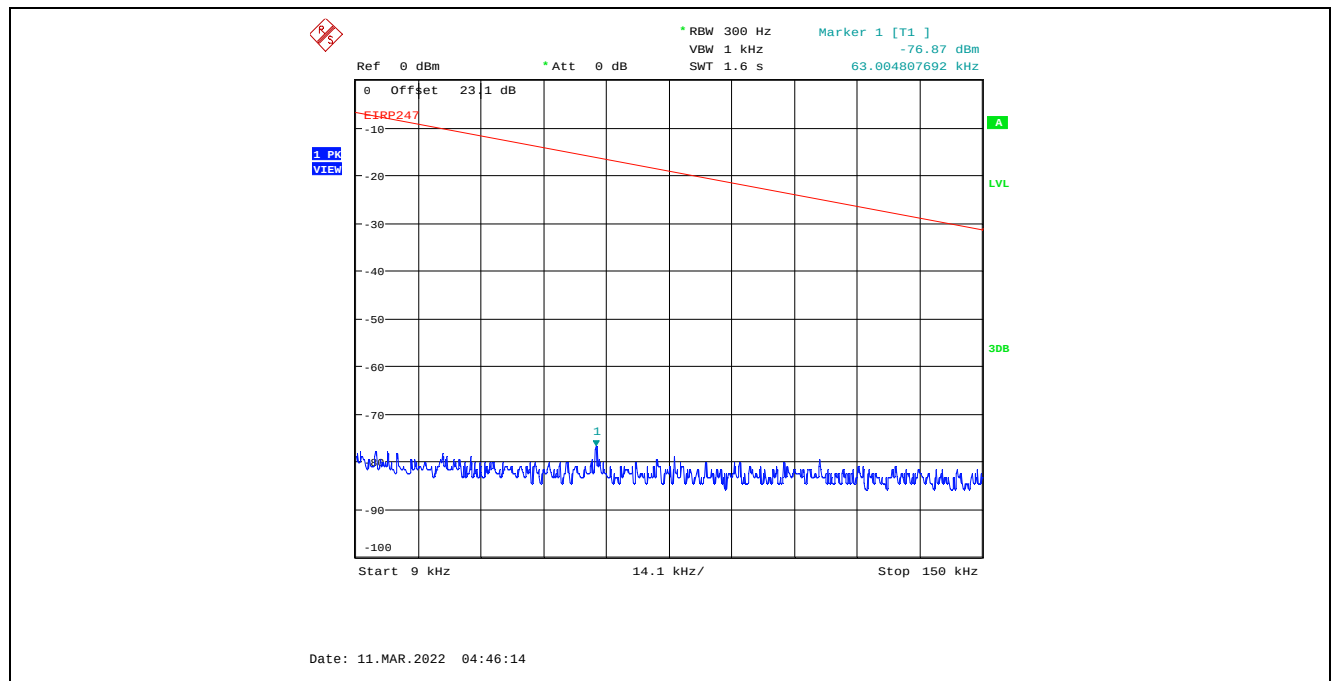
Plot C.1.101. Conducted Spurious Emissions in Restricted Frequency Bands, Chain 1 40 MHz Channel Bandwidth, Data Rate 3, Raw Power Setting 22, 2437 MHz, 9 kHz - 150 kHz, Peak Detector
