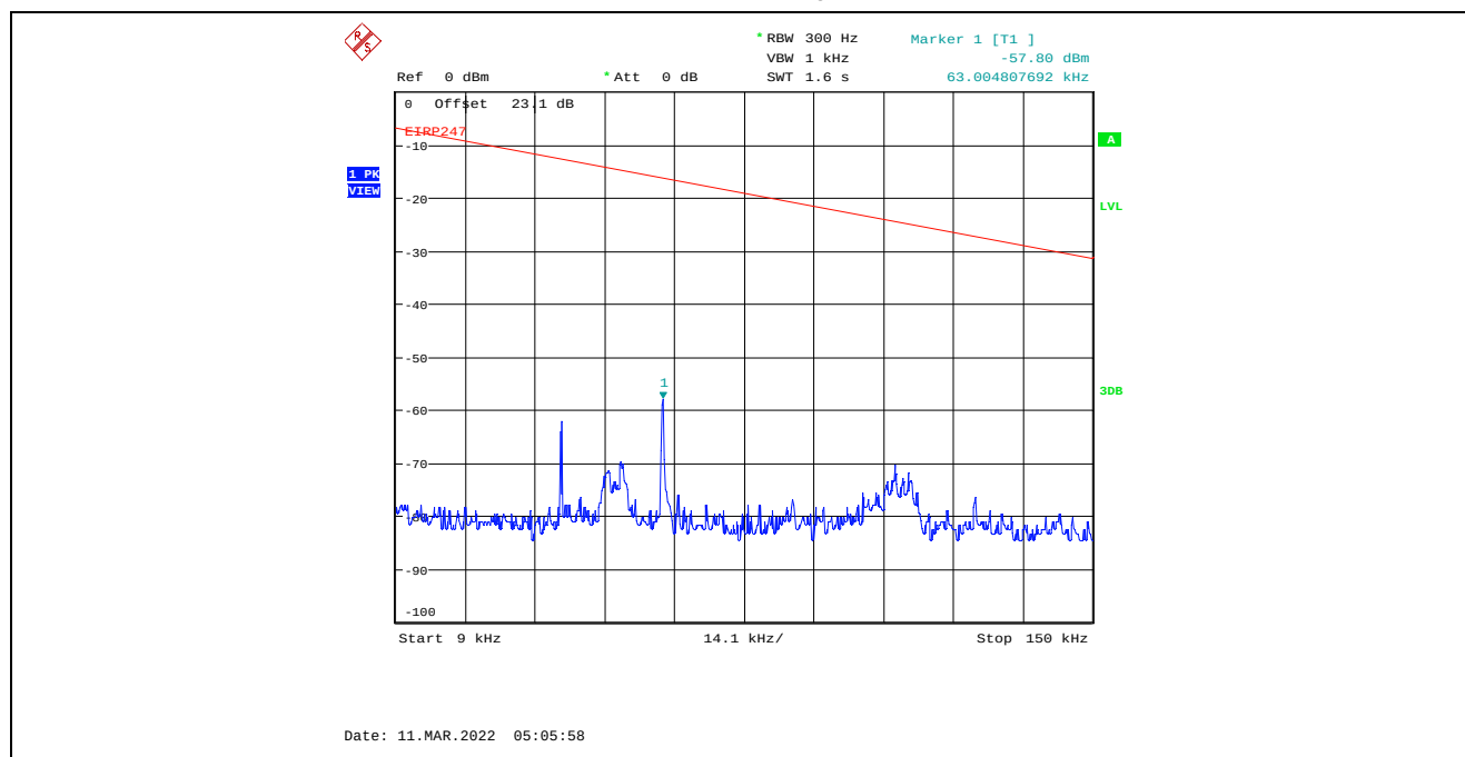
Plot C.1.92. Conducted Spurious Emissions in Restricted Frequency Bands, Chain 2 40 MHz Channel Bandwidth, Data Rate 3, Raw Power Setting 13, 2422 MHz, 9 kHz - 150 kHz, Peak Detector
