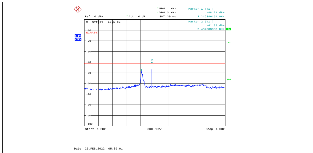
Plot C.2.18. Conducted Spurious Emissions in Restricted Frequency Bands, Chain 2 4 MHz Channel Bandwidth, Data Rate 7, Raw Power Setting 22, 2437 MHz, 1 GHz – 4 GHz, Peak Detector Marker 2 is Fundamental Signal
