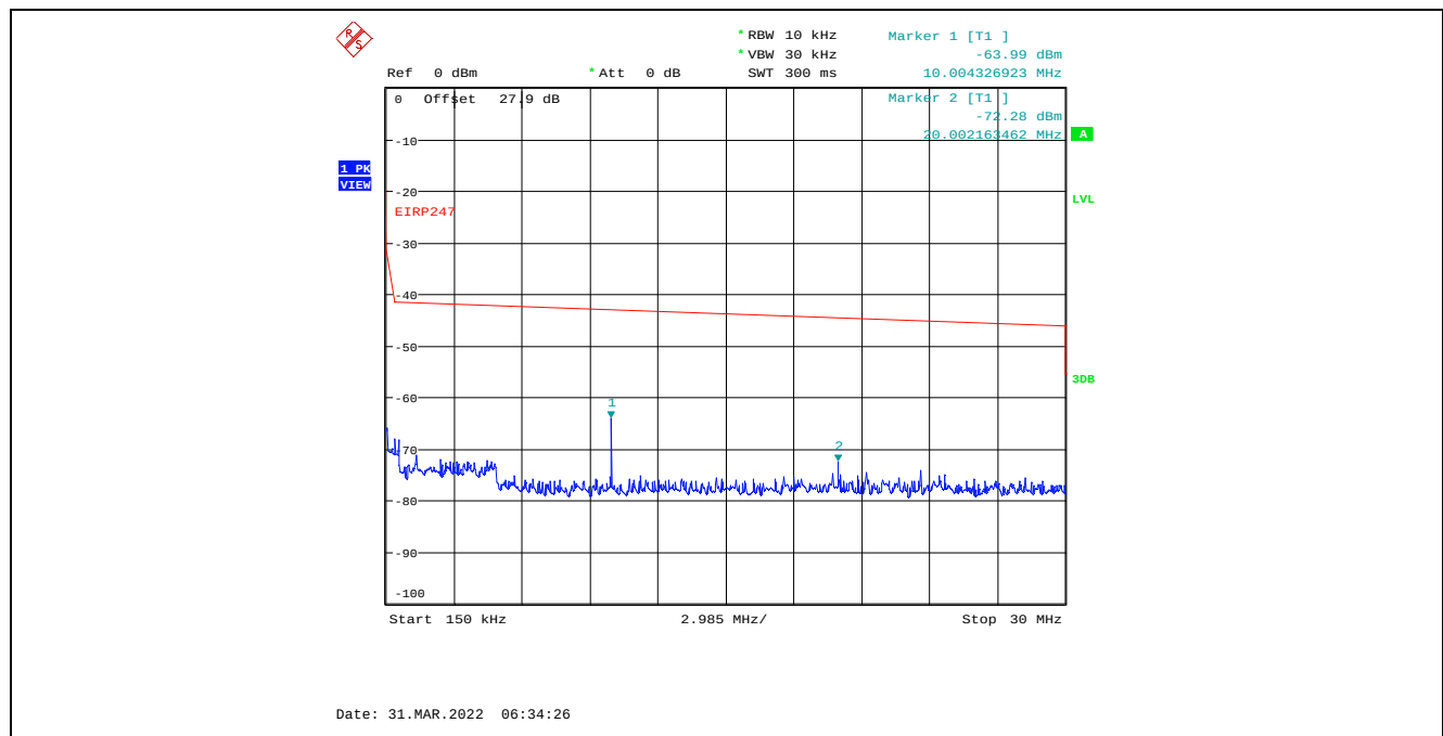
Plot C.4.94. Conducted Spurious Emissions in Restricted Frequency Bands, Chain 2 40 MHz Channel Bandwidth, Data Rate 7, Raw Power Setting 0, 2422 MHz, 150 kHz – 30 MHz, Peak Detector
