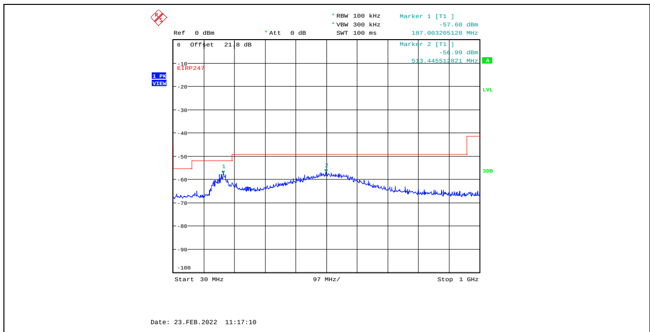
Plot C.1.16. Conducted Spurious Emissions in Restricted Frequency Bands, Chain 2 4 MHz Channel Bandwidth, Data Rate 3, Raw Power Setting 16, 2437 MHz, 30 MHz - 1 GHz, Peak Detector
