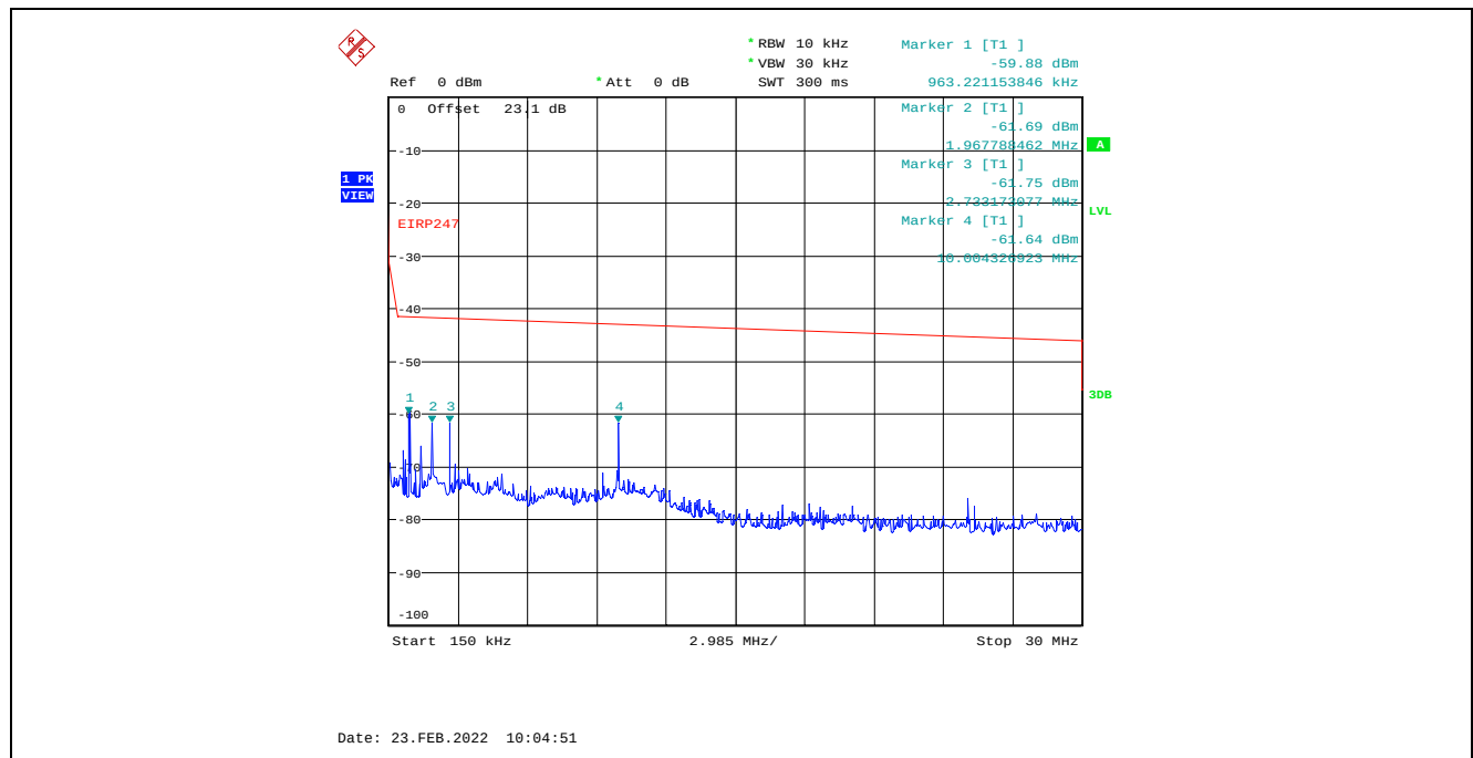
Plot C.1.4. Conducted Spurious Emissions in Restricted Frequency Bands, Chain 2 4 MHz Channel Bandwidth, Data Rate 3, Raw Power Setting 16, 2402 MHz, 150 kHz – 30 MHz, Peak Detector
