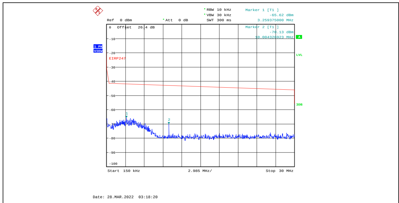
Plot C.4.44. Conducted Spurious Emissions in Restricted Frequency Bands, Chain 2 8 MHz Channel Bandwidth, Data Rate 7, Raw Power Setting 0, 2437 MHz, 150 kHz – 30 MHz, Peak Detector
