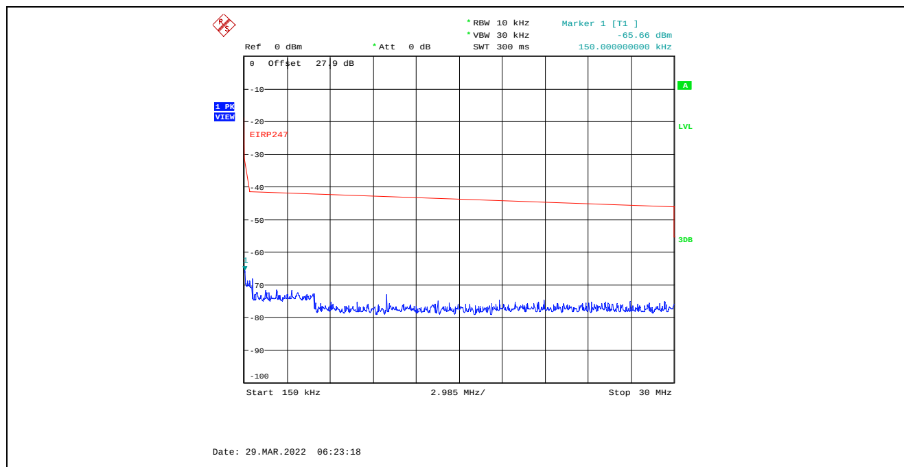
Plot C.4.83. Conducted Spurious Emissions in Restricted Frequency Bands, Chain 1 20 MHz Channel Bandwidth, Data Rate 7, Raw Power Setting 0, 2462 MHz, 150 kHz – 30 MHz, Peak Detector
