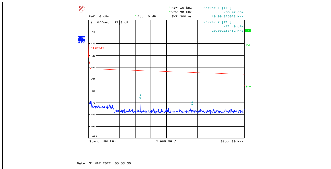
Plot C.3.103. Conducted Spurious Emissions in Restricted Frequency Bands, Chain 1 40 MHz Channel Bandwidth, Data Rate 3, Raw Power Setting 0, 2437 MHz, 150 kHz – 30 MHz, Peak Detector
