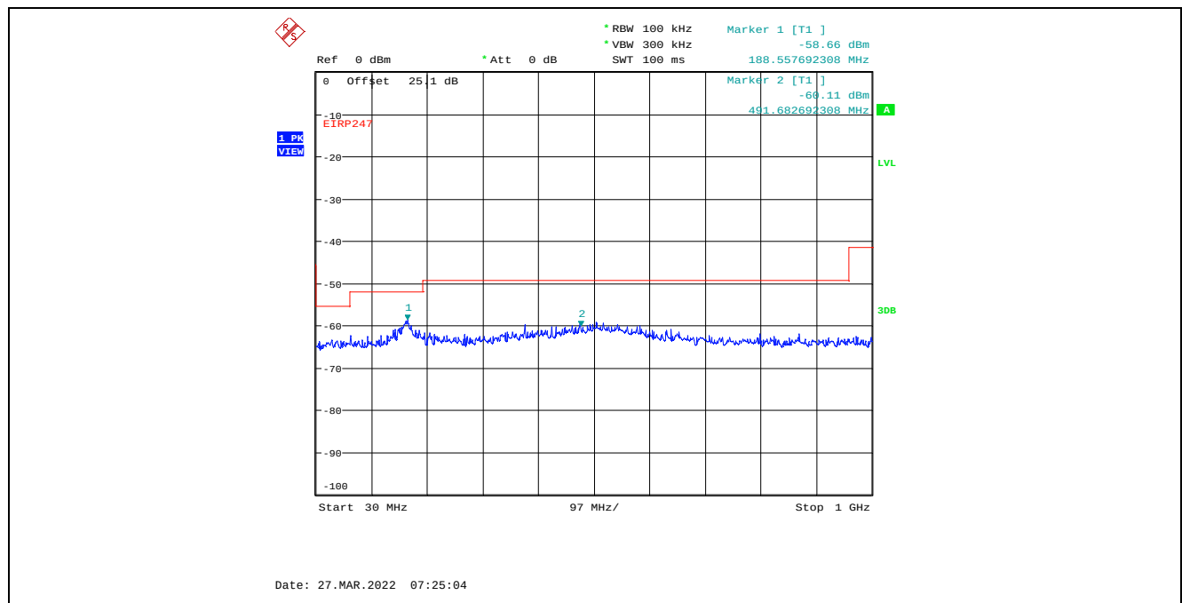
Plot C.4.46. Conducted Spurious Emissions in Restricted Frequency Bands, Chain 2 8 MHz Channel Bandwidth, Data Rate 7, Raw Power Setting 0, 2437 MHz, 30 MHz - 1 GHz, Peak Detector
