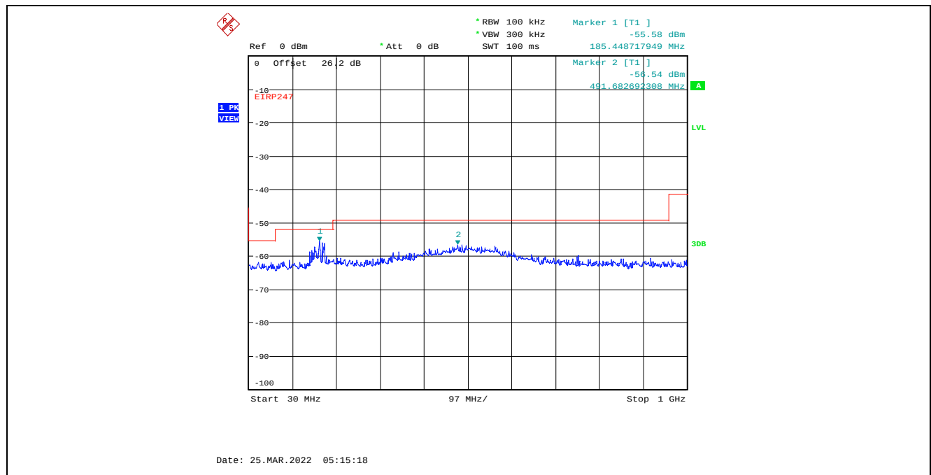
Plot C.4.6. Conducted Spurious Emissions in Restricted Frequency Bands, Chain 1 4 MHz Channel Bandwidth, Data Rate 7, Raw Power Setting 0, 2405 MHz, 30 MHz - 1 GHz, Peak Detector
