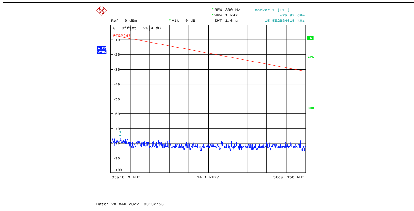
Plot C.4.51. Conducted Spurious Emissions in Restricted Frequency Bands, Chain 1 8 MHz Channel Bandwidth, Data Rate 7, Raw Power Setting 0, 2476 MHz, 9 kHz - 150 kHz, Peak Detector
