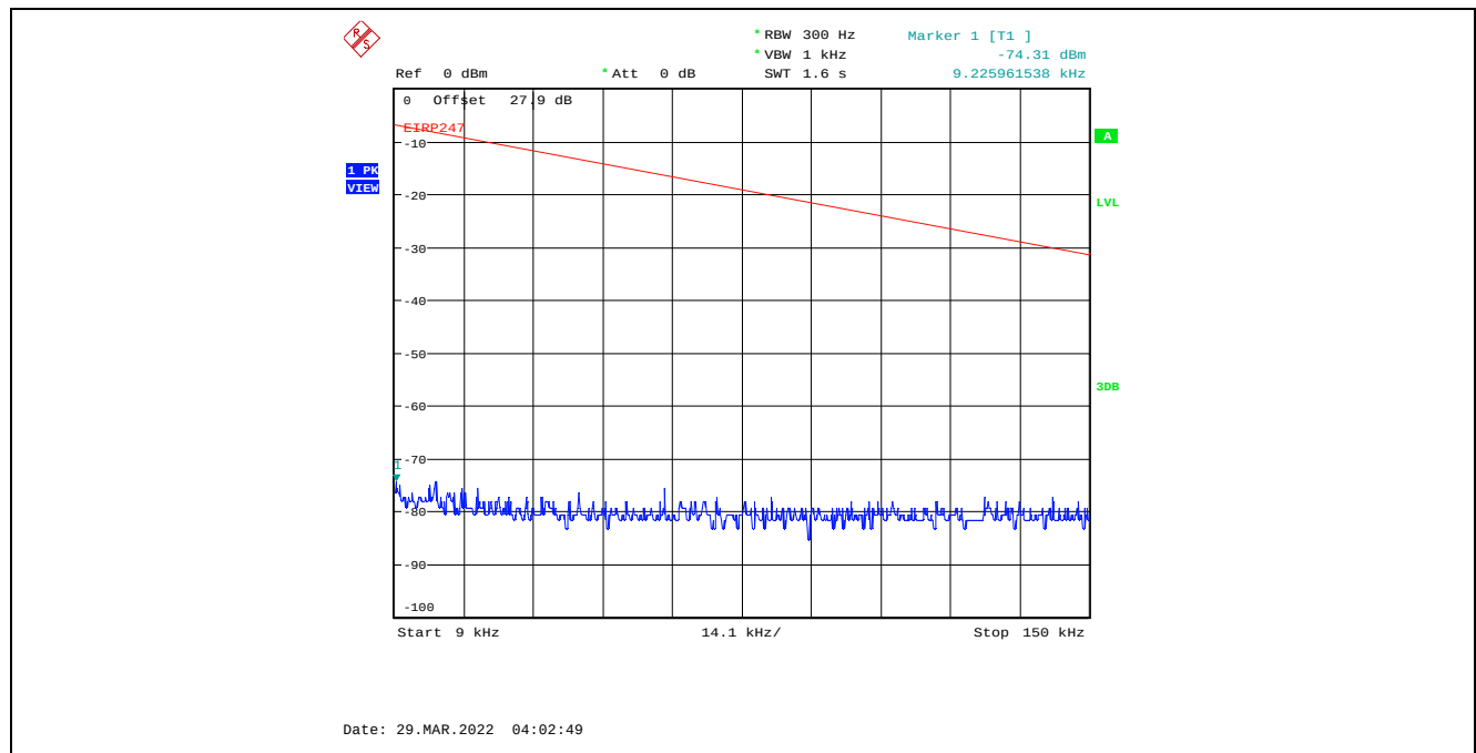
Plot C.3.62. Conducted Spurious Emissions in Restricted Frequency Bands, Chain 2 20 MHz Channel Bandwidth, Data Rate 3, Raw Power Setting 7, 2412 MHz, 9 kHz - 150 kHz, Peak Detector
