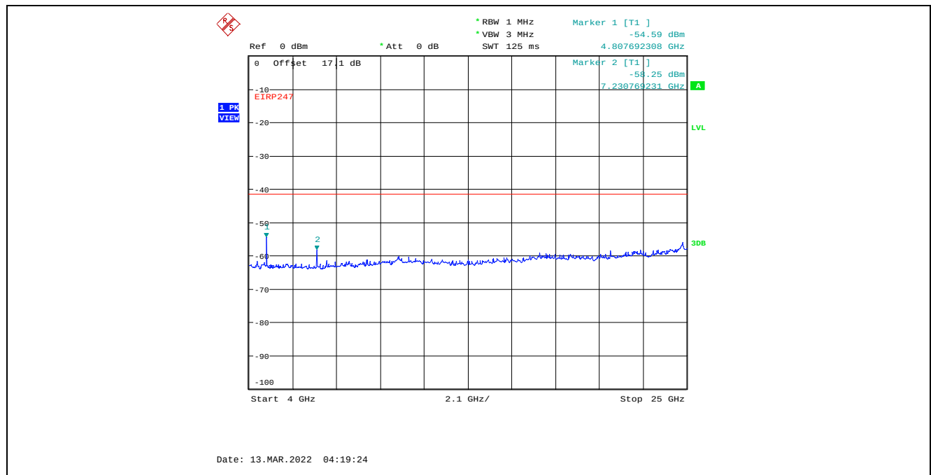
Plot C.1.69. Conducted Spurious Emissions in Restricted Frequency Bands, Chain 1 20 MHz Channel Bandwidth, Data Rate 3, Raw Power Setting 26, 2412 MHz, 4 GHz - 25 GHz, Peak Detector
