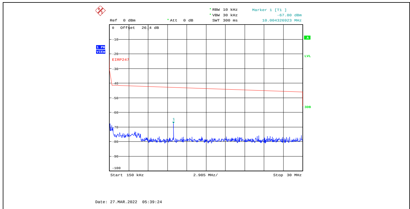
Plot C.3.33. Conducted Spurious Emissions in Restricted Frequency Bands, Chain 1 8 MHz Channel Bandwidth, Data Rate 3, Raw Power Setting 6, 2407 MHz, 150 kHz – 30 MHz, Peak Detector
