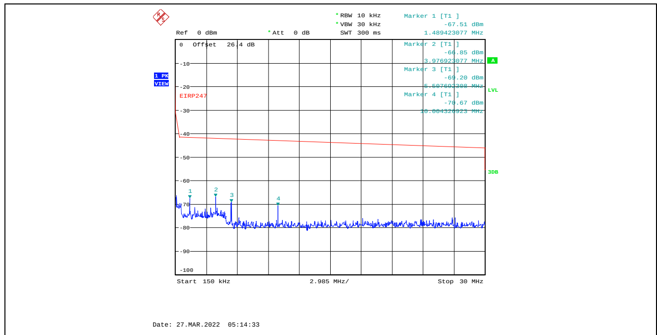
Plot C.3.34. Conducted Spurious Emissions in Restricted Frequency Bands, Chain 2 8 MHz Channel Bandwidth, Data Rate 3, Raw Power Setting 6, 2407 MHz, 150 kHz – 30 MHz, Peak Detector
