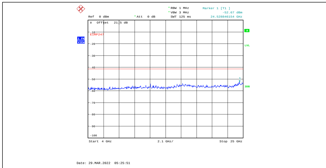
Plot C.4.80. Conducted Spurious Emissions in Restricted Frequency Bands, Chain 2 20 MHz Channel Bandwidth, Data Rate 7, Raw Power Setting 0, 2437 MHz, 4 GHz - 25 GHz, Peak Detector
