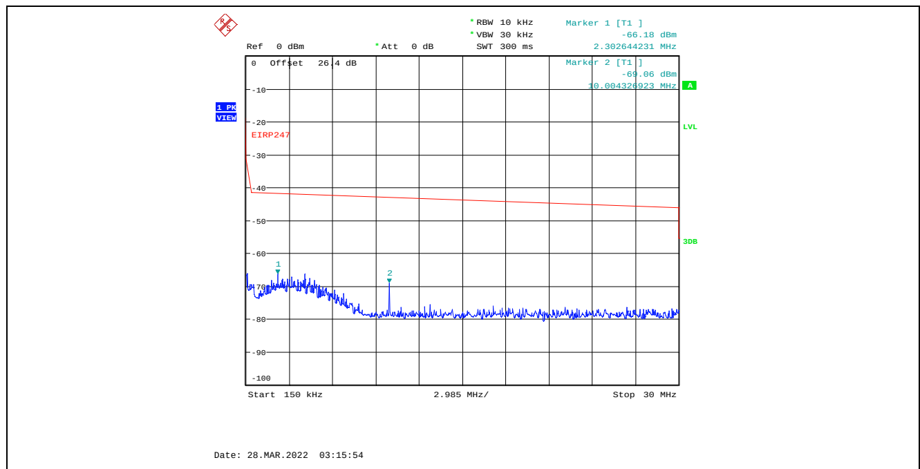
Plot C.4.34. Conducted Spurious Emissions in Restricted Frequency Bands, Chain 2 8 MHz Channel Bandwidth, Data Rate 7, Raw Power Setting 0, 2407 MHz, 150 kHz – 30 MHz, Peak Detector
