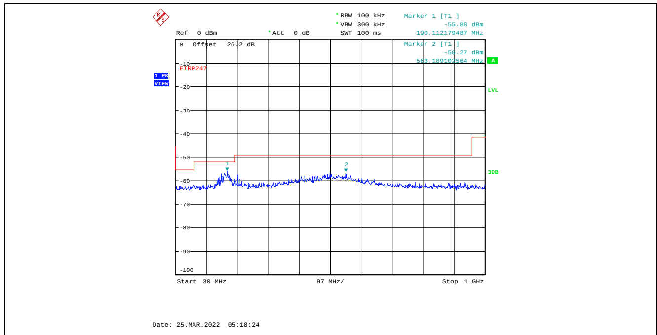
Plot C.4.16. Conducted Spurious Emissions in Restricted Frequency Bands, Chain 2 4 MHz Channel Bandwidth, Data Rate 7, Raw Power Setting 0, 2437 MHz, 30 MHz - 1 GHz, Peak Detector
