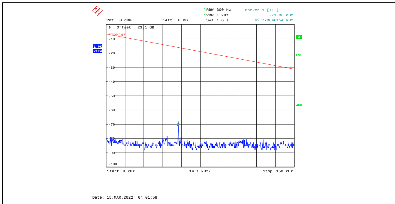
Plot C.2.22. Conducted Spurious Emissions in Restricted Frequency Bands, Chain 2 4 MHz Channel Bandwidth, Data Rate 7, Raw Power Setting 20, 2477 MHz, 9 kHz - 150 kHz, Peak Detector
