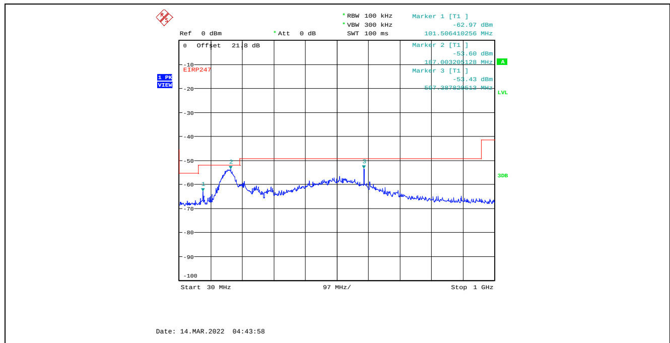
Plot C.2.55. Conducted Spurious Emissions in Restricted Frequency Bands, Chain 1 8 MHz Channel Bandwidth, Data Rate 7, Raw Power Setting 12, 2476 MHz, 30 MHz - 1 GHz, Peak Detector
