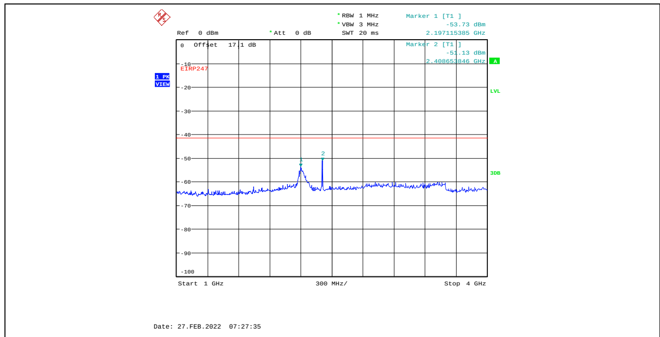
Plot C.2.38. Conducted Spurious Emissions in Restricted Frequency Bands, Chain 2 8 MHz Channel Bandwidth, Data Rate 7, Raw Power Setting 23, 2407 MHz, 1 GHz – 4 GHz, Peak Detector
