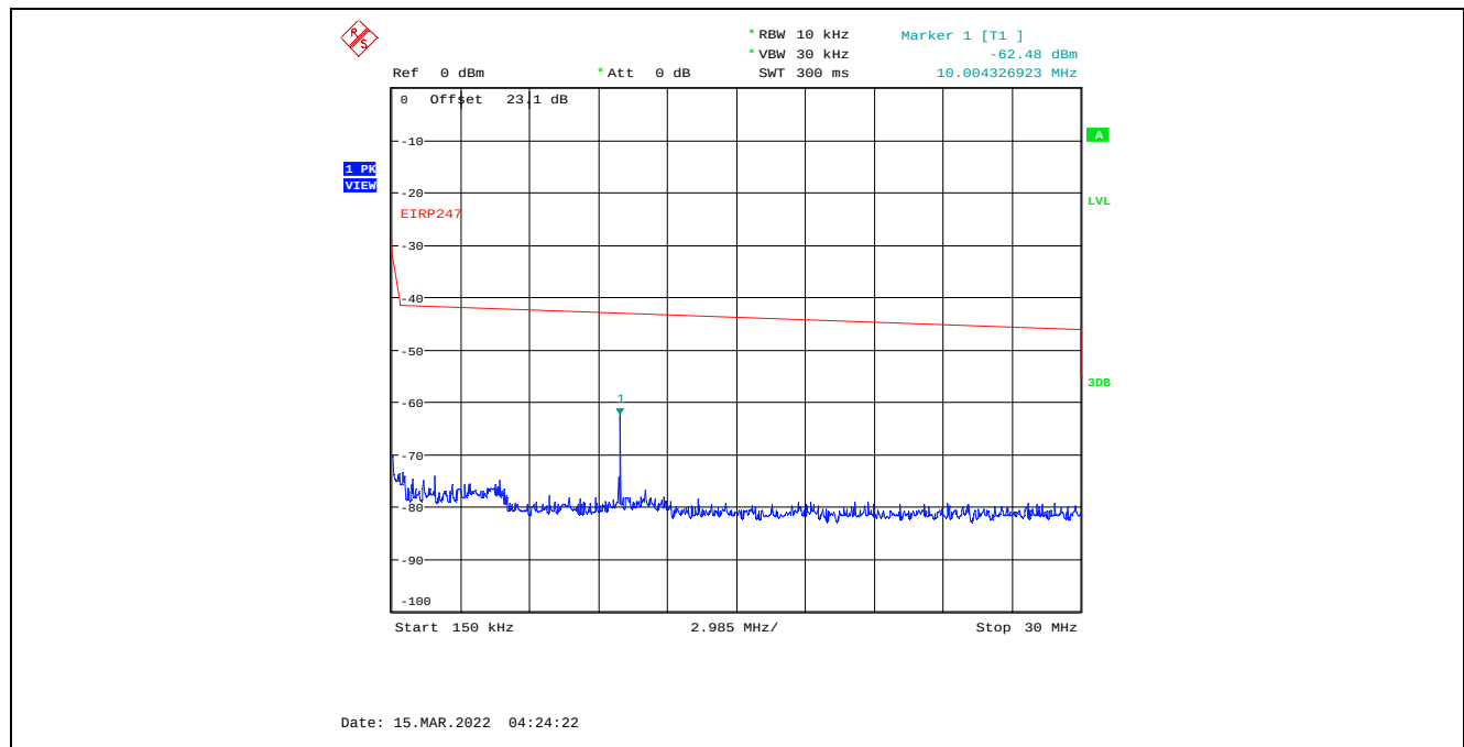
Plot C.2.23. Conducted Spurious Emissions in Restricted Frequency Bands, Chain 1 4 MHz Channel Bandwidth, Data Rate 7, Raw Power Setting 20, 2477 MHz, 150 kHz – 30 MHz, Peak Detector
