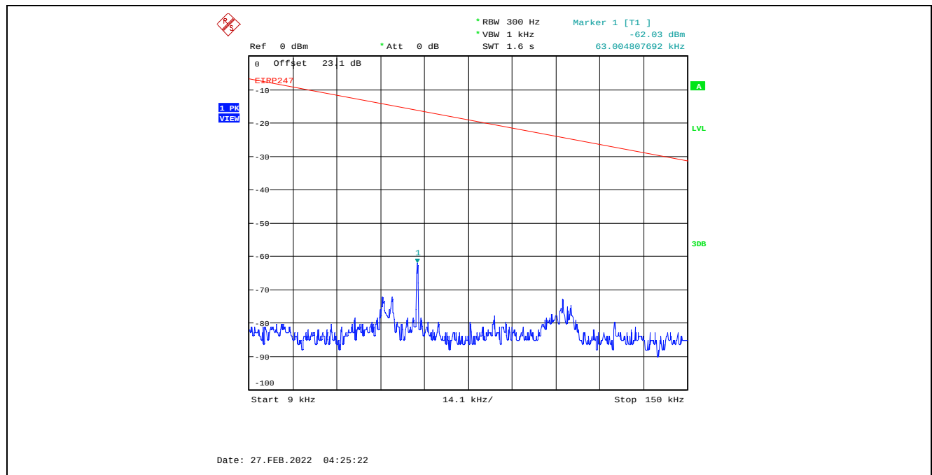
Plot C.2.42. Conducted Spurious Emissions in Restricted Frequency Bands, Chain 2 8 MHz Channel Bandwidth, Data Rate 7, Raw Power Setting 23, 2437 MHz, 9 kHz - 150 kHz, Peak Detector
