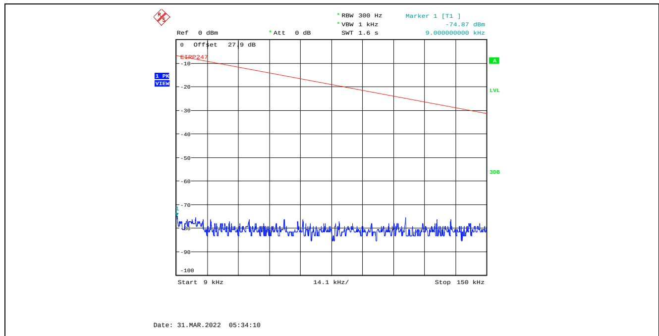
Plot C.4.101. Conducted Spurious Emissions in Restricted Frequency Bands, Chain 1 40 MHz Channel Bandwidth, Data Rate 7, Raw Power Setting 0, 2437 MHz, 9 kHz - 150 kHz, Peak Detector
