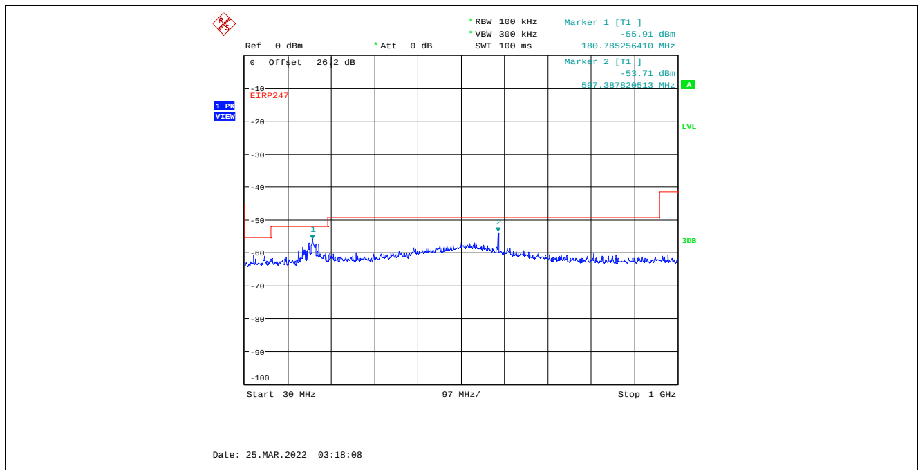
Plot C.3.5. Conducted Spurious Emissions in Restricted Frequency Bands, Chain 1 4 MHz Channel Bandwidth, Data Rate 3, Raw Power Setting 8, 2402 MHz, 30 MHz - 1 GHz, Peak Detector
