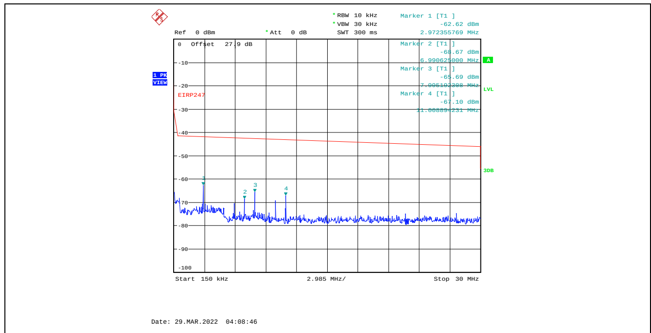
Plot C.3.73. Conducted Spurious Emissions in Restricted Frequency Bands, Chain 1 20 MHz Channel Bandwidth, Data Rate 3, Raw Power Setting 7, 2437 MHz, 150 kHz – 30 MHz, Peak Detector
