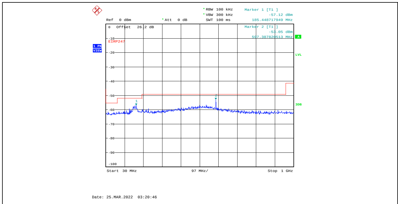
Plot C.3.15. Conducted Spurious Emissions in Restricted Frequency Bands, Chain 1 4 MHz Channel Bandwidth, Data Rate 3, Raw Power Setting 8, 2437 MHz, 30 MHz - 1 GHz, Peak Detector
