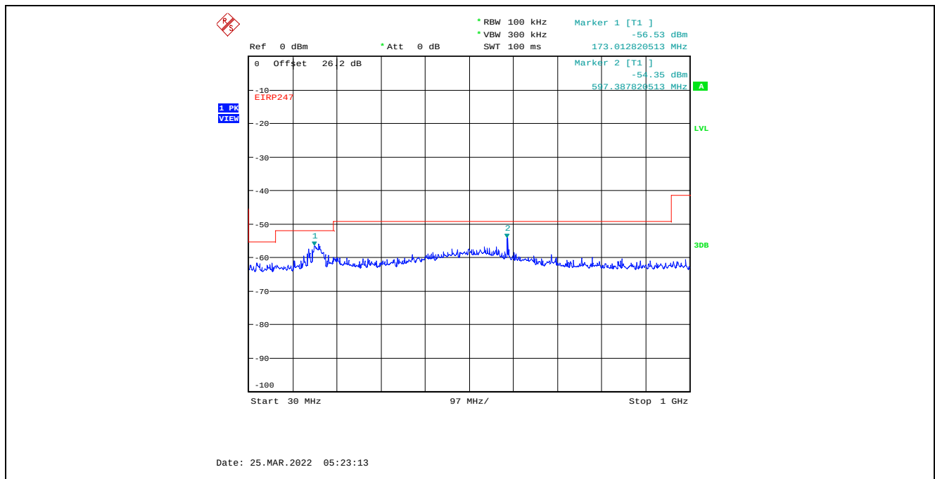
Plot C.4.25. Conducted Spurious Emissions in Restricted Frequency Bands, Chain 1 4 MHz Channel Bandwidth, Data Rate 7, Raw Power Setting 0, 2477 MHz, 30 MHz - 1 GHz, Peak Detector
