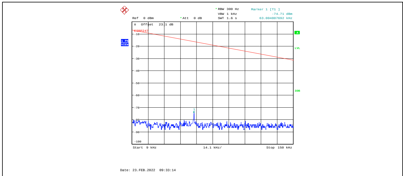
Plot C.1.2. Conducted Spurious Emissions in Restricted Frequency Bands, Chain 2 4 MHz Channel Bandwidth, Data Rate 3, Raw Power Setting 16, 2402 MHz, 9 kHz - 150 kHz, Peak Detector
