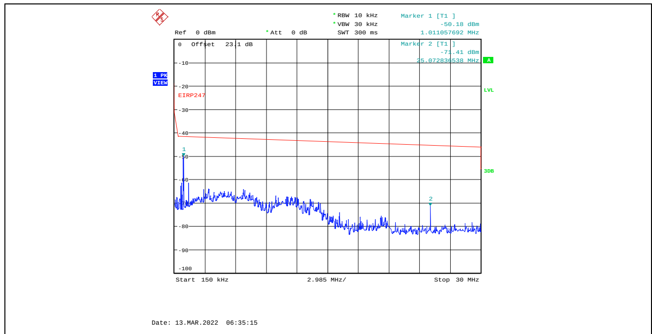
Plot C.2.83. Conducted Spurious Emissions in Restricted Frequency Bands, Chain 1 20 MHz Channel Bandwidth, Data Rate 7, Raw Power Setting 23, 2462 MHz, 150 kHz – 30 MHz, Peak Detector
