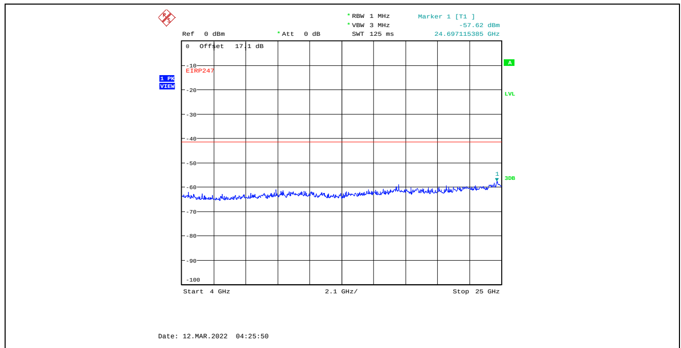
Plot C.2.99. Conducted Spurious Emissions in Restricted Frequency Bands, Chain 1 40 MHz Channel Bandwidth, Data Rate 7, Raw Power Setting 20, 2422 MHz, 4 GHz - 25 GHz, Peak Detector
