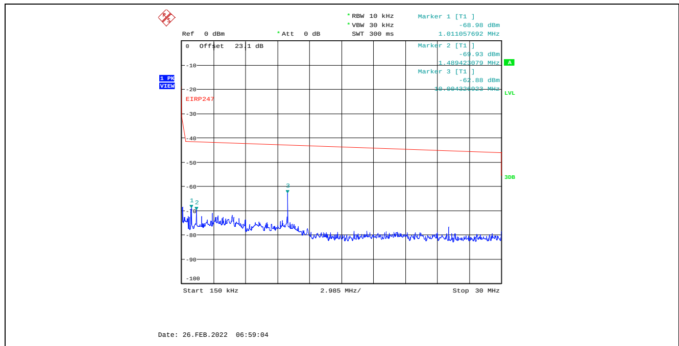
Plot C.2.3. Conducted Spurious Emissions in Restricted Frequency Bands, Chain 1 4 MHz Channel Bandwidth, Data Rate 7, Raw Power Setting 22, 2405 MHz, 150 kHz – 30 MHz, Peak Detector
