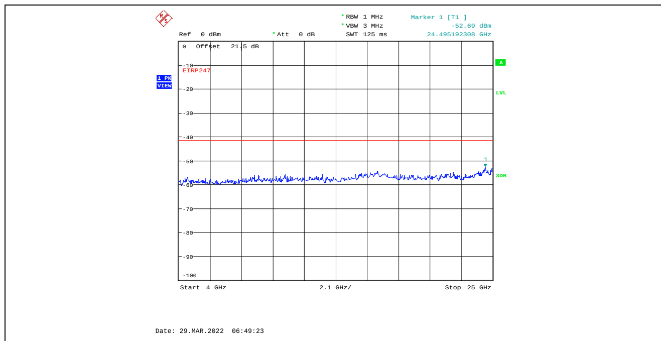
Plot C.4.69. Conducted Spurious Emissions in Restricted Frequency Bands, Chain 1 20 MHz Channel Bandwidth, Data Rate 7, Raw Power Setting 0, 2412 MHz, 4 GHz - 25 GHz, Peak Detector
