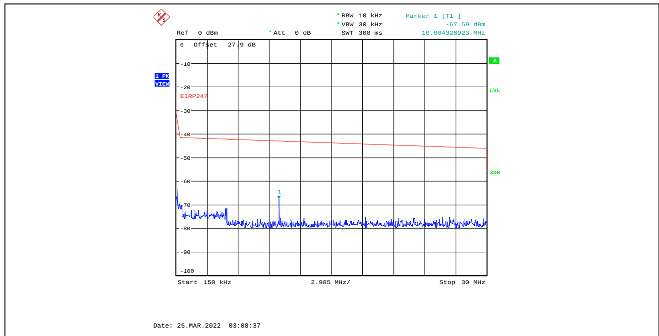
Plot C.3.24. Conducted Spurious Emissions in Restricted Frequency Bands, Chain 2 4 MHz Channel Bandwidth, Data Rate 3, Raw Power Setting 0, 2477 MHz, 150 kHz – 30 MHz, Peak Detector
