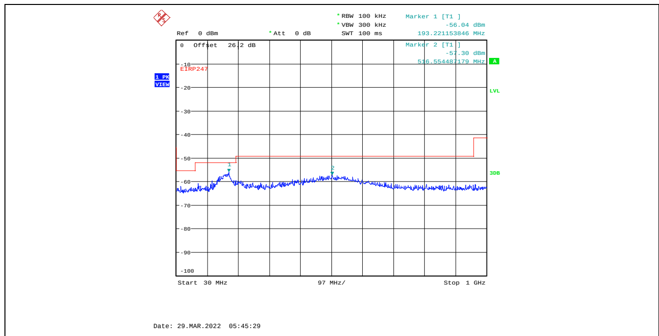
Plot C.4.66. Conducted Spurious Emissions in Restricted Frequency Bands, Chain 2 20 MHz Channel Bandwidth, Data Rate 7, Raw Power Setting 0, 2412 MHz, 30 MHz - 1 GHz, Peak Detector
