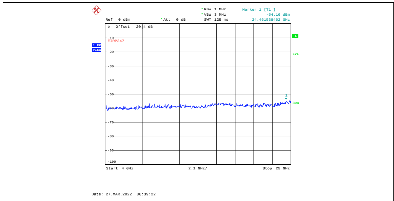
Plot C.3.59. Conducted Spurious Emissions in Restricted Frequency Bands, Chain 1 8 MHz Channel Bandwidth, Data Rate 3, Raw Power Setting 0, 2476 MHz, 4 GHz - 25 GHz, Peak Detector
