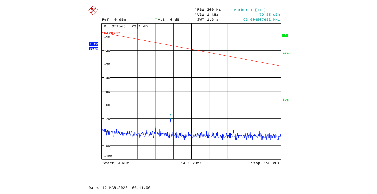
Plot C.1.61. Conducted Spurious Emissions in Restricted Frequency Bands, Chain 1 20 MHz Channel Bandwidth, Data Rate 3, Raw Power Setting 26, 2412 MHz, 9 kHz - 150 kHz, Peak Detector
