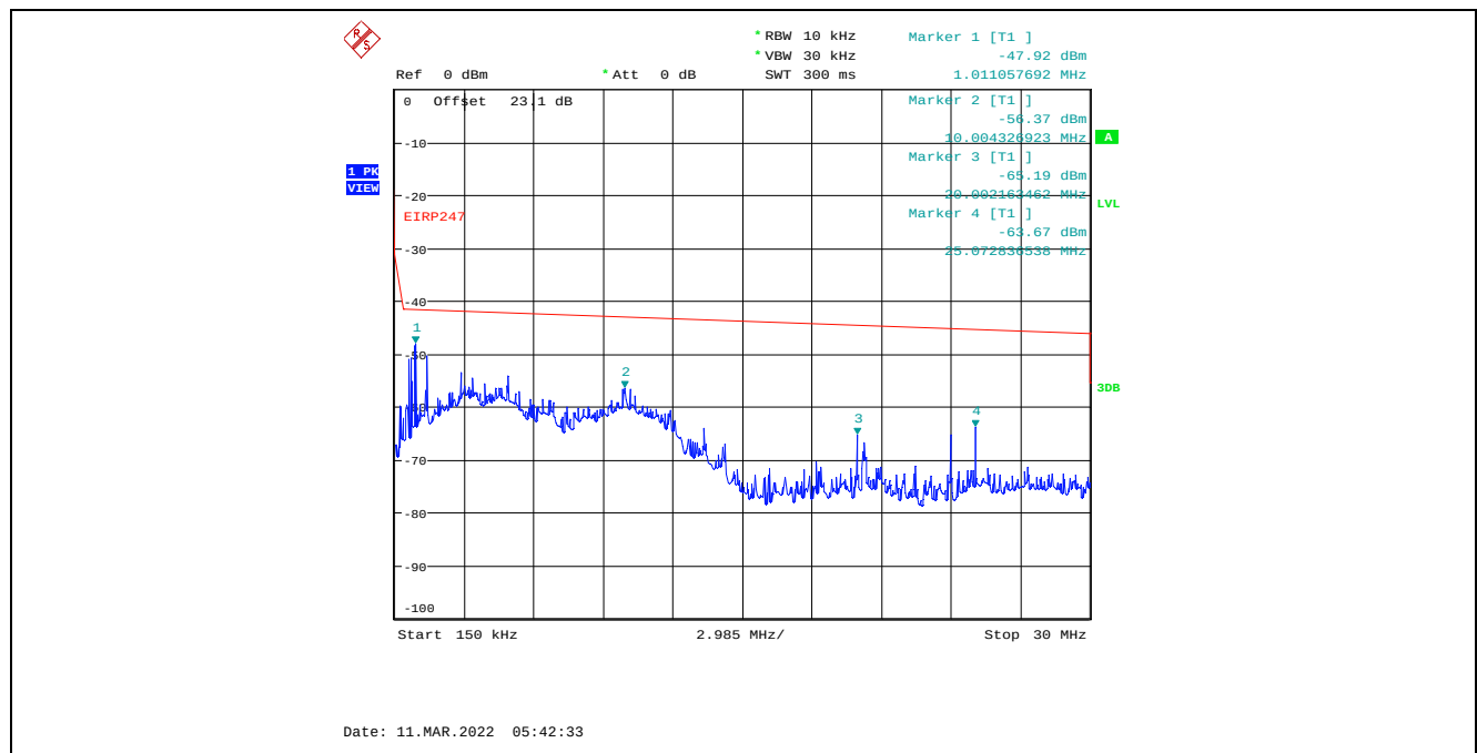
Plot C.1.114. Conducted Spurious Emissions in Restricted Frequency Bands, Chain 2 40 MHz Channel Bandwidth, Data Rate 3, Raw Power Setting 15, 2452 MHz, 150 kHz – 30 MHz, Peak Detector
