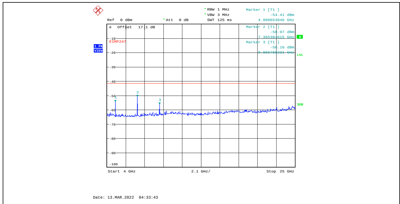
Plot C.1.89. Conducted Spurious Emissions in Restricted Frequency Bands, Chain 1 20 MHz Channel Bandwidth, Data Rate 3, Raw Power Setting 26, 2462 MHz, 4 GHz - 25 GHz, Peak Detector
