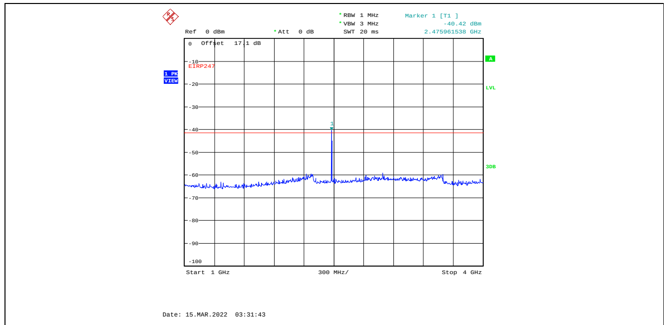
Plot C.1.27. Conducted Spurious Emissions in Restricted Frequency Bands, Chain 1 4 MHz Channel Bandwidth, Data Rate 3, Raw Power Setting 13, 2477 MHz, 1 GHz – 4 GHz, Peak Detector Marker 1 is Fundamental Signal
