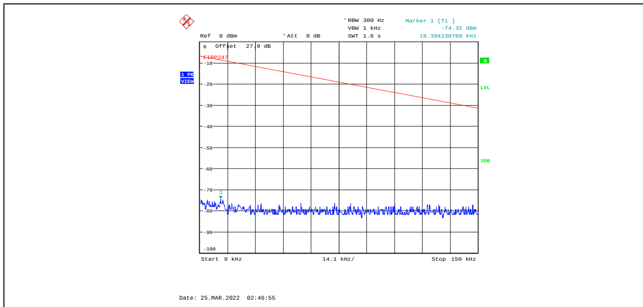
Plot C.3.1. Conducted Spurious Emissions in Restricted Frequency Bands, Chain 1 4 MHz Channel Bandwidth, Data Rate 3, Raw Power Setting 8, 2402 MHz, 9 kHz - 150 kHz, Peak Detector
