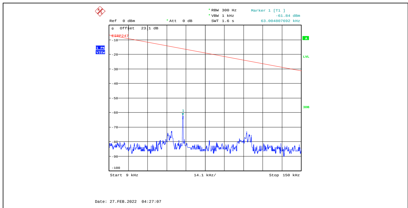
Plot C.2.32. Conducted Spurious Emissions in Restricted Frequency Bands, Chain 2 8 MHz Channel Bandwidth, Data Rate 7, Raw Power Setting 23, 2407 MHz, 9 kHz - 150 kHz, Peak Detector
