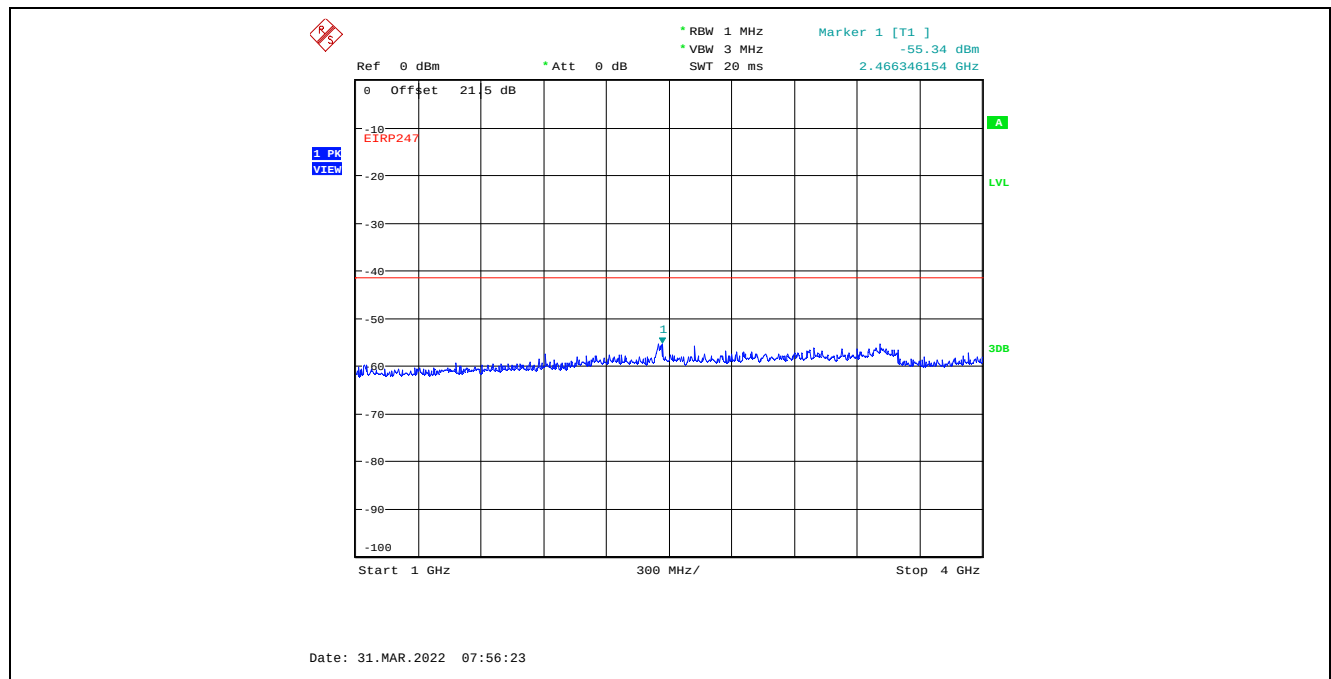
Plot C.3.118. Conducted Spurious Emissions in Restricted Frequency Bands, Chain 2 40 MHz Channel Bandwidth, Data Rate 3, Raw Power Setting 0, 2452 MHz, 1 GHz – 4 GHz, Peak Detector
