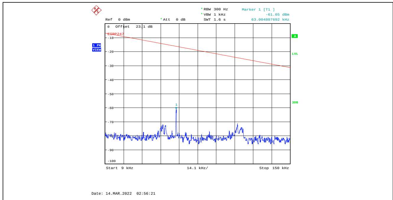
Plot C.1.51. Conducted Spurious Emissions in Restricted Frequency Bands, Chain 1 8 MHz Channel Bandwidth, Data Rate 3, Raw Power Setting 14, 2476 MHz, 9 kHz - 150 kHz, Peak Detector
