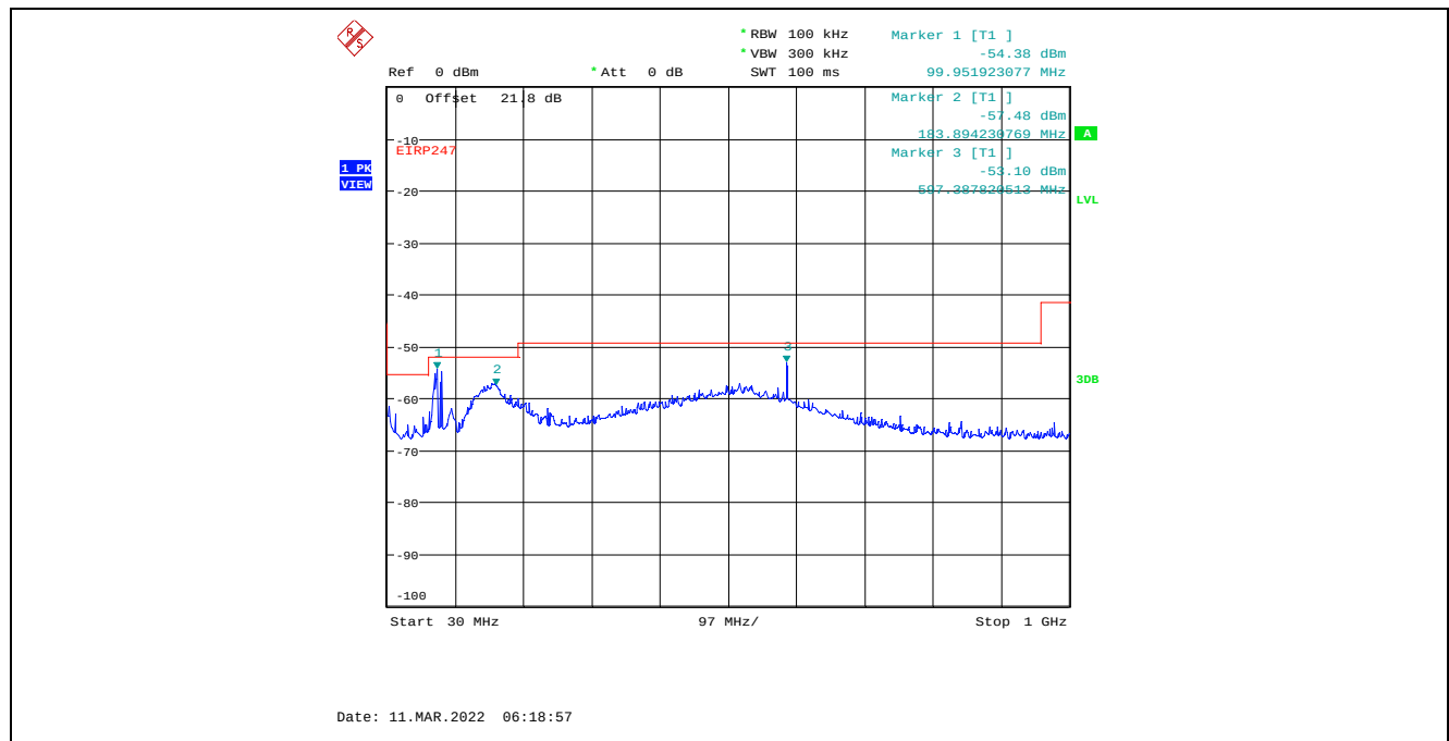
Plot C.1.105. Conducted Spurious Emissions in Restricted Frequency Bands, Chain 1 40 MHz Channel Bandwidth, Data Rate 3, Raw Power Setting 22, 2437 MHz, 30 MHz - 1 GHz, Peak Detector
