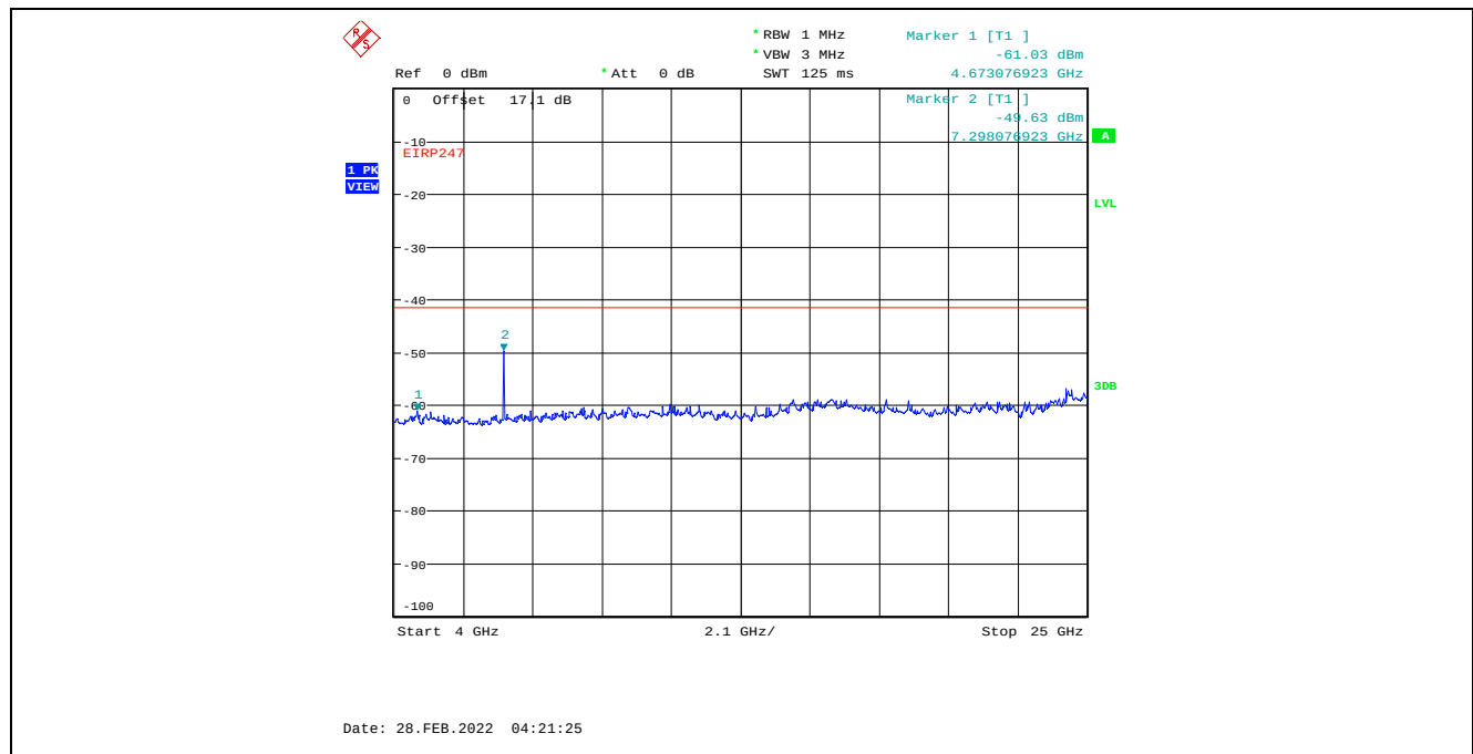
Plot C.2.49. Conducted Spurious Emissions in Restricted Frequency Bands, Chain 1 8 MHz Channel Bandwidth, Data Rate 7, Raw Power Setting 23, 2437 MHz, 4 GHz - 25 GHz, Peak Detector
