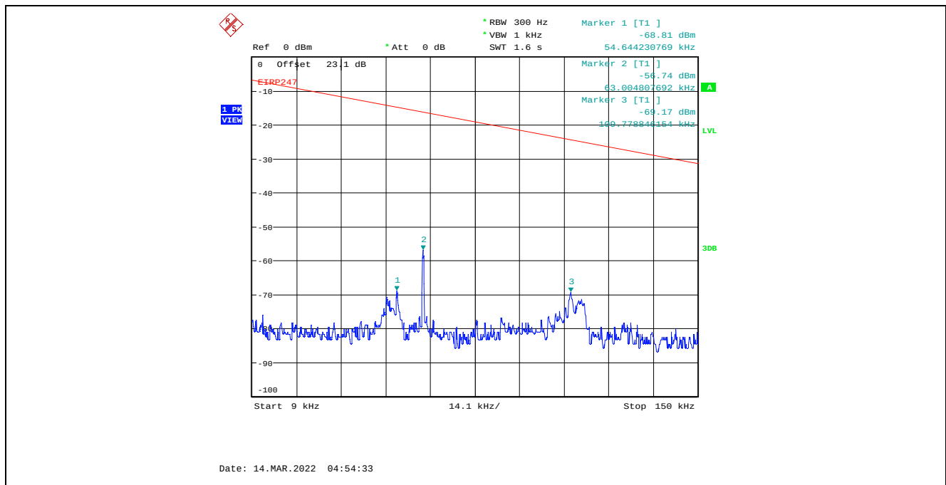
Plot C.2.51. Conducted Spurious Emissions in Restricted Frequency Bands, Chain 1 8 MHz Channel Bandwidth, Data Rate 7, Raw Power Setting 12, 2476 MHz, 9 kHz - 150 kHz, Peak Detector
