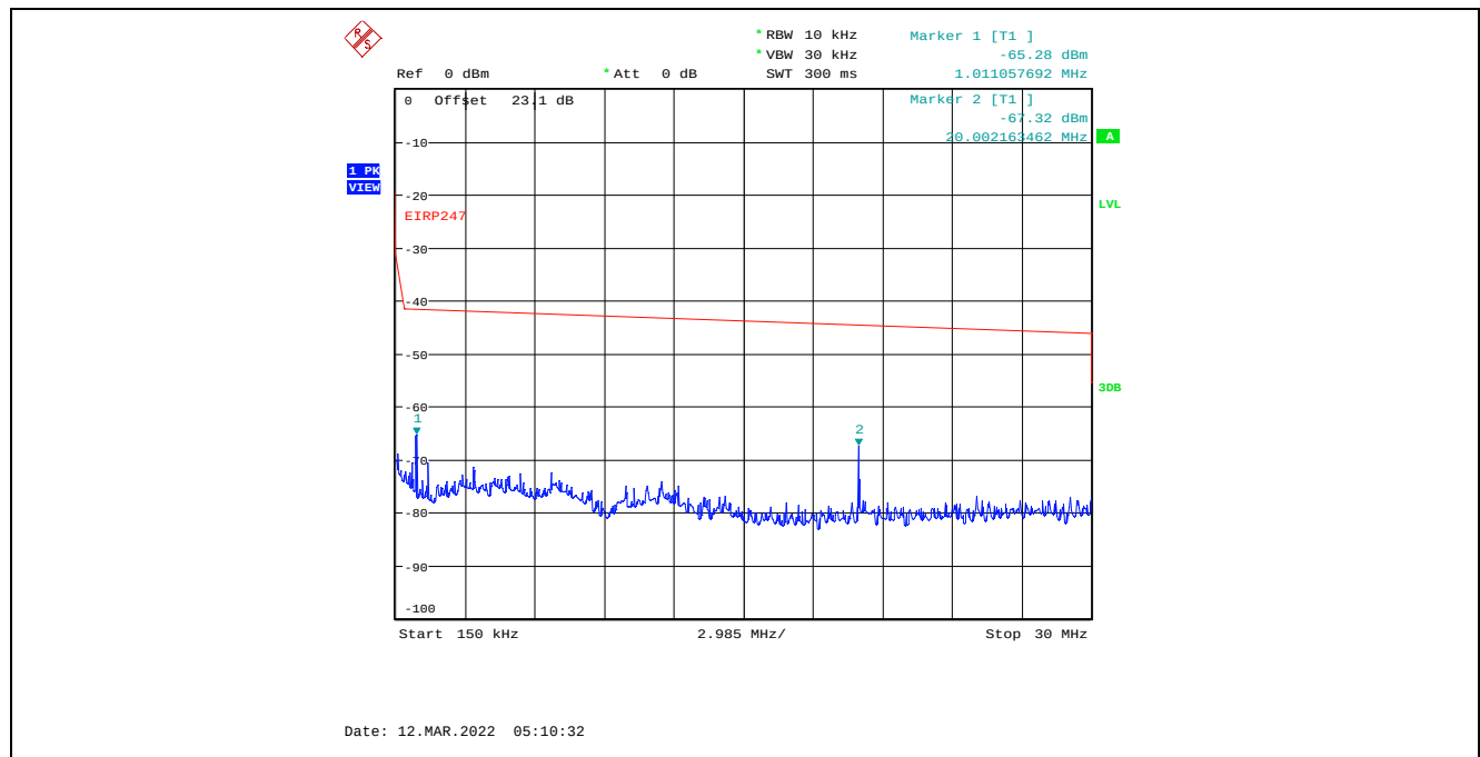
Plot C.2.103. Conducted Spurious Emissions in Restricted Frequency Bands, Chain 1 40 MHz Channel Bandwidth, Data Rate 7, Raw Power Setting 24, 2437 MHz, 150 kHz – 30 MHz, Peak Detector
