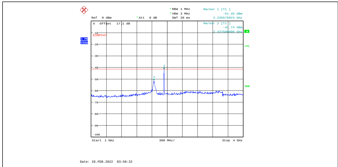
Plot C.1.47. Conducted Spurious Emissions in Restricted Frequency Bands, Chain 1 8 MHz Channel Bandwidth, Data Rate 3, Raw Power Setting 21, 2437 MHz, 1 GHz – 4 GHz, Peak Detector Marker 2 is Fundamental Signal
