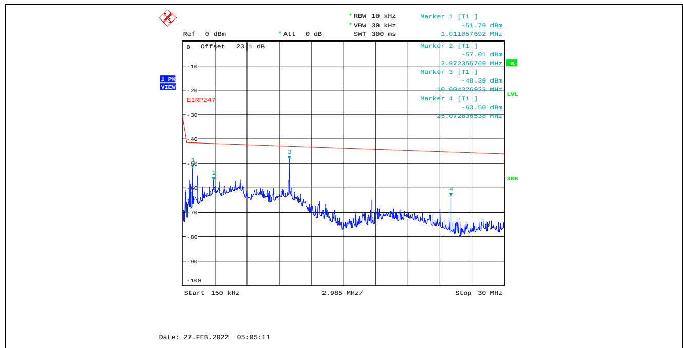
Plot C.2.44. Conducted Spurious Emissions in Restricted Frequency Bands, Chain 2 8 MHz Channel Bandwidth, Data Rate 7, Raw Power Setting 23, 2437 MHz, 150 kHz – 30 MHz, Peak Detector
