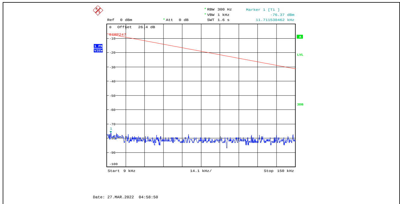
Plot C.3.41. Conducted Spurious Emissions in Restricted Frequency Bands, Chain 1 8 MHz Channel Bandwidth, Data Rate 3, Raw Power Setting 6, 2437 MHz, 9 kHz - 150 kHz, Peak Detector
