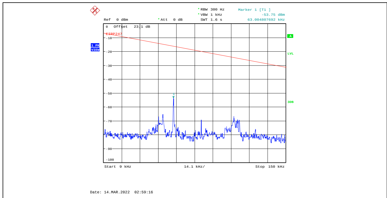
Plot C.1.52. Conducted Spurious Emissions in Restricted Frequency Bands, Chain 2 8 MHz Channel Bandwidth, Data Rate 3, Raw Power Setting 14, 2476 MHz, 9 kHz - 150 kHz, Peak Detector
