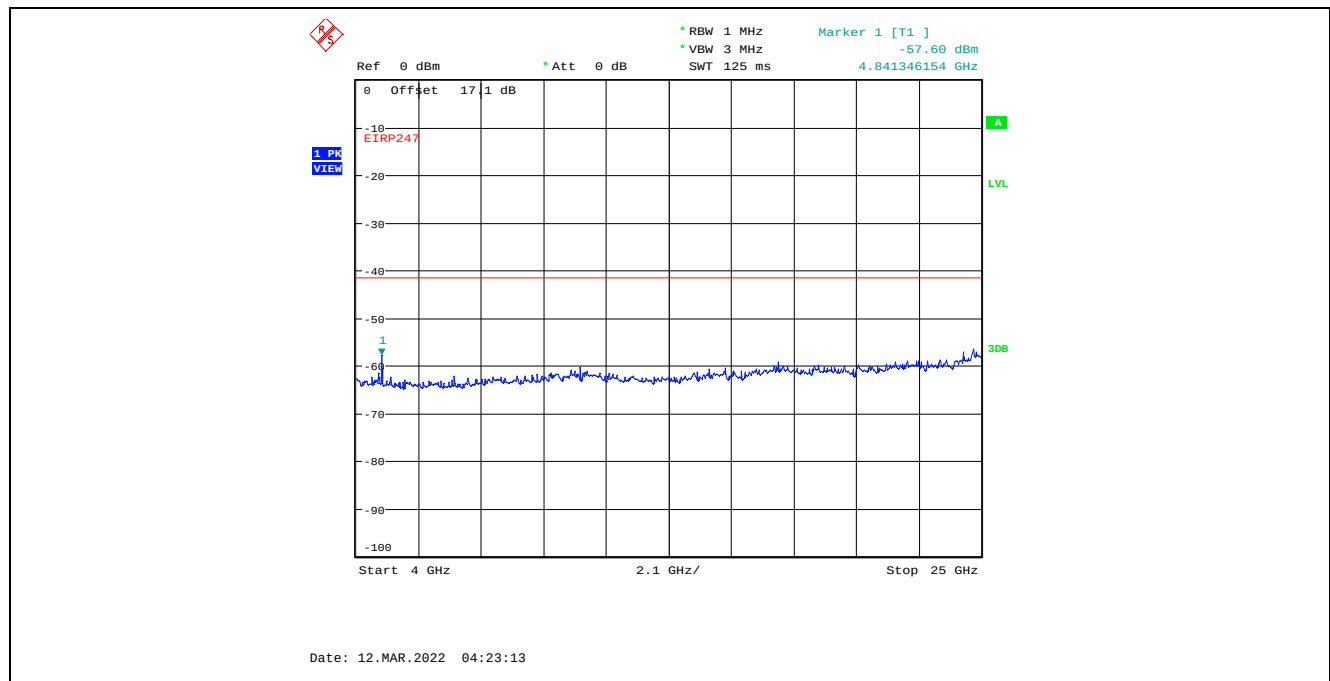
Plot C.2.109. Conducted Spurious Emissions in Restricted Frequency Bands, Chain 1 40 MHz Channel Bandwidth, Data Rate 7, Raw Power Setting 24, 2437 MHz, 4 GHz - 25 GHz, Peak Detector
