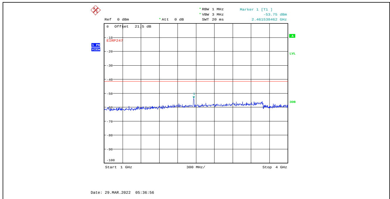
Plot C.4.87. Conducted Spurious Emissions in Restricted Frequency Bands, Chain 1 20 MHz Channel Bandwidth, Data Rate 7, Raw Power Setting 0, 2462 MHz, 1 GHz – 4 GHz, Peak Detector
