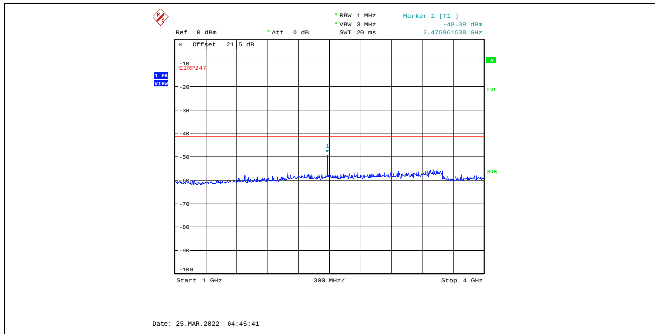
Plot C.4.28. Conducted Spurious Emissions in Restricted Frequency Bands, Chain 2 4 MHz Channel Bandwidth, Data Rate 7, Raw Power Setting 0, 2477 MHz, 1 GHz – 4 GHz, Peak Detector
