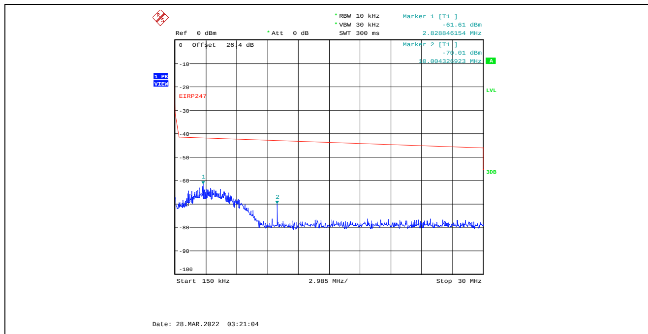
Plot C.4.54. Conducted Spurious Emissions in Restricted Frequency Bands, Chain 2 8 MHz Channel Bandwidth, Data Rate 7, Raw Power Setting 0, 2476 MHz, 150 kHz – 30 MHz, Peak Detector
