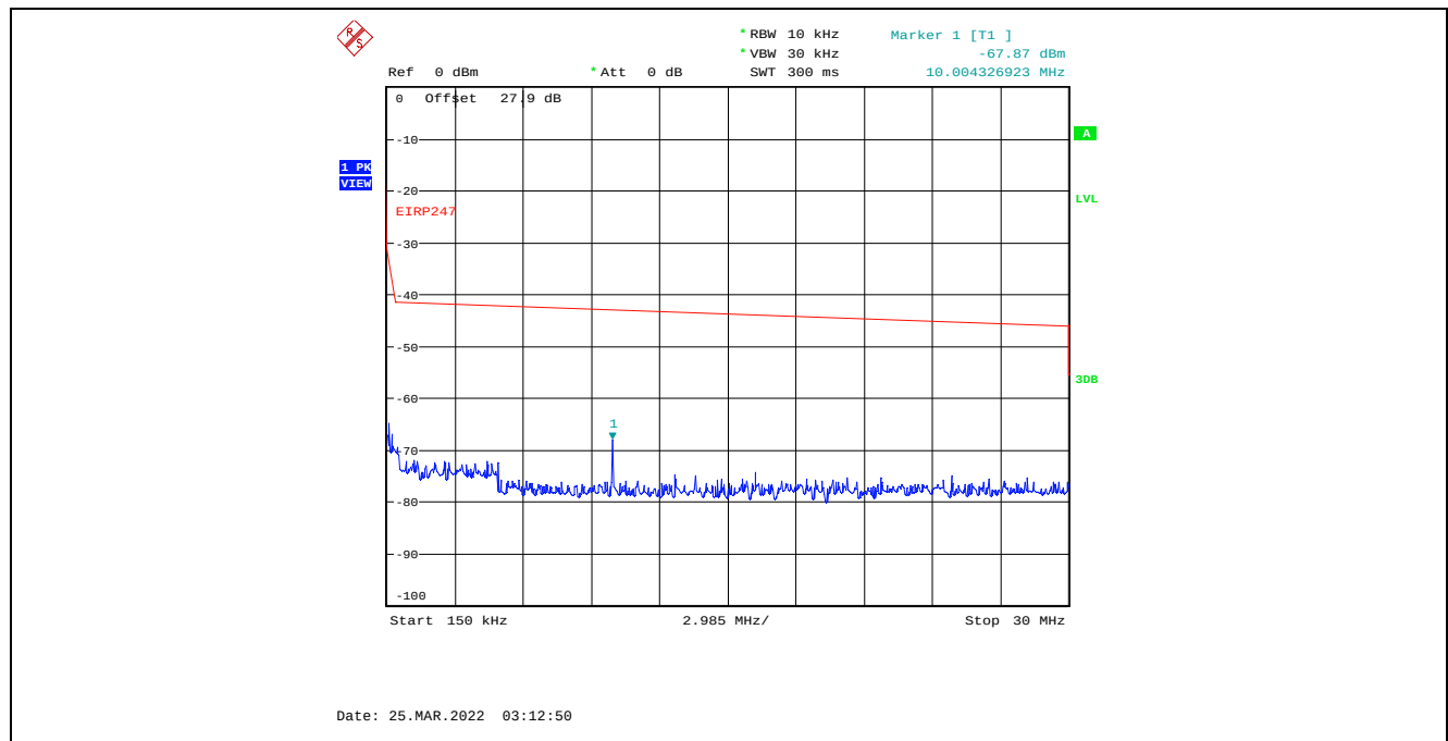
Plot C.3.13. Conducted Spurious Emissions in Restricted Frequency Bands, Chain 1 4 MHz Channel Bandwidth, Data Rate 3, Raw Power Setting 8, 2437 MHz, 150 kHz – 30 MHz, Peak Detector
