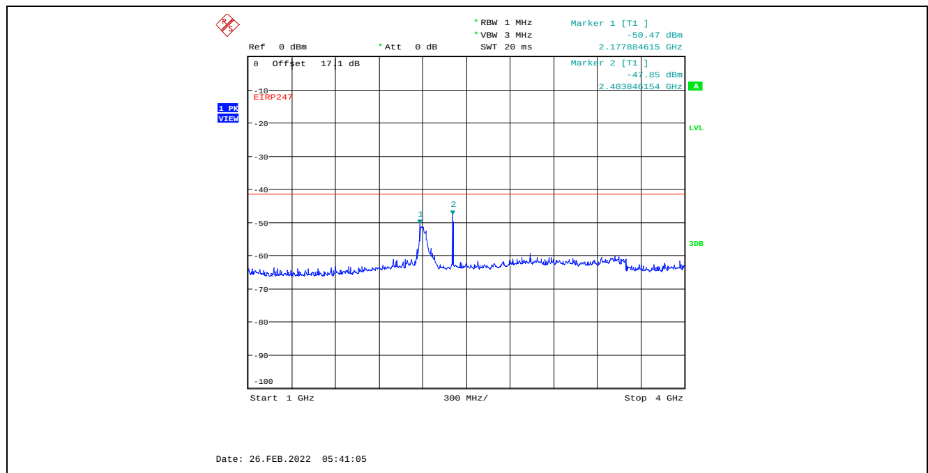
Plot C.2.8. Conducted Spurious Emissions in Restricted Frequency Bands, Chain 2 4 MHz Channel Bandwidth, Data Rate 7, Raw Power Setting 22, 2405 MHz, 1 GHz – 4 GHz, Peak Detector
