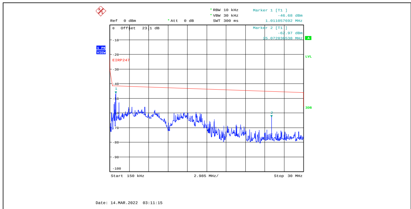
Plot C.1.54. Conducted Spurious Emissions in Restricted Frequency Bands, Chain 2 8 MHz Channel Bandwidth, Data Rate 3, Raw Power Setting 14, 2476 MHz, 150 kHz – 30 MHz, Peak Detector
