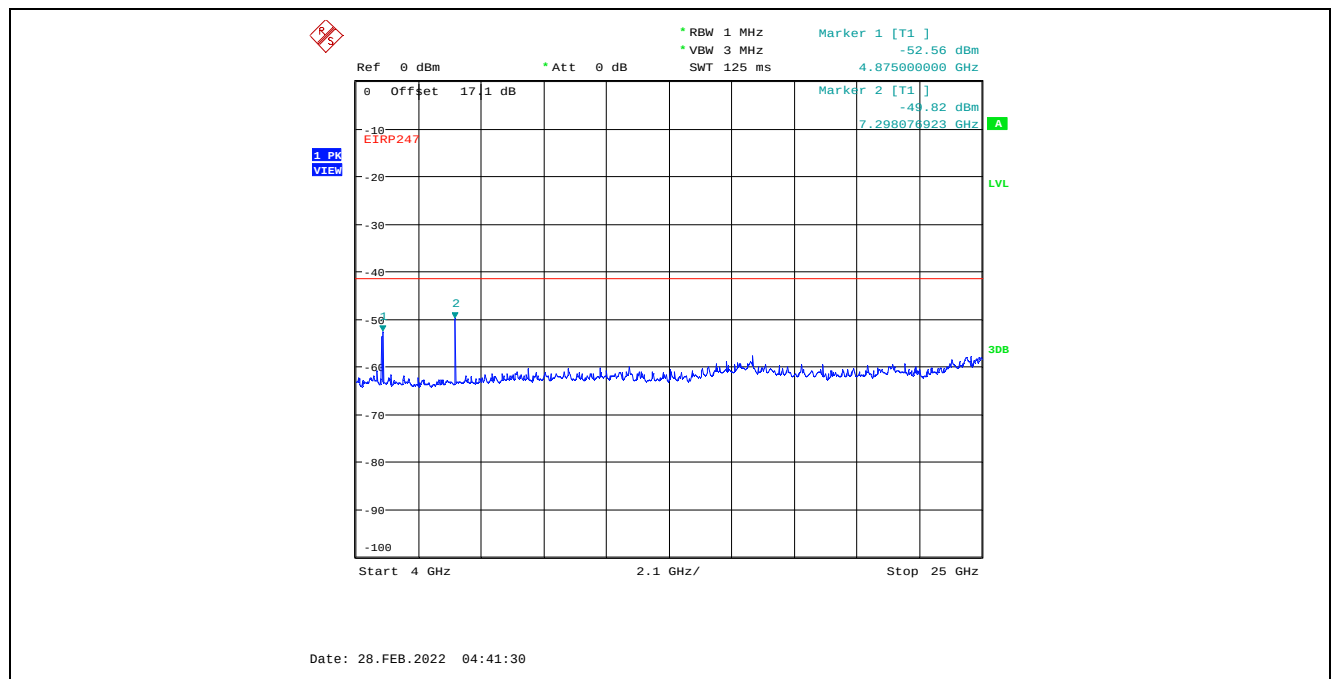
Plot C.1.50. Conducted Spurious Emissions in Restricted Frequency Bands, Chain 2 8 MHz Channel Bandwidth, Data Rate 3, Raw Power Setting 21, 2437 MHz, 4 GHz - 25 GHz, Peak Detector
