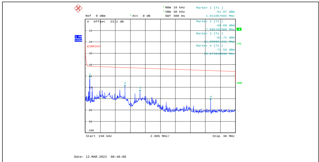
Plot C.1.63. Conducted Spurious Emissions in Restricted Frequency Bands, Chain 1 20 MHz Channel Bandwidth, Data Rate 3, Raw Power Setting 26, 2412 MHz, 150 kHz – 30 MHz, Peak Detector
