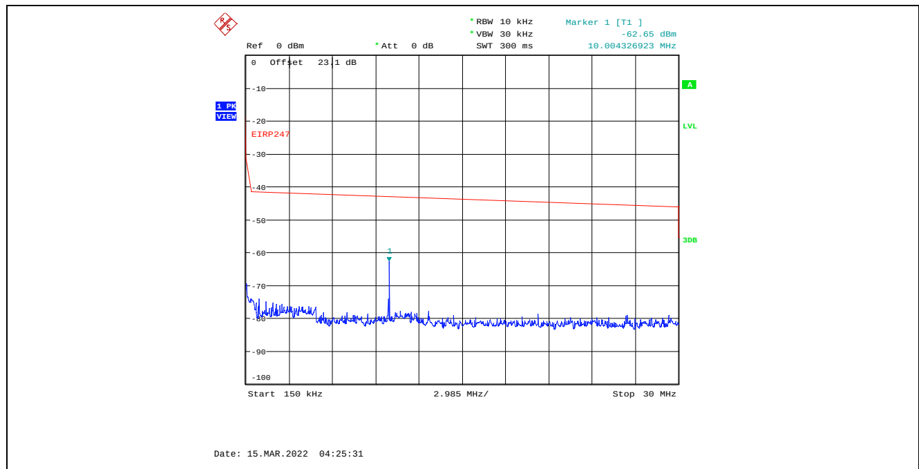
Plot C.1.23. Conducted Spurious Emissions in Restricted Frequency Bands, Chain 1 4 MHz Channel Bandwidth, Data Rate 3, Raw Power Setting 13, 2477 MHz, 150 kHz – 30 MHz, Peak Detector
