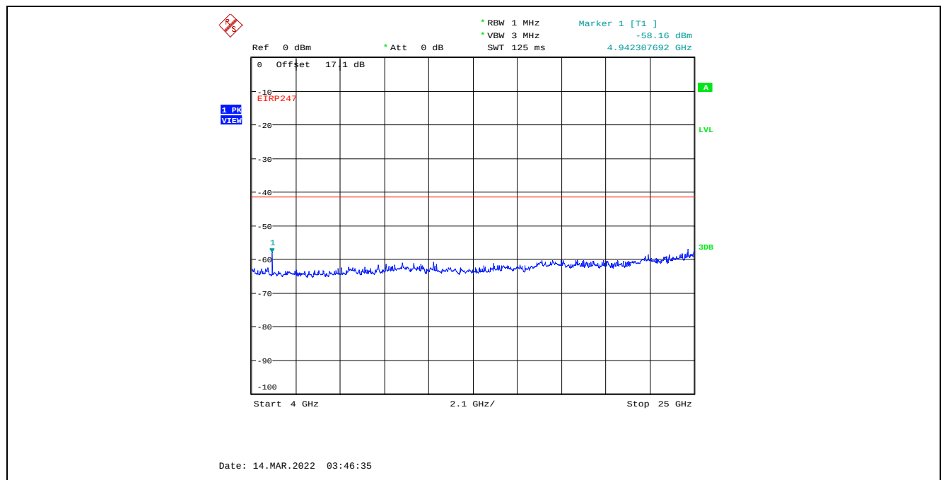
Plot C.1.60. Conducted Spurious Emissions in Restricted Frequency Bands, Chain 2 8 MHz Channel Bandwidth, Data Rate 3, Raw Power Setting 14, 2476 MHz, 4 GHz - 25 GHz, Peak Detector
