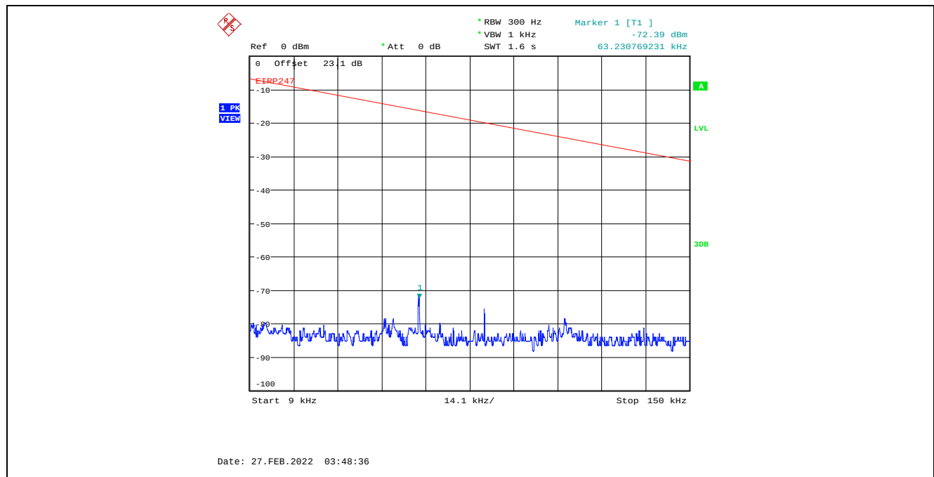
Plot C.1.41. Conducted Spurious Emissions in Restricted Frequency Bands, Chain 1 8 MHz Channel Bandwidth, Data Rate 3, Raw Power Setting 21, 2437 MHz, 9 kHz - 150 kHz, Peak Detector
