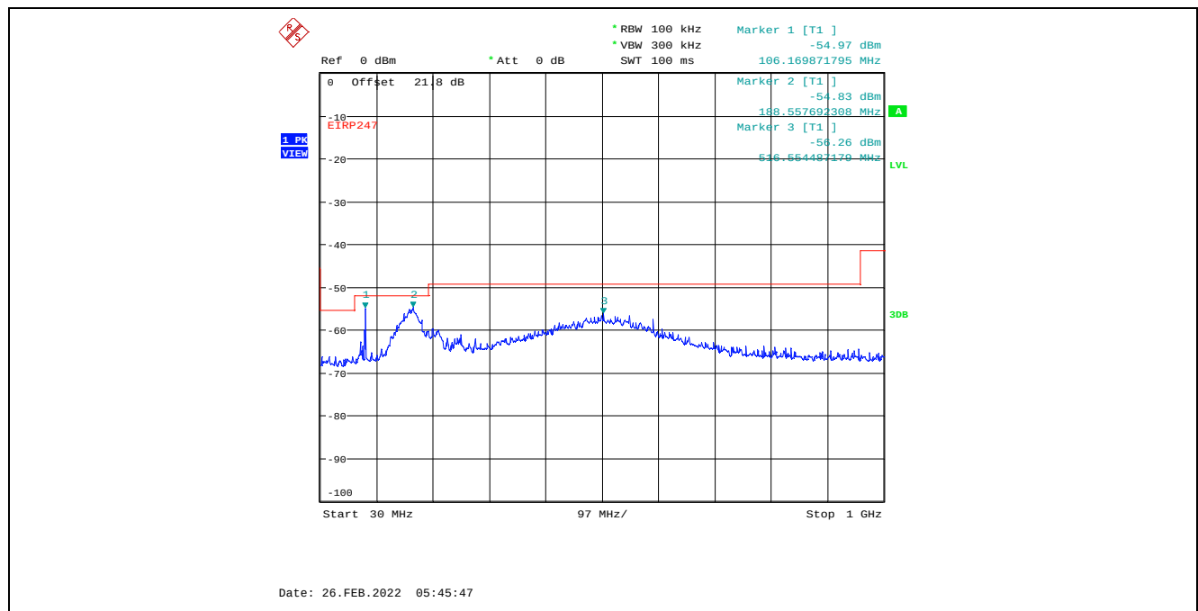
Plot C.2.6. Conducted Spurious Emissions in Restricted Frequency Bands, Chain 2 4 MHz Channel Bandwidth, Data Rate 7, Raw Power Setting 22, 2405 MHz, 30 MHz - 1 GHz, Peak Detector
