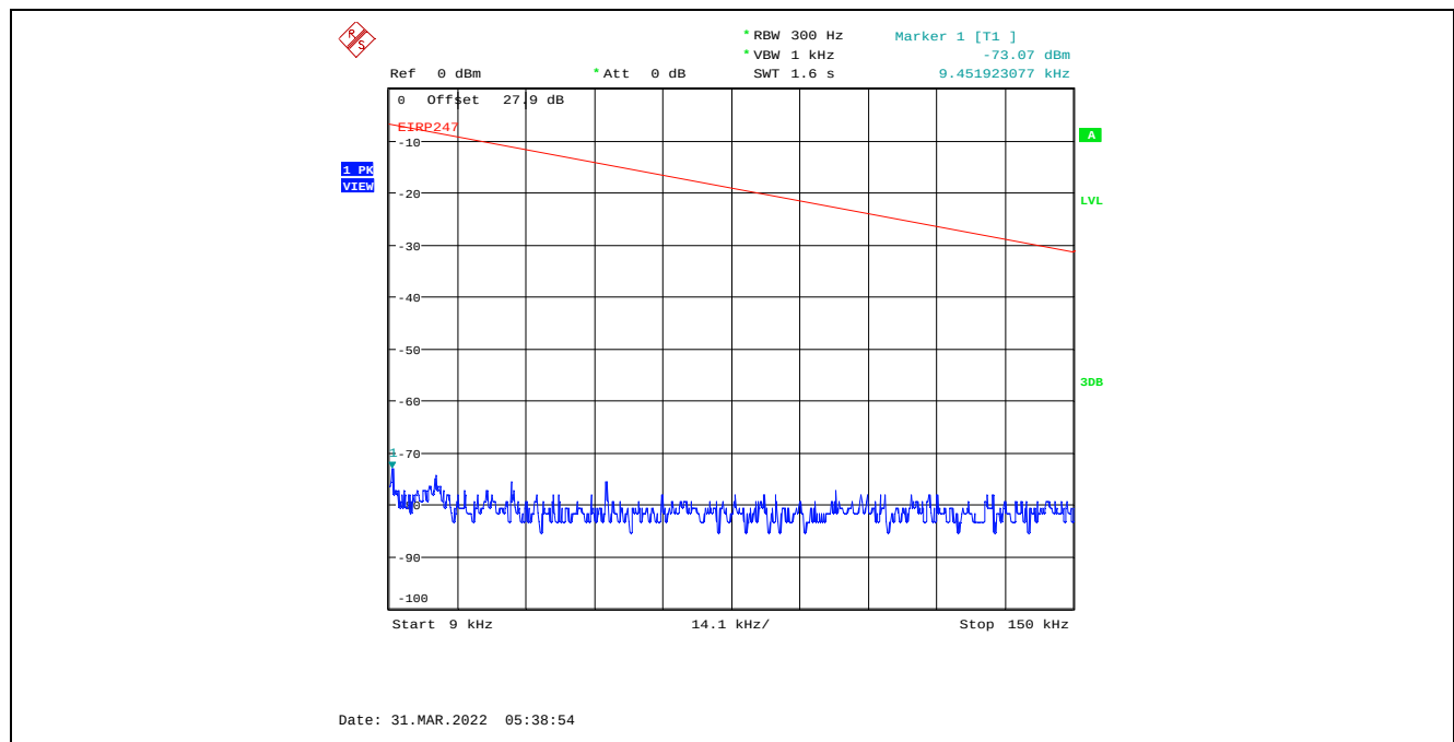
Plot C.4.102. Conducted Spurious Emissions in Restricted Frequency Bands, Chain 2 40 MHz Channel Bandwidth, Data Rate 7, Raw Power Setting 0, 2437 MHz, 9 kHz - 150 kHz, Peak Detector
