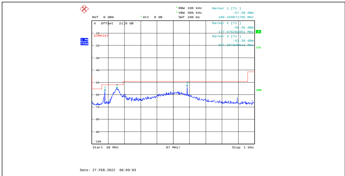
Plot C.2.35. Conducted Spurious Emissions in Restricted Frequency Bands, Chain 1 8 MHz Channel Bandwidth, Data Rate 7, Raw Power Setting 23, 2407 MHz, 30 MHz - 1 GHz, Peak Detector
