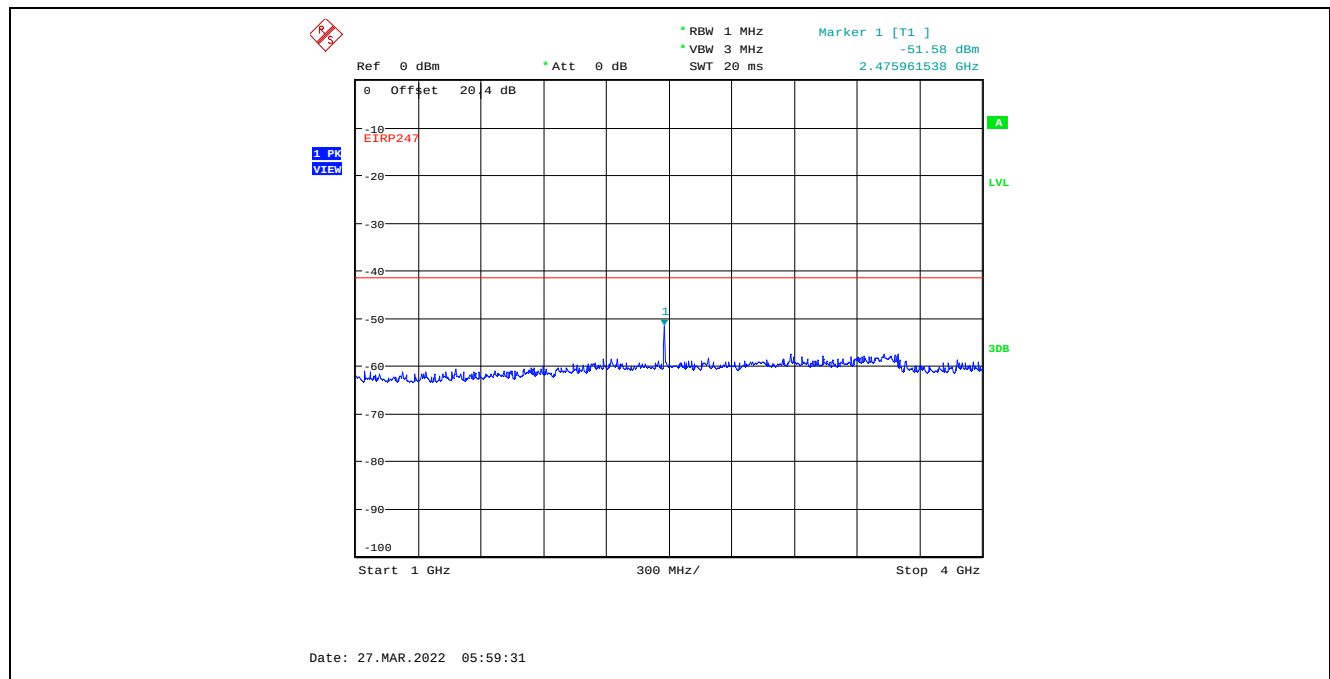
Plot C.3.58. Conducted Spurious Emissions in Restricted Frequency Bands, Chain 2 8 MHz Channel Bandwidth, Data Rate 3, Raw Power Setting 0, 2476 MHz, 1 GHz – 4 GHz, Peak Detector
