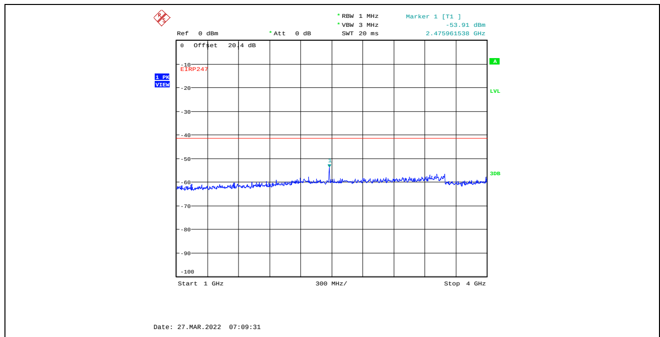
Plot C.4.58. Conducted Spurious Emissions in Restricted Frequency Bands, Chain 2 8 MHz Channel Bandwidth, Data Rate 7, Raw Power Setting 0, 2476 MHz, 1 GHz – 4 GHz, Peak Detector
