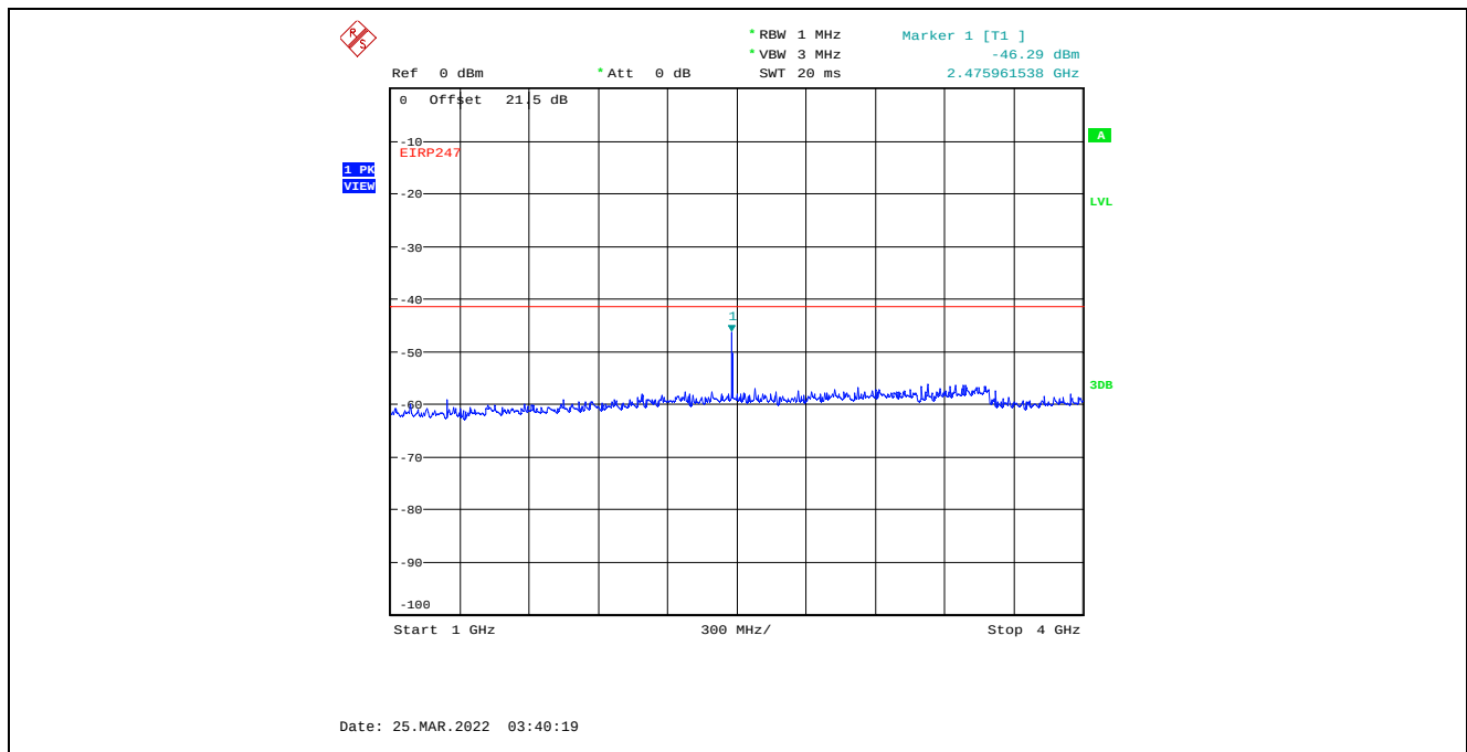
Plot C.3.27. Conducted Spurious Emissions in Restricted Frequency Bands, Chain 1 4 MHz Channel Bandwidth, Data Rate 3, Raw Power Setting 0, 2477 MHz, 1 GHz – 4 GHz, Peak Detector
