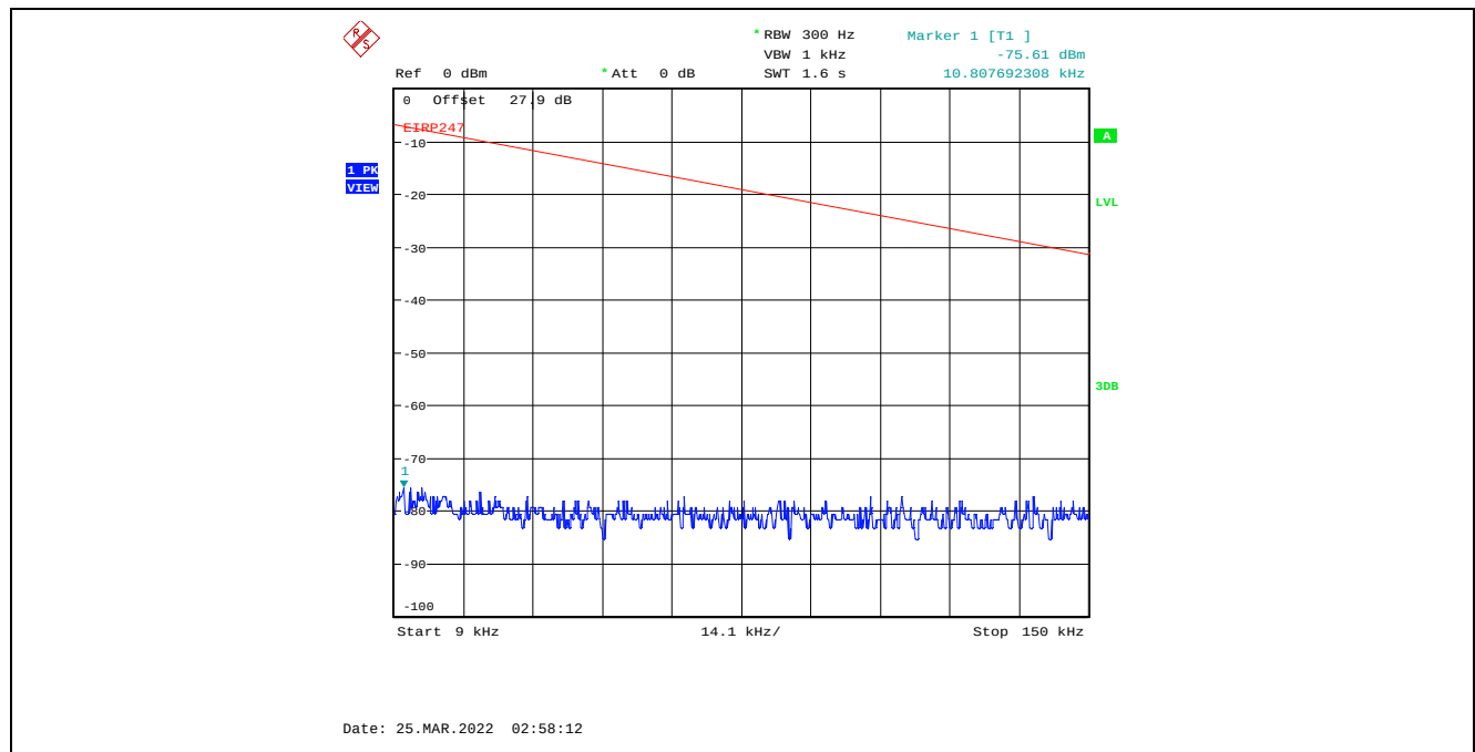
Plot C.3.12. Conducted Spurious Emissions in Restricted Frequency Bands, Chain 2 4 MHz Channel Bandwidth, Data Rate 3, Raw Power Setting 8, 2437 MHz, 9 kHz - 150 kHz, Peak Detector
