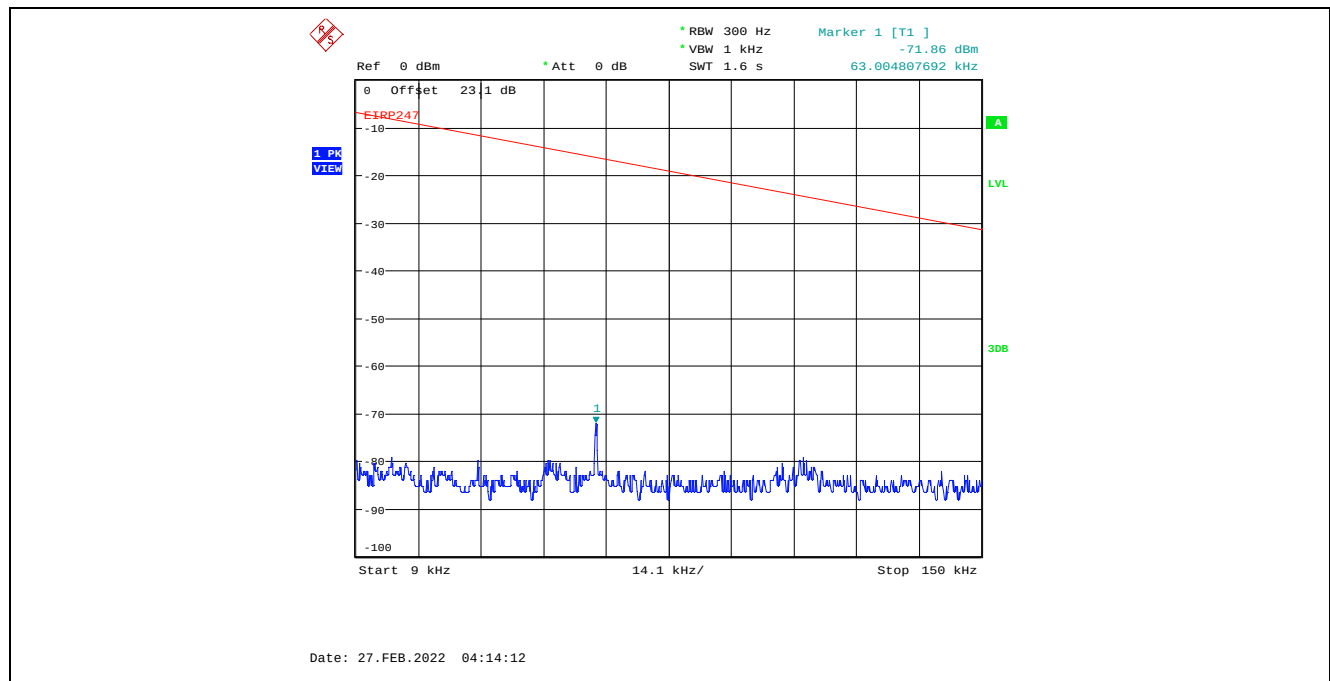
Plot C.2.31. Conducted Spurious Emissions in Restricted Frequency Bands, Chain 1 8 MHz Channel Bandwidth, Data Rate 7, Raw Power Setting 23, 2407 MHz, 9 kHz - 150 kHz, Peak Detector
