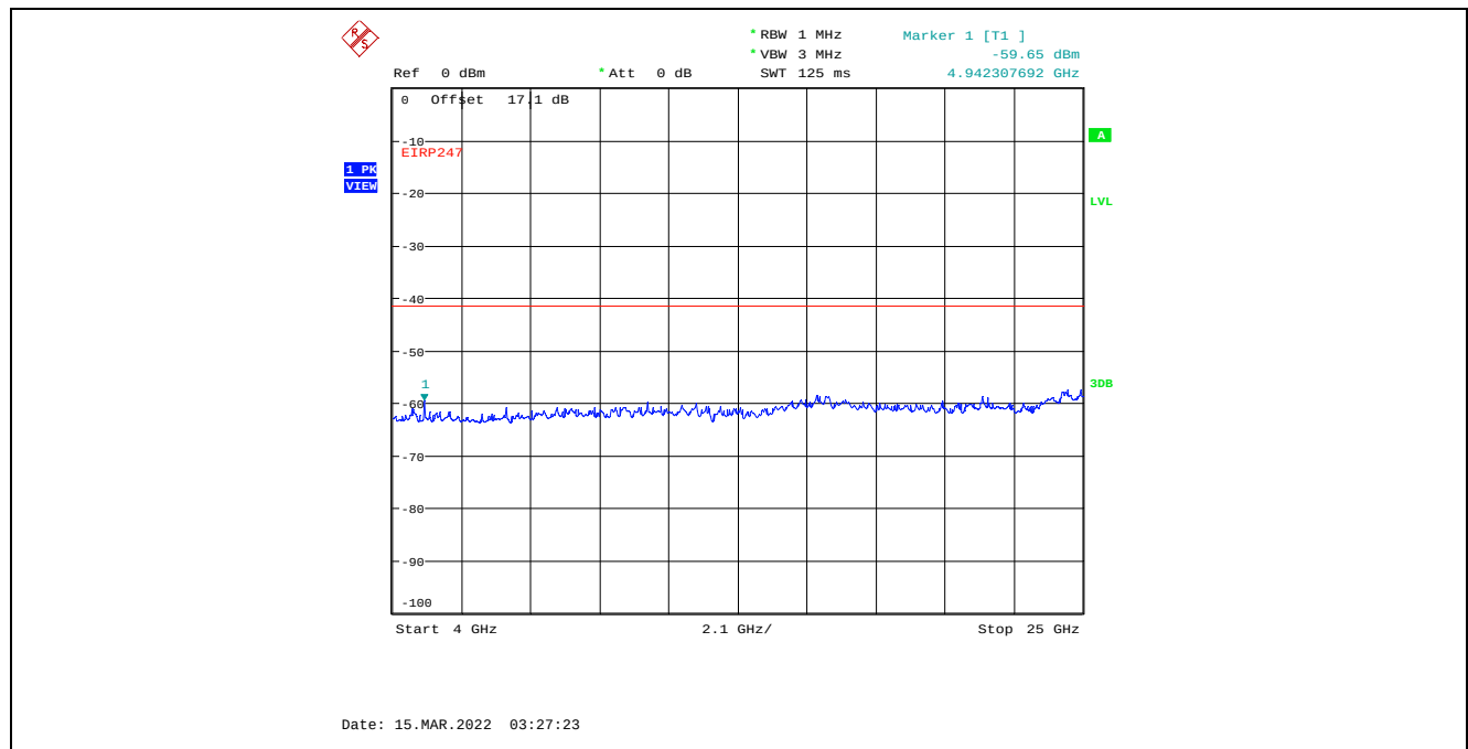
Plot C.2.29. Conducted Spurious Emissions in Restricted Frequency Bands, Chain 1 4 MHz Channel Bandwidth, Data Rate 7, Raw Power Setting 20, 2477 MHz, 4 GHz - 25 GHz, Peak Detector
