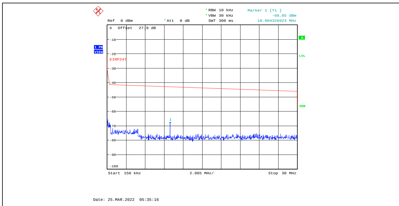
Plot C.4.24. Conducted Spurious Emissions in Restricted Frequency Bands, Chain 2 4 MHz Channel Bandwidth, Data Rate 7, Raw Power Setting 0, 2477 MHz, 150 kHz – 30 MHz, Peak Detector
