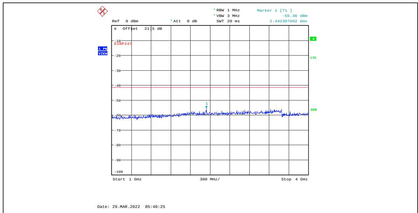
Plot C.4.78. Conducted Spurious Emissions in Restricted Frequency Bands, Chain 2 20 MHz Channel Bandwidth, Data Rate 7, Raw Power Setting 0, 2437 MHz, 1 GHz – 4 GHz, Peak Detector
