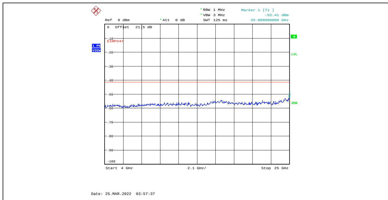
Plot C.3.20. Conducted Spurious Emissions in Restricted Frequency Bands, Chain 2 4 MHz Channel Bandwidth, Data Rate 3, Raw Power Setting 8, 2437 MHz, 4 GHz - 25 GHz, Peak Detector
