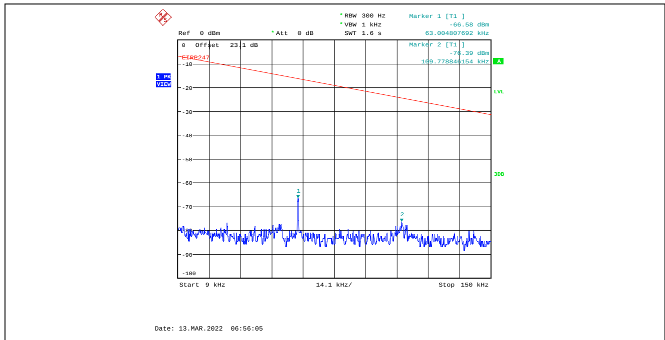
Plot C.2.61. Conducted Spurious Emissions in Restricted Frequency Bands, Chain 1 20 MHz Channel Bandwidth, Data Rate 7, Raw Power Setting 23, 2412 MHz, 9 kHz - 150 kHz, Peak Detector
