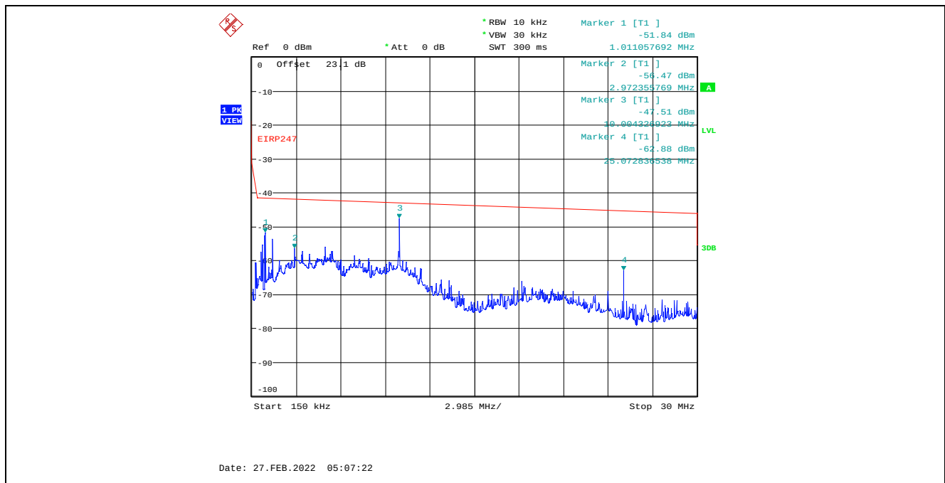
Plot C.2.34. Conducted Spurious Emissions in Restricted Frequency Bands, Chain 2 8 MHz Channel Bandwidth, Data Rate 7, Raw Power Setting 23, 2407 MHz, 150 kHz – 30 MHz, Peak Detector
