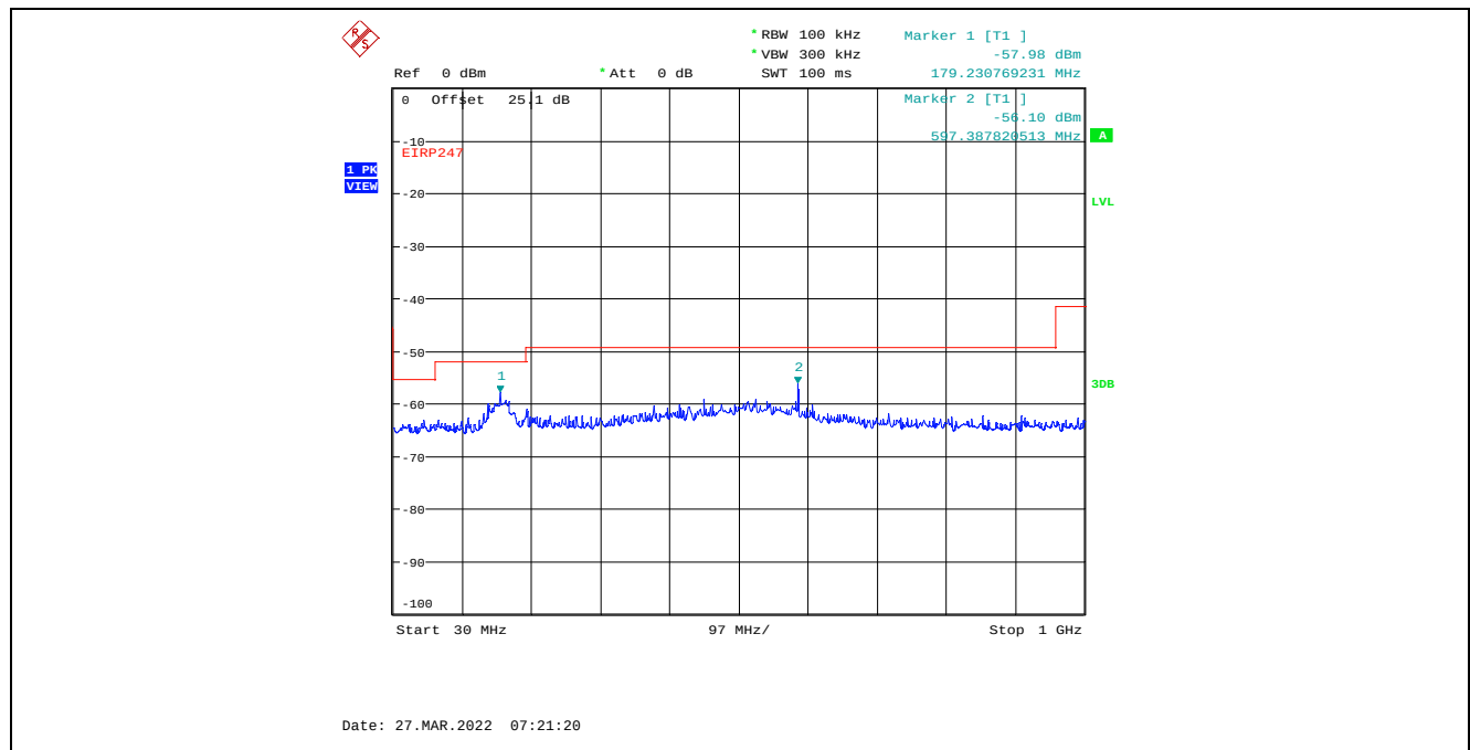
Plot C.4.55. Conducted Spurious Emissions in Restricted Frequency Bands, Chain 1 8 MHz Channel Bandwidth, Data Rate 7, Raw Power Setting 0, 2476 MHz, 30 MHz - 1 GHz, Peak Detector
