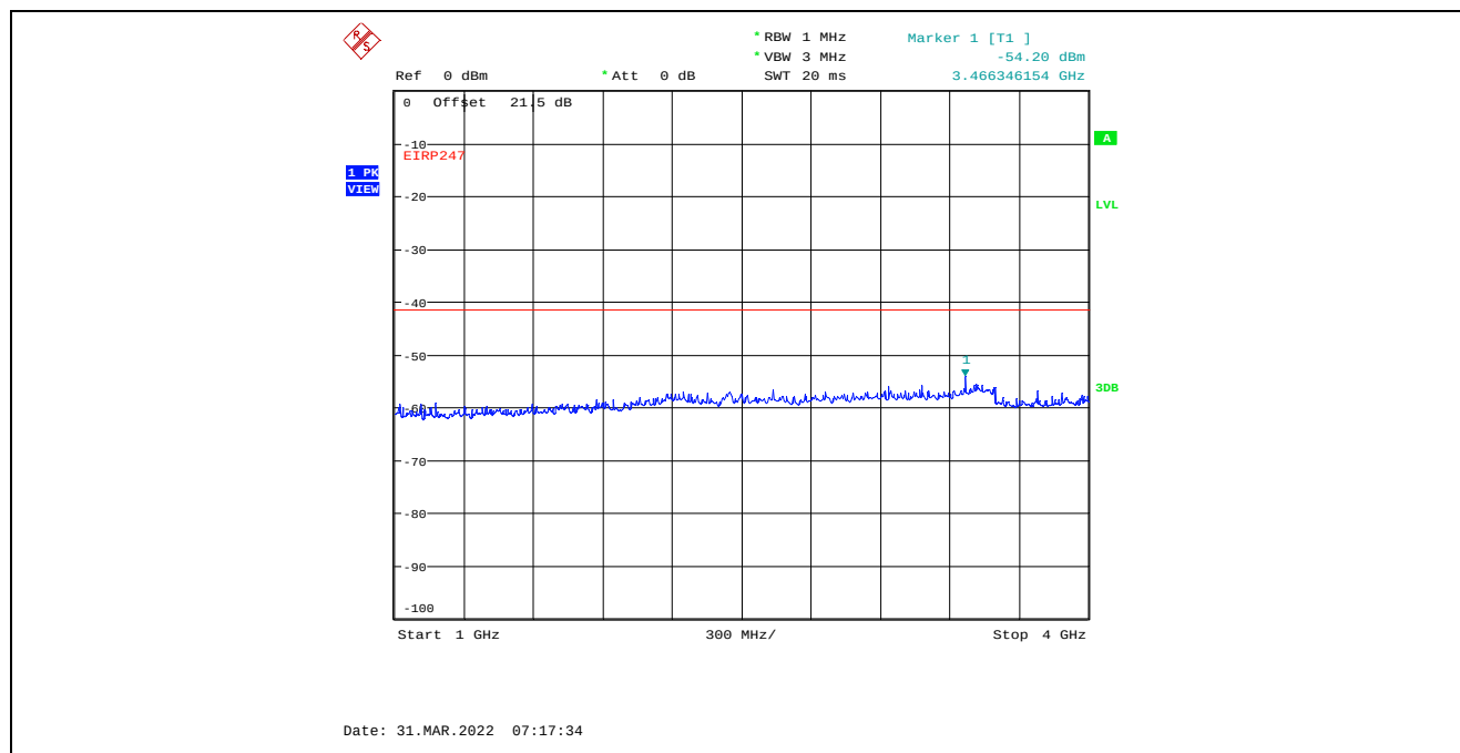
Plot C.4.107. Conducted Spurious Emissions in Restricted Frequency Bands, Chain 1 40 MHz Channel Bandwidth, Data Rate 7, Raw Power Setting 0, 2437 MHz, 1 GHz – 4 GHz, Peak Detector
