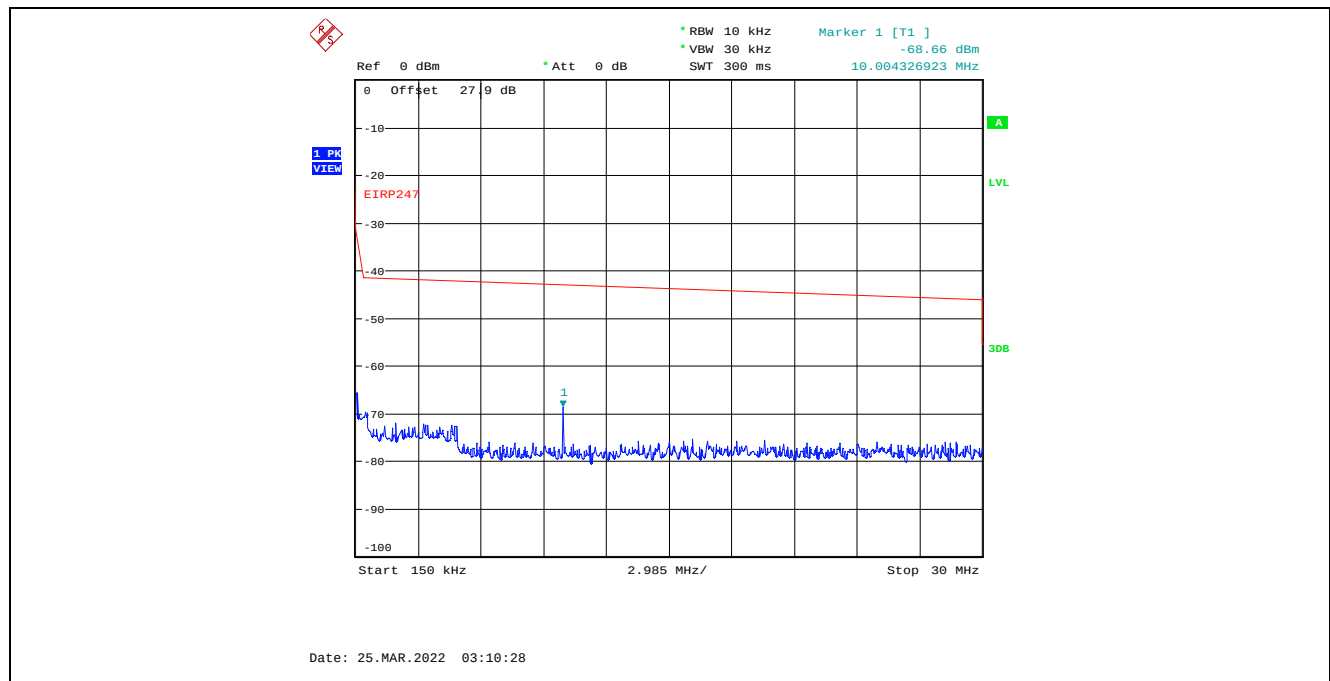
Plot C.3.23. Conducted Spurious Emissions in Restricted Frequency Bands, Chain 1 4 MHz Channel Bandwidth, Data Rate 3, Raw Power Setting 0, 2477 MHz, 150 kHz – 30 MHz, Peak Detector
