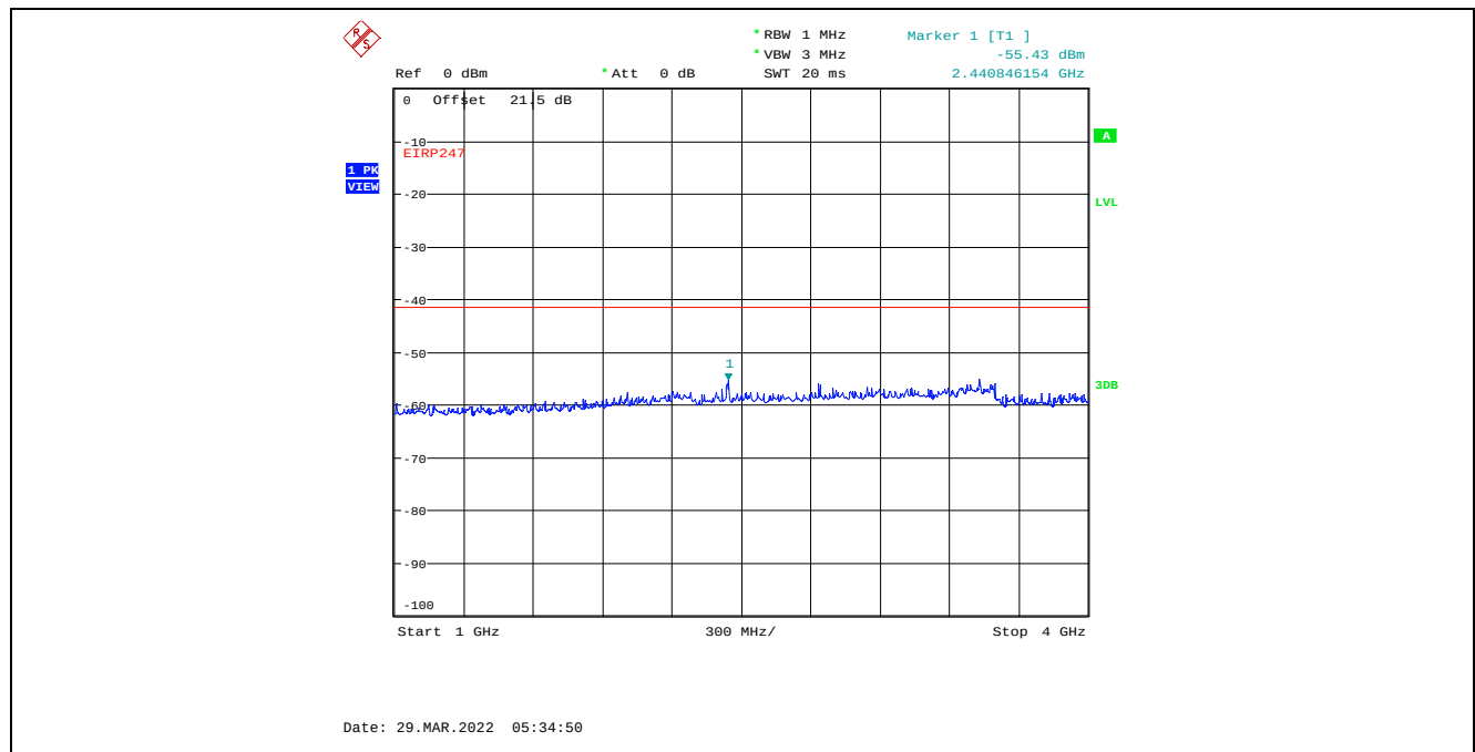
Plot C.4.77. Conducted Spurious Emissions in Restricted Frequency Bands, Chain 1 20 MHz Channel Bandwidth, Data Rate 7, Raw Power Setting 0, 2437 MHz, 1 GHz – 4 GHz, Peak Detector
