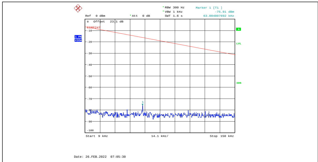
Plot C.2.11. Conducted Spurious Emissions in Restricted Frequency Bands, Chain 1 4 MHz Channel Bandwidth, Data Rate 7, Raw Power Setting 22, 2437 MHz, 9 kHz - 150 kHz, Peak Detector
