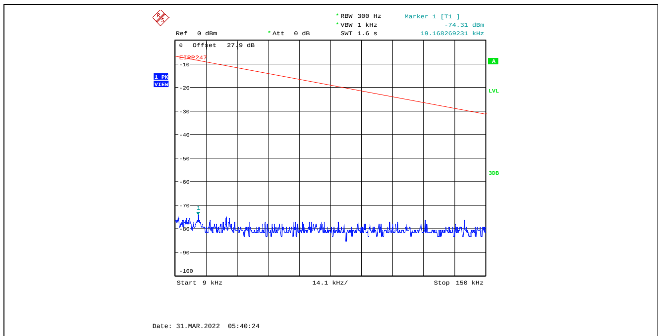
Plot C.4.112. Conducted Spurious Emissions in Restricted Frequency Bands, Chain 2 40 MHz Channel Bandwidth, Data Rate 7, Raw Power Setting 0, 2452 MHz, 9 kHz - 150 kHz, Peak Detector
