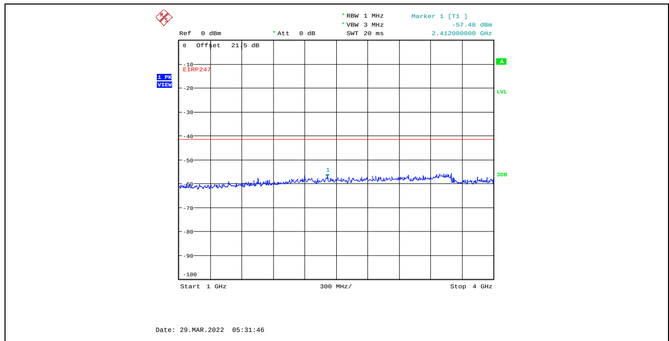
Plot C.4.67. Conducted Spurious Emissions in Restricted Frequency Bands, Chain 1 20 MHz Channel Bandwidth, Data Rate 7, Raw Power Setting 0, 2412 MHz, 1 GHz – 4 GHz, Peak Detector
