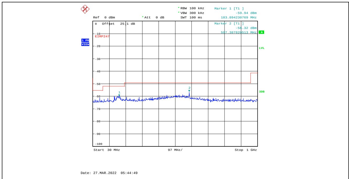
Plot C.3.45. Conducted Spurious Emissions in Restricted Frequency Bands, Chain 1 8 MHz Channel Bandwidth, Data Rate 3, Raw Power Setting 6, 2437 MHz, 30 MHz - 1 GHz, Peak Detector
