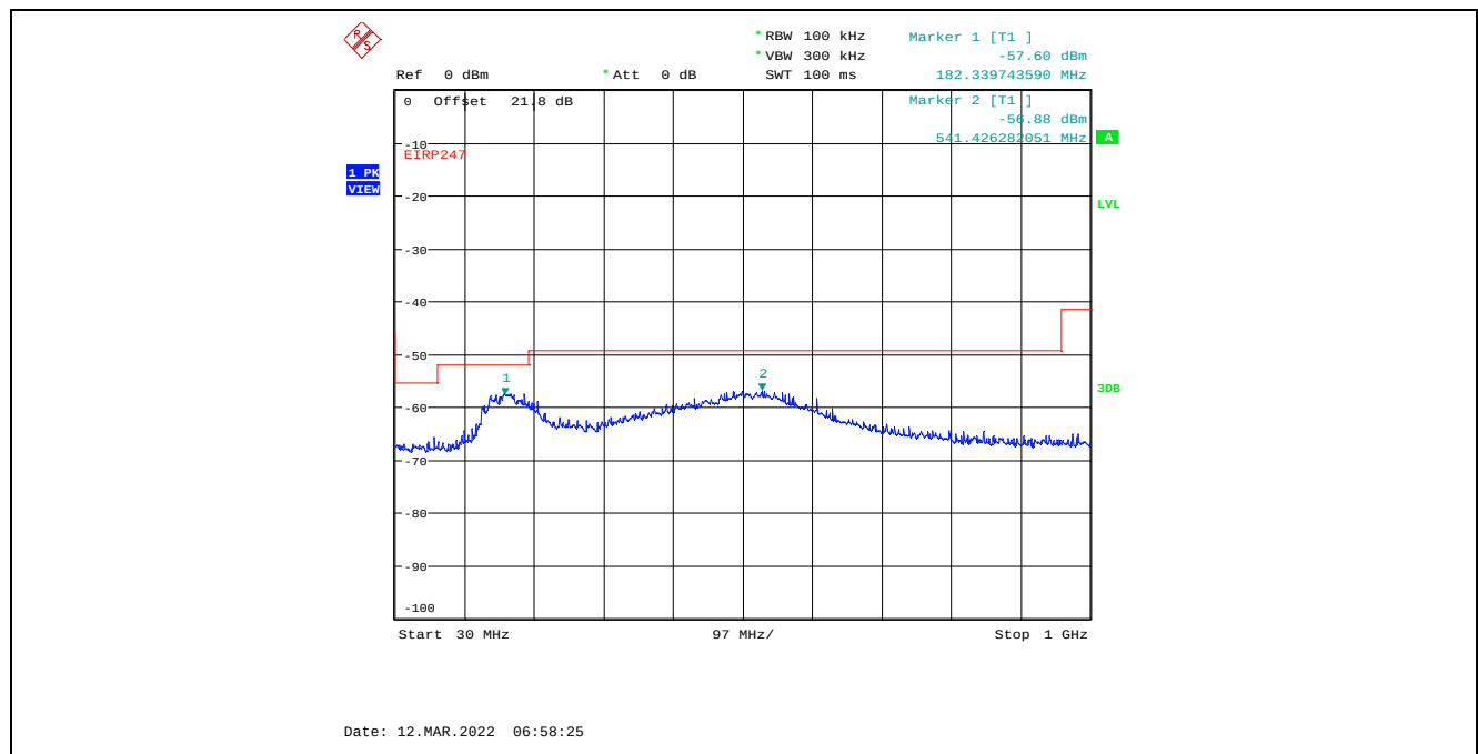
Plot C.1.86. Conducted Spurious Emissions in Restricted Frequency Bands, Chain 2 20 MHz Channel Bandwidth, Data Rate 3, Raw Power Setting 26, 2462 MHz, 30 MHz - 1 GHz, Peak Detector
