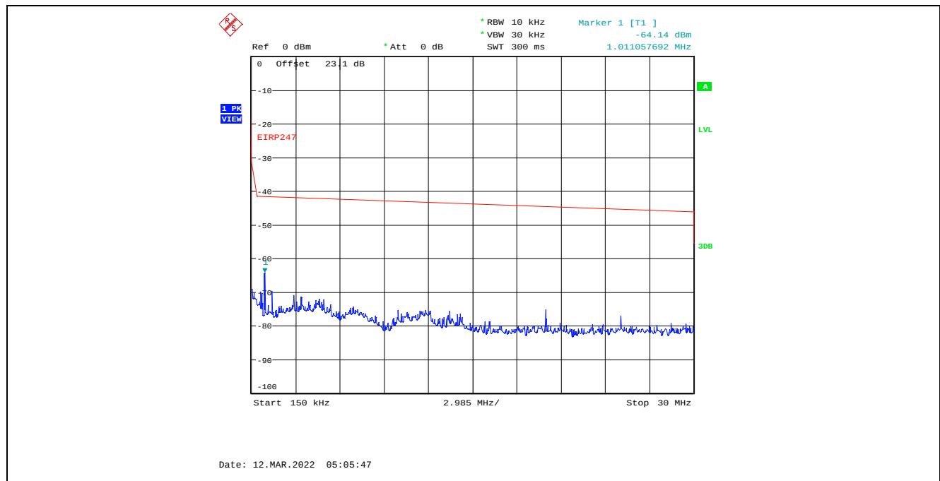
Plot C.2.93. Conducted Spurious Emissions in Restricted Frequency Bands, Chain 1 40 MHz Channel Bandwidth, Data Rate 7, Raw Power Setting 20, 2422 MHz, 150 kHz – 30 MHz, Peak Detector
