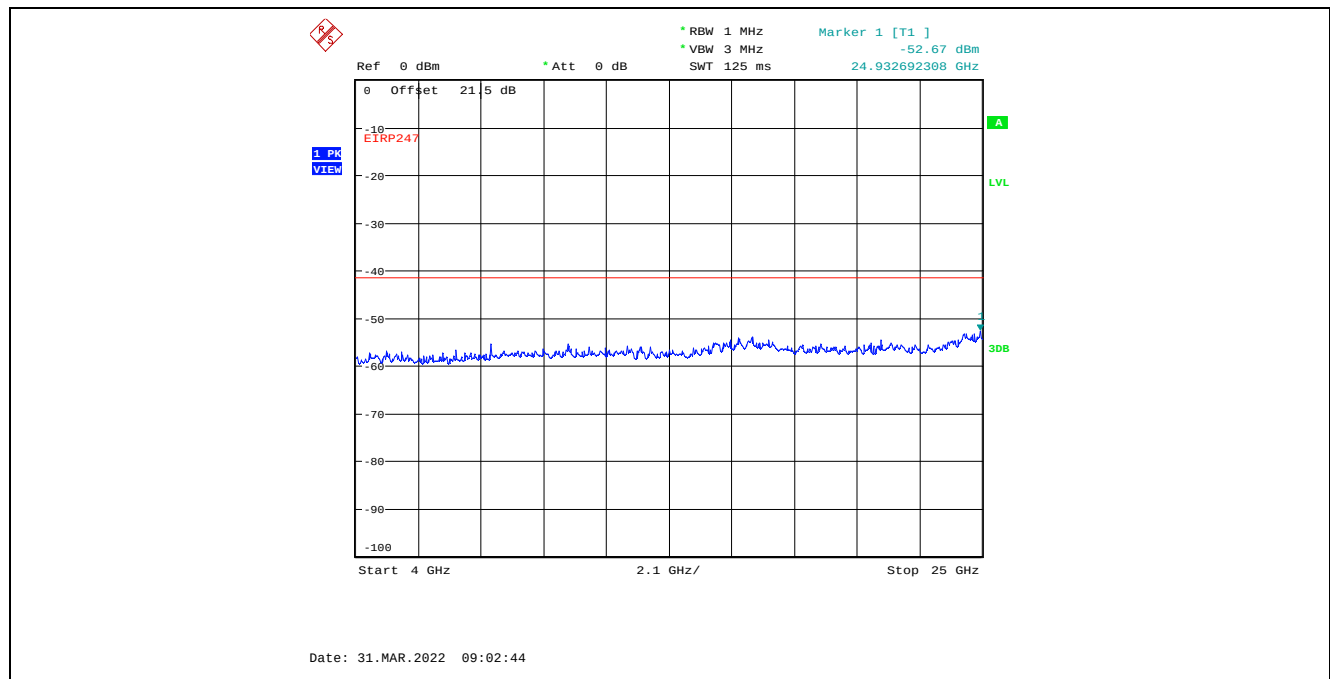
Plot C.3.120. Conducted Spurious Emissions in Restricted Frequency Bands, Chain 2 40 MHz Channel Bandwidth, Data Rate 3, Raw Power Setting 0, 2452 MHz, 4 GHz - 25 GHz, Peak Detector
