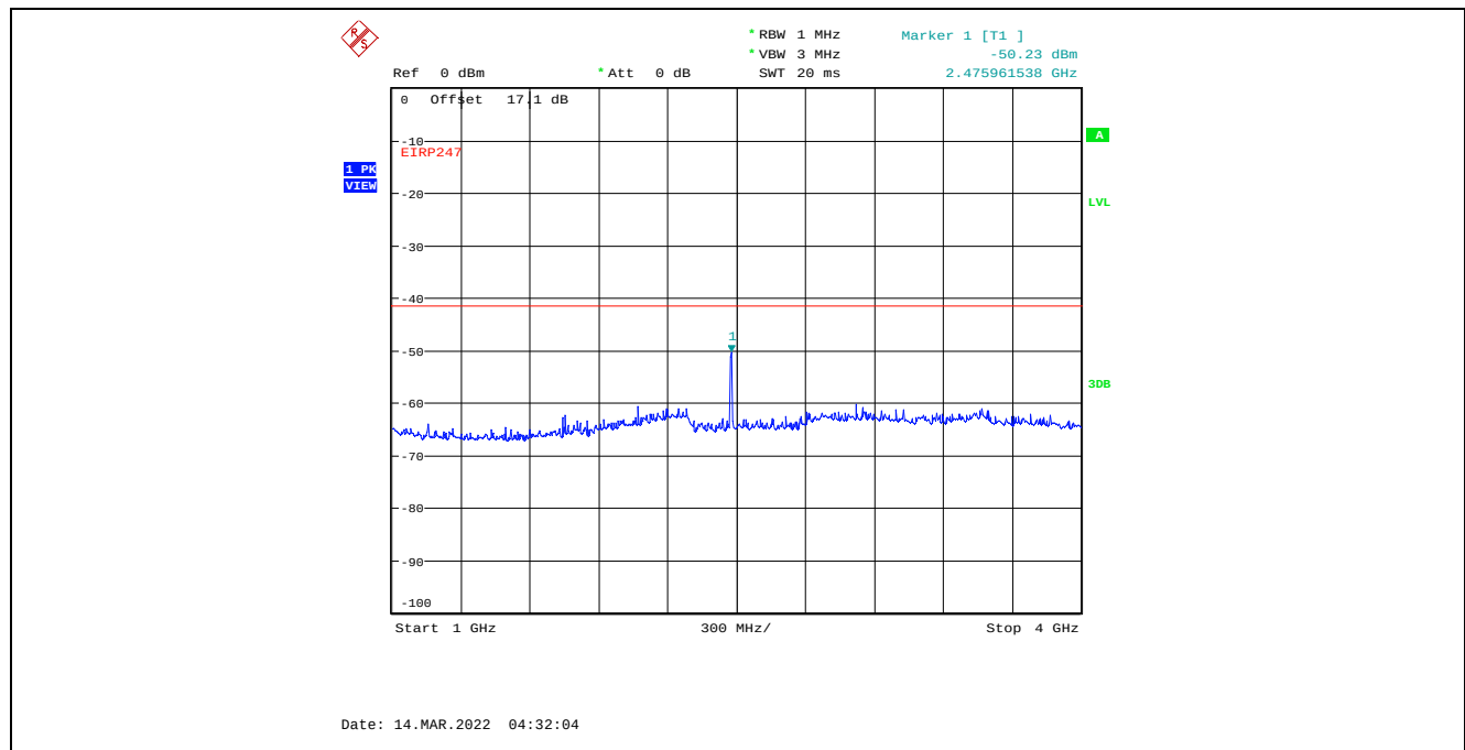
Plot C.2.57. Conducted Spurious Emissions in Restricted Frequency Bands, Chain 1 8 MHz Channel Bandwidth, Data Rate 7, Raw Power Setting 12, 2476 MHz, 1 GHz – 4 GHz, Peak Detector
