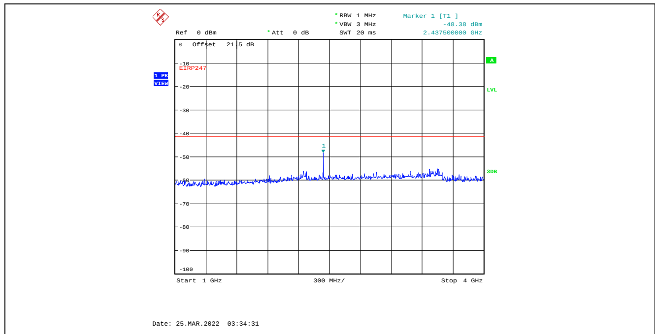
Plot C.3.18. Conducted Spurious Emissions in Restricted Frequency Bands, Chain 2 4 MHz Channel Bandwidth, Data Rate 3, Raw Power Setting 8, 2437 MHz, 1 GHz – 4 GHz, Peak Detector
