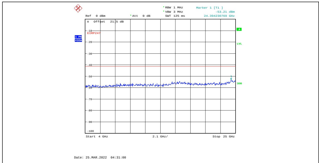
Plot C.4.19. Conducted Spurious Emissions in Restricted Frequency Bands, Chain 1 4 MHz Channel Bandwidth, Data Rate 7, Raw Power Setting 0, 2437 MHz, 4 GHz - 25 GHz, Peak Detector
