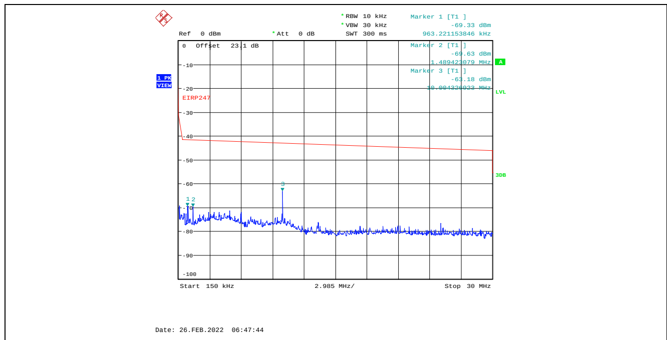
Plot C.2.14. Conducted Spurious Emissions in Restricted Frequency Bands, Chain 2 4 MHz Channel Bandwidth, Data Rate 7, Raw Power Setting 22, 2437 MHz, 150 kHz – 30 MHz, Peak Detector
