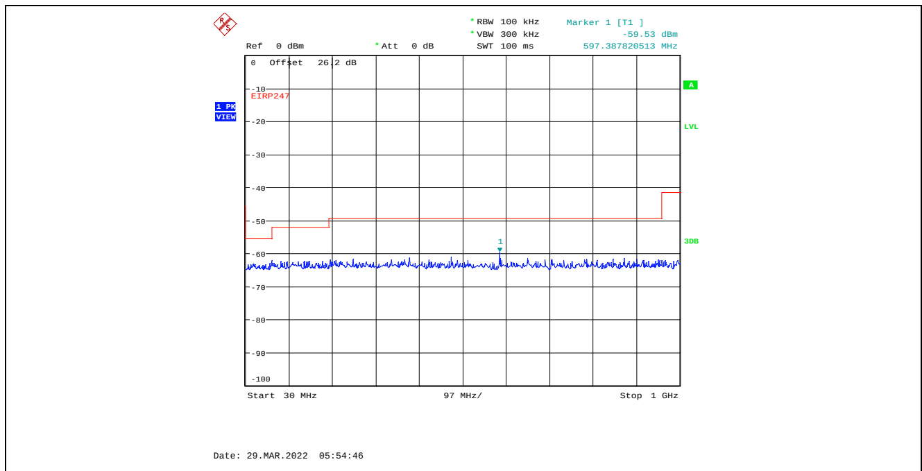
Plot C.4.75. Conducted Spurious Emissions in Restricted Frequency Bands, Chain 1 20 MHz Channel Bandwidth, Data Rate 7, Raw Power Setting 0, 2437 MHz, 30 MHz - 1 GHz, Peak Detector
