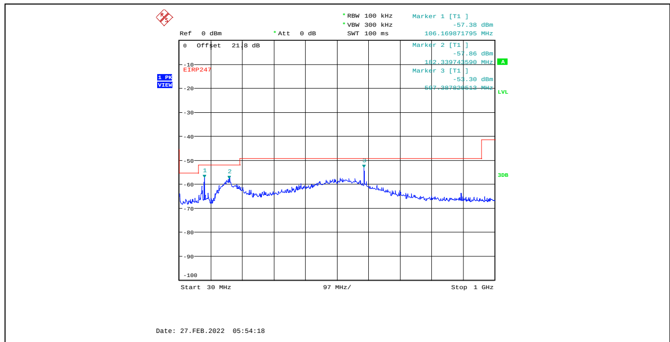
Plot C.1.45. Conducted Spurious Emissions in Restricted Frequency Bands, Chain 1 8 MHz Channel Bandwidth, Data Rate 3, Raw Power Setting 21, 2437 MHz, 30 MHz - 1 GHz, Peak Detector
