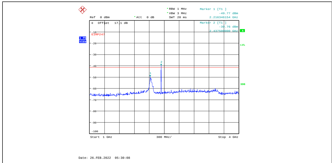
Plot C.2.17. Conducted Spurious Emissions in Restricted Frequency Bands, Chain 1 4 MHz Channel Bandwidth, Data Rate 7, Raw Power Setting 22, 2437 MHz, 1 GHz – 4 GHz, Peak Detector Marker 2 is Fundamental Signal
