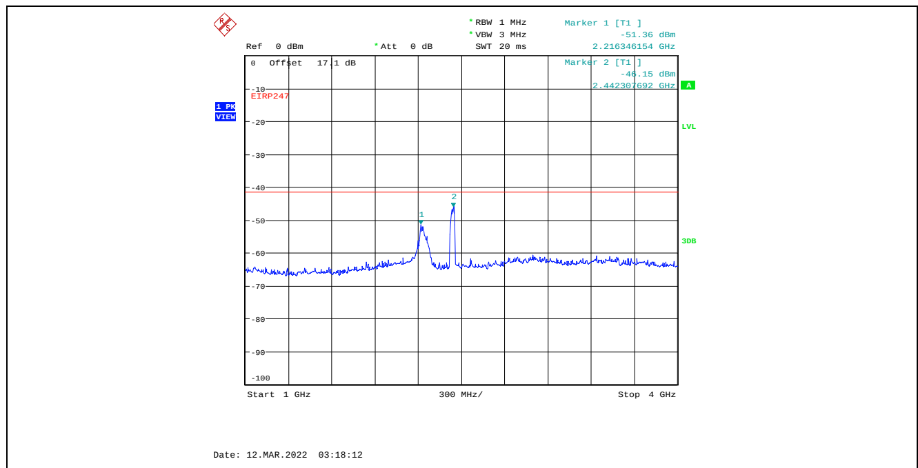
Plot C.1.108. Conducted Spurious Emissions in Restricted Frequency Bands, Chain 2 40 MHz Channel Bandwidth, Data Rate 3, Raw Power Setting 22, 2437 MHz, 1 GHz – 4 GHz, Peak Detector
