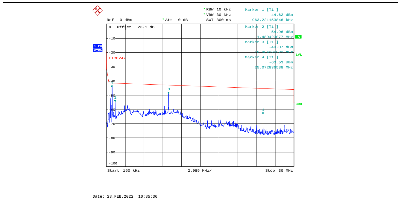
Plot C.1.13. Conducted Spurious Emissions in Restricted Frequency Bands, Chain 1 4 MHz Channel Bandwidth, Data Rate 3, Raw Power Setting 16, 2437 MHz, 150 kHz – 30 MHz, Peak Detector
