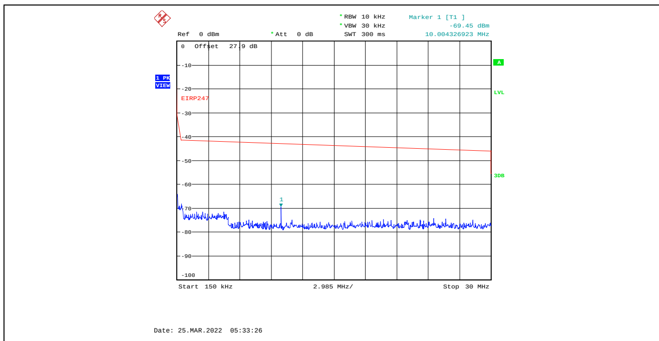
Plot C.4.23. Conducted Spurious Emissions in Restricted Frequency Bands, Chain 1 4 MHz Channel Bandwidth, Data Rate 7, Raw Power Setting 0, 2477 MHz, 150 kHz – 30 MHz, Peak Detector
