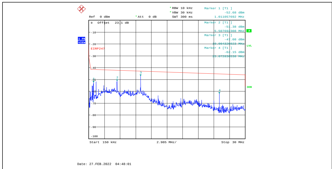
Plot C.1.44. Conducted Spurious Emissions in Restricted Frequency Bands, Chain 2 8 MHz Channel Bandwidth, Data Rate 3, Raw Power Setting 21, 2437 MHz, 150 kHz – 30 MHz, Peak Detector
