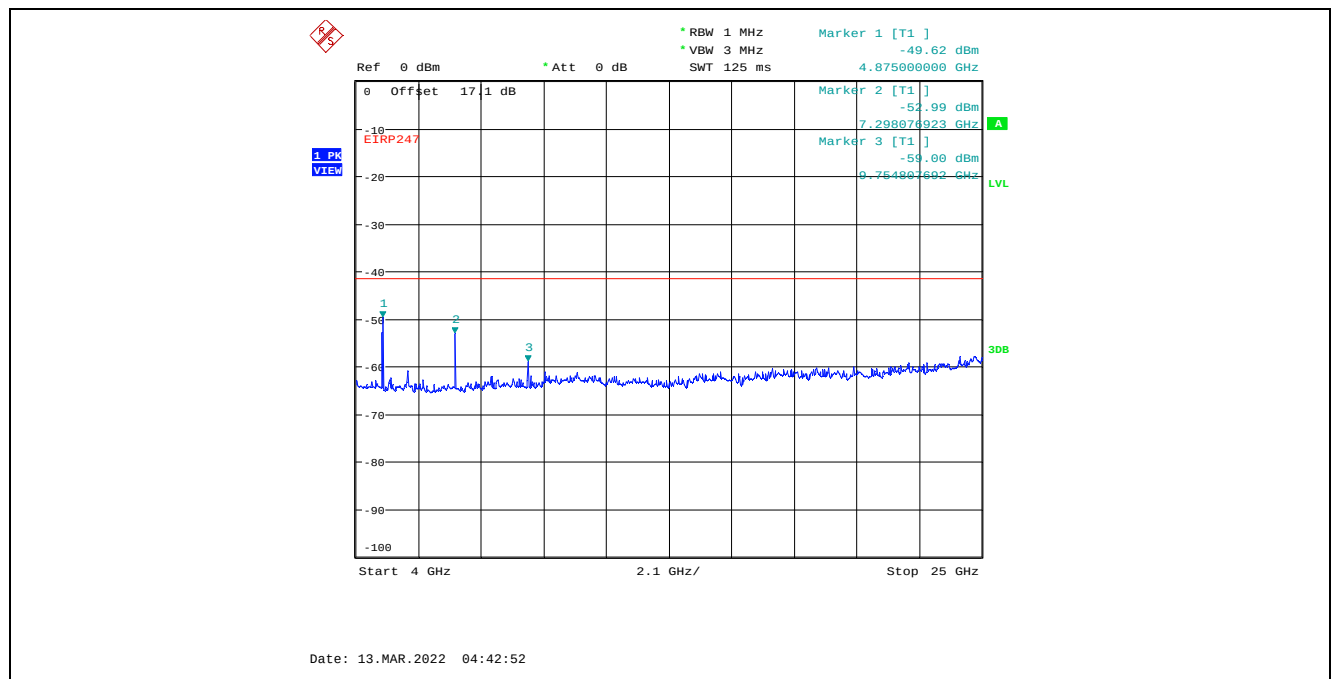
Plot C.1.80. Conducted Spurious Emissions in Restricted Frequency Bands, Chain 2 20 MHz Channel Bandwidth, Data Rate 3, Raw Power Setting 26, 2437 MHz, 4 GHz - 25 GHz, Peak Detector
