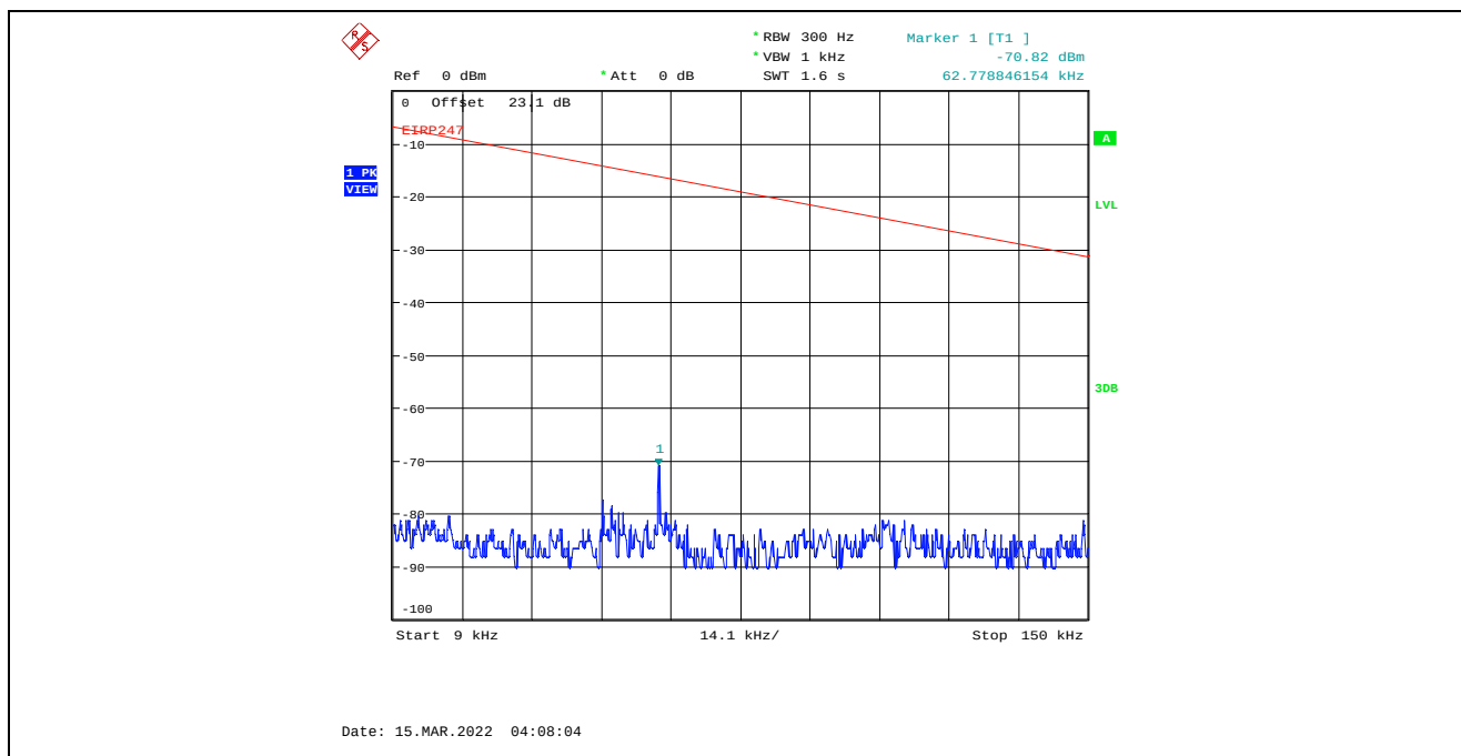
Plot C.2.21. Conducted Spurious Emissions in Restricted Frequency Bands, Chain 1 4 MHz Channel Bandwidth, Data Rate 7, Raw Power Setting 20, 2477 MHz, 9 kHz - 150 kHz, Peak Detector
