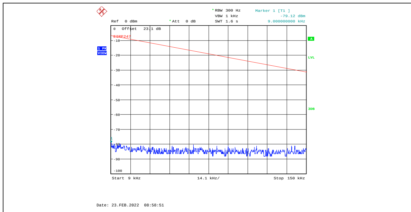
Plot C.1.11. Conducted Spurious Emissions in Restricted Frequency Bands, Chain 1 4 MHz Channel Bandwidth, Data Rate 3, Raw Power Setting 16, 2437 MHz, 9 kHz - 150 kHz, Peak Detector
