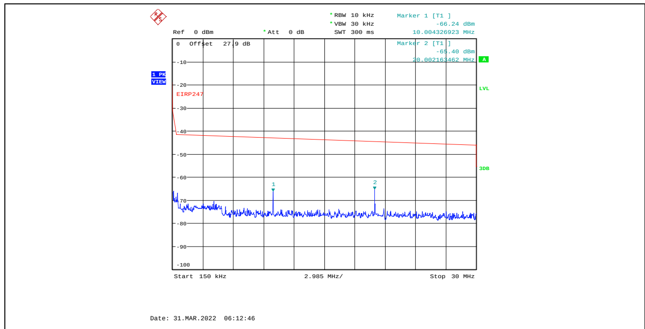
Plot C.4.113. Conducted Spurious Emissions in Restricted Frequency Bands, Chain 1 40 MHz Channel Bandwidth, Data Rate 7, Raw Power Setting 0, 2452 MHz, 150 kHz – 30 MHz, Peak Detector
