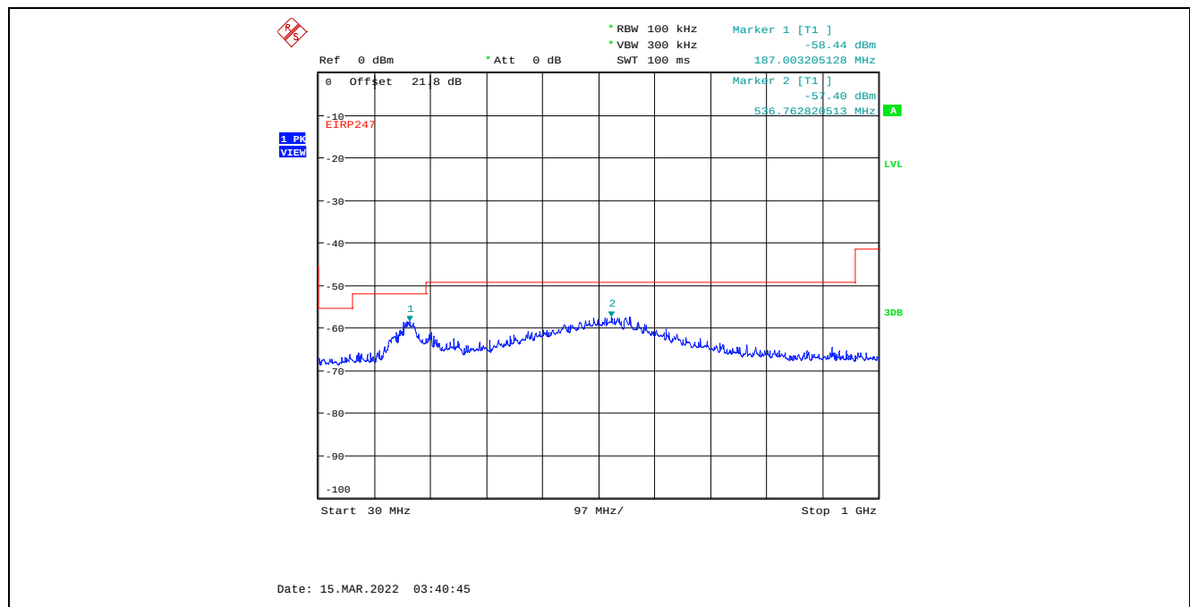
Plot C.1.26. Conducted Spurious Emissions in Restricted Frequency Bands, Chain 2 4 MHz Channel Bandwidth, Data Rate 3, Raw Power Setting 13, 2477 MHz, 30 MHz - 1 GHz, Peak Detector
