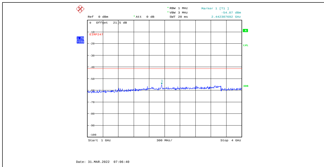
Plot C.3.107. Conducted Spurious Emissions in Restricted Frequency Bands, Chain 1 40 MHz Channel Bandwidth, Data Rate 3, Raw Power Setting 0, 2437 MHz, 1 GHz – 4 GHz, Peak Detector
