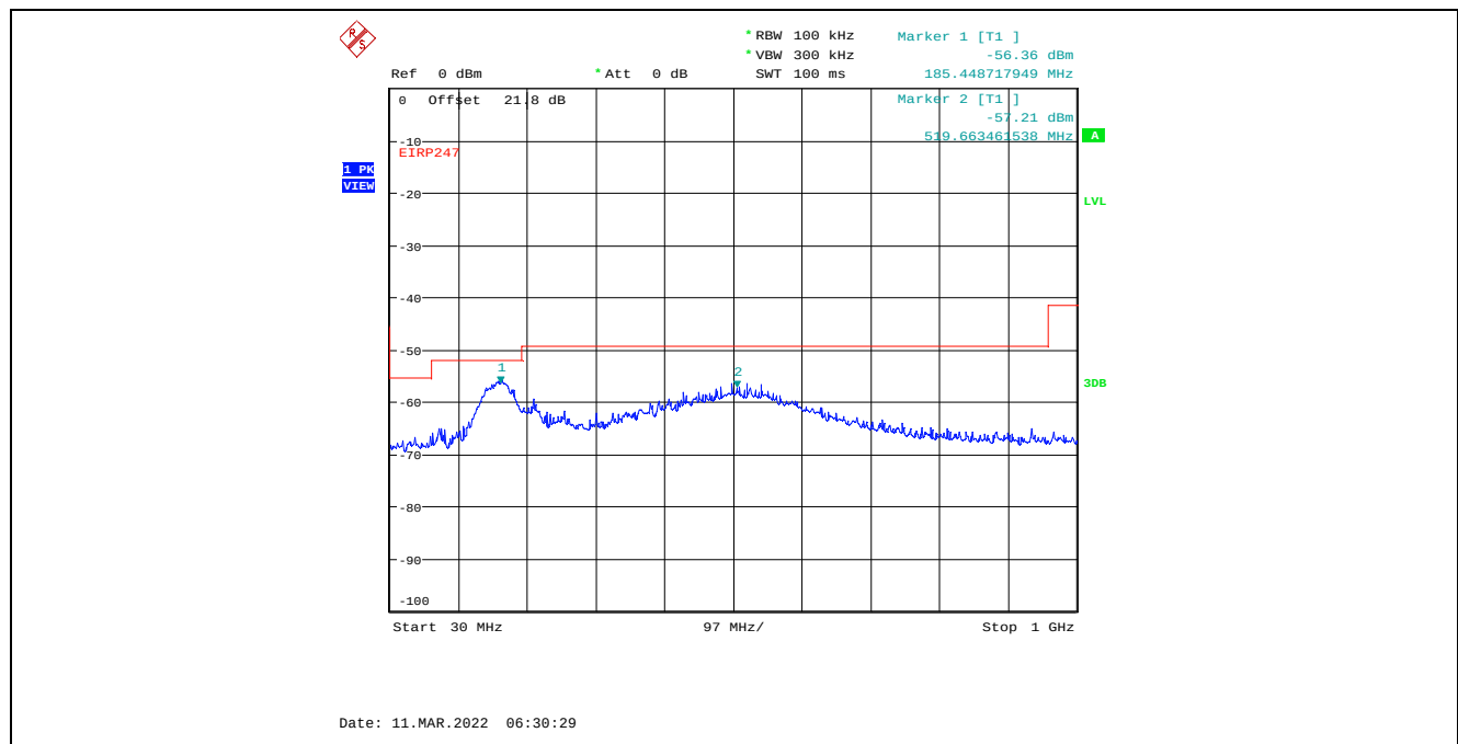
Plot C.1.116. Conducted Spurious Emissions in Restricted Frequency Bands, Chain 2 40 MHz Channel Bandwidth, Data Rate 3, Raw Power Setting 15, 2452 MHz, 30 MHz - 1 GHz, Peak Detector
