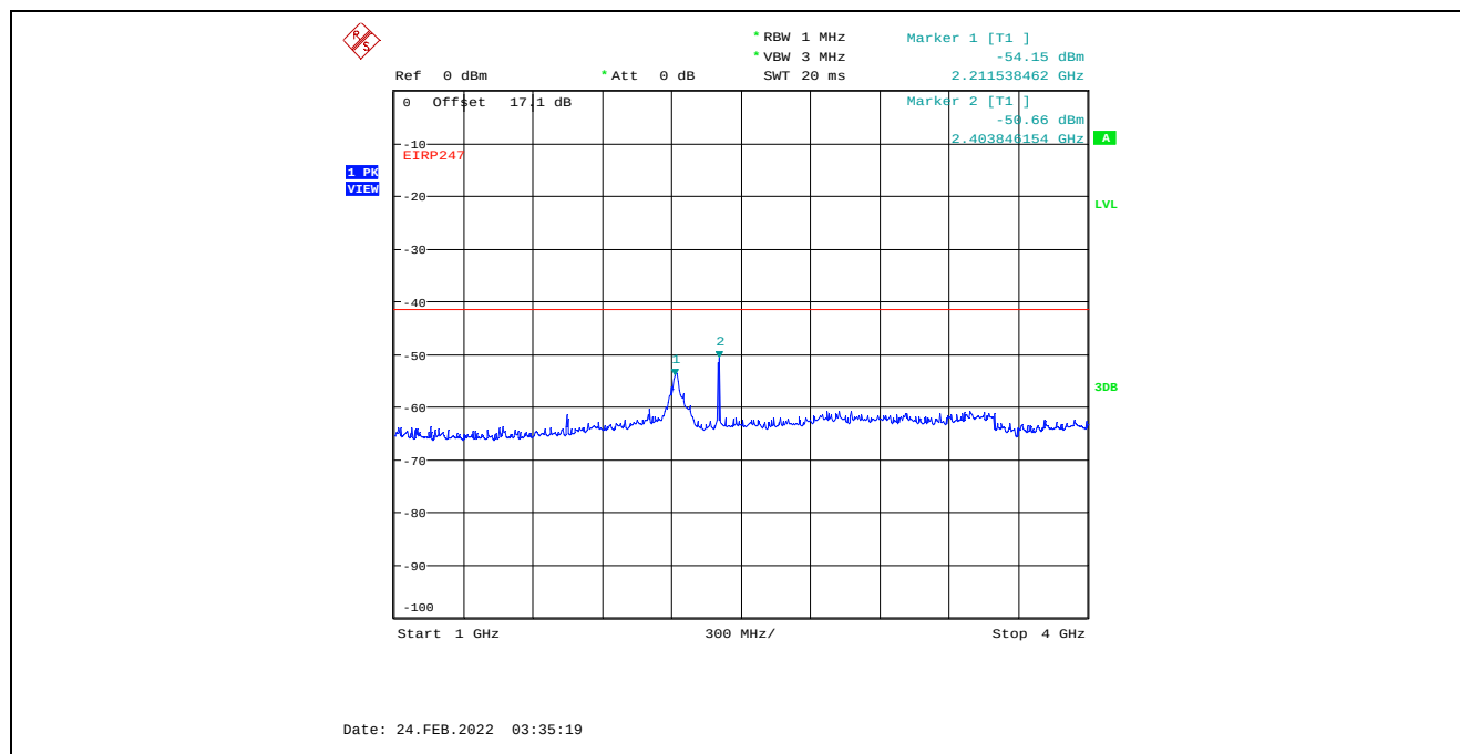
Plot C.1.7. Conducted Spurious Emissions in Restricted Frequency Bands, Chain 1 4 MHz Channel Bandwidth, Data Rate 3, Raw Power Setting 16, 2402 MHz, 1 GHz – 4 GHz, Peak Detector
