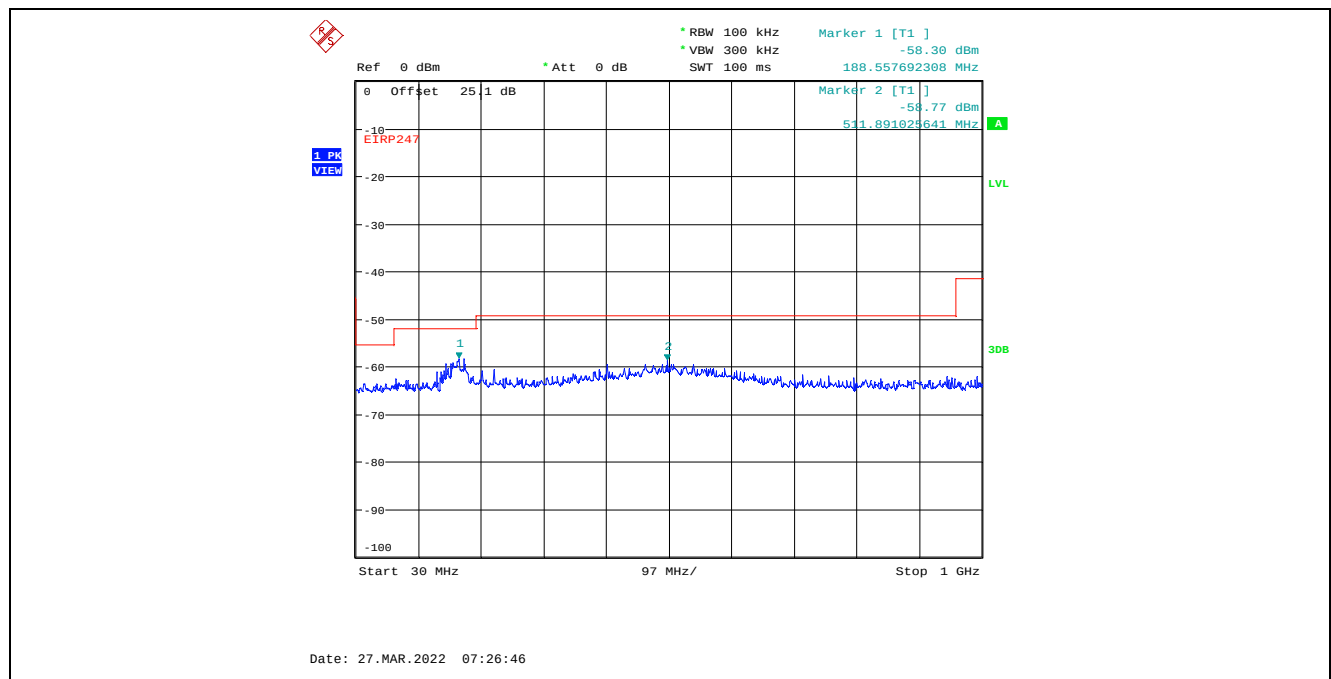
Plot C.4.36. Conducted Spurious Emissions in Restricted Frequency Bands, Chain 1 8 MHz Channel Bandwidth, Data Rate 7, Raw Power Setting 0, 2407 MHz, 30 MHz - 1 GHz, Peak Detector
