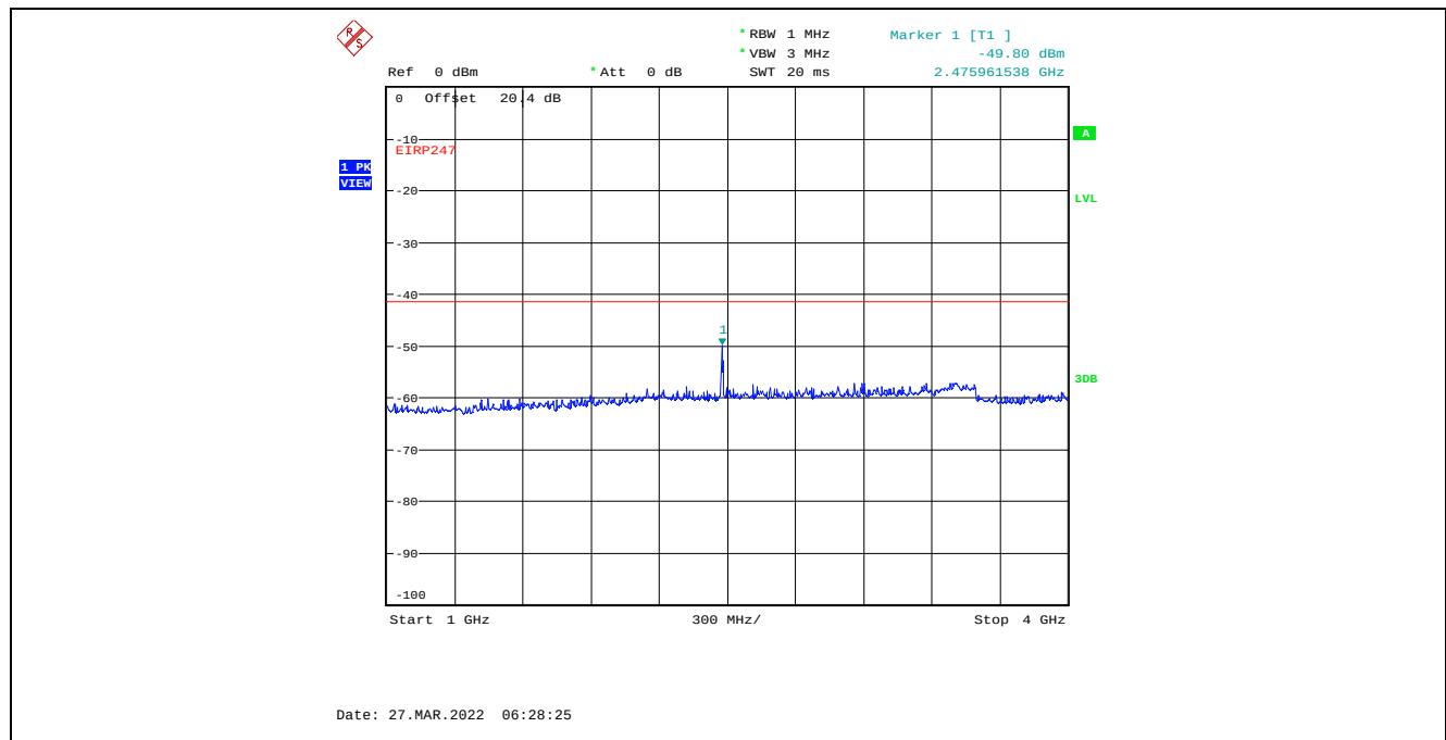
Plot C.3.57. Conducted Spurious Emissions in Restricted Frequency Bands, Chain 1 8 MHz Channel Bandwidth, Data Rate 3, Raw Power Setting 0, 2476 MHz, 1 GHz – 4 GHz, Peak Detector
