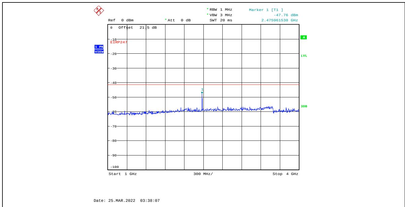
Plot C.3.28. Conducted Spurious Emissions in Restricted Frequency Bands, Chain 2 4 MHz Channel Bandwidth, Data Rate 3, Raw Power Setting 0, 2477 MHz, 1 GHz – 4 GHz, Peak Detector
