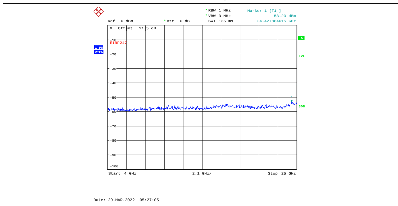
Plot C.4.70. Conducted Spurious Emissions in Restricted Frequency Bands, Chain 2 20 MHz Channel Bandwidth, Data Rate 7, Raw Power Setting 0, 2412 MHz, 4 GHz - 25 GHz, Peak Detector
