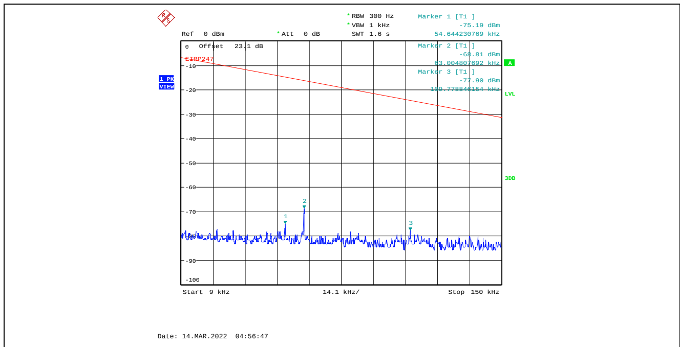
Plot C.2.52. Conducted Spurious Emissions in Restricted Frequency Bands, Chain 2 8 MHz Channel Bandwidth, Data Rate 7, Raw Power Setting 12, 2476 MHz, 9 kHz - 150 kHz, Peak Detector
