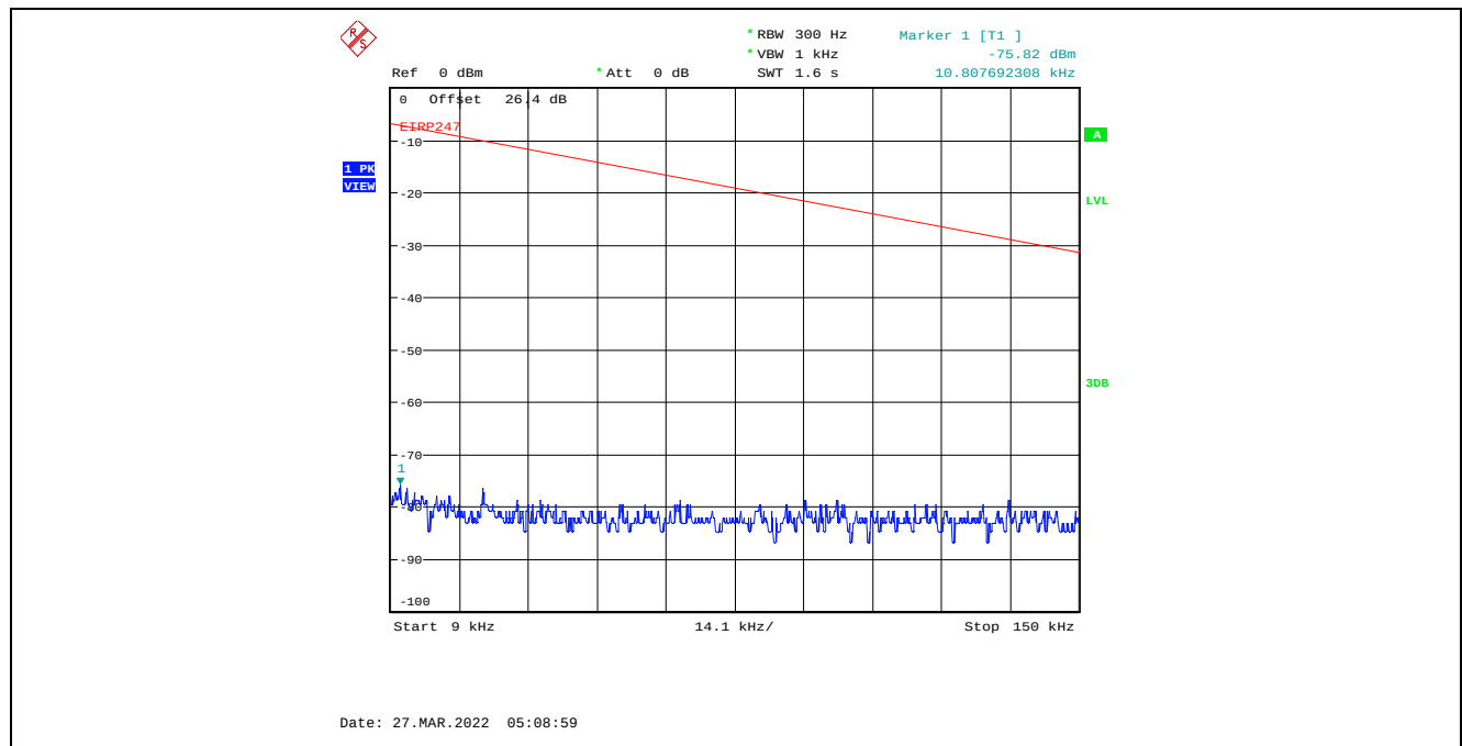
Plot C.3.52. Conducted Spurious Emissions in Restricted Frequency Bands, Chain 2 8 MHz Channel Bandwidth, Data Rate 3, Raw Power Setting 0, 2476 MHz, 9 kHz - 150 kHz, Peak Detector
