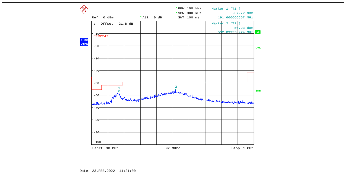
Plot C.1.6. Conducted Spurious Emissions in Restricted Frequency Bands, Chain 2 4 MHz Channel Bandwidth, Data Rate 3, Raw Power Setting 16, 2402 MHz, 30 MHz - 1 GHz, Peak Detector
