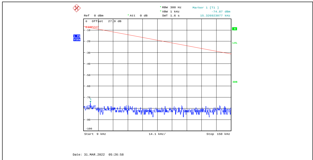
Plot C.3.101. Conducted Spurious Emissions in Restricted Frequency Bands, Chain 1 40 MHz Channel Bandwidth, Data Rate 3, Raw Power Setting 0, 2437 MHz, 9 kHz - 150 kHz, Peak Detector
