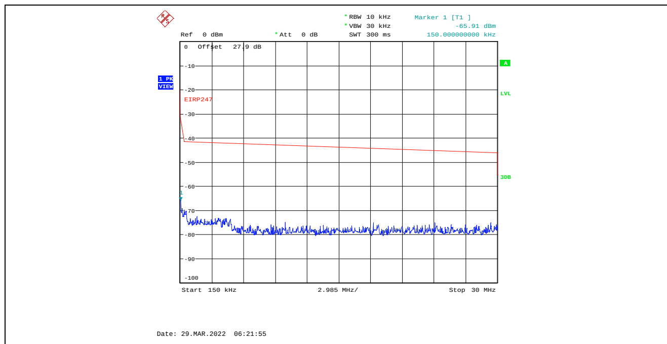
Plot C.4.73. Conducted Spurious Emissions in Restricted Frequency Bands, Chain 1 20 MHz Channel Bandwidth, Data Rate 7, Raw Power Setting 0, 2437 MHz, 150 kHz – 30 MHz, Peak Detector
