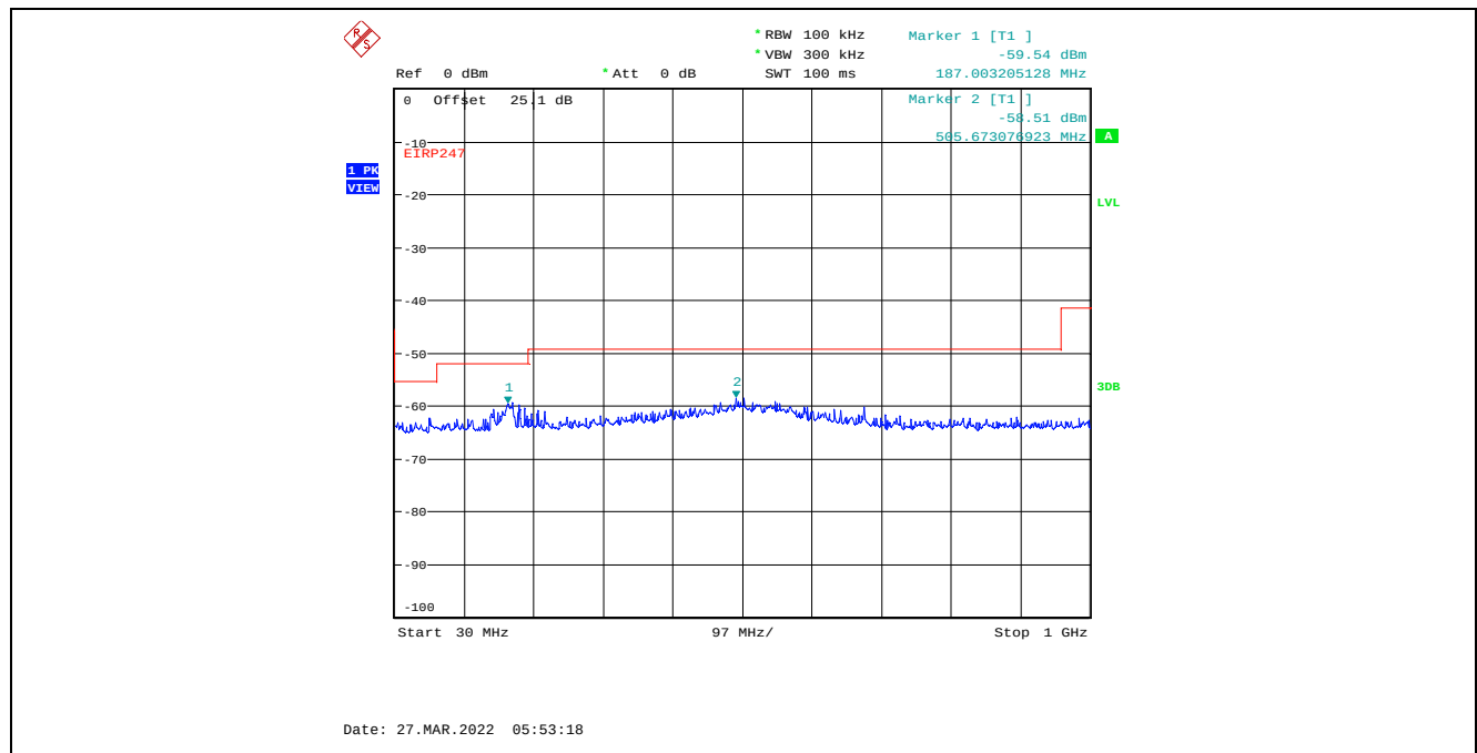
Plot C.3.36. Conducted Spurious Emissions in Restricted Frequency Bands, Chain 1 8 MHz Channel Bandwidth, Data Rate 3, Raw Power Setting 6, 2407 MHz, 30 MHz - 1 GHz, Peak Detector
