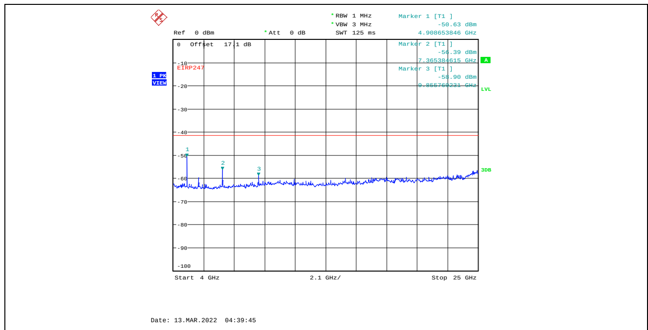
Plot C.1.90. Conducted Spurious Emissions in Restricted Frequency Bands, Chain 2 20 MHz Channel Bandwidth, Data Rate 3, Raw Power Setting 26, 2462 MHz, 4 GHz - 25 GHz, Peak Detector
