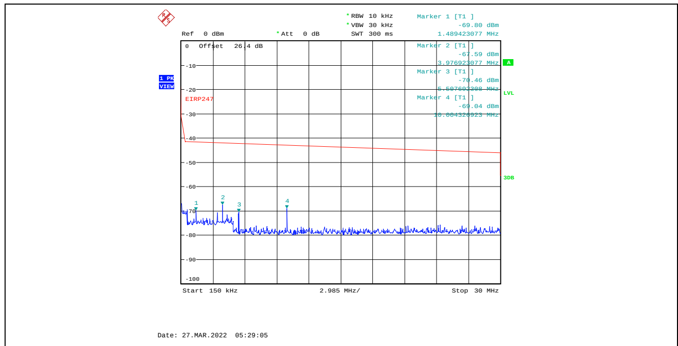
Plot C.3.54. Conducted Spurious Emissions in Restricted Frequency Bands, Chain 2 8 MHz Channel Bandwidth, Data Rate 3, Raw Power Setting 0, 2476 MHz, 150 kHz – 30 MHz, Peak Detector
