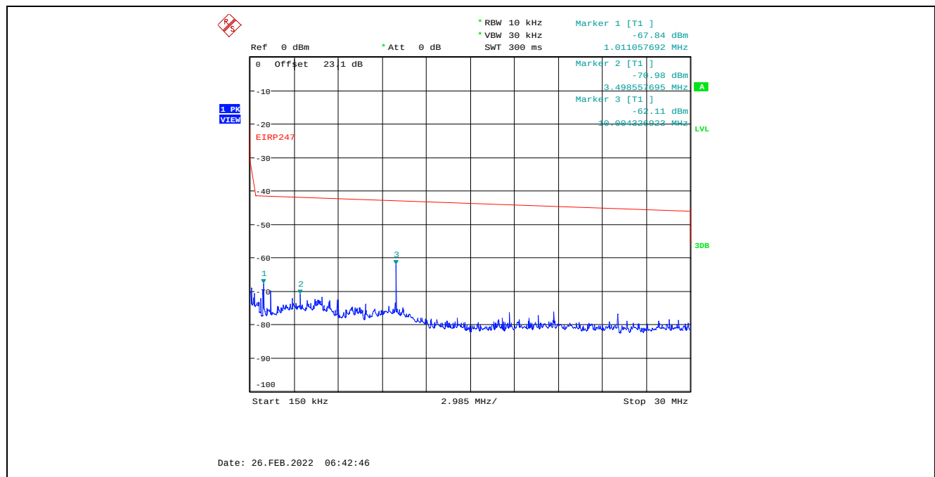
Plot C.2.4. Conducted Spurious Emissions in Restricted Frequency Bands, Chain 2 4 MHz Channel Bandwidth, Data Rate 7, Raw Power Setting 22, 2405 MHz, 150 kHz – 30 MHz, Peak Detector
