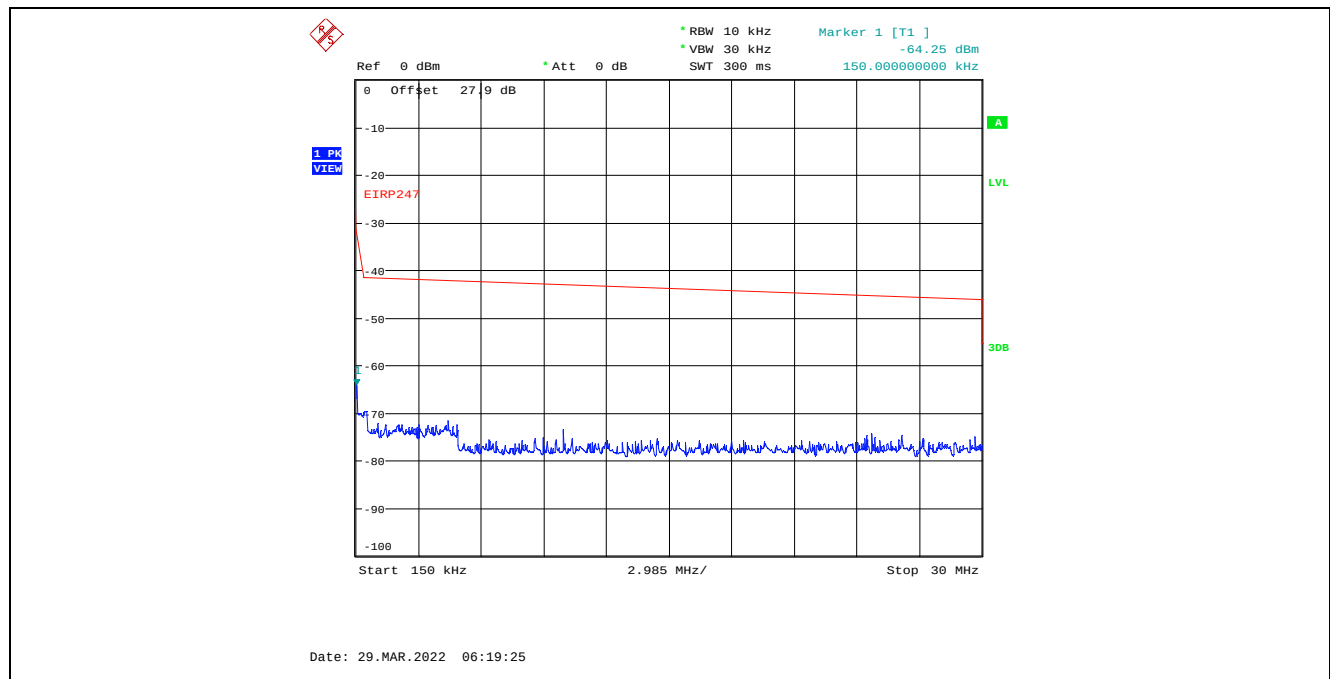
Plot C.4.63. Conducted Spurious Emissions in Restricted Frequency Bands, Chain 1 20 MHz Channel Bandwidth, Data Rate 7, Raw Power Setting 0, 2412 MHz, 150 kHz – 30 MHz, Peak Detector
