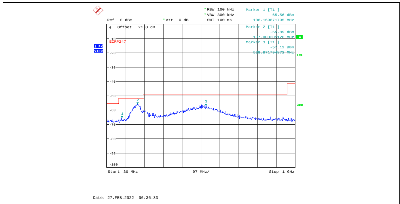
Plot C.2.46. Conducted Spurious Emissions in Restricted Frequency Bands, Chain 2 8 MHz Channel Bandwidth, Data Rate 7, Raw Power Setting 23, 2437 MHz, 30 MHz - 1 GHz, Peak Detector
