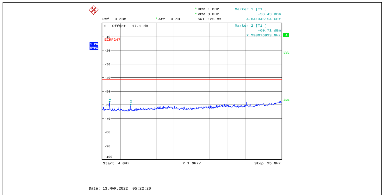
Plot C.2.79. Conducted Spurious Emissions in Restricted Frequency Bands, Chain 1 20 MHz Channel Bandwidth, Data Rate 7, Raw Power Setting 23, 2437 MHz, 4 GHz - 25 GHz, Peak Detector
