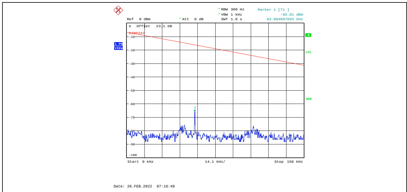
Plot C.2.2. Conducted Spurious Emissions in Restricted Frequency Bands, Chain 2 4 MHz Channel Bandwidth, Data Rate 7, Raw Power Setting 22, 2405 MHz, 9 kHz - 150 kHz, Peak Detector
