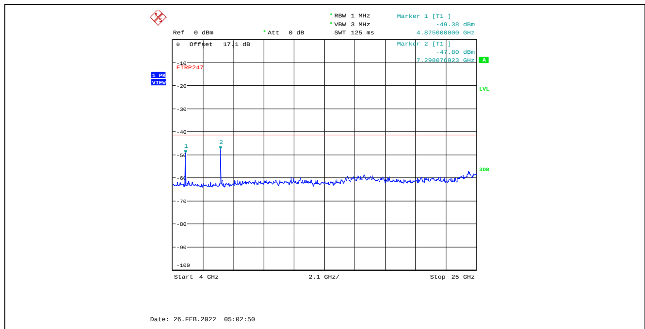
Plot C.2.20. Conducted Spurious Emissions in Restricted Frequency Bands, Chain 2 4 MHz Channel Bandwidth, Data Rate 7, Raw Power Setting 22, 2437 MHz, 4 GHz - 25 GHz, Peak Detector
