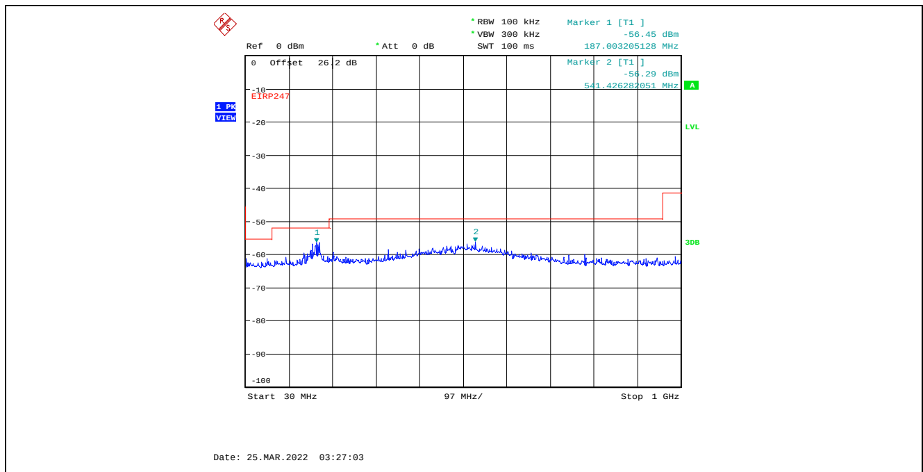
Plot C.3.16. Conducted Spurious Emissions in Restricted Frequency Bands, Chain 2 4 MHz Channel Bandwidth, Data Rate 3, Raw Power Setting 8, 2437 MHz, 30 MHz - 1 GHz, Peak Detector
