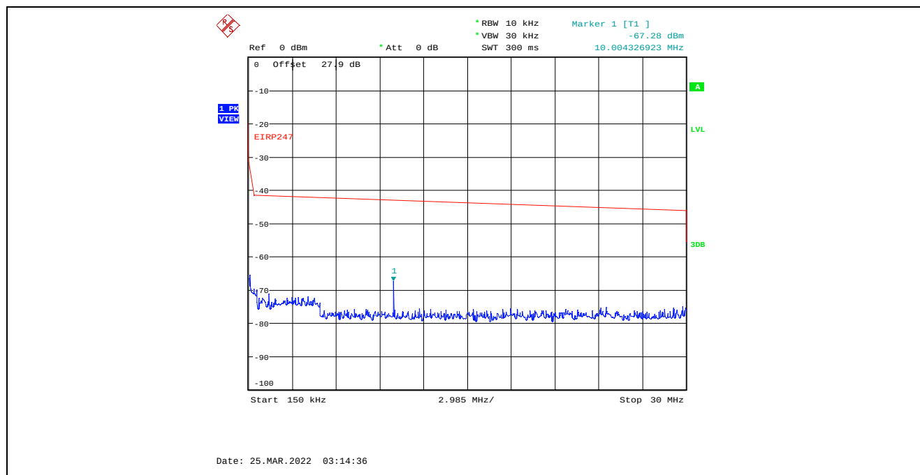
Plot C.3.3. Conducted Spurious Emissions in Restricted Frequency Bands, Chain 1 4 MHz Channel Bandwidth, Data Rate 3, Raw Power Setting 8, 2402 MHz, 150 kHz – 30 MHz, Peak Detector
