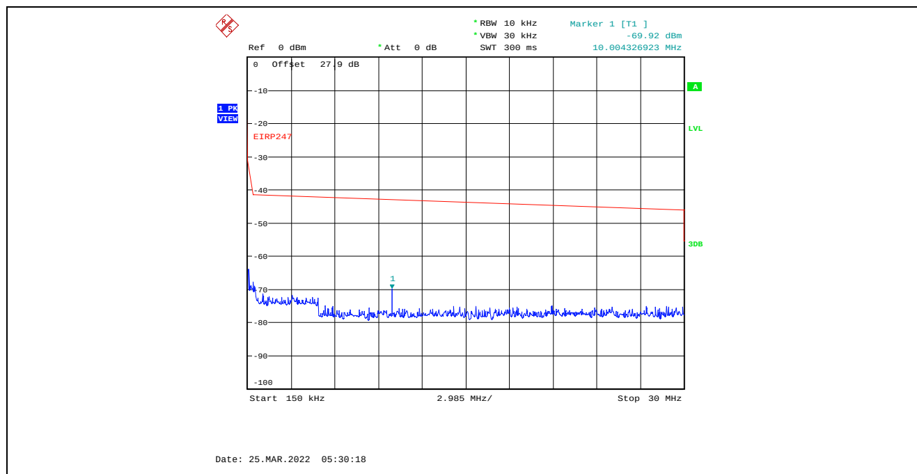
Plot C.4.3. Conducted Spurious Emissions in Restricted Frequency Bands, Chain 1 4 MHz Channel Bandwidth, Data Rate 7, Raw Power Setting 0, 2405 MHz, 150 kHz – 30 MHz, Peak Detector
