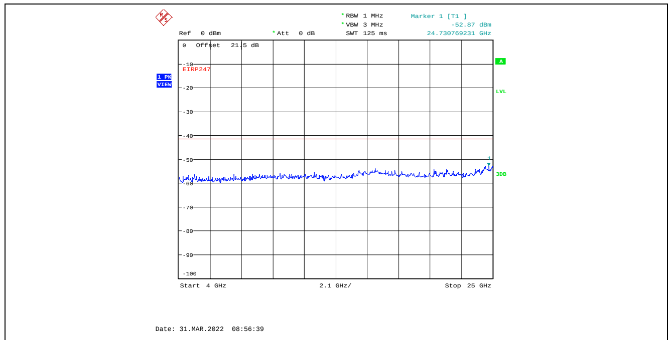
Plot C.4.109. Conducted Spurious Emissions in Restricted Frequency Bands, Chain 1 40 MHz Channel Bandwidth, Data Rate 7, Raw Power Setting 0, 2437 MHz, 4 GHz - 25 GHz, Peak Detector
