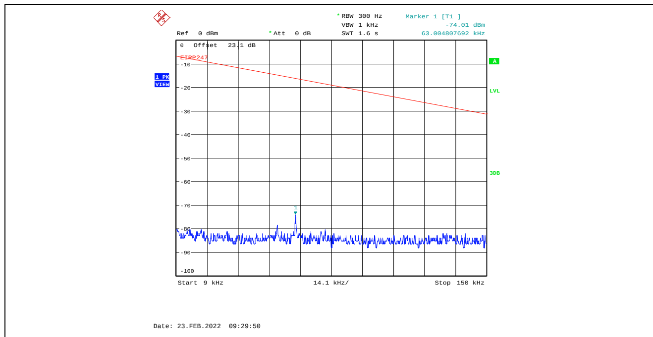
Plot C.1.12. Conducted Spurious Emissions in Restricted Frequency Bands, Chain 2 4 MHz Channel Bandwidth, Data Rate 3, Raw Power Setting 16, 2437 MHz, 9 kHz - 150 kHz, Peak Detector
