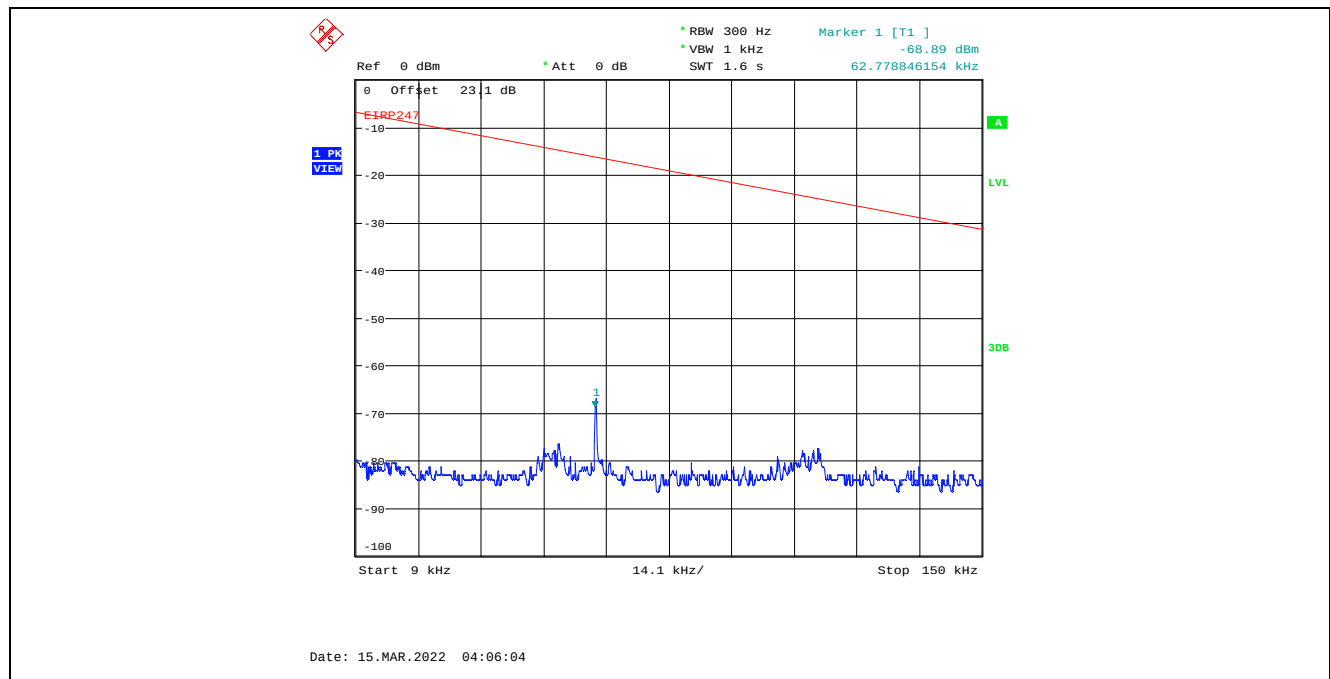
Plot C.1.21. Conducted Spurious Emissions in Restricted Frequency Bands, Chain 1 4 MHz Channel Bandwidth, Data Rate 3, Raw Power Setting 13, 2477 MHz, 9 kHz - 150 kHz, Peak Detector
