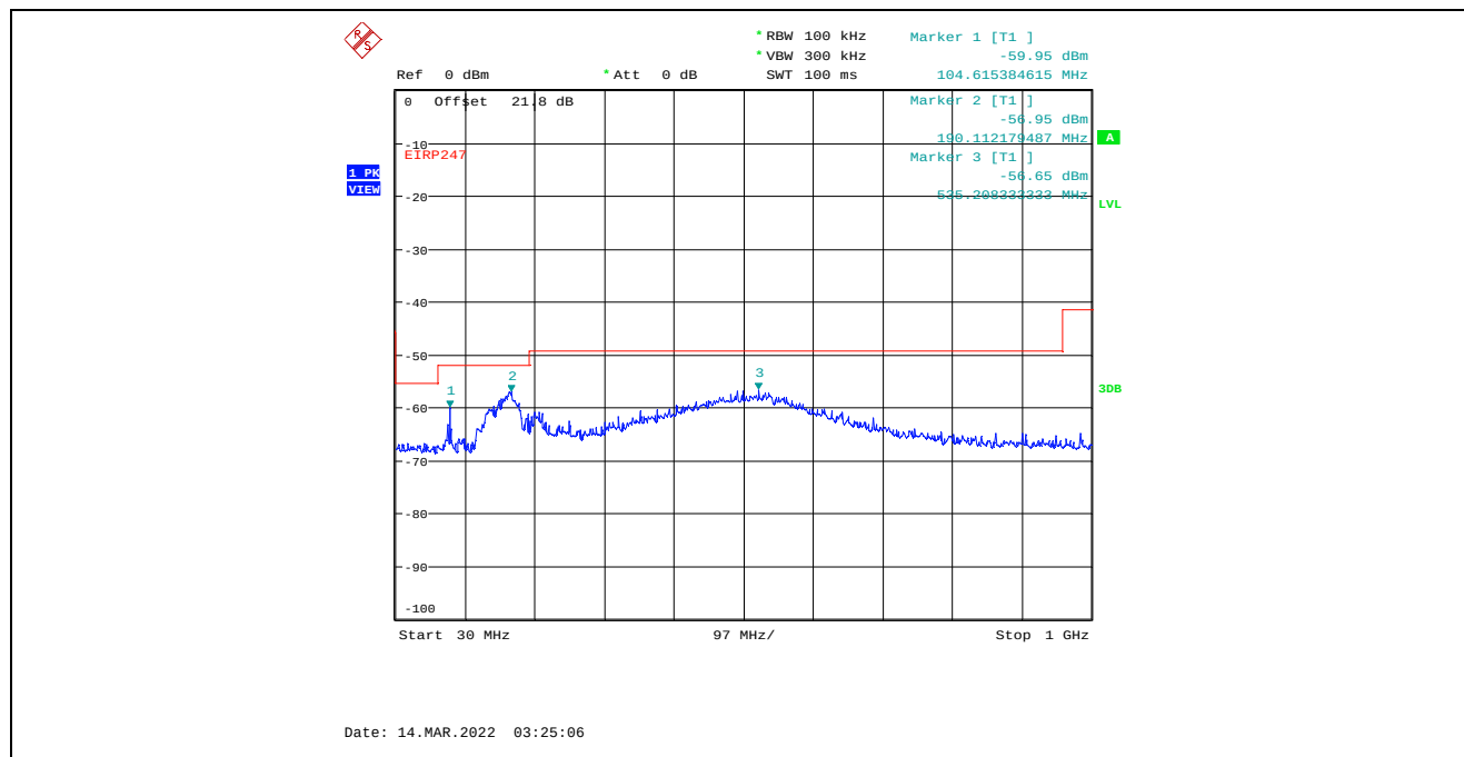
Plot C.1.56. Conducted Spurious Emissions in Restricted Frequency Bands, Chain 2 8 MHz Channel Bandwidth, Data Rate 3, Raw Power Setting 14, 2476 MHz, 30 MHz - 1 GHz, Peak Detector
