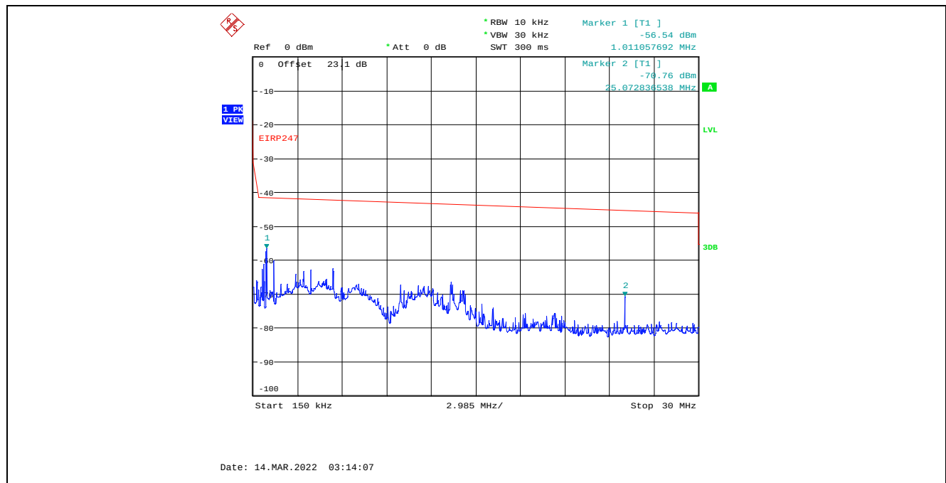
Plot C.1.53. Conducted Spurious Emissions in Restricted Frequency Bands, Chain 1 8 MHz Channel Bandwidth, Data Rate 3, Raw Power Setting 14, 2476 MHz, 150 kHz – 30 MHz, Peak Detector
