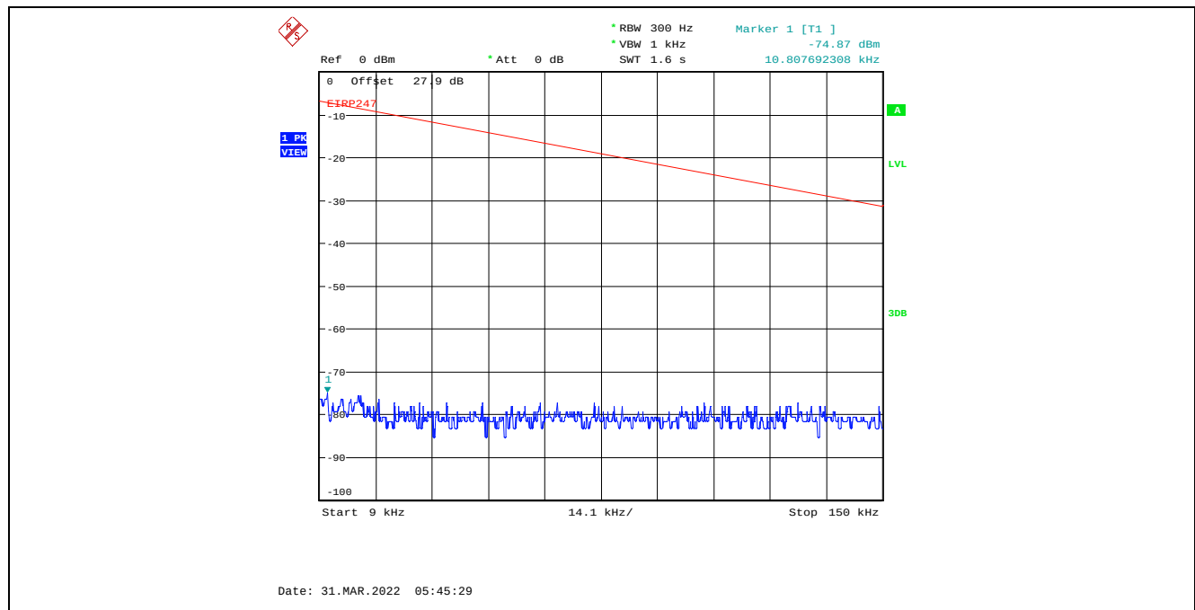
Plot C.3.92. Conducted Spurious Emissions in Restricted Frequency Bands, Chain 2 40 MHz Channel Bandwidth, Data Rate 3, Raw Power Setting 0, 2422 MHz, 9 kHz - 150 kHz, Peak Detector
