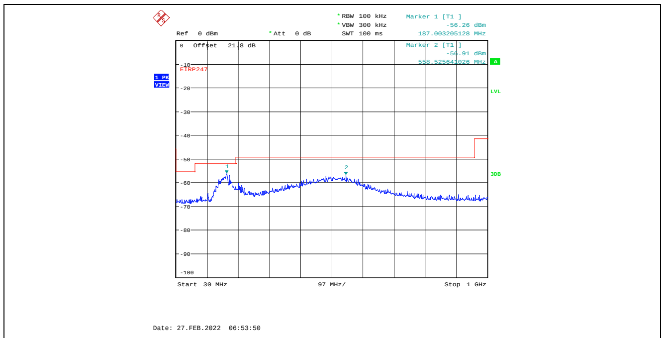
Plot C.1.36. Conducted Spurious Emissions in Restricted Frequency Bands, Chain 2 8 MHz Channel Bandwidth, Data Rate 3, Raw Power Setting 21, 2407 MHz, 30 MHz - 1 GHz, Peak Detector
