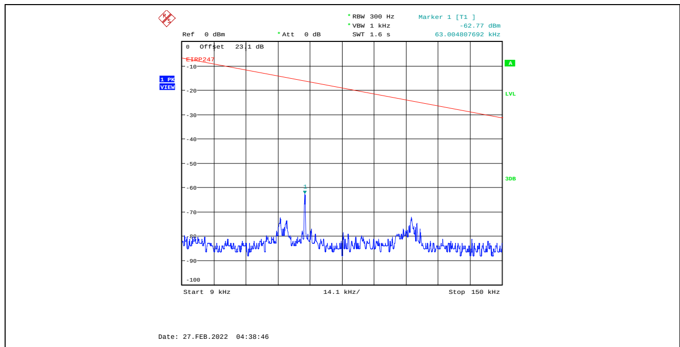
Plot C.1.42. Conducted Spurious Emissions in Restricted Frequency Bands, Chain 2 8 MHz Channel Bandwidth, Data Rate 3, Raw Power Setting 21, 2437 MHz, 9 kHz - 150 kHz, Peak Detector
