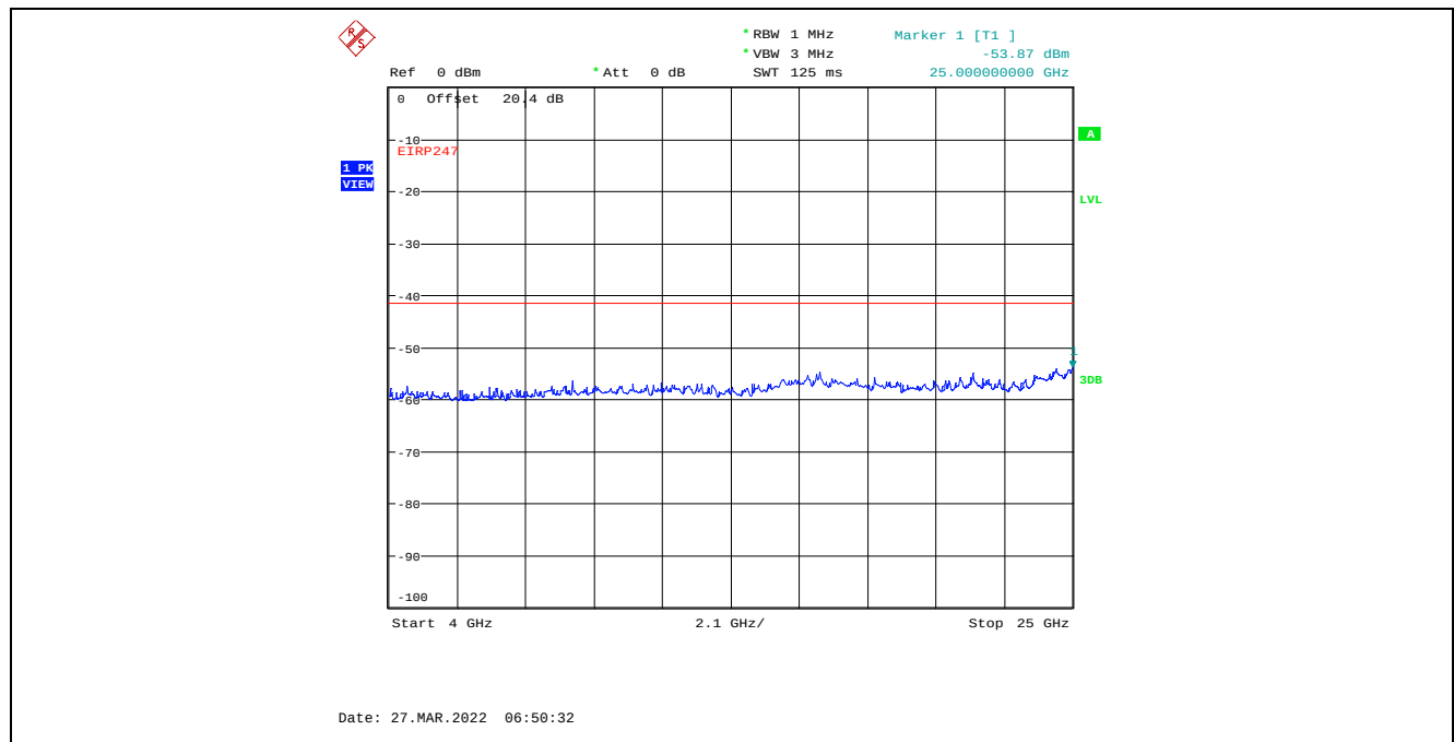
Plot C.4.49. Conducted Spurious Emissions in Restricted Frequency Bands, Chain 1 8 MHz Channel Bandwidth, Data Rate 7, Raw Power Setting 0, 2437 MHz, 4 GHz - 25 GHz, Peak Detector
