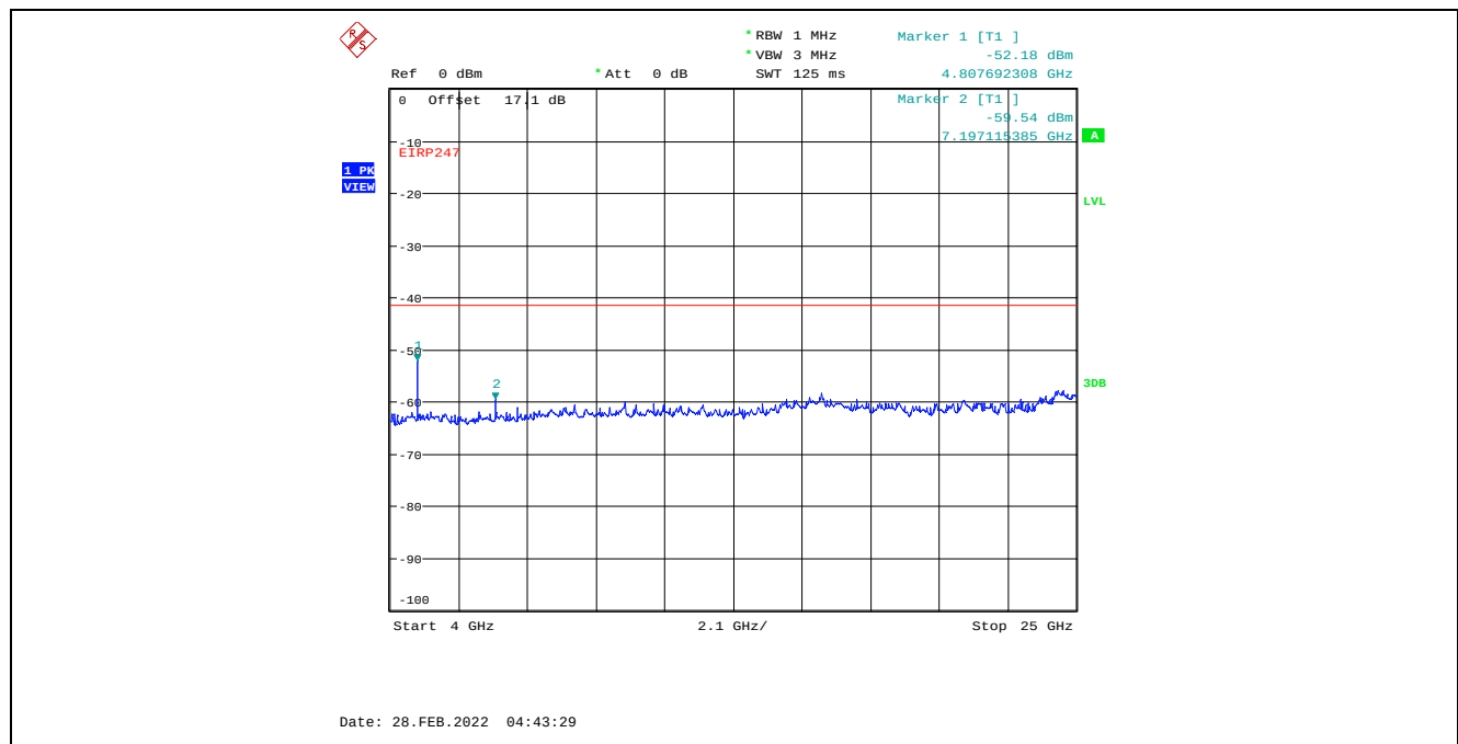
Plot C.1.40. Conducted Spurious Emissions in Restricted Frequency Bands, Chain 2 8 MHz Channel Bandwidth, Data Rate 3, Raw Power Setting 21, 2407 MHz, 4 GHz - 25 GHz, Peak Detector
