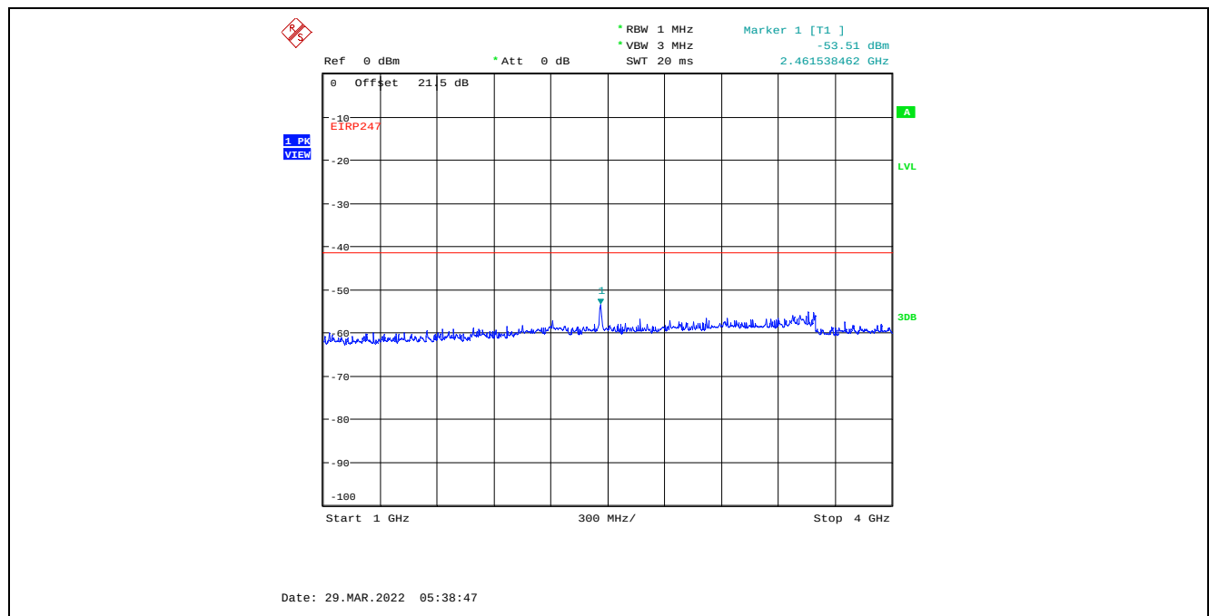
Plot C.4.88. Conducted Spurious Emissions in Restricted Frequency Bands, Chain 2 20 MHz Channel Bandwidth, Data Rate 7, Raw Power Setting 0, 2462 MHz, 1 GHz – 4 GHz, Peak Detector
