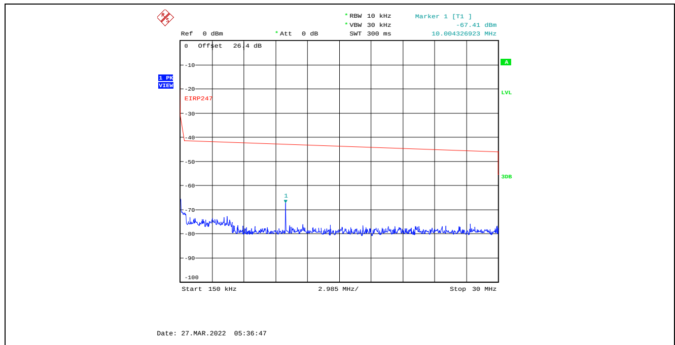
Plot C.3.43. Conducted Spurious Emissions in Restricted Frequency Bands, Chain 1 8 MHz Channel Bandwidth, Data Rate 3, Raw Power Setting 6, 2437 MHz, 150 kHz – 30 MHz, Peak Detector
