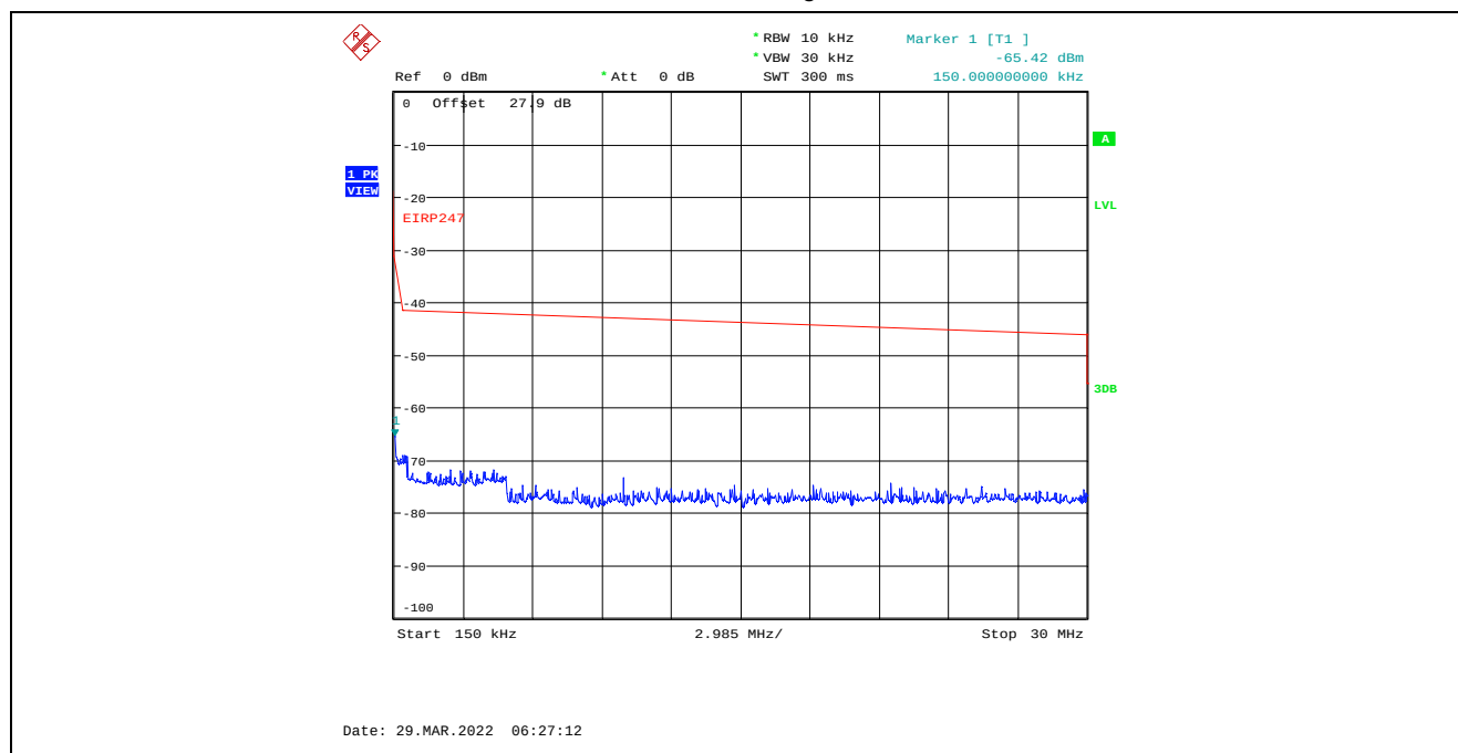
Plot C.4.74. Conducted Spurious Emissions in Restricted Frequency Bands, Chain 2 20 MHz Channel Bandwidth, Data Rate 7, Raw Power Setting 0, 2437 MHz, 150 kHz – 30 MHz, Peak Detector
