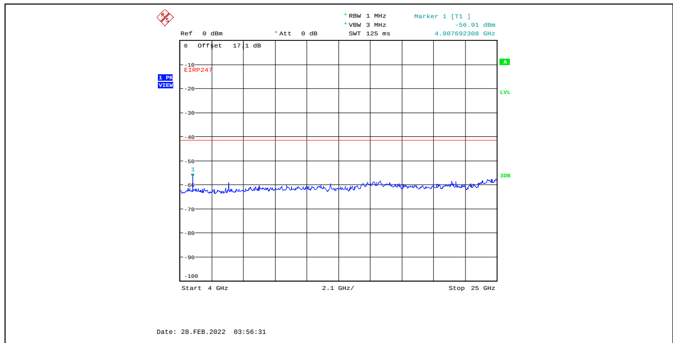
Plot C.1.39. Conducted Spurious Emissions in Restricted Frequency Bands, Chain 1 8 MHz Channel Bandwidth, Data Rate 3, Raw Power Setting 21, 2407 MHz, 4 GHz - 25 GHz, Peak Detector
