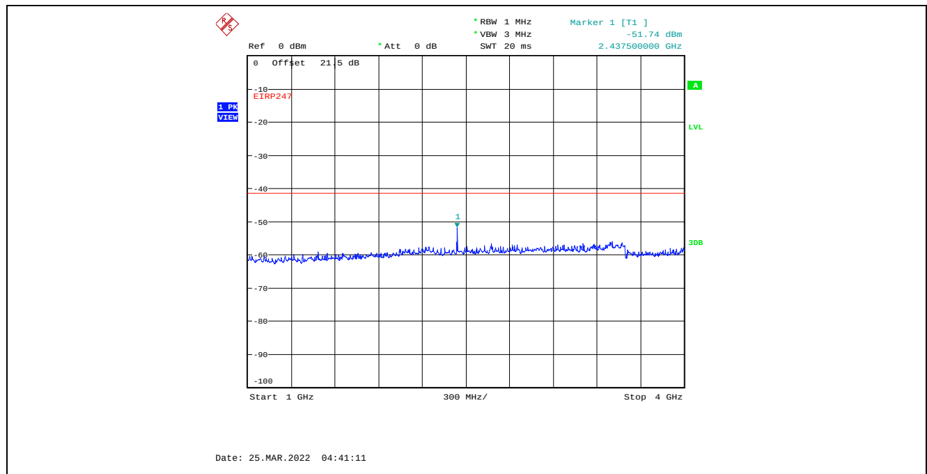
Plot C.4.17. Conducted Spurious Emissions in Restricted Frequency Bands, Chain 1 4 MHz Channel Bandwidth, Data Rate 7, Raw Power Setting 0, 2437 MHz, 1 GHz – 4 GHz, Peak Detector
