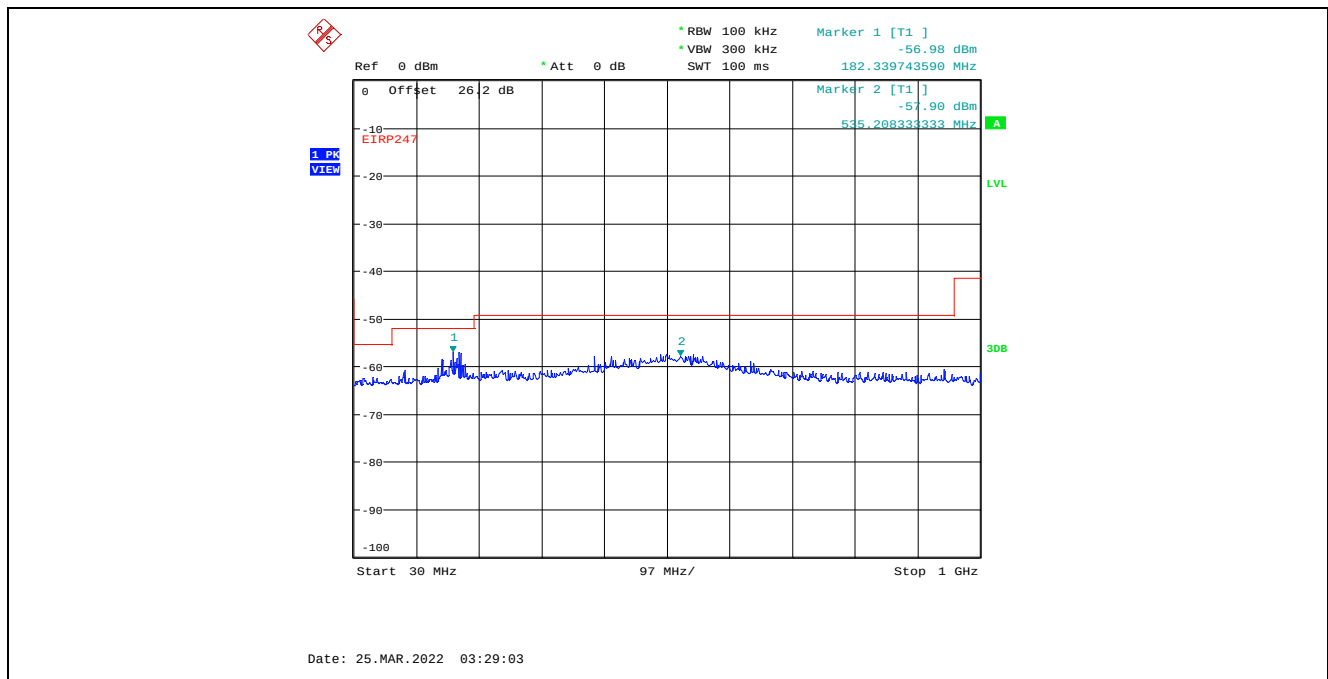
Plot C.3.6. Conducted Spurious Emissions in Restricted Frequency Bands, Chain 1 4 MHz Channel Bandwidth, Data Rate 3, Raw Power Setting 8, 2402 MHz, 30 MHz - 1 GHz, Peak Detector
