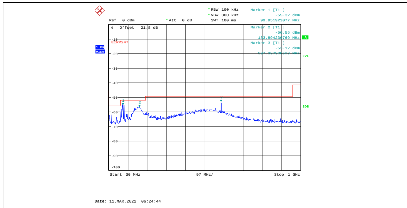
Plot C.1.115. Conducted Spurious Emissions in Restricted Frequency Bands, Chain 1 40 MHz Channel Bandwidth, Data Rate 3, Raw Power Setting 15, 2452 MHz, 30 MHz - 1 GHz, Peak Detector
