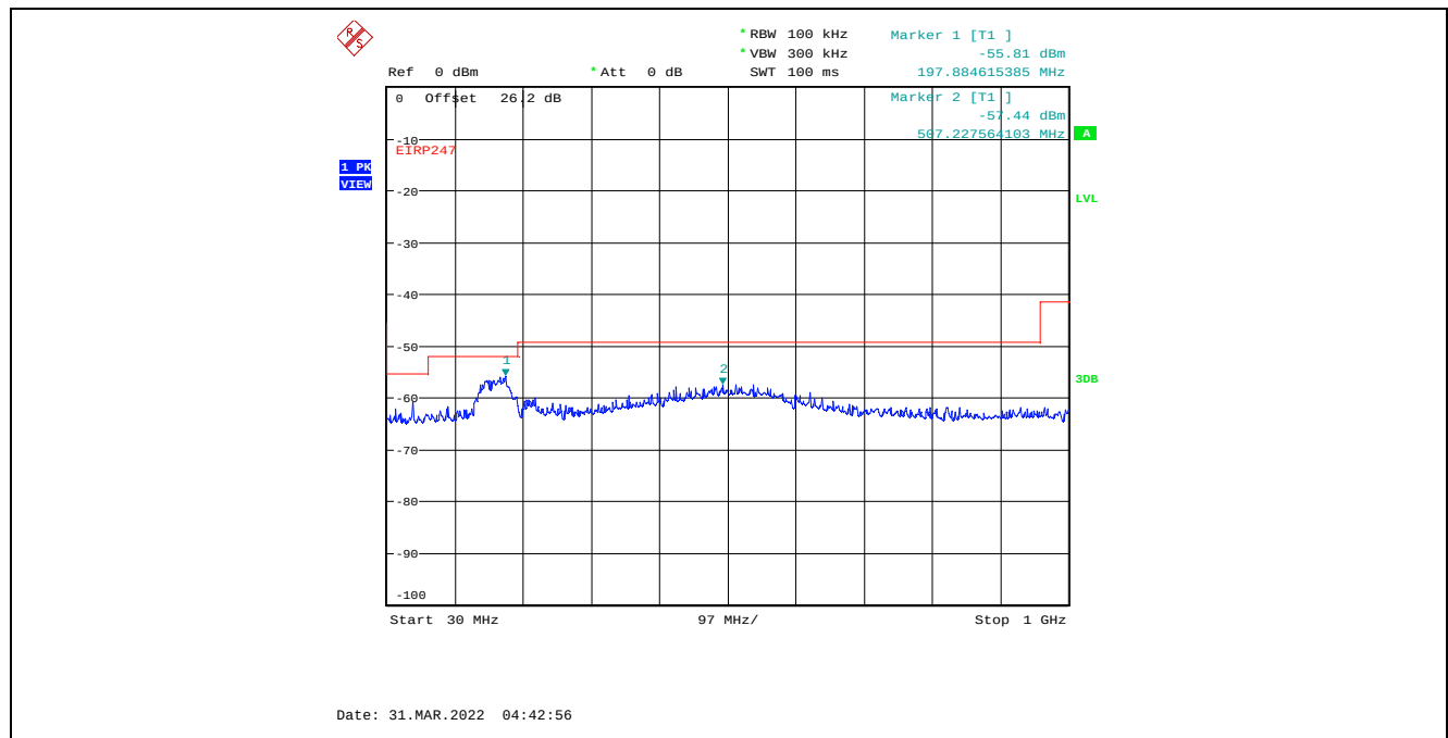
Plot C.3.116. Conducted Spurious Emissions in Restricted Frequency Bands, Chain 2 40 MHz Channel Bandwidth, Data Rate 3, Raw Power Setting 0, 2452 MHz, 30 MHz - 1 GHz, Peak Detector
