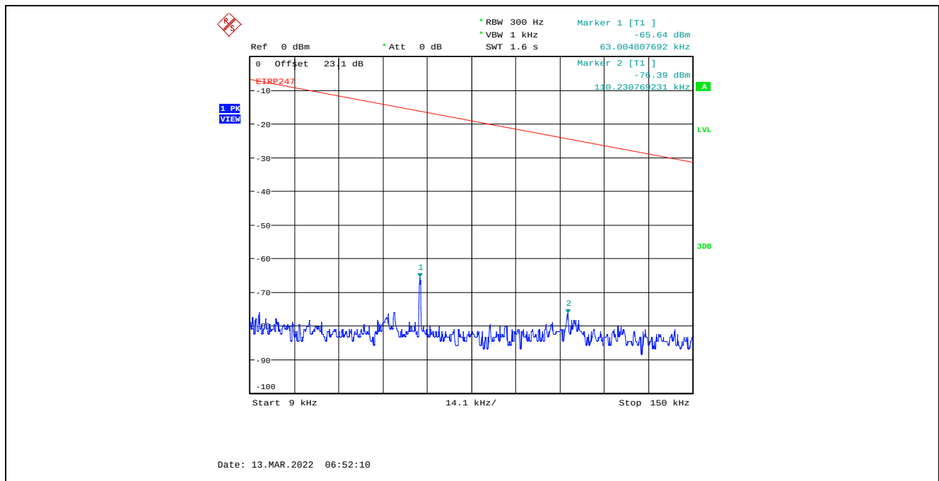
Plot C.2.81. Conducted Spurious Emissions in Restricted Frequency Bands, Chain 1 20 MHz Channel Bandwidth, Data Rate 7, Raw Power Setting 23, 2462 MHz, 9 kHz - 150 kHz, Peak Detector
