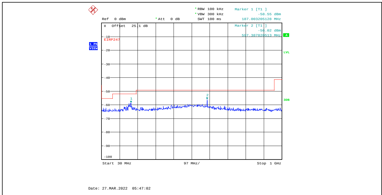
Plot C.3.55. Conducted Spurious Emissions in Restricted Frequency Bands, Chain 1 8 MHz Channel Bandwidth, Data Rate 3, Raw Power Setting 0, 2476 MHz, 30 MHz - 1 GHz, Peak Detector
