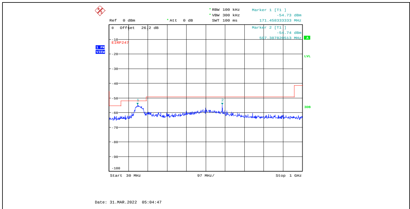
Plot C.4.95. Conducted Spurious Emissions in Restricted Frequency Bands, Chain 1 40 MHz Channel Bandwidth, Data Rate 7, Raw Power Setting 0, 2422 MHz, 30 MHz - 1 GHz, Peak Detector
