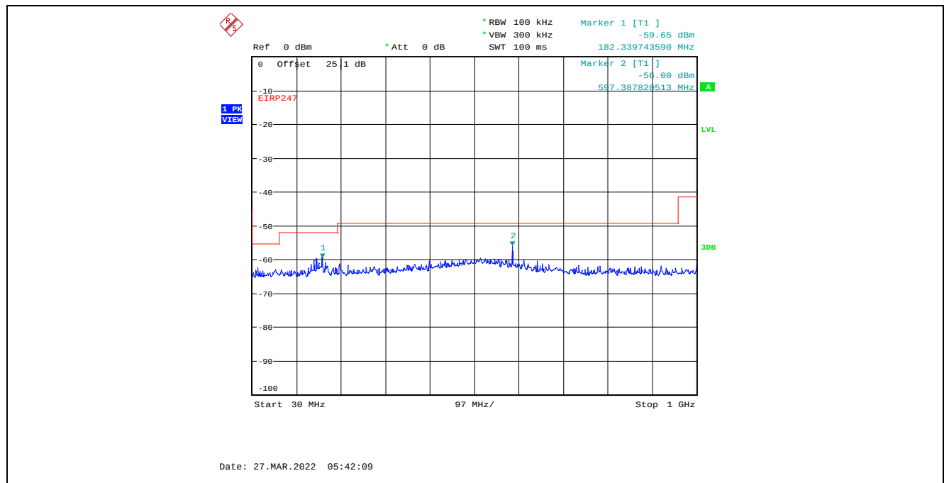
Plot C.3.35. Conducted Spurious Emissions in Restricted Frequency Bands, Chain 1 8 MHz Channel Bandwidth, Data Rate 3, Raw Power Setting 6, 2407 MHz, 30 MHz - 1 GHz, Peak Detector
