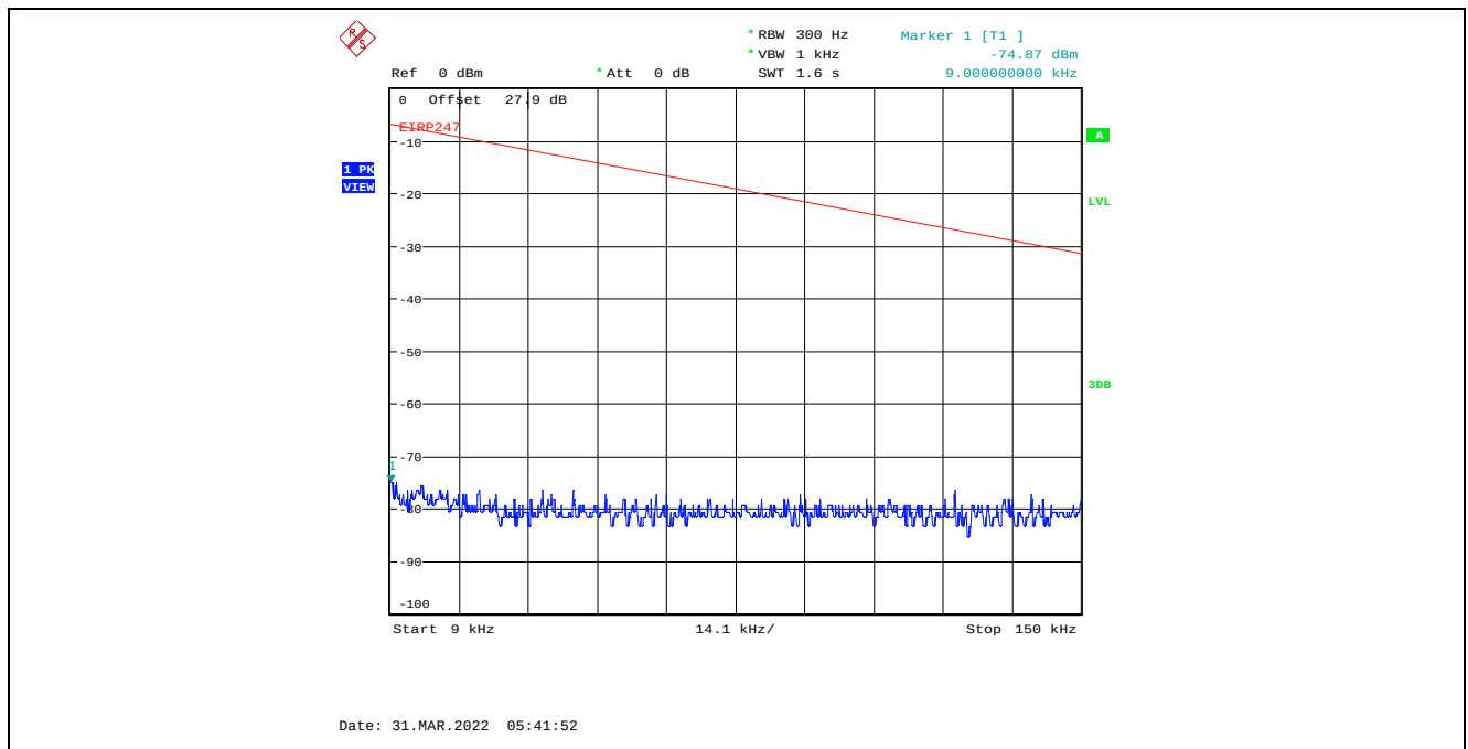
Plot C.3.112. Conducted Spurious Emissions in Restricted Frequency Bands, Chain 2 40 MHz Channel Bandwidth, Data Rate 3, Raw Power Setting 0, 2452 MHz, 9 kHz - 150 kHz, Peak Detector
