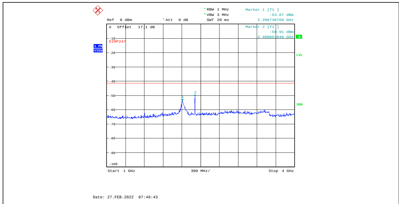
Plot C.2.37. Conducted Spurious Emissions in Restricted Frequency Bands, Chain 1 8 MHz Channel Bandwidth, Data Rate 7, Raw Power Setting 23, 2407 MHz, 1 GHz – 4 GHz, Peak Detector
