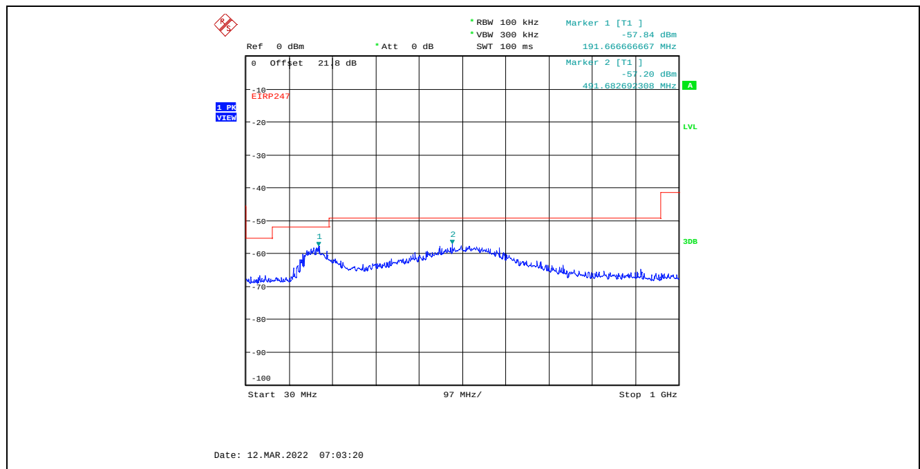
Plot C.1.66. Conducted Spurious Emissions in Restricted Frequency Bands, Chain 2 20 MHz Channel Bandwidth, Data Rate 3, Raw Power Setting 26, 2412 MHz, 30 MHz - 1 GHz, Peak Detector
