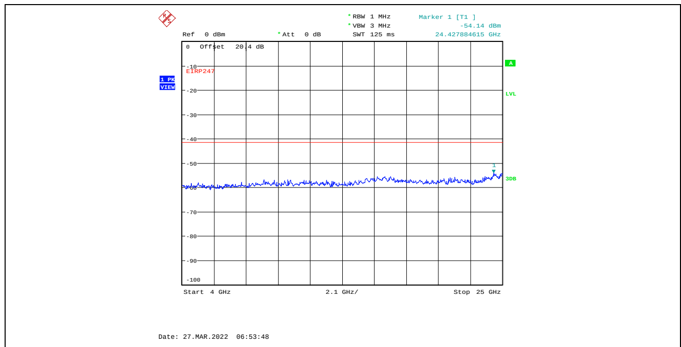
Plot C.4.50. Conducted Spurious Emissions in Restricted Frequency Bands, Chain 2 8 MHz Channel Bandwidth, Data Rate 7, Raw Power Setting 0, 2437 MHz, 4 GHz - 25 GHz, Peak Detector
