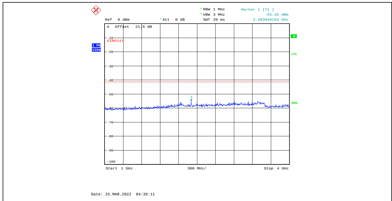
Plot C.4.7. Conducted Spurious Emissions in Restricted Frequency Bands, Chain 1 4 MHz Channel Bandwidth, Data Rate 7, Raw Power Setting 0, 2405 MHz, 1 GHz - 4 GHz, Peak Detector
