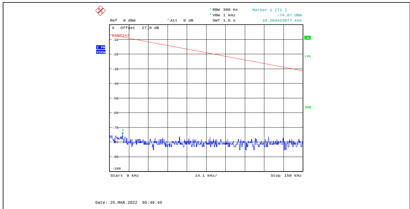
Plot C.4.12. Conducted Spurious Emissions in Restricted Frequency Bands, Chain 2 4 MHz Channel Bandwidth, Data Rate 7, Raw Power Setting 0, 2437 MHz, 9 kHz - 150 kHz, Peak Detector
