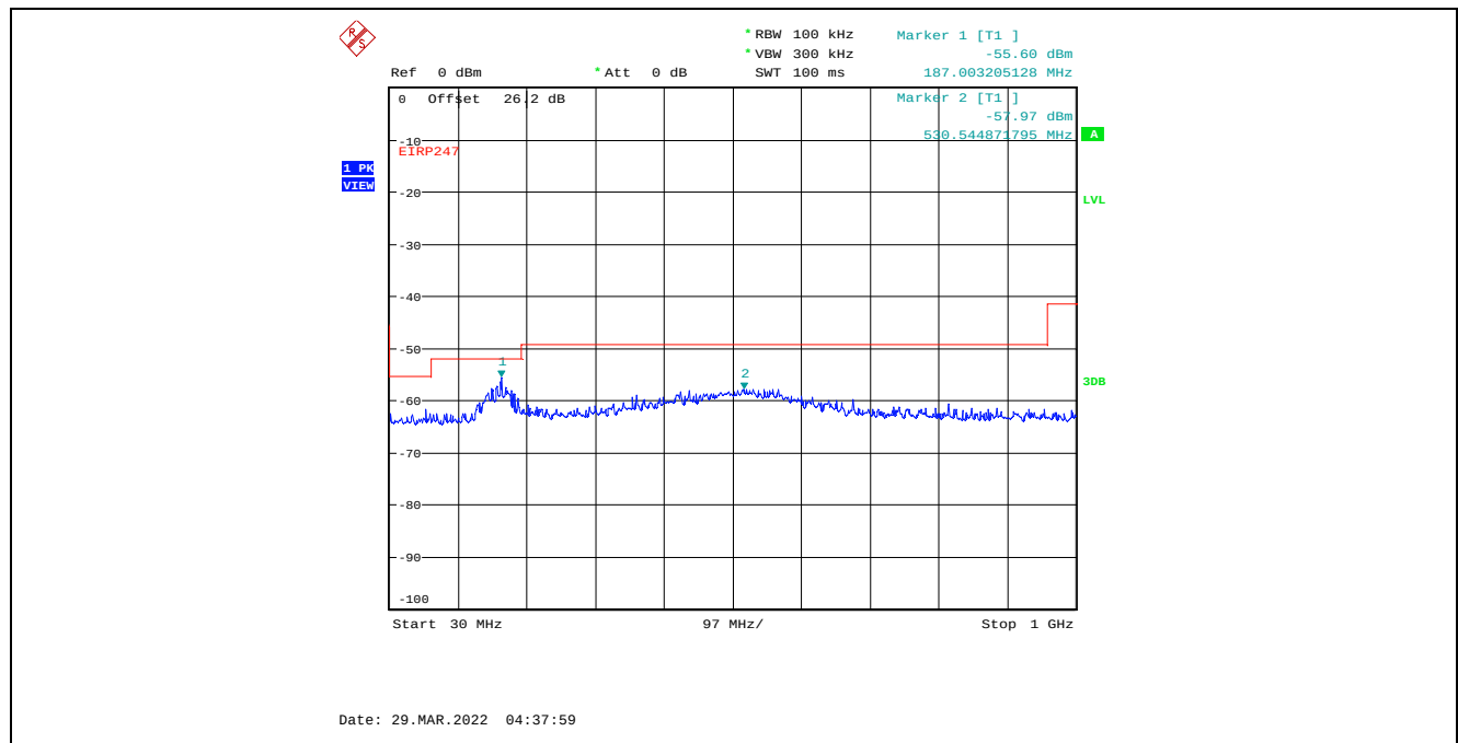
Plot C.3.76. Conducted Spurious Emissions in Restricted Frequency Bands, Chain 2 20 MHz Channel Bandwidth, Data Rate 3, Raw Power Setting 7, 2437 MHz, 30 MHz - 1 GHz, Peak Detector
