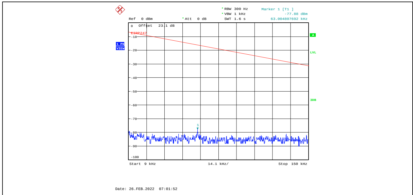
Plot C.2.1. Conducted Spurious Emissions in Restricted Frequency Bands, Chain 1 4 MHz Channel Bandwidth, Data Rate 7, Raw Power Setting 22, 2405 MHz, 9 kHz - 150 kHz, Peak Detector
