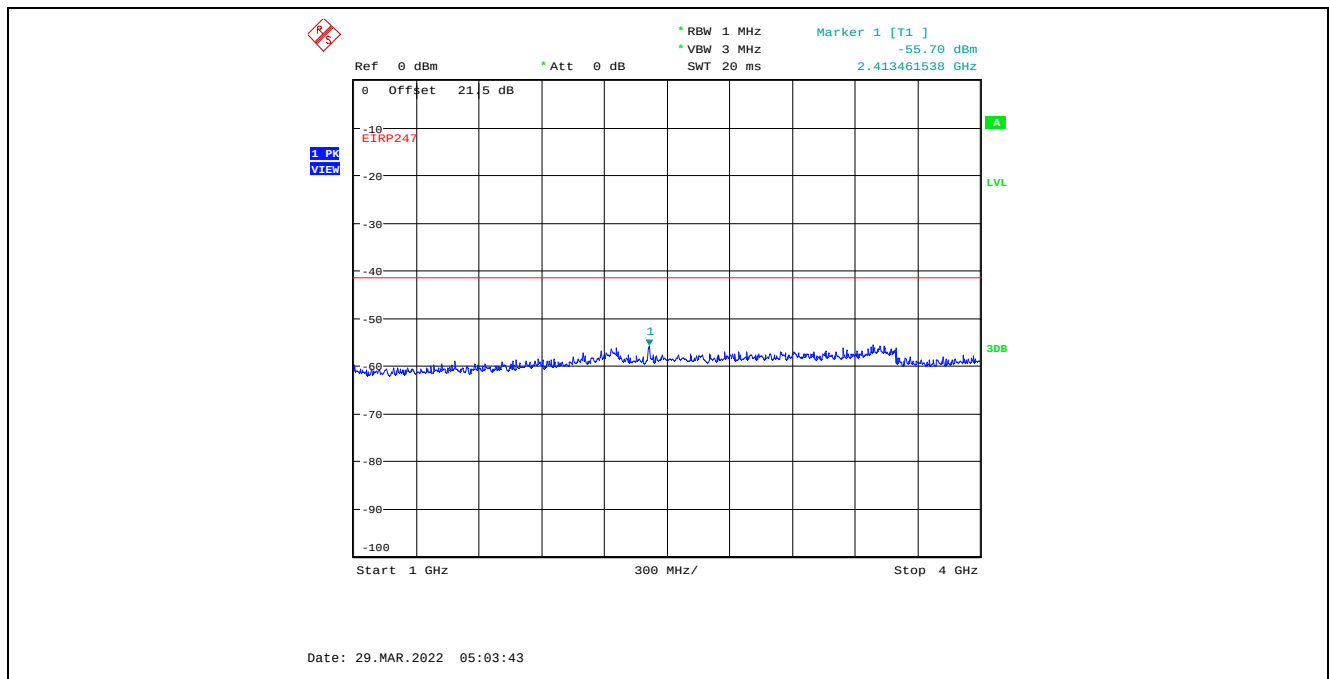
Plot C.3.68. Conducted Spurious Emissions in Restricted Frequency Bands, Chain 2 20 MHz Channel Bandwidth, Data Rate 3, Raw Power Setting 7, 2412 MHz, 1 GHz – 4 GHz, Peak Detector
