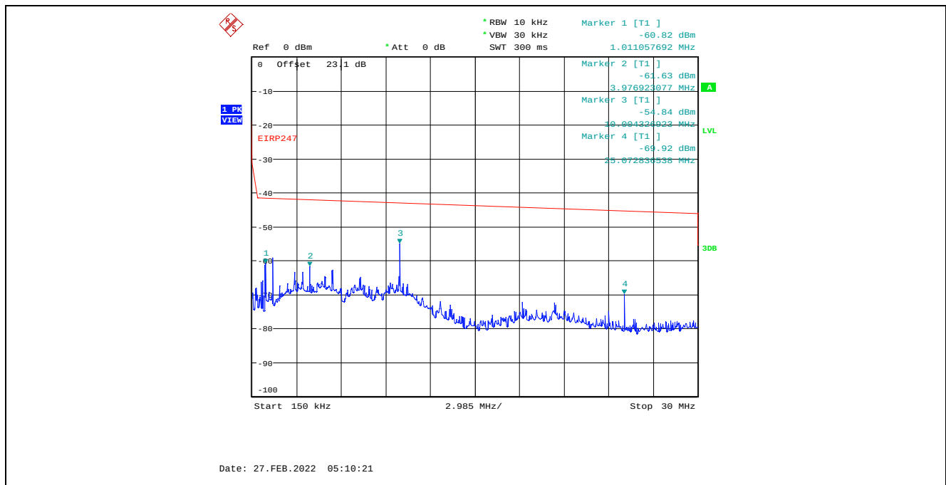
Plot C.2.33. Conducted Spurious Emissions in Restricted Frequency Bands, Chain 1 8 MHz Channel Bandwidth, Data Rate 7, Raw Power Setting 23, 2407 MHz, 150 kHz – 30 MHz, Peak Detector
