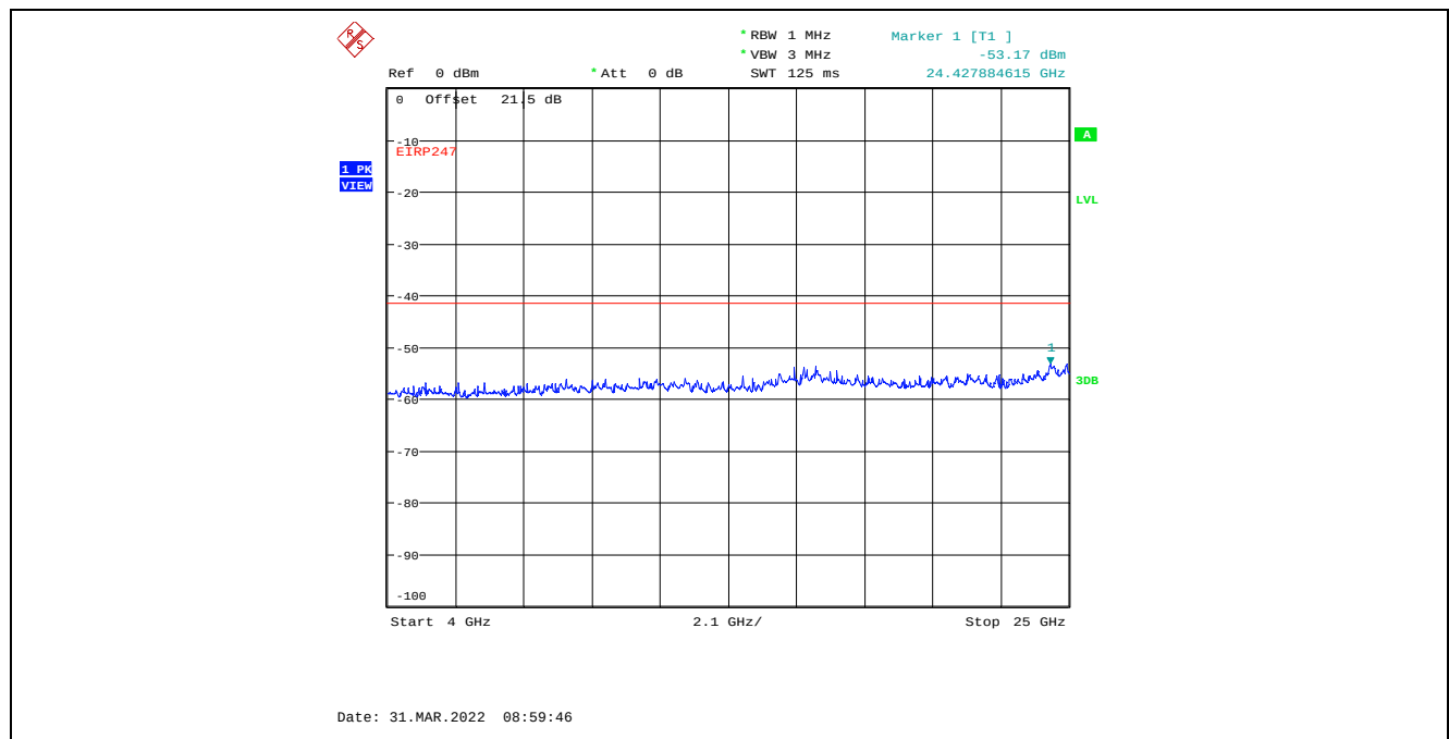
Plot C.4.100. Conducted Spurious Emissions in Restricted Frequency Bands, Chain 2 40 MHz Channel Bandwidth, Data Rate 7, Raw Power Setting 0, 2422 MHz, 4 GHz - 25 GHz, Peak Detector
