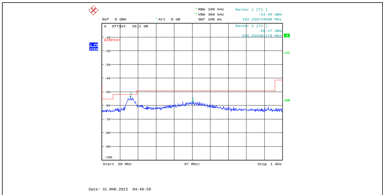
Plot C.4.116. Conducted Spurious Emissions in Restricted Frequency Bands, Chain 2 40 MHz Channel Bandwidth, Data Rate 7, Raw Power Setting 0, 2452 MHz, 30 MHz - 1 GHz, Peak Detector
