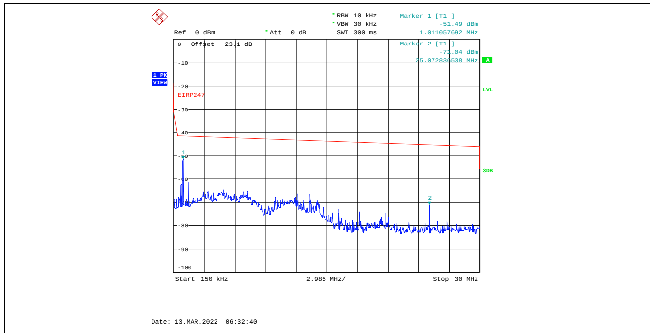
Plot C.2.73. Conducted Spurious Emissions in Restricted Frequency Bands, Chain 1 20 MHz Channel Bandwidth, Data Rate 7, Raw Power Setting 23, 2437 MHz, 150 kHz – 30 MHz, Peak Detector
