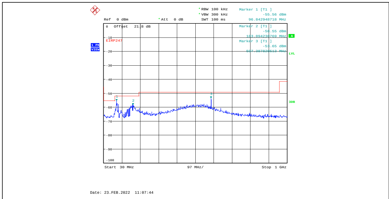
Plot C.1.15. Conducted Spurious Emissions in Restricted Frequency Bands, Chain 1 4 MHz Channel Bandwidth, Data Rate 3, Raw Power Setting 16, 2437 MHz, 30 MHz - 1 GHz, Peak Detector
