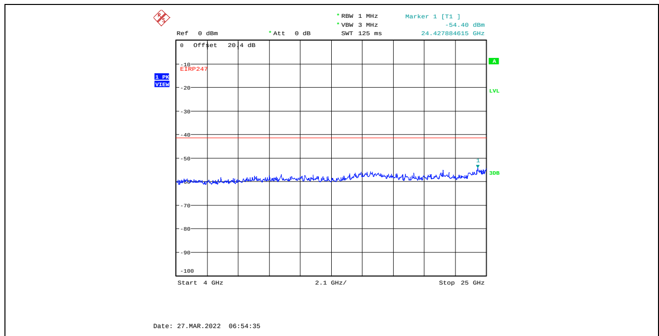
Plot C.4.40. Conducted Spurious Emissions in Restricted Frequency Bands, Chain 2 8 MHz Channel Bandwidth, Data Rate 7, Raw Power Setting 0, 2407 MHz, 4 GHz - 25 GHz, Peak Detector
