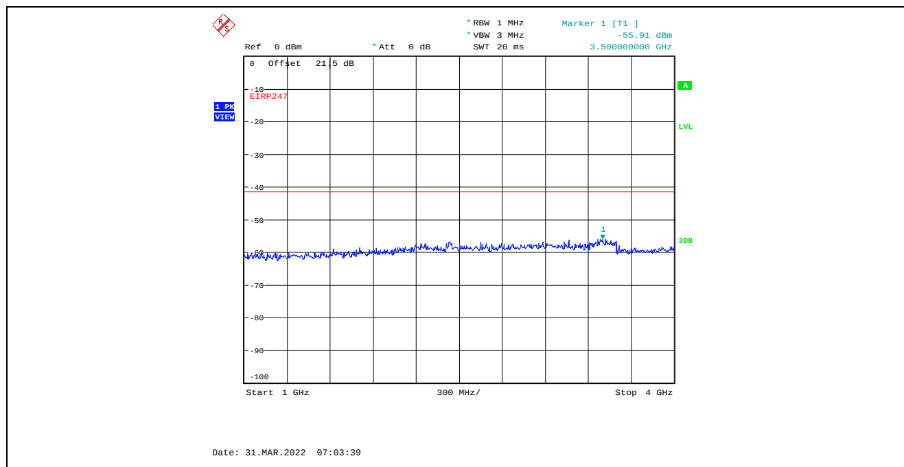
Plot C.3.97. Conducted Spurious Emissions in Restricted Frequency Bands, Chain 1 40 MHz Channel Bandwidth, Data Rate 3, Raw Power Setting 0, 2422 MHz, 1 GHz – 4 GHz, Peak Detector
