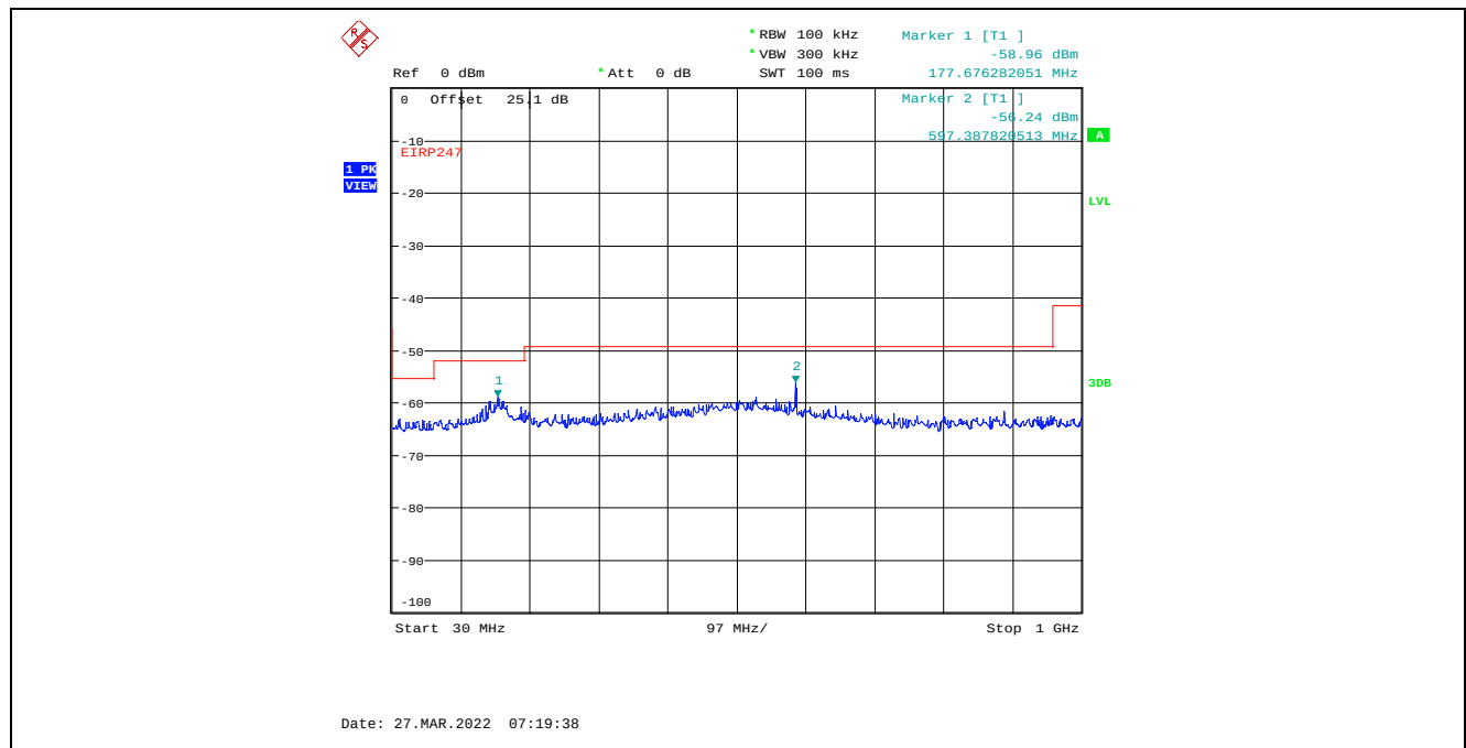
Plot C.4.45. Conducted Spurious Emissions in Restricted Frequency Bands, Chain 1 8 MHz Channel Bandwidth, Data Rate 7, Raw Power Setting 0, 2437 MHz, 30 MHz - 1 GHz, Peak Detector
