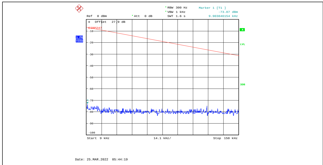
Plot C.4.11. Conducted Spurious Emissions in Restricted Frequency Bands, Chain 1 4 MHz Channel Bandwidth, Data Rate 7, Raw Power Setting 0, 2437 MHz, 9 kHz - 150 kHz, Peak Detector
