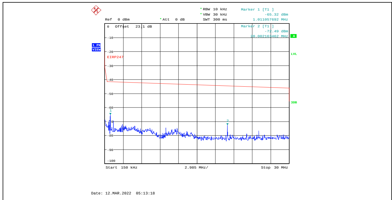
Plot C.2.113. Conducted Spurious Emissions in Restricted Frequency Bands, Chain 1 40 MHz Channel Bandwidth, Data Rate 7, Raw Power Setting 22, 2452 MHz, 150 kHz – 30 MHz, Peak Detector
