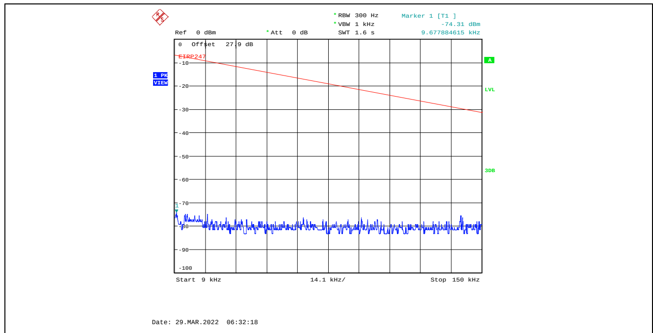
Plot C.4.71. Conducted Spurious Emissions in Restricted Frequency Bands, Chain 1 20 MHz Channel Bandwidth, Data Rate 7, Raw Power Setting 0, 2437 MHz, 9 kHz - 150 kHz, Peak Detector
