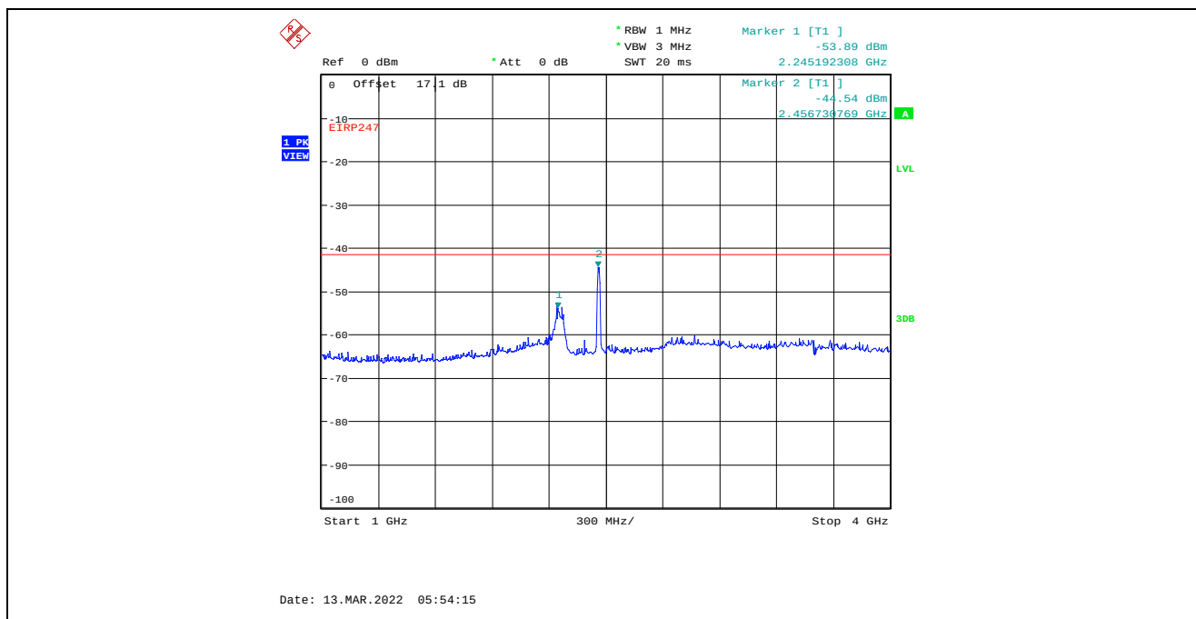
Plot C.2.88. Conducted Spurious Emissions in Restricted Frequency Bands, Chain 2 20 MHz Channel Bandwidth, Data Rate 7, Raw Power Setting 23, 2462 MHz, 1 GHz – 4 GHz, Peak Detector
