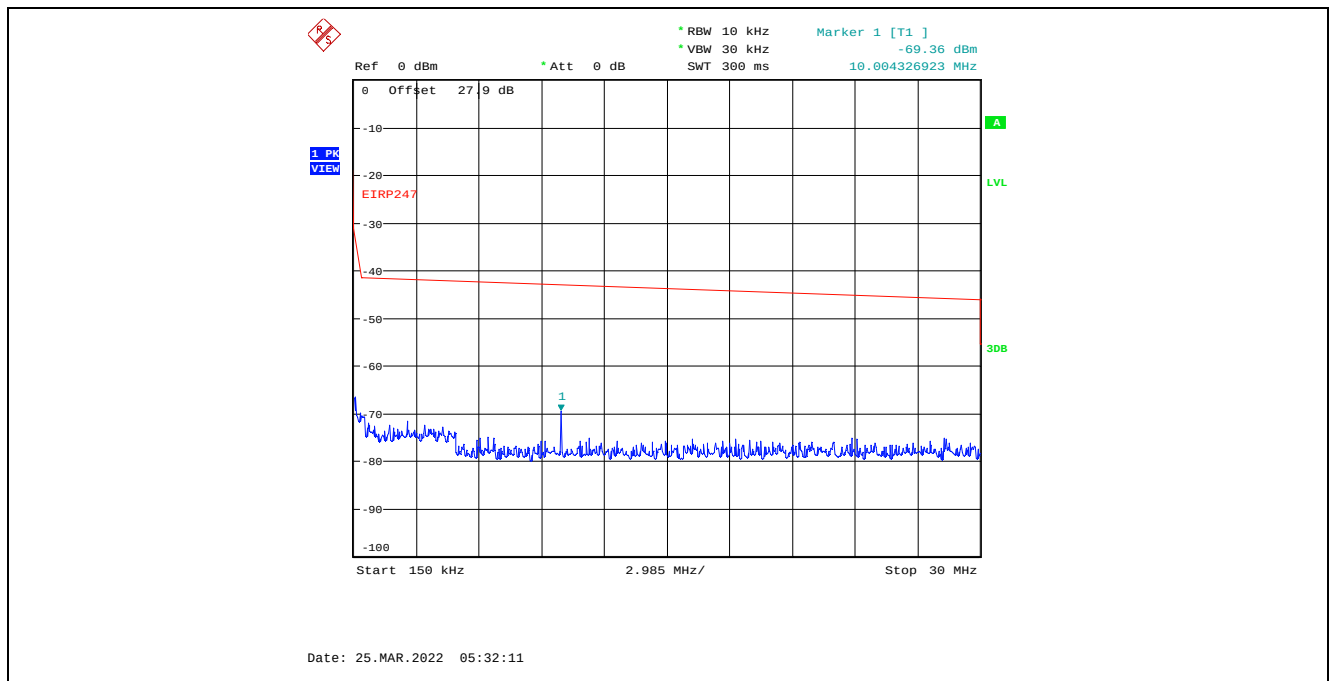
Plot C.4.13. Conducted Spurious Emissions in Restricted Frequency Bands, Chain 1 4 MHz Channel Bandwidth, Data Rate 7, Raw Power Setting 0, 2437 MHz, 150 kHz – 30 MHz, Peak Detector
