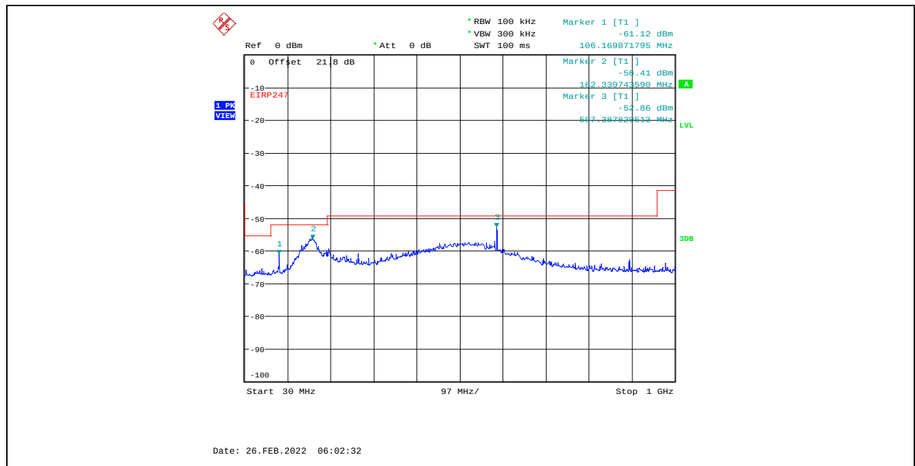
Plot C.2.5. Conducted Spurious Emissions in Restricted Frequency Bands, Chain 1 4 MHz Channel Bandwidth, Data Rate 7, Raw Power Setting 22, 2405 MHz, 30 MHz - 1 GHz, Peak Detector
