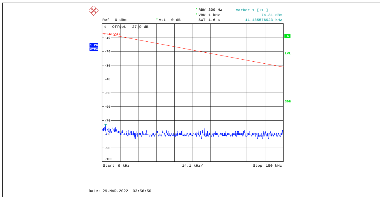
Plot C.3.81. Conducted Spurious Emissions in Restricted Frequency Bands, Chain 1 20 MHz Channel Bandwidth, Data Rate 3, Raw Power Setting 7, 2462 MHz, 9 kHz - 150 kHz, Peak Detector
