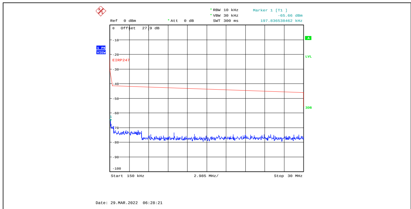
Plot C.4.64. Conducted Spurious Emissions in Restricted Frequency Bands, Chain 2 20 MHz Channel Bandwidth, Data Rate 7, Raw Power Setting 0, 2412 MHz, 150 kHz – 30 MHz, Peak Detector
