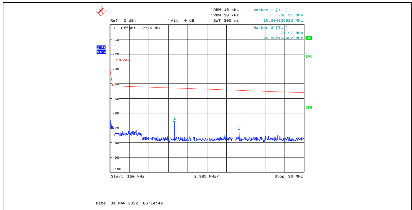
Plot C.4.103. Conducted Spurious Emissions in Restricted Frequency Bands, Chain 1 40 MHz Channel Bandwidth, Data Rate 7, Raw Power Setting 0, 2437 MHz, 150 kHz – 30 MHz, Peak Detector
