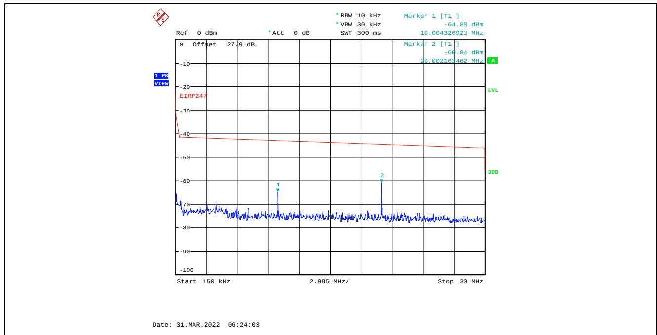
Plot C.3.104. Conducted Spurious Emissions in Restricted Frequency Bands, Chain 2 40 MHz Channel Bandwidth, Data Rate 3, Raw Power Setting 0, 2437 MHz, 150 kHz – 30 MHz, Peak Detector
