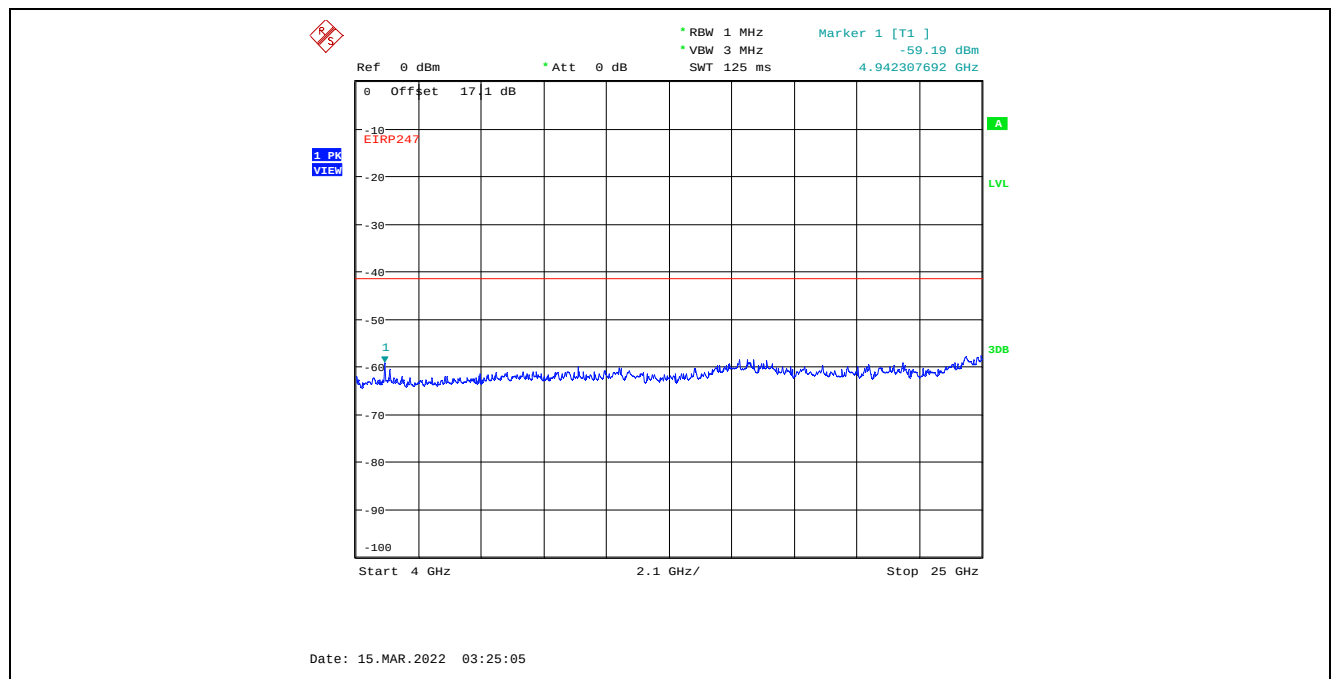
Plot C.2.30. Conducted Spurious Emissions in Restricted Frequency Bands, Chain 2 4 MHz Channel Bandwidth, Data Rate 7, Raw Power Setting 20, 2477 MHz, 4 GHz - 25 GHz, Peak Detector
