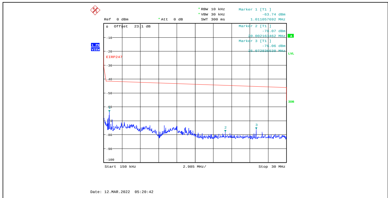
Plot C.2.94. Conducted Spurious Emissions in Restricted Frequency Bands, Chain 2 40 MHz Channel Bandwidth, Data Rate 7, Raw Power Setting 20, 2422 MHz, 150 kHz – 30 MHz, Peak Detector
