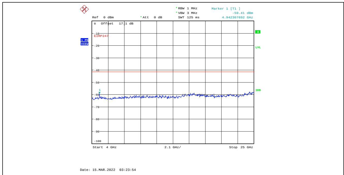
Plot C.1.30. Conducted Spurious Emissions in Restricted Frequency Bands, Chain 2 4 MHz Channel Bandwidth, Data Rate 3, Raw Power Setting 13, 2477 MHz, 4 GHz - 25 GHz, Peak Detector
