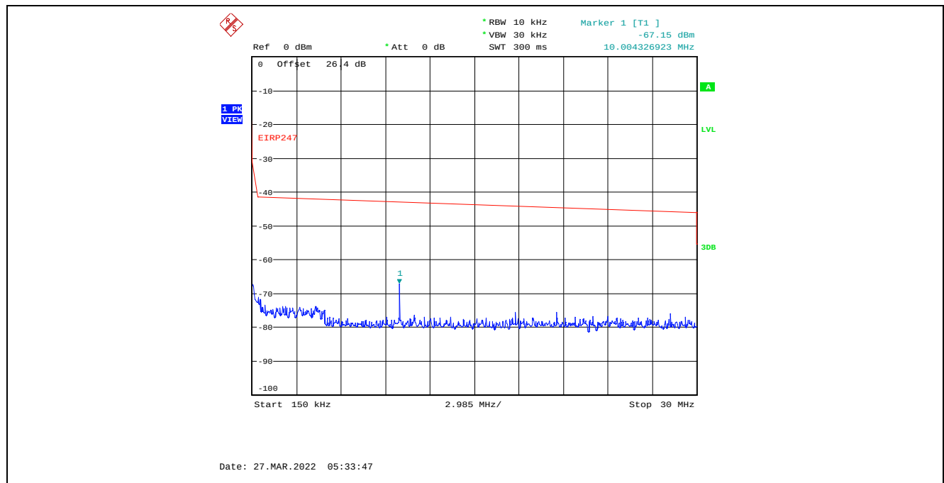
Plot C.3.53. Conducted Spurious Emissions in Restricted Frequency Bands, Chain 1 8 MHz Channel Bandwidth, Data Rate 3, Raw Power Setting 0, 2476 MHz, 150 kHz – 30 MHz, Peak Detector
