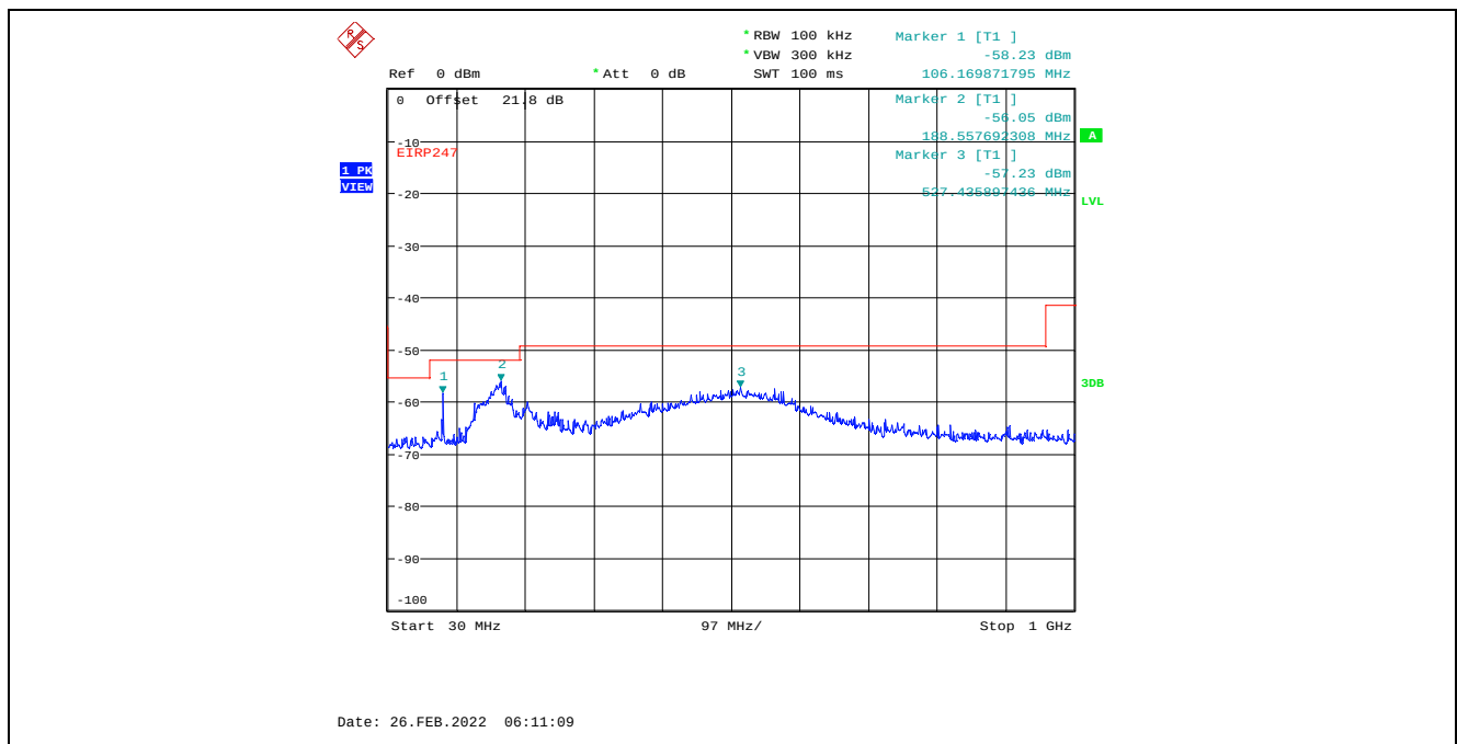
Plot C.2.16. Conducted Spurious Emissions in Restricted Frequency Bands, Chain 2 4 MHz Channel Bandwidth, Data Rate 7, Raw Power Setting 22, 2437 MHz, 30 MHz - 1 GHz, Peak Detector
