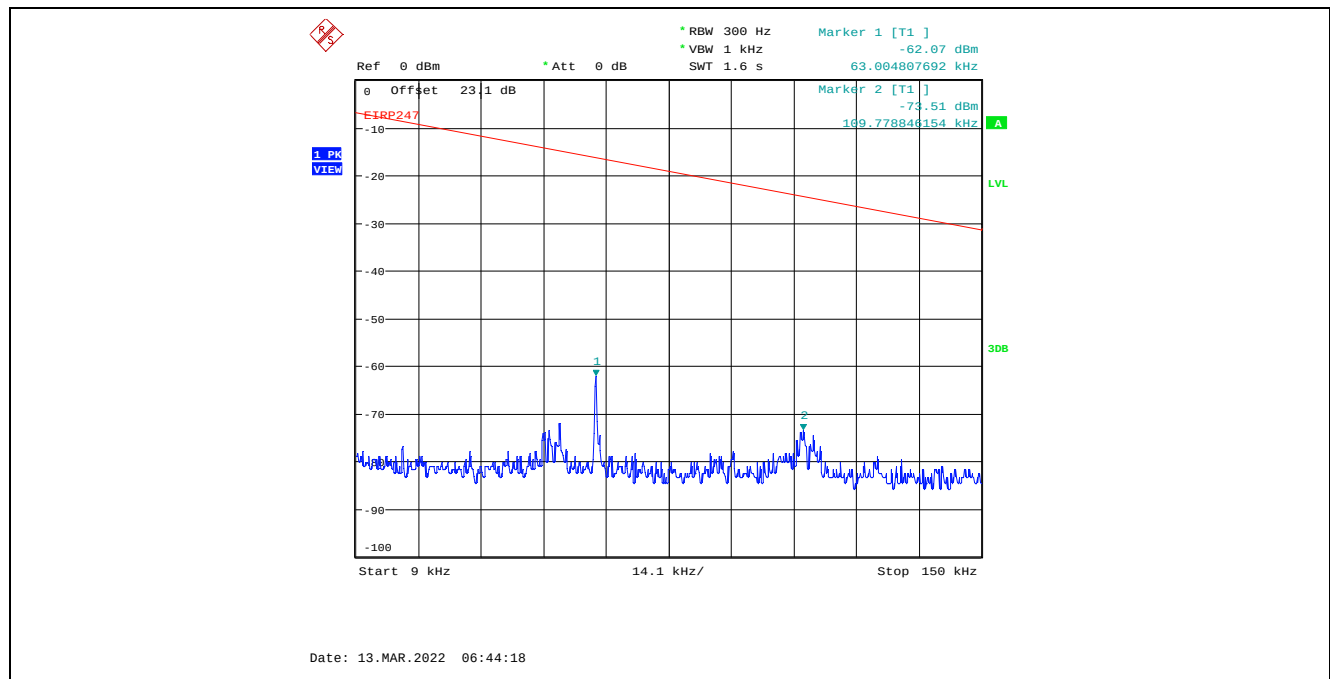
Plot C.2.62. Conducted Spurious Emissions in Restricted Frequency Bands, Chain 2 20 MHz Channel Bandwidth, Data Rate 7, Raw Power Setting 23, 2412 MHz, 9 kHz - 150 kHz, Peak Detector
