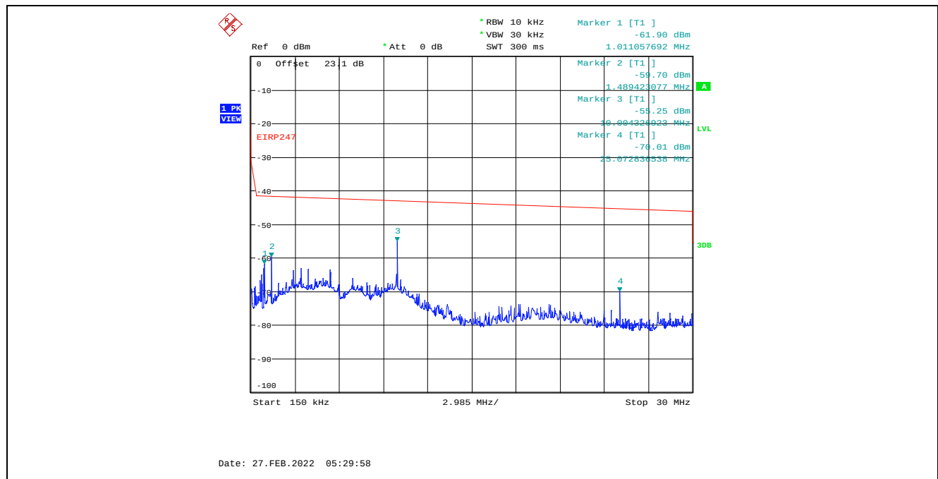
Plot C.1.33. Conducted Spurious Emissions in Restricted Frequency Bands, Chain 1 8 MHz Channel Bandwidth, Data Rate 3, Raw Power Setting 21, 2407 MHz, 150 kHz – 30 MHz, Peak Detector
