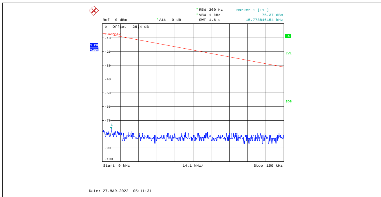
Plot C.3.32. Conducted Spurious Emissions in Restricted Frequency Bands, Chain 2 8 MHz Channel Bandwidth, Data Rate 3, Raw Power Setting 6, 2407 MHz, 9 kHz - 150 kHz, Peak Detector
