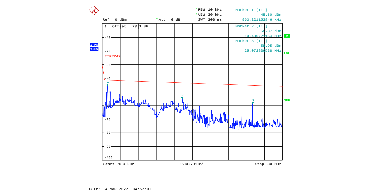
Plot C.2.53. Conducted Spurious Emissions in Restricted Frequency Bands, Chain 1 8 MHz Channel Bandwidth, Data Rate 7, Raw Power Setting 12, 2476 MHz, 150 kHz – 30 MHz, Peak Detector
