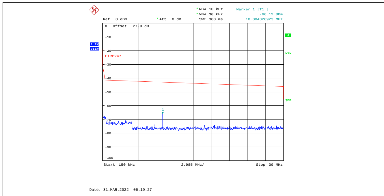
Plot C.4.93. Conducted Spurious Emissions in Restricted Frequency Bands, Chain 1 40 MHz Channel Bandwidth, Data Rate 7, Raw Power Setting 0, 2422 MHz, 150 kHz – 30 MHz, Peak Detector
