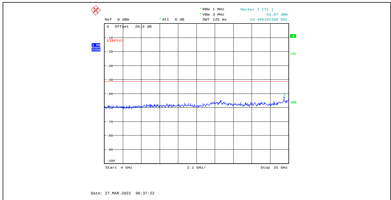
Plot C.3.49. Conducted Spurious Emissions in Restricted Frequency Bands, Chain 1 8 MHz Channel Bandwidth, Data Rate 3, Raw Power Setting 6, 2437 MHz, 4 GHz - 25 GHz, Peak Detector
