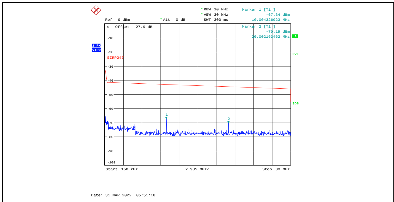
Plot C.3.93. Conducted Spurious Emissions in Restricted Frequency Bands, Chain 1 40 MHz Channel Bandwidth, Data Rate 3, Raw Power Setting 0, 2422 MHz, 150 kHz – 30 MHz, Peak Detector
