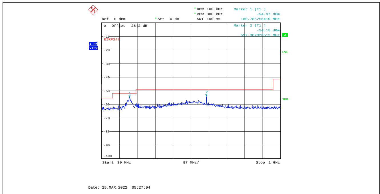
Plot C.4.5. Conducted Spurious Emissions in Restricted Frequency Bands, Chain 1 4 MHz Channel Bandwidth, Data Rate 7, Raw Power Setting 0, 2405 MHz, 30 MHz - 1 GHz, Peak Detector
