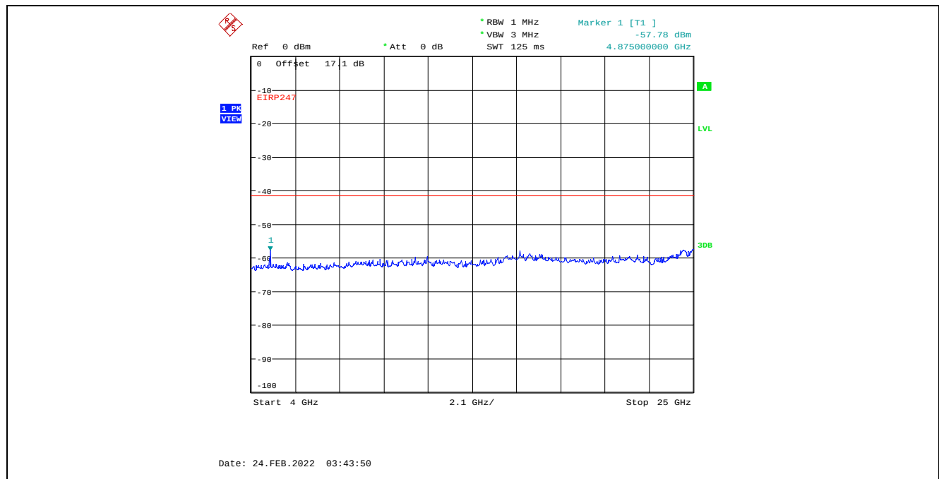
Plot C.1.19. Conducted Spurious Emissions in Restricted Frequency Bands, Chain 1 4 MHz Channel Bandwidth, Data Rate 3, Raw Power Setting 16, 2437 MHz, 4 GHz - 25 GHz, Peak Detector
