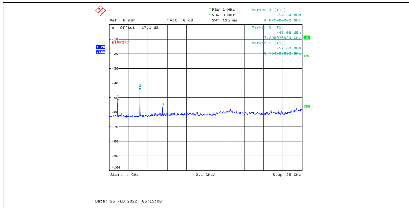
Plot C.2.19. Conducted Spurious Emissions in Restricted Frequency Bands, Chain 1 4 MHz Channel Bandwidth, Data Rate 7, Raw Power Setting 22, 2437 MHz, 4 GHz - 25 GHz, Peak Detector
