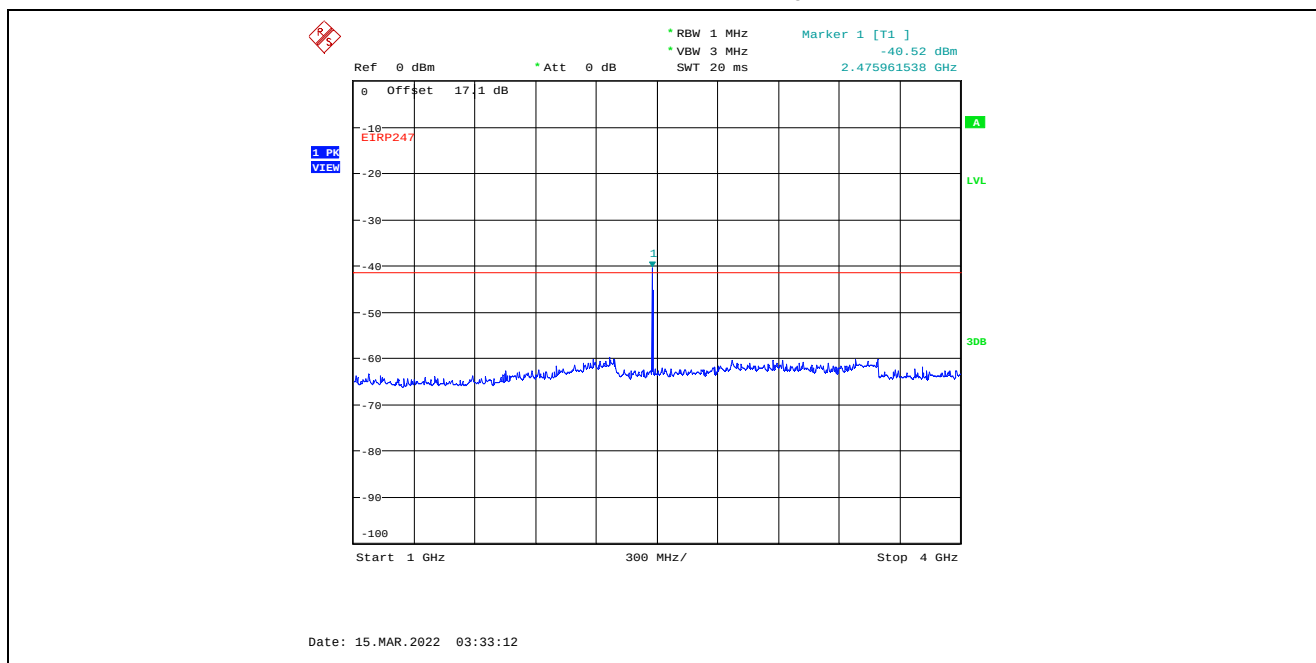
Plot C.2.27. Conducted Spurious Emissions in Restricted Frequency Bands, Chain 1 4 MHz Channel Bandwidth, Data Rate 7, Raw Power Setting 20, 2477 MHz, 1 GHz – 4 GHz, Peak Detector Marker 1 is Fundamental Signal
