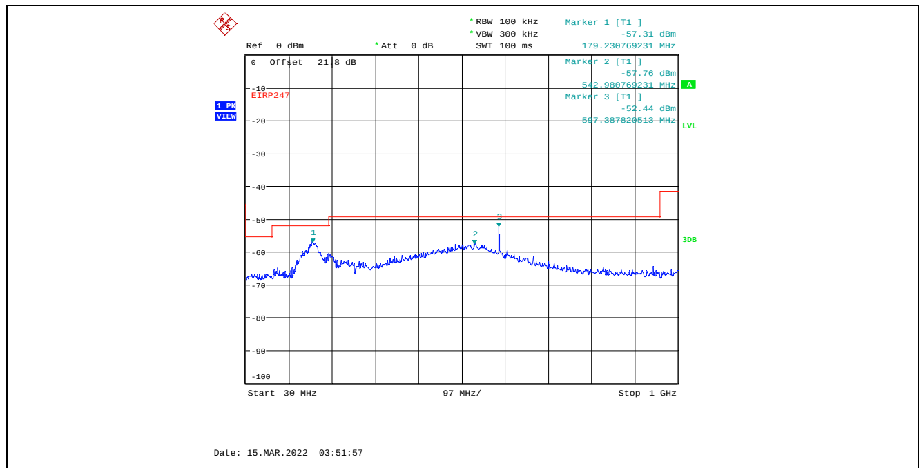
Plot C.2.25. Conducted Spurious Emissions in Restricted Frequency Bands, Chain 1 4 MHz Channel Bandwidth, Data Rate 7, Raw Power Setting 20, 2477 MHz, 30 MHz - 1 GHz, Peak Detector
