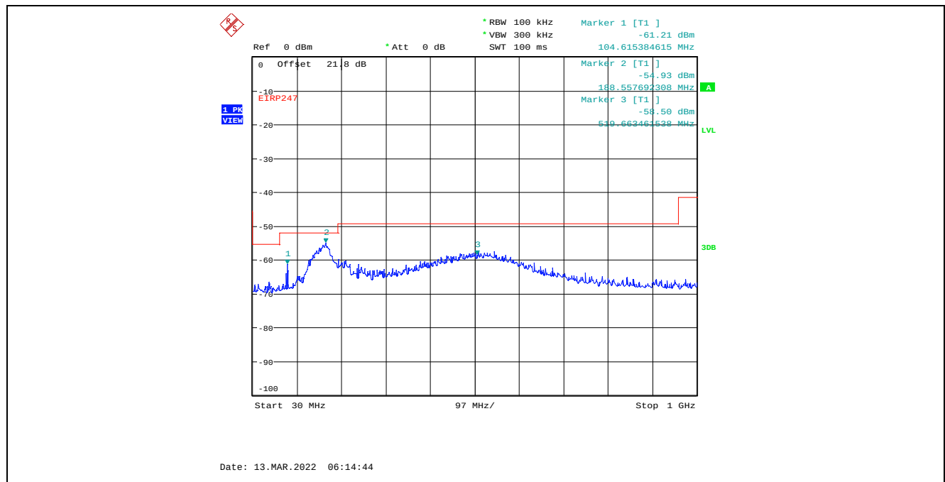
Plot C.2.76. Conducted Spurious Emissions in Restricted Frequency Bands, Chain 2 20 MHz Channel Bandwidth, Data Rate 7, Raw Power Setting 23, 2437 MHz, 30 MHz - 1 GHz, Peak Detector
