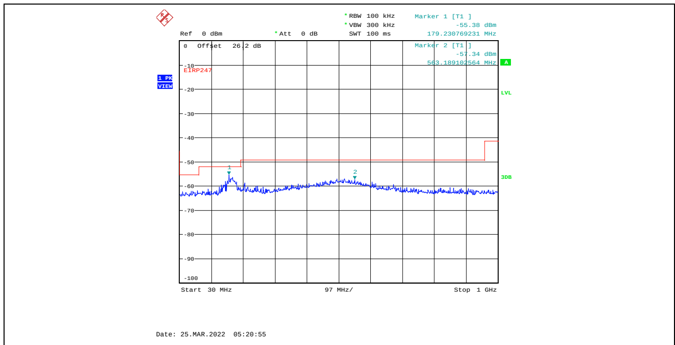
Plot C.4.26. Conducted Spurious Emissions in Restricted Frequency Bands, Chain 2 4 MHz Channel Bandwidth, Data Rate 7, Raw Power Setting 0, 2477 MHz, 30 MHz - 1 GHz, Peak Detector
