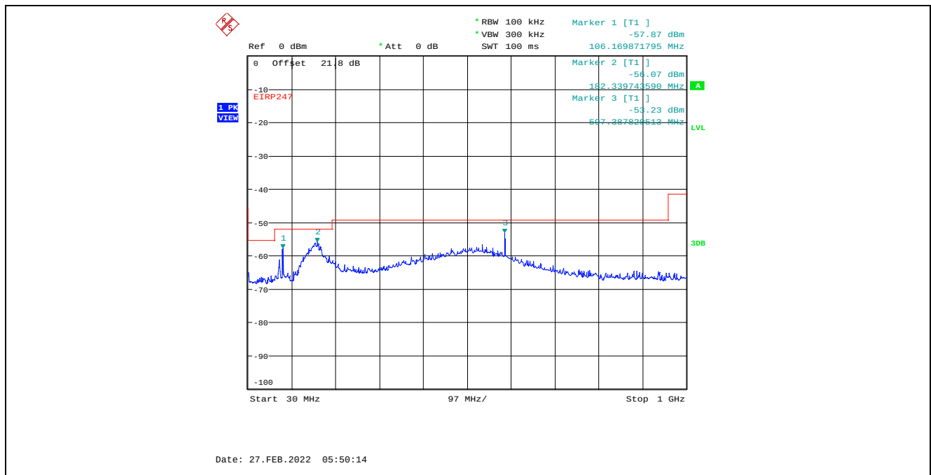
Plot C.1.35. Conducted Spurious Emissions in Restricted Frequency Bands, Chain 1 8 MHz Channel Bandwidth, Data Rate 3, Raw Power Setting 21, 2407 MHz, 30 MHz - 1 GHz, Peak Detector
