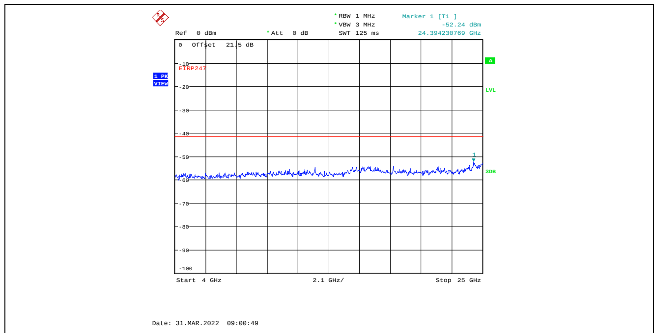
Plot C.4.110. Conducted Spurious Emissions in Restricted Frequency Bands, Chain 2 40 MHz Channel Bandwidth, Data Rate 7, Raw Power Setting 0, 2437 MHz, 4 GHz - 25 GHz, Peak Detector
