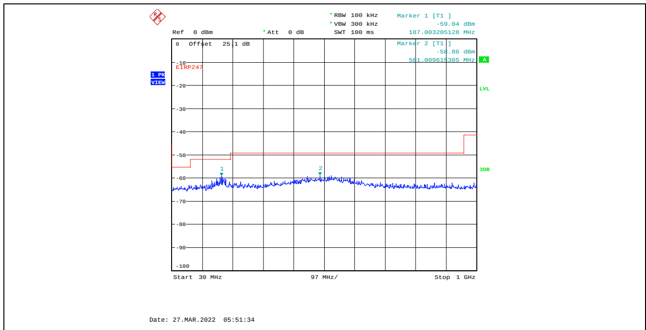
Plot C.3.46. Conducted Spurious Emissions in Restricted Frequency Bands, Chain 2 8 MHz Channel Bandwidth, Data Rate 3, Raw Power Setting 6, 2437 MHz, 30 MHz - 1 GHz, Peak Detector
