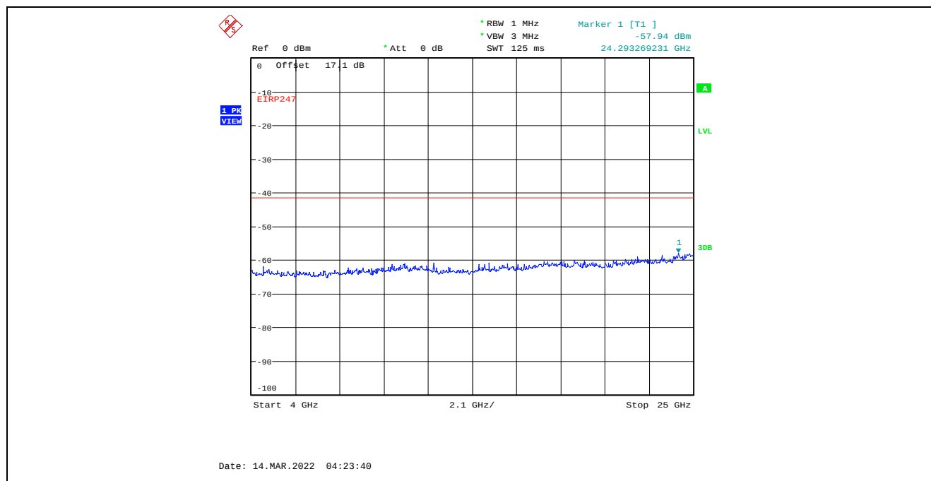
Plot C.2.60. Conducted Spurious Emissions in Restricted Frequency Bands, Chain 2 8 MHz Channel Bandwidth, Data Rate 7, Raw Power Setting 12, 2476 MHz, 4 GHz - 25 GHz, Peak Detector
