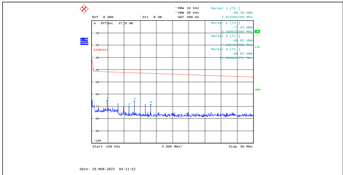
Plot C.3.83. Conducted Spurious Emissions in Restricted Frequency Bands, Chain 1 20 MHz Channel Bandwidth, Data Rate 3, Raw Power Setting 7, 2462 MHz, 150 kHz – 30 MHz, Peak Detector
