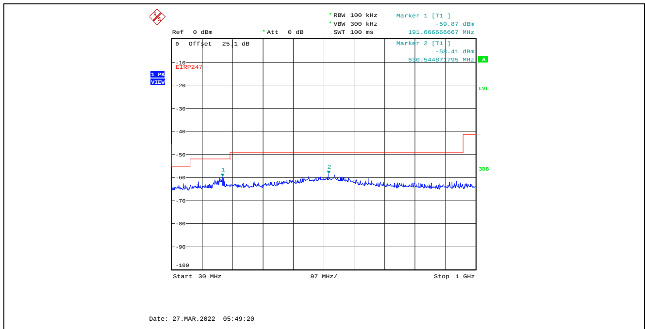
Plot C.3.56. Conducted Spurious Emissions in Restricted Frequency Bands, Chain 2 8 MHz Channel Bandwidth, Data Rate 3, Raw Power Setting 0, 2476 MHz, 30 MHz - 1 GHz, Peak Detector
