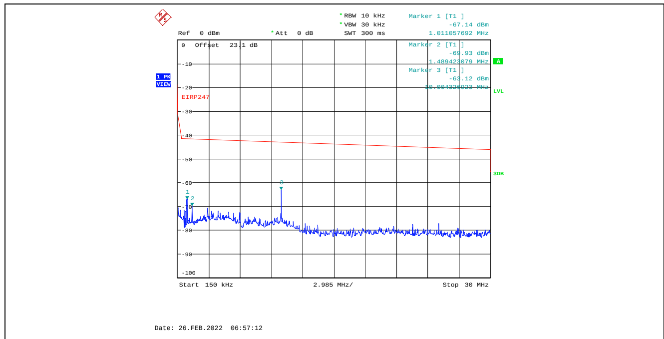
Plot C.2.13. Conducted Spurious Emissions in Restricted Frequency Bands, Chain 1 4 MHz Channel Bandwidth, Data Rate 7, Raw Power Setting 22, 2437 MHz, 150 kHz – 30 MHz, Peak Detector
