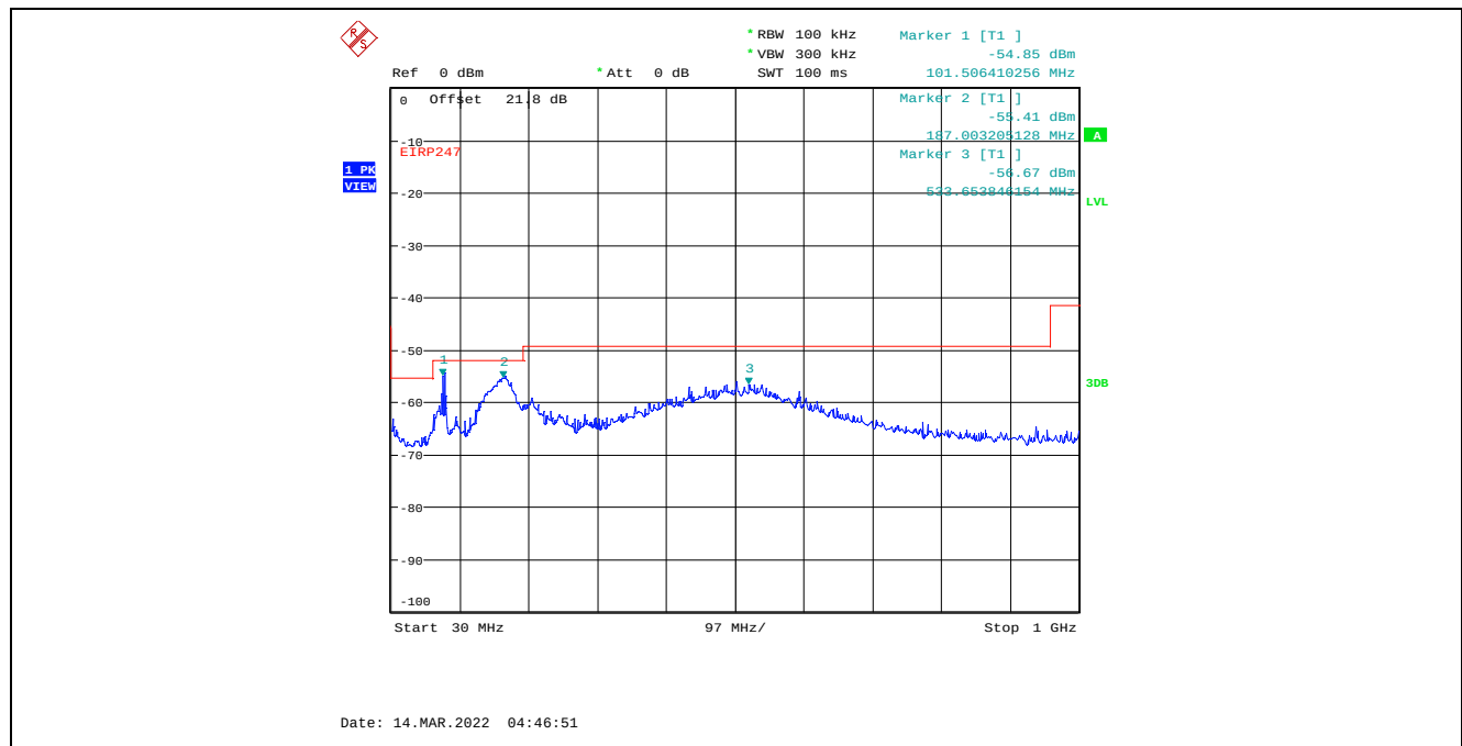
Plot C.2.56. Conducted Spurious Emissions in Restricted Frequency Bands, Chain 2 8 MHz Channel Bandwidth, Data Rate 7, Raw Power Setting 12, 2476 MHz, 30 MHz - 1 GHz, Peak Detector
