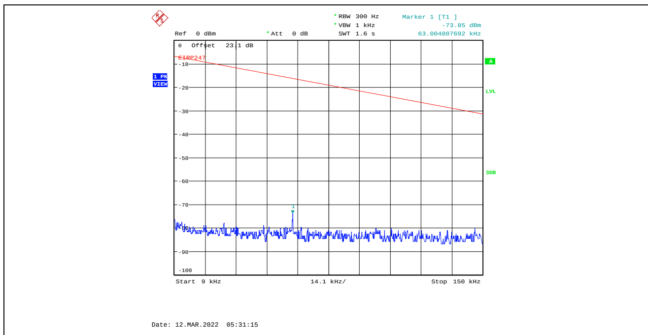
Plot C.2.101. Conducted Spurious Emissions in Restricted Frequency Bands, Chain 1 40 MHz Channel Bandwidth, Data Rate 7, Raw Power Setting 24, 2437 MHz, 9 kHz - 150 kHz, Peak Detector
