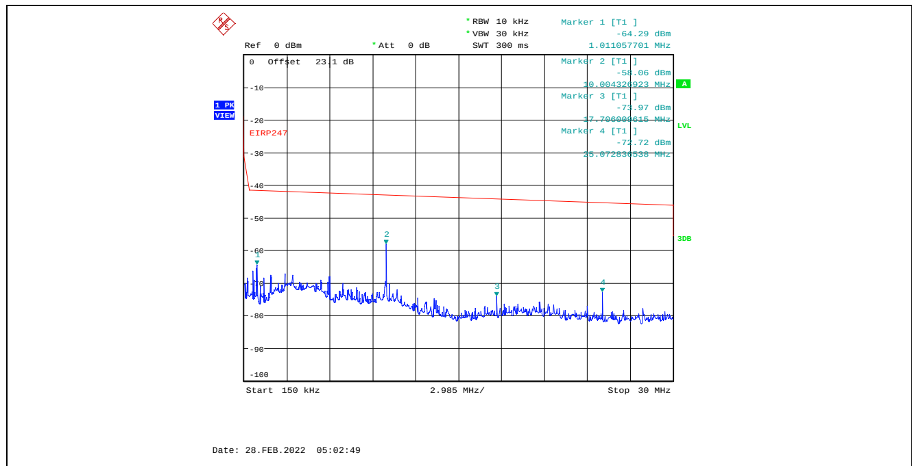
Plot C.2.43. Conducted Spurious Emissions in Restricted Frequency Bands, Chain 1 8 MHz Channel Bandwidth, Data Rate 7, Raw Power Setting 23, 2437 MHz, 150 kHz – 30 MHz, Peak Detector
