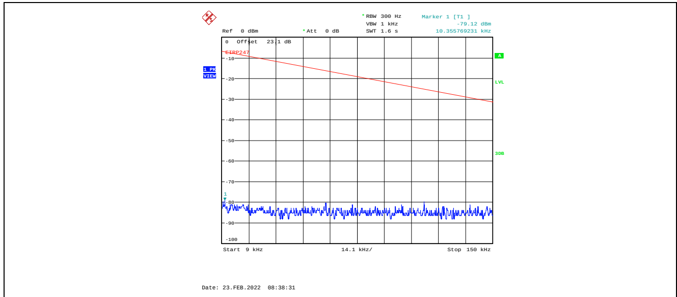
Plot C.1.1. Conducted Spurious Emissions in Restricted Frequency Bands, Chain 1 4 MHz Channel Bandwidth, Data Rate 3, Raw Power Setting 16, 2402 MHz, 9 kHz - 150 kHz, Peak Detector
