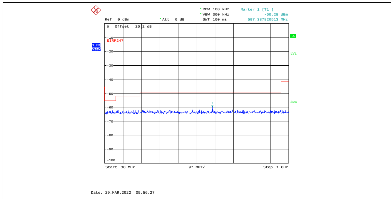
Plot C.4.65. Conducted Spurious Emissions in Restricted Frequency Bands, Chain 1 20 MHz Channel Bandwidth, Data Rate 7, Raw Power Setting 0, 2412 MHz, 30 MHz - 1 GHz, Peak Detector
