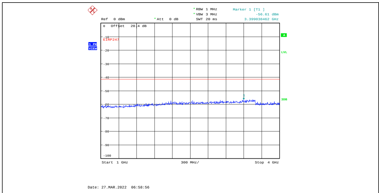
Plot C.4.38. Conducted Spurious Emissions in Restricted Frequency Bands, Chain 2 8 MHz Channel Bandwidth, Data Rate 7, Raw Power Setting 0, 2407 MHz, 1 GHz – 4 GHz, Peak Detector
