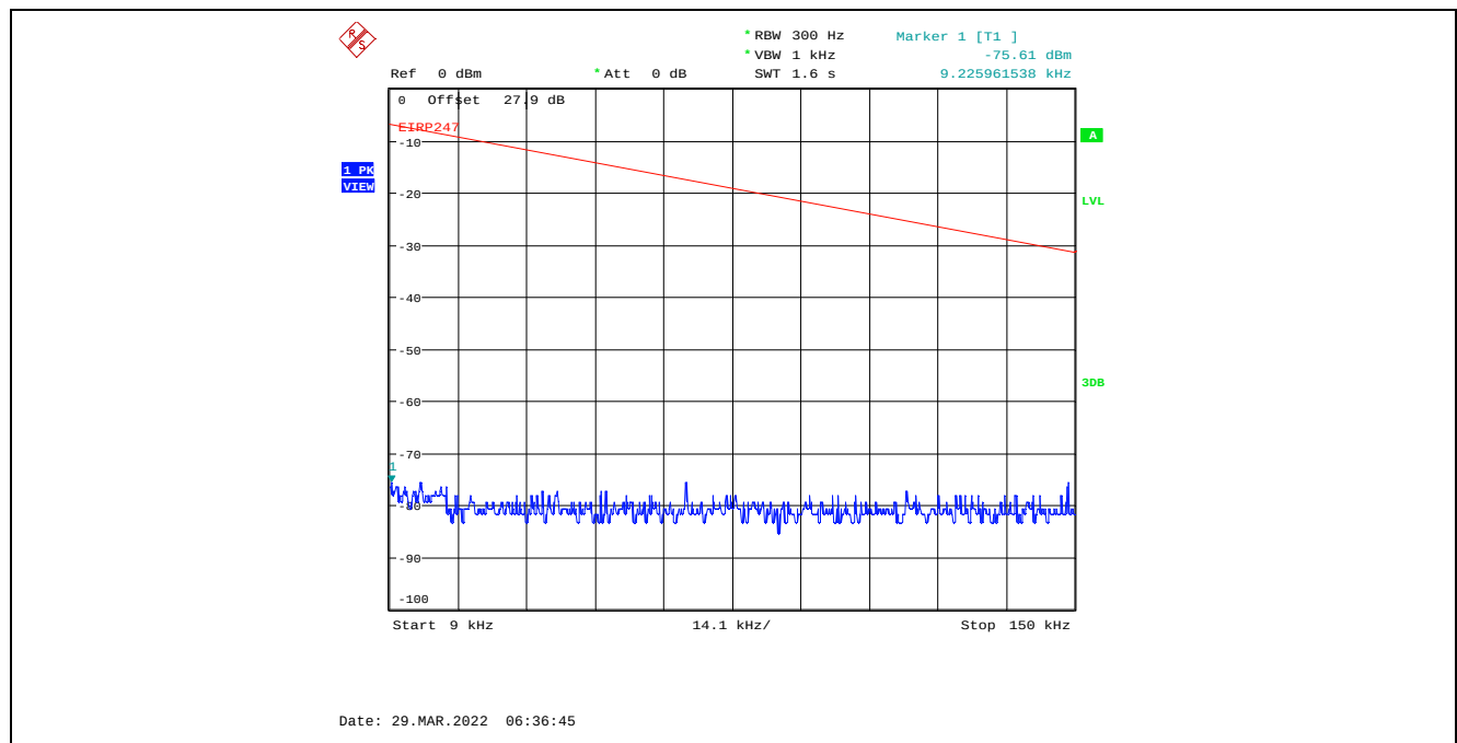
Plot C.4.72. Conducted Spurious Emissions in Restricted Frequency Bands, Chain 2 20 MHz Channel Bandwidth, Data Rate 7, Raw Power Setting 0, 2437 MHz, 9 kHz - 150 kHz, Peak Detector
