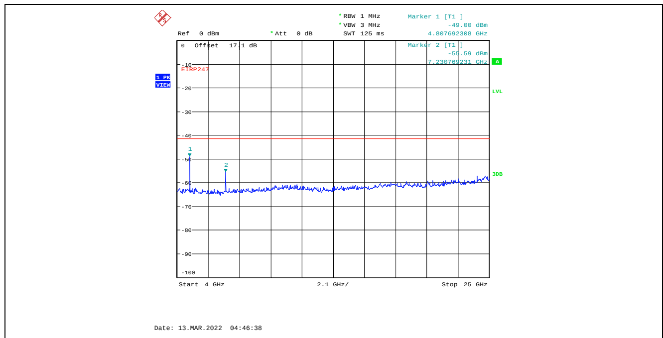
Plot C.1.70. Conducted Spurious Emissions in Restricted Frequency Bands, Chain 2 20 MHz Channel Bandwidth, Data Rate 3, Raw Power Setting 26, 2412 MHz, 4 GHz - 25 GHz, Peak Detector
