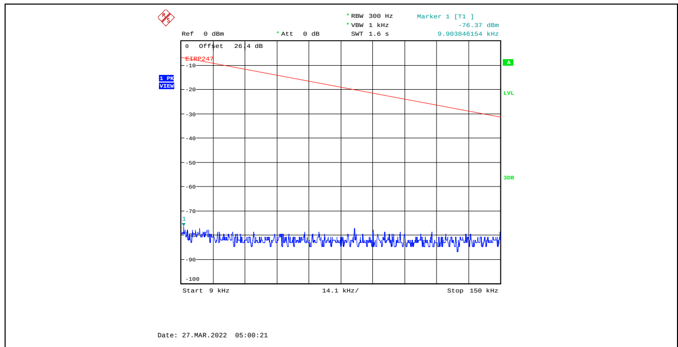
Plot C.3.51. Conducted Spurious Emissions in Restricted Frequency Bands, Chain 1 8 MHz Channel Bandwidth, Data Rate 3, Raw Power Setting 0, 2476 MHz, 9 kHz - 150 kHz, Peak Detector
