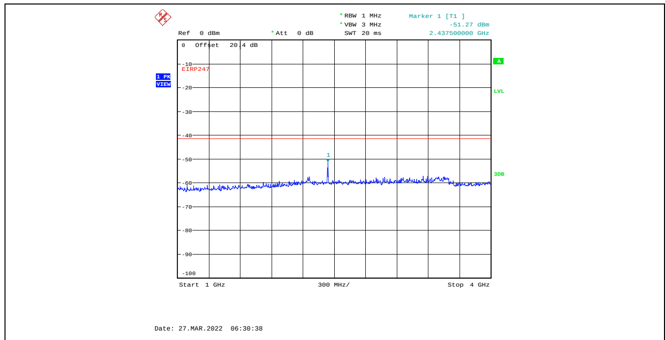
Plot C.3.47. Conducted Spurious Emissions in Restricted Frequency Bands, Chain 1 8 MHz Channel Bandwidth, Data Rate 3, Raw Power Setting 6, 2437 MHz, 1 GHz – 4 GHz, Peak Detector
