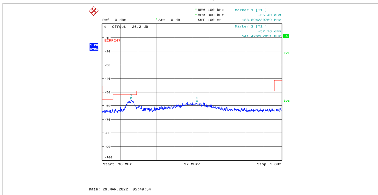
Plot C.4.86. Conducted Spurious Emissions in Restricted Frequency Bands, Chain 2 20 MHz Channel Bandwidth, Data Rate 7, Raw Power Setting 0, 2462 MHz, 30 MHz - 1 GHz, Peak Detector
