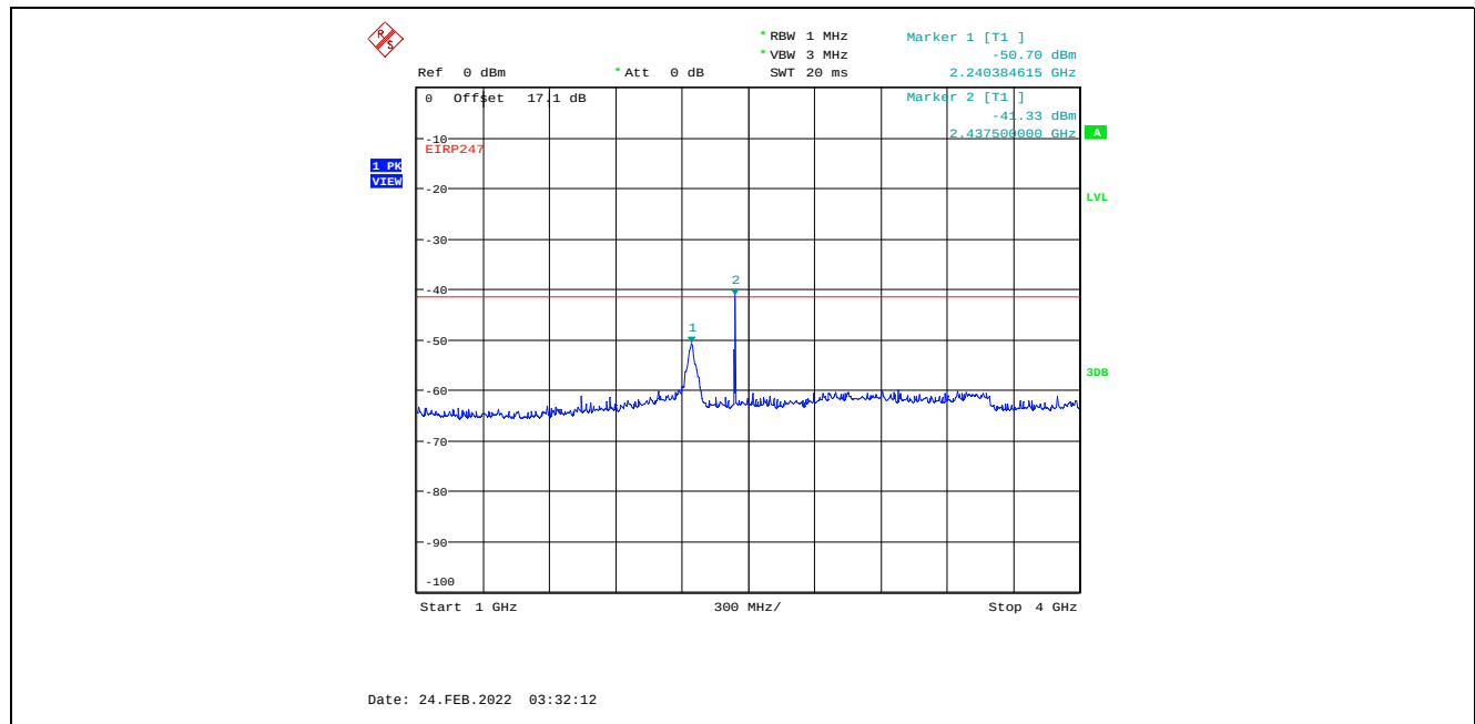
Plot C.1.17. Conducted Spurious Emissions in Restricted Frequency Bands, Chain 1 4 MHz Channel Bandwidth, Data Rate 3, Raw Power Setting 16, 2437 MHz, 1 GHz – 4 GHz, Peak Detector Marker 2 is Fundamental Signal
