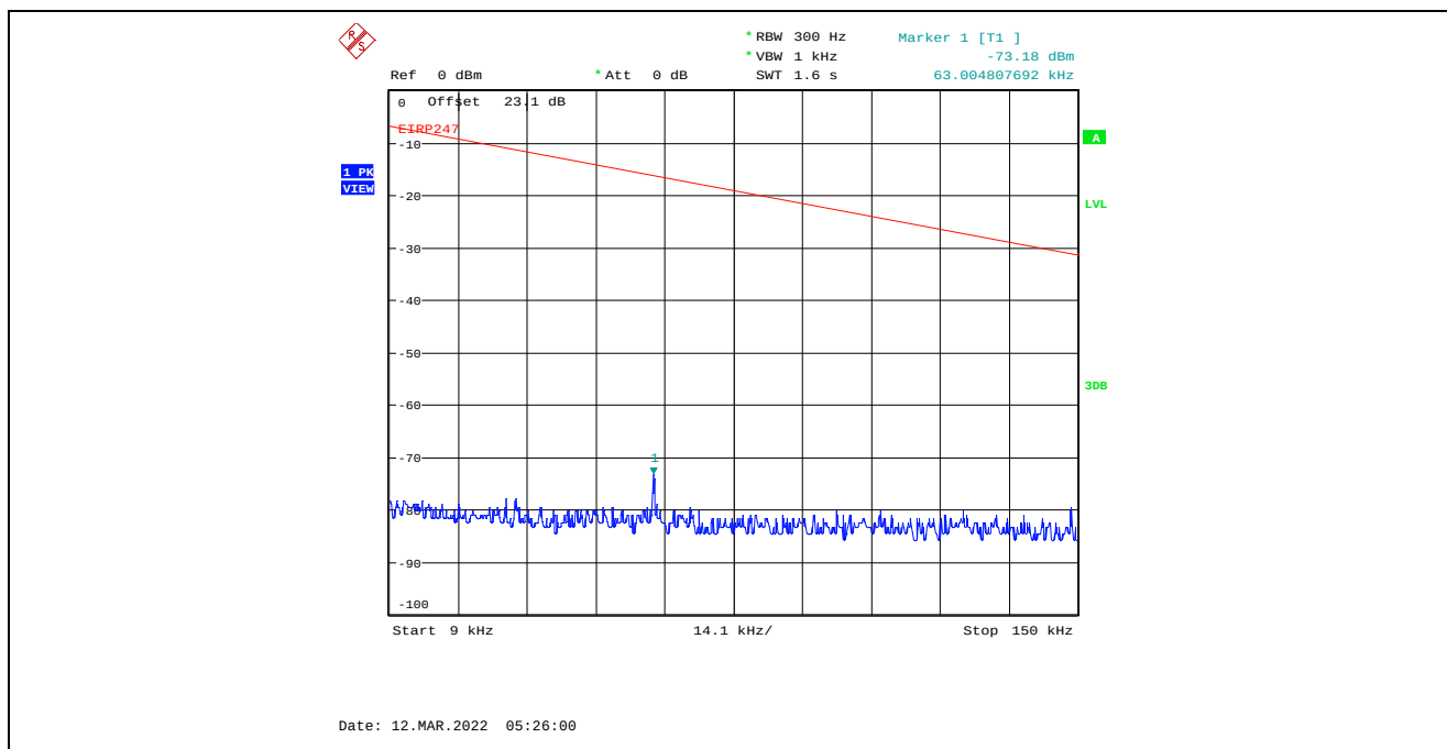
Plot C.2.102. Conducted Spurious Emissions in Restricted Frequency Bands, Chain 2 40 MHz Channel Bandwidth, Data Rate 7, Raw Power Setting 24, 2437 MHz, 9 kHz - 150 kHz, Peak Detector
