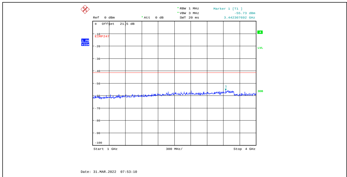
Plot C.4.118. Conducted Spurious Emissions in Restricted Frequency Bands, Chain 2 40 MHz Channel Bandwidth, Data Rate 7, Raw Power Setting 0, 2452 MHz, 1 GHz – 4 GHz, Peak Detector
