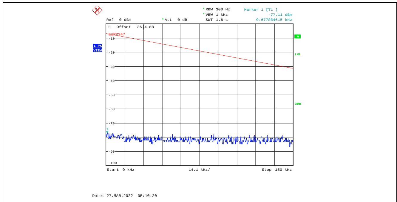
Plot C.3.42. Conducted Spurious Emissions in Restricted Frequency Bands, Chain 2 8 MHz Channel Bandwidth, Data Rate 3, Raw Power Setting 6, 2437 MHz, 9 kHz - 150 kHz, Peak Detector
