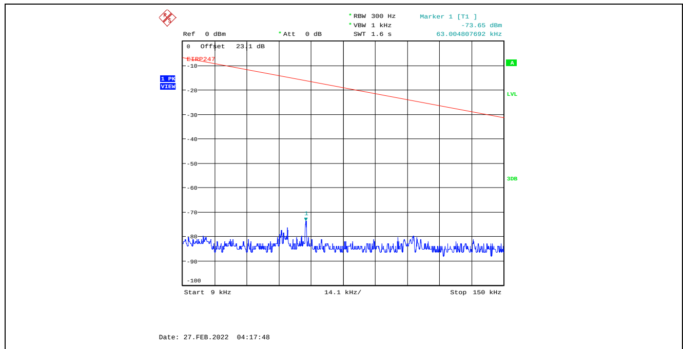
Plot C.2.41. Conducted Spurious Emissions in Restricted Frequency Bands, Chain 1 8 MHz Channel Bandwidth, Data Rate 7, Raw Power Setting 23, 2437 MHz, 9 kHz - 150 kHz, Peak Detector
