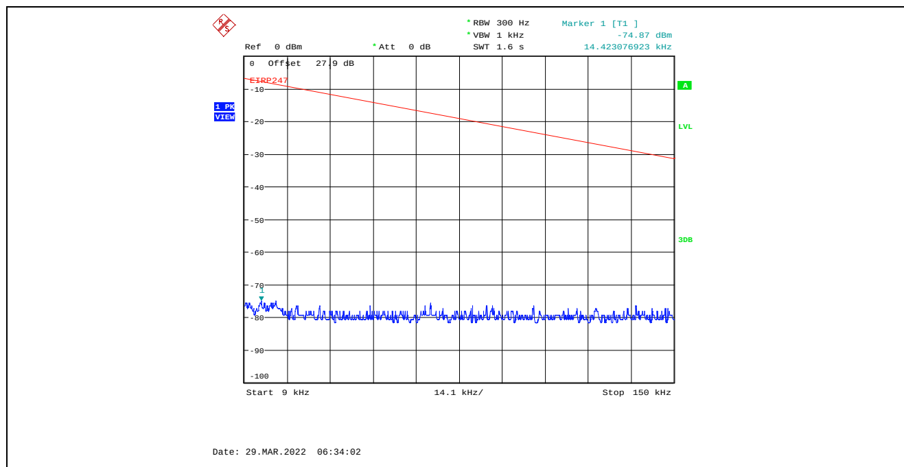
Plot C.4.81. Conducted Spurious Emissions in Restricted Frequency Bands, Chain 1 20 MHz Channel Bandwidth, Data Rate 7, Raw Power Setting 0, 2462 MHz, 9 kHz - 150 kHz, Peak Detector
