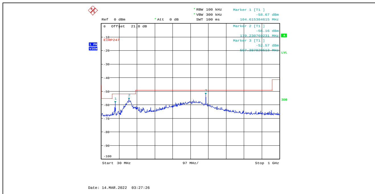
Plot C.1.55. Conducted Spurious Emissions in Restricted Frequency Bands, Chain 1 8 MHz Channel Bandwidth, Data Rate 3, Raw Power Setting 14, 2476 MHz, 30 MHz - 1 GHz, Peak Detector
