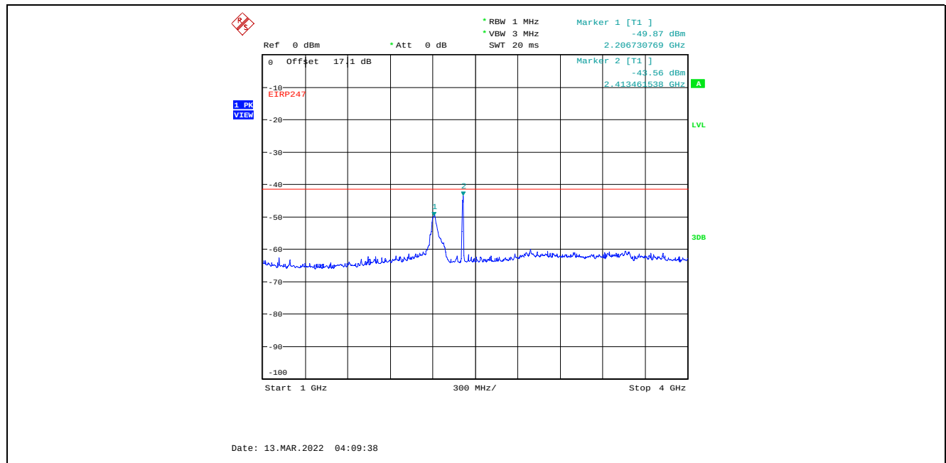
Plot C.1.67. Conducted Spurious Emissions in Restricted Frequency Bands, Chain 1 20 MHz Channel Bandwidth, Data Rate 3, Raw Power Setting 26, 2412 MHz, 1 GHz – 4 GHz, Peak Detector Marker 2 is Fundamental Signal
