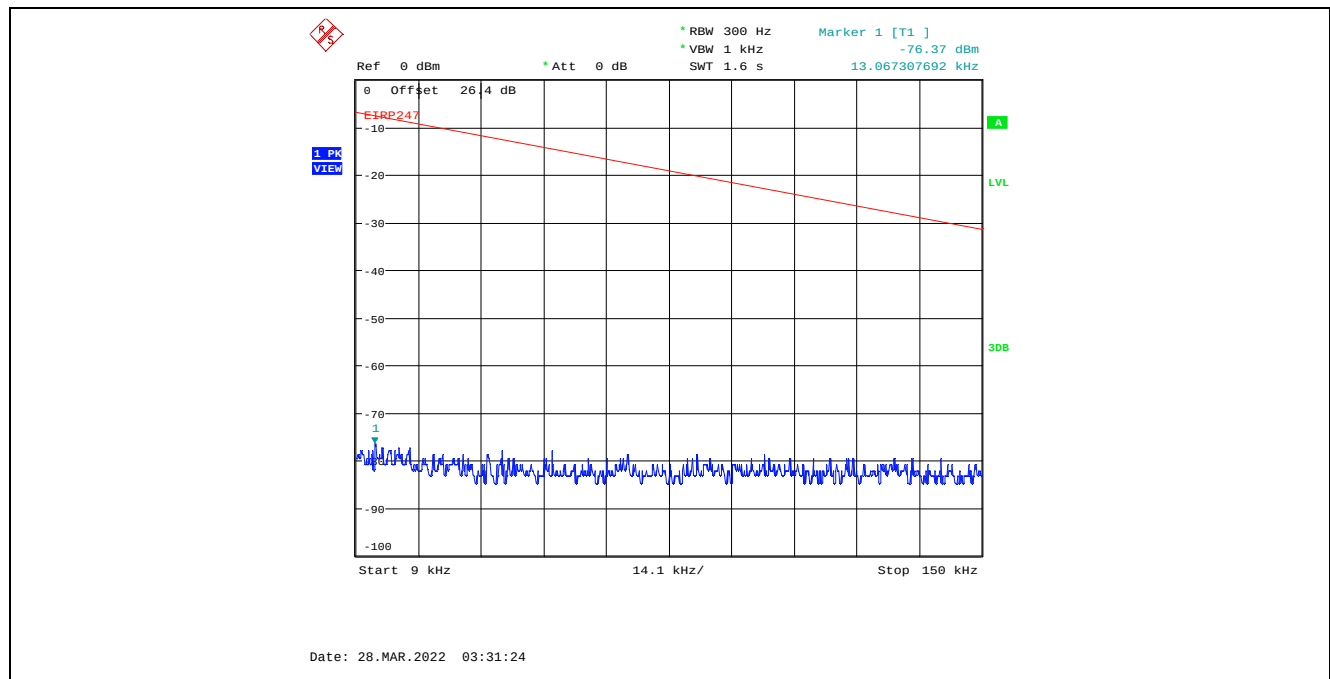
Plot C.4.41. Conducted Spurious Emissions in Restricted Frequency Bands, Chain 1 8 MHz Channel Bandwidth, Data Rate 7, Raw Power Setting 0, 2437 MHz, 9 kHz - 150 kHz, Peak Detector
