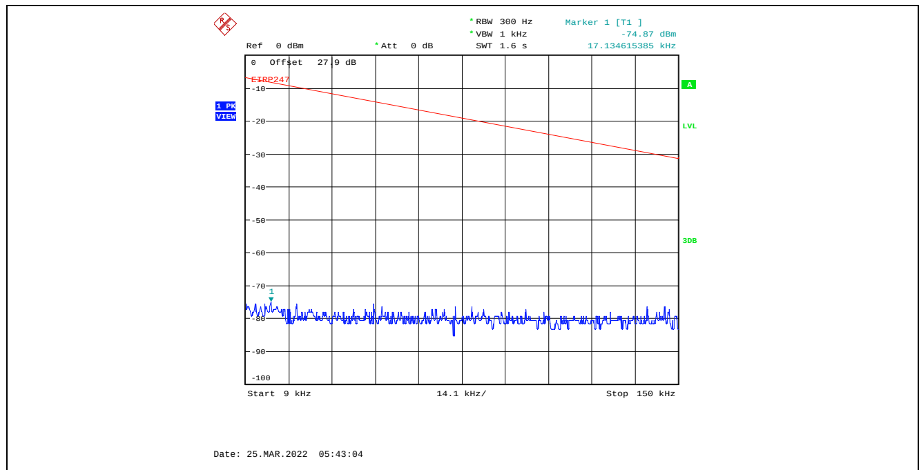
Plot C.4.21. Conducted Spurious Emissions in Restricted Frequency Bands, Chain 1 4 MHz Channel Bandwidth, Data Rate 7, Raw Power Setting 0, 2477 MHz, 9 kHz - 150 kHz, Peak Detector
