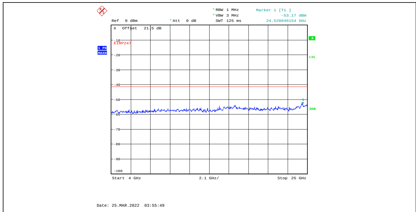
Plot C.3.30. Conducted Spurious Emissions in Restricted Frequency Bands, Chain 2 4 MHz Channel Bandwidth, Data Rate 3, Raw Power Setting 0, 2477 MHz, 4 GHz - 25 GHz, Peak Detector
