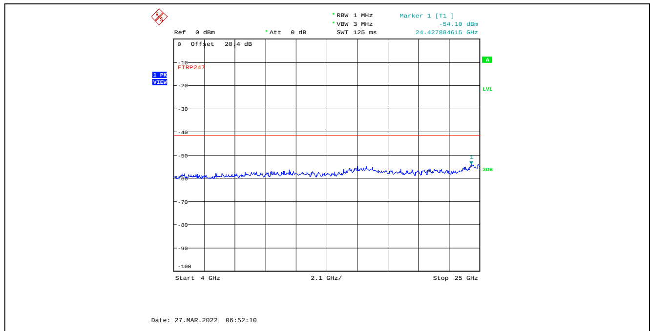
Plot C.4.59. Conducted Spurious Emissions in Restricted Frequency Bands, Chain 1 8 MHz Channel Bandwidth, Data Rate 7, Raw Power Setting 0, 2476 MHz, 4 GHz - 25 GHz, Peak Detector
