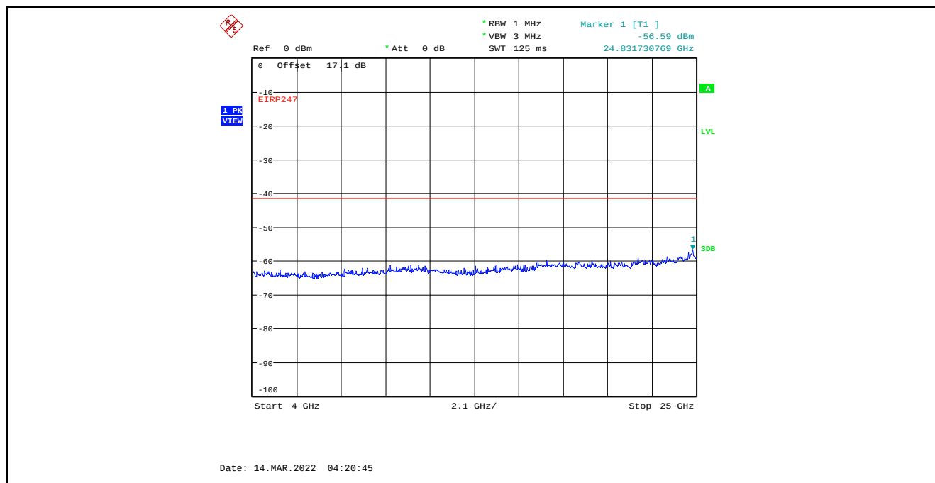
Plot C.2.59. Conducted Spurious Emissions in Restricted Frequency Bands, Chain 1 8 MHz Channel Bandwidth, Data Rate 7, Raw Power Setting 12, 2476 MHz, 4 GHz - 25 GHz, Peak Detector
