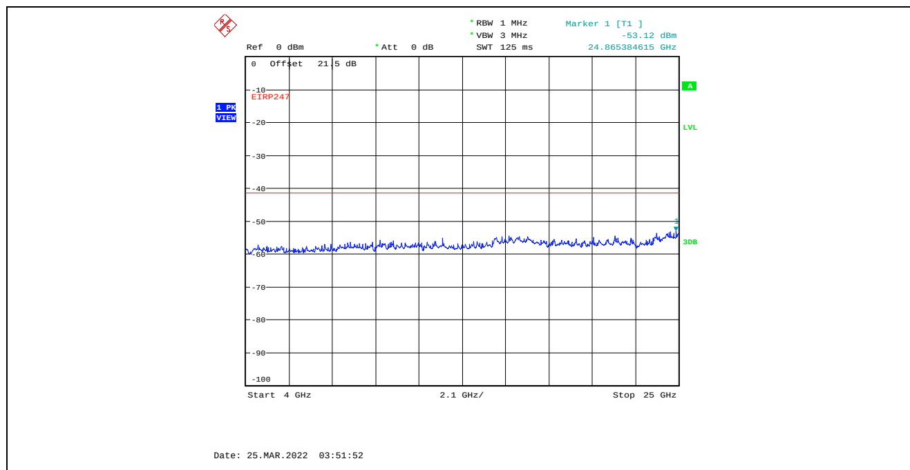
Plot C.3.19. Conducted Spurious Emissions in Restricted Frequency Bands, Chain 1 4 MHz Channel Bandwidth, Data Rate 3, Raw Power Setting 8, 2437 MHz, 4 GHz - 25 GHz, Peak Detector
