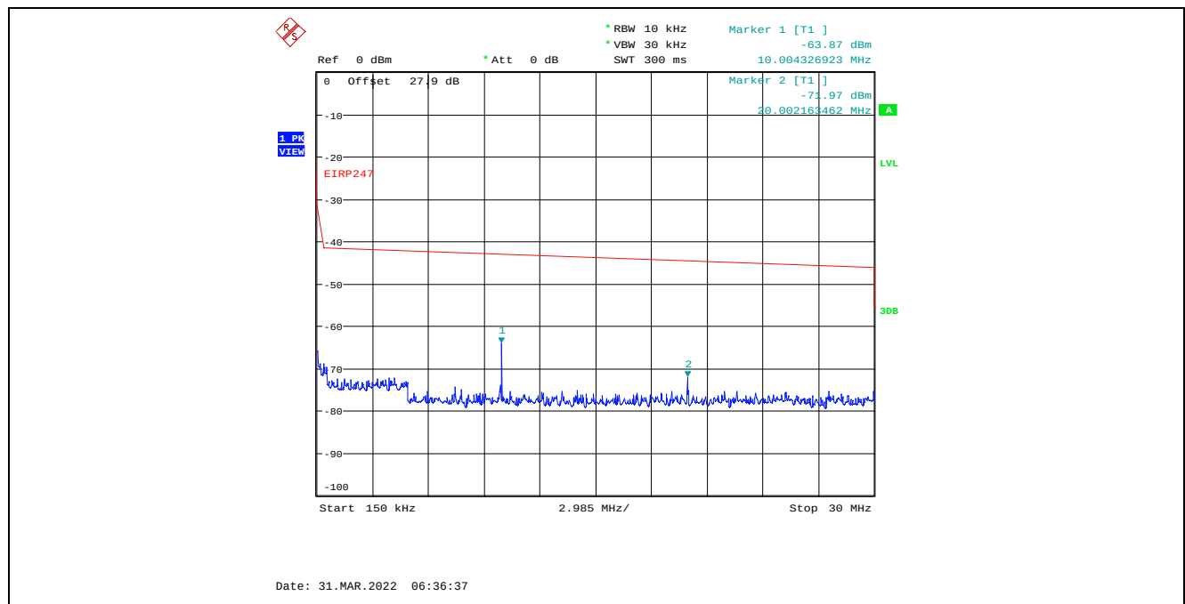
Plot C.4.104. Conducted Spurious Emissions in Restricted Frequency Bands, Chain 2 40 MHz Channel Bandwidth, Data Rate 7, Raw Power Setting 0, 2437 MHz, 150 kHz – 30 MHz, Peak Detector
