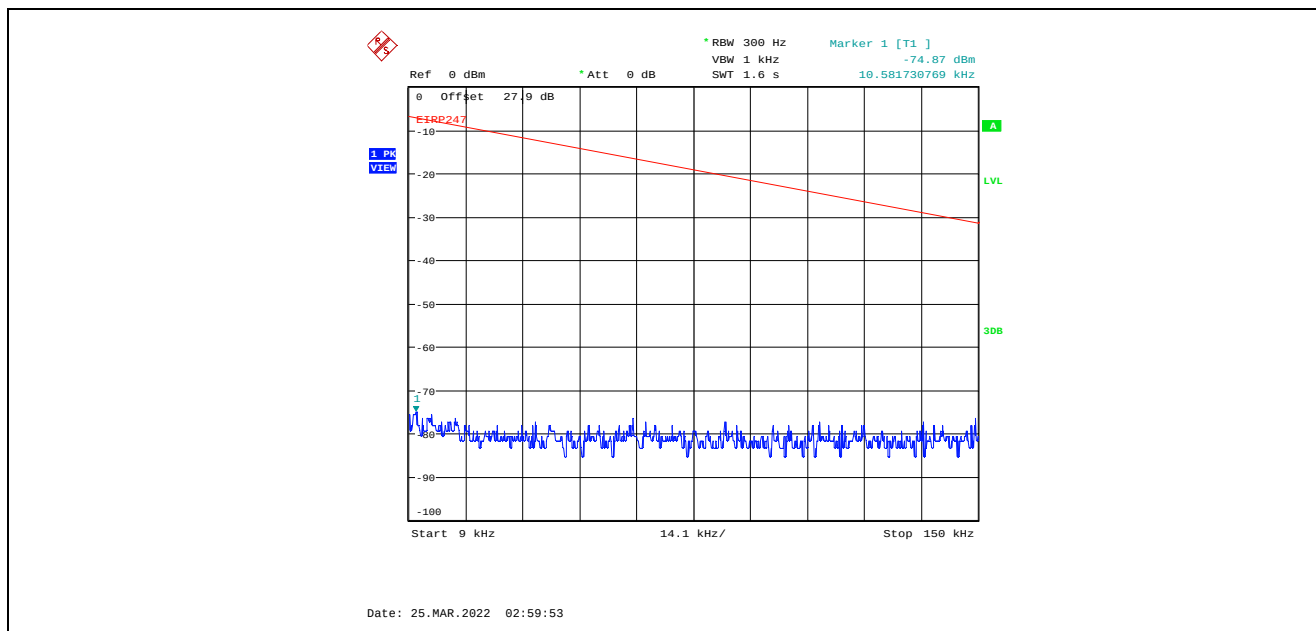
Plot C.3.2. Conducted Spurious Emissions in Restricted Frequency Bands, Chain 2 4 MHz Channel Bandwidth, Data Rate 3, Raw Power Setting 8, 2402 MHz, 9 kHz - 150 kHz, Peak Detector
