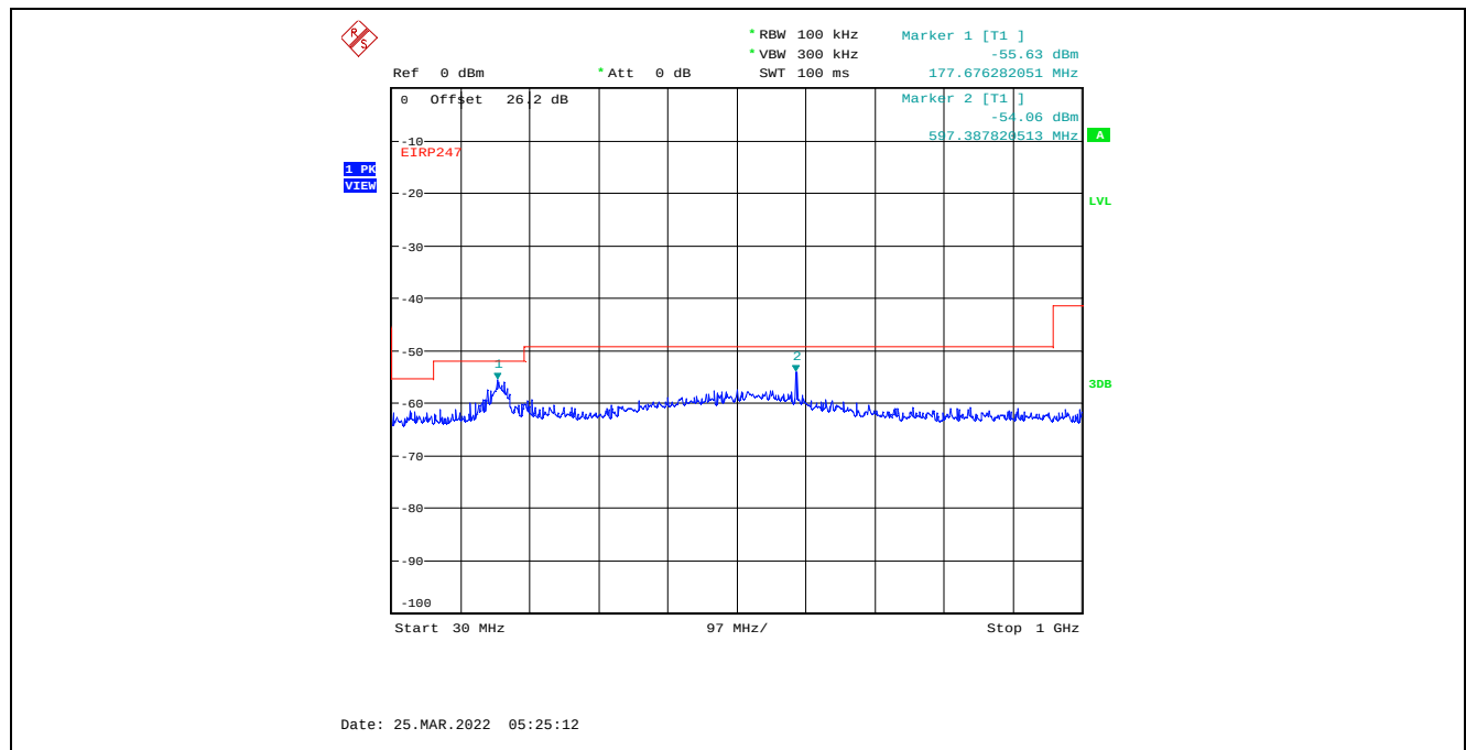
Plot C.4.15. Conducted Spurious Emissions in Restricted Frequency Bands, Chain 1 4 MHz Channel Bandwidth, Data Rate 7, Raw Power Setting 0, 2437 MHz, 30 MHz - 1 GHz, Peak Detector
