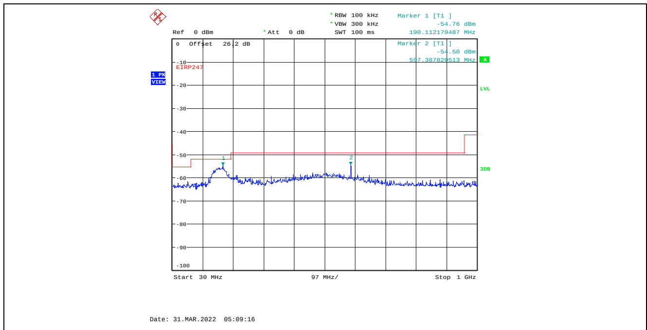
Plot C.4.115. Conducted Spurious Emissions in Restricted Frequency Bands, Chain 1 40 MHz Channel Bandwidth, Data Rate 7, Raw Power Setting 0, 2452 MHz, 30 MHz - 1 GHz, Peak Detector
