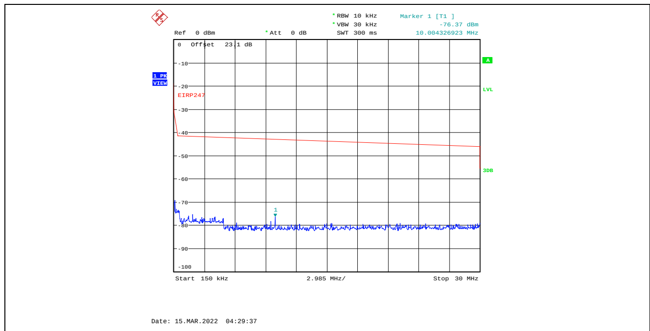
Plot C.2.24. Conducted Spurious Emissions in Restricted Frequency Bands, Chain 2 4 MHz Channel Bandwidth, Data Rate 7, Raw Power Setting 20, 2477 MHz, 150 kHz – 30 MHz, Peak Detector
