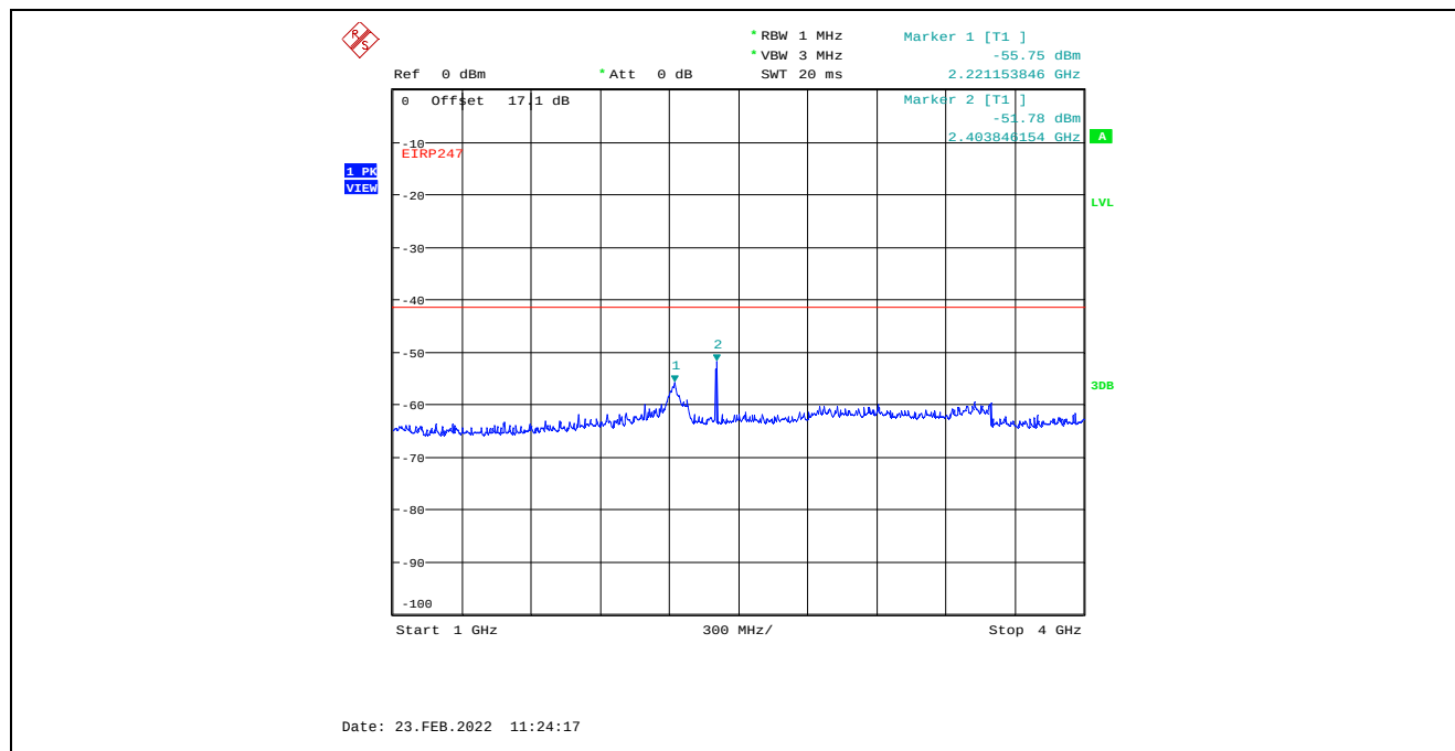
Plot C.1.8. Conducted Spurious Emissions in Restricted Frequency Bands, Chain 2 4 MHz Channel Bandwidth, Data Rate 3, Raw Power Setting 16, 2402 MHz, 1 GHz – 4 GHz, Peak Detector
