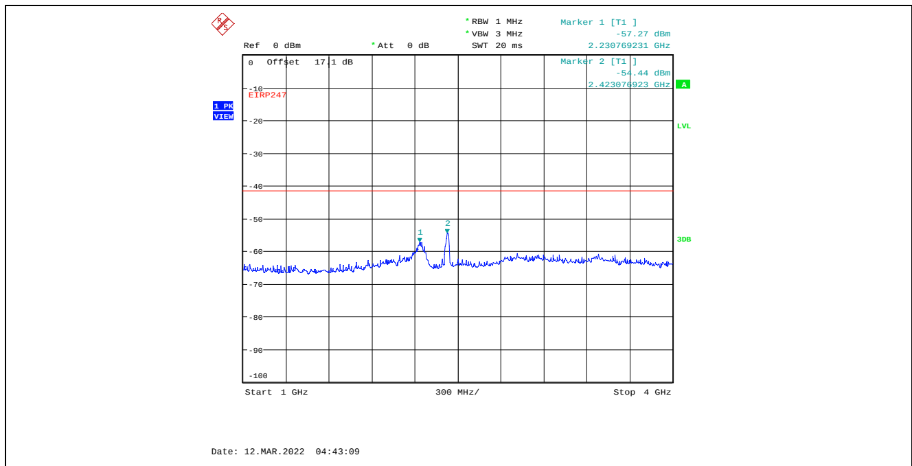
Plot C.2.98. Conducted Spurious Emissions in Restricted Frequency Bands, Chain 2 40 MHz Channel Bandwidth, Data Rate 7, Raw Power Setting 20, 2422 MHz, 1 GHz – 4 GHz, Peak Detector
