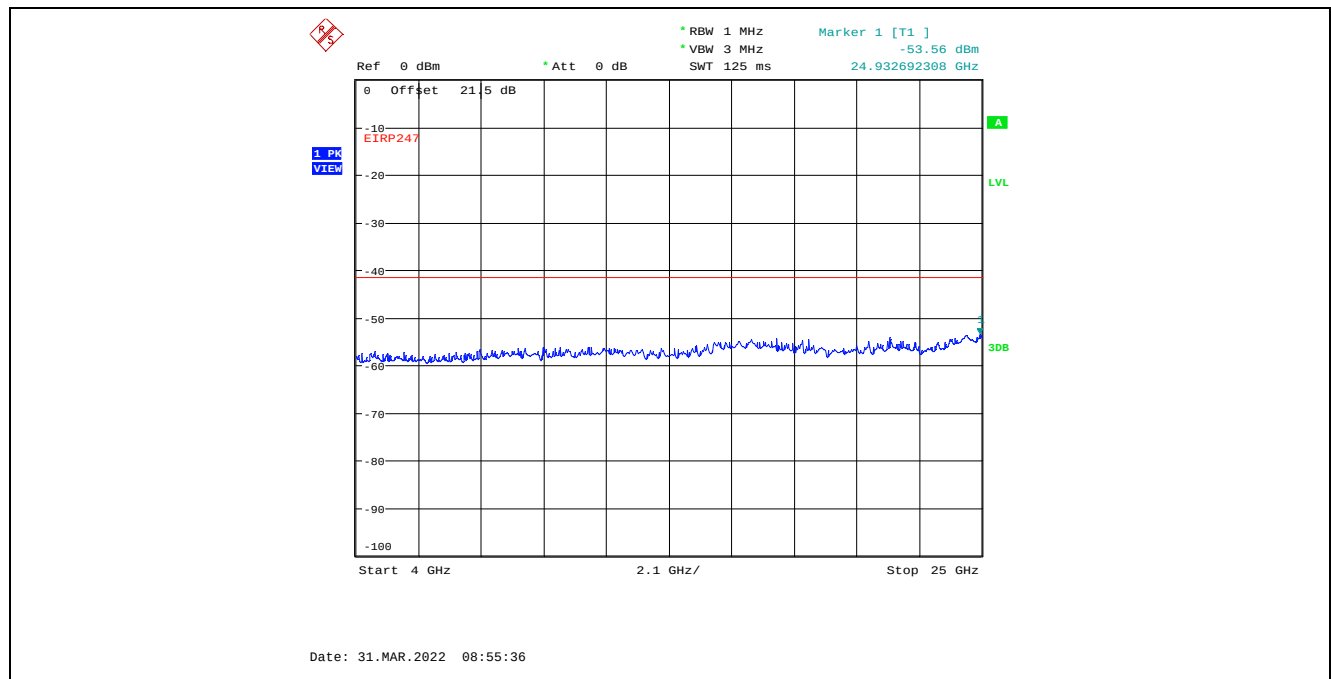
Plot C.4.119. Conducted Spurious Emissions in Restricted Frequency Bands, Chain 1 40 MHz Channel Bandwidth, Data Rate 7, Raw Power Setting 0, 2452 MHz, 4 GHz - 25 GHz, Peak Detector
