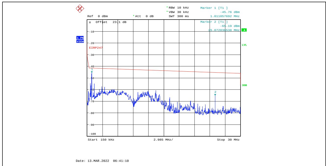
Plot C.2.64. Conducted Spurious Emissions in Restricted Frequency Bands, Chain 2 20 MHz Channel Bandwidth, Data Rate 7, Raw Power Setting 23, 2412 MHz, 150 kHz – 30 MHz, Peak Detector
