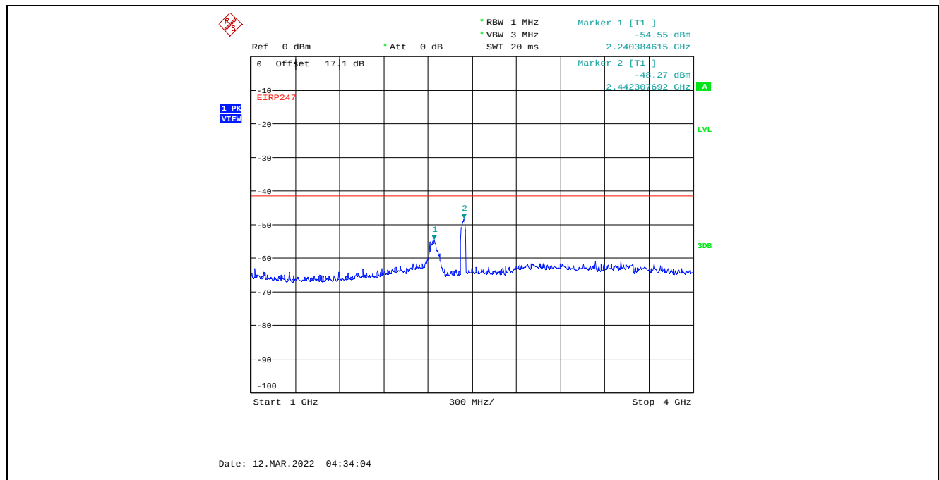
Plot C.2.107. Conducted Spurious Emissions in Restricted Frequency Bands, Chain 1 40 MHz Channel Bandwidth, Data Rate 7, Raw Power Setting 24, 2437 MHz, 1 GHz – 4 GHz, Peak Detector
