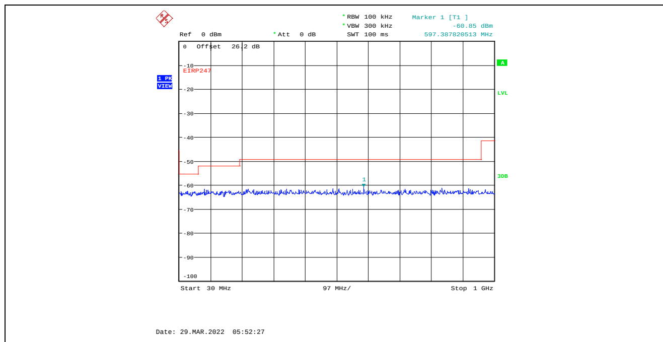
Plot C.4.85. Conducted Spurious Emissions in Restricted Frequency Bands, Chain 1 20 MHz Channel Bandwidth, Data Rate 7, Raw Power Setting 0, 2462 MHz, 30 MHz - 1 GHz, Peak Detector
