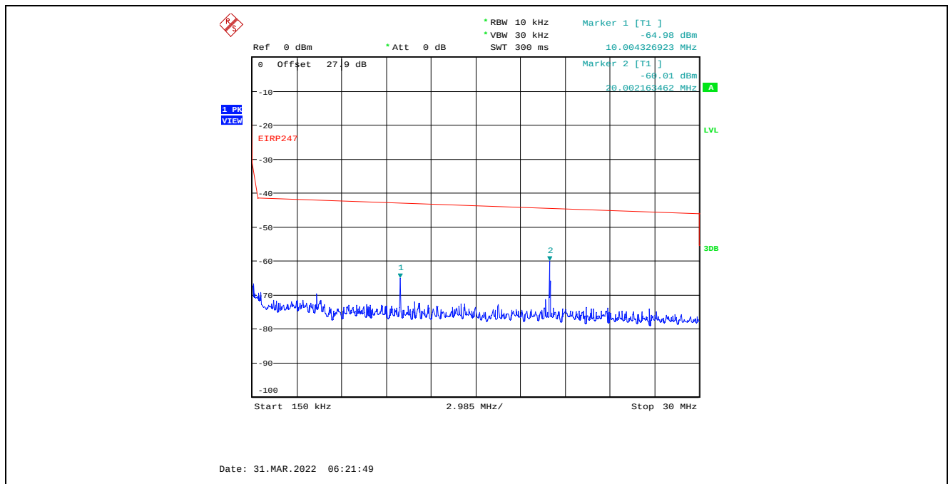
Plot C.3.94. Conducted Spurious Emissions in Restricted Frequency Bands, Chain 2 40 MHz Channel Bandwidth, Data Rate 3, Raw Power Setting 0, 2422 MHz, 150 kHz – 30 MHz, Peak Detector
