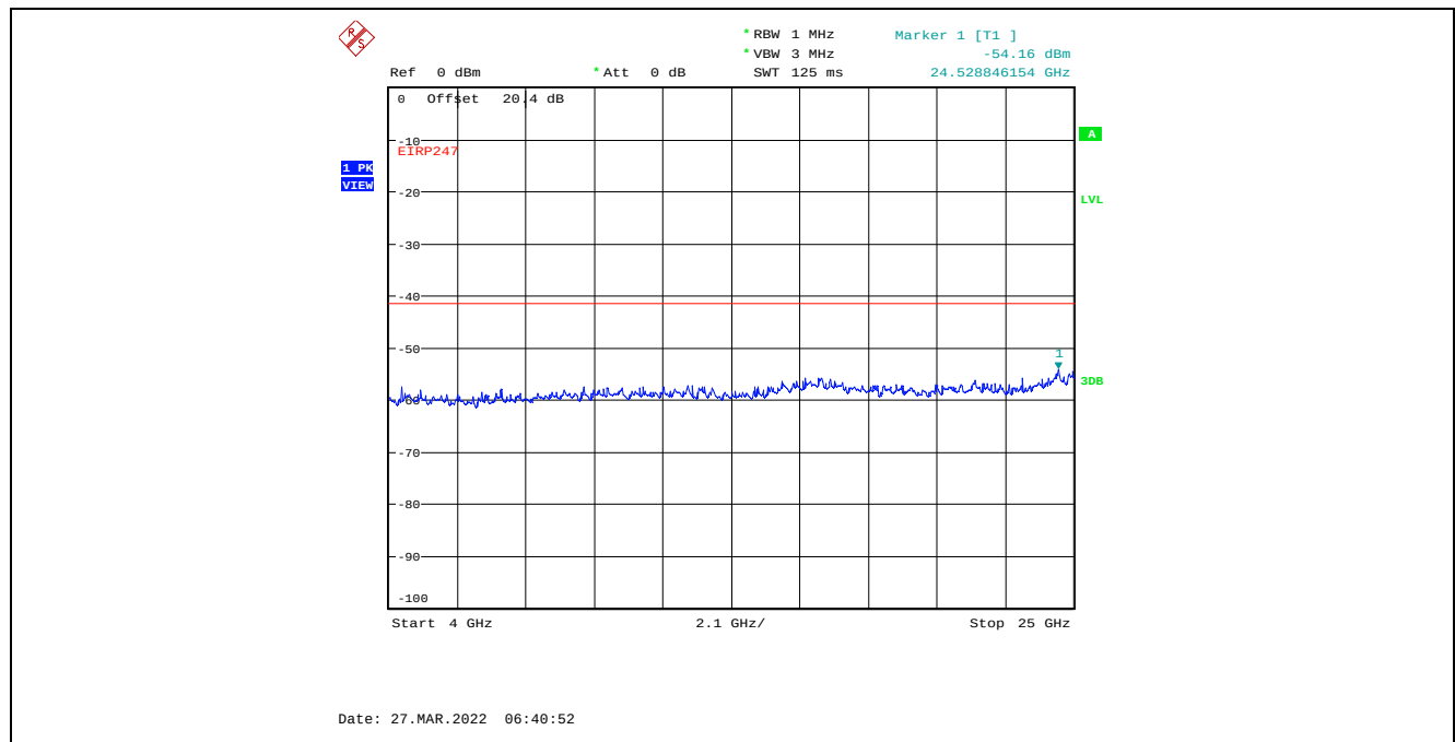
Plot C.3.60. Conducted Spurious Emissions in Restricted Frequency Bands, Chain 2 8 MHz Channel Bandwidth, Data Rate 3, Raw Power Setting 0, 2476 MHz, 4 GHz - 25 GHz, Peak Detector
