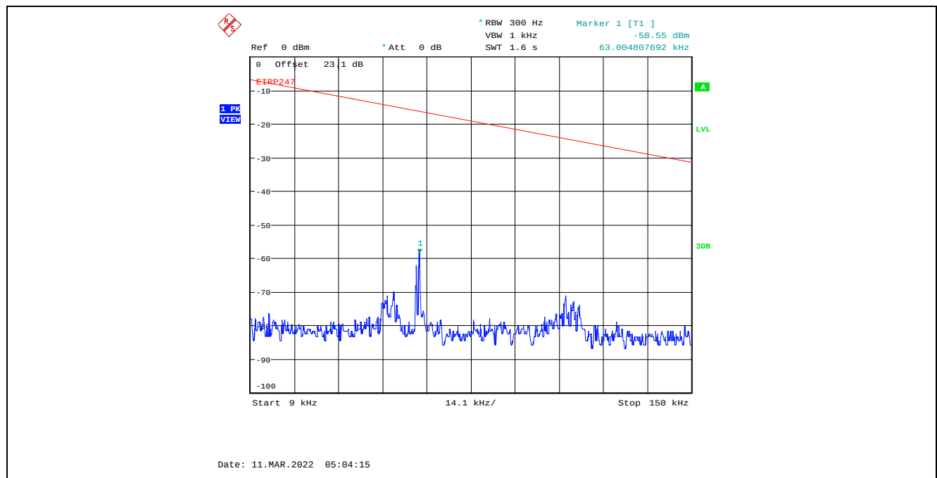
Plot C.1.102. Conducted Spurious Emissions in Restricted Frequency Bands, Chain 2 40 MHz Channel Bandwidth, Data Rate 3, Raw Power Setting 22, 2437 MHz, 9 kHz - 150 kHz, Peak Detector
