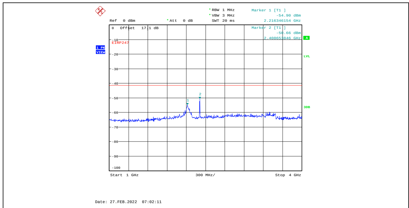
Plot C.1.38. Conducted Spurious Emissions in Restricted Frequency Bands, Chain 2 8 MHz Channel Bandwidth, Data Rate 3, Raw Power Setting 21, 2407 MHz, 1 GHz – 4 GHz, Peak Detector
