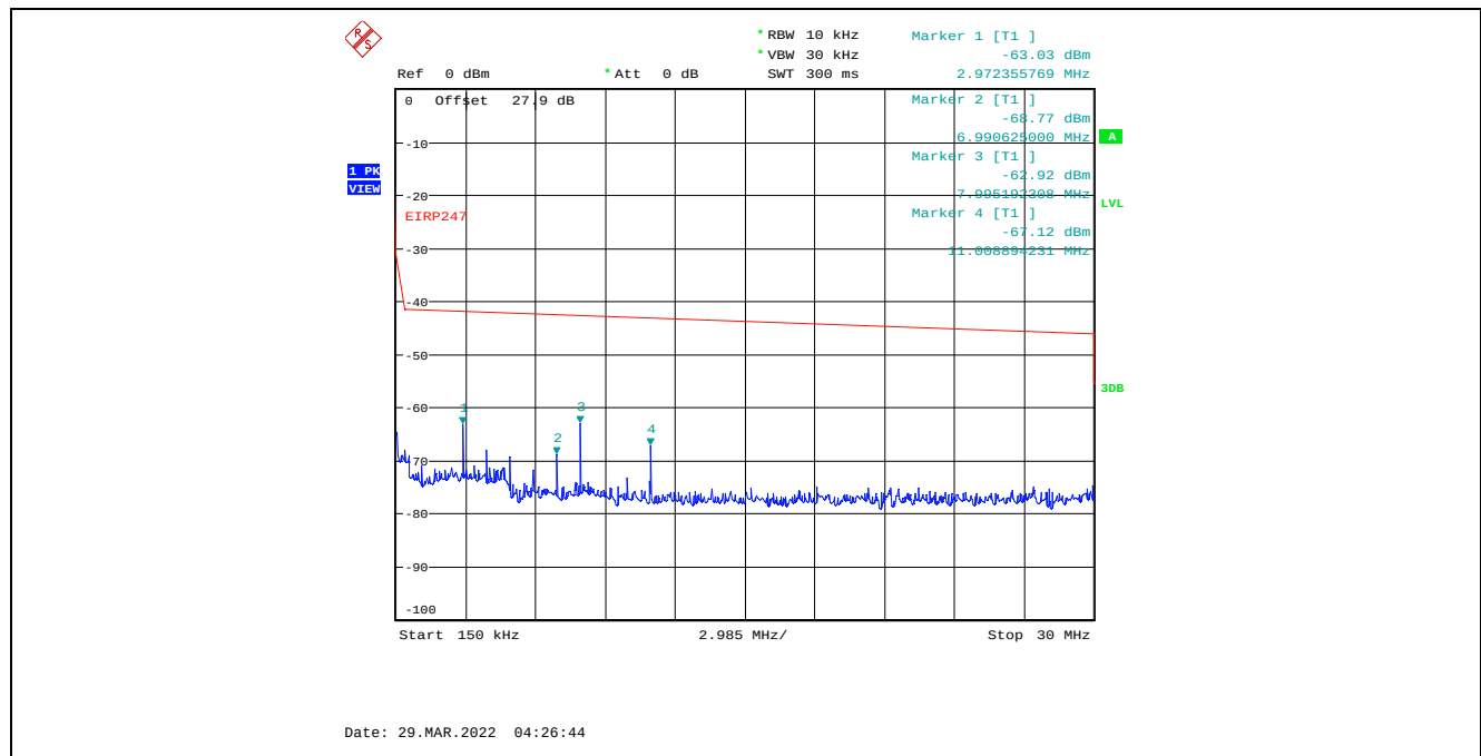
Plot C.3.84. Conducted Spurious Emissions in Restricted Frequency Bands, Chain 2 20 MHz Channel Bandwidth, Data Rate 3, Raw Power Setting 7, 2462 MHz, 150 kHz – 30 MHz, Peak Detector
