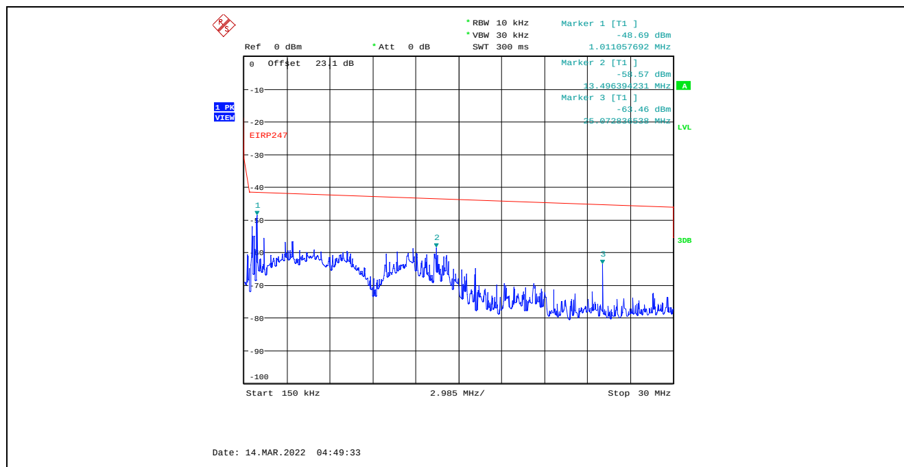
Plot C.2.54. Conducted Spurious Emissions in Restricted Frequency Bands, Chain 2 8 MHz Channel Bandwidth, Data Rate 7, Raw Power Setting 12, 2476 MHz, 150 kHz – 30 MHz, Peak Detector
