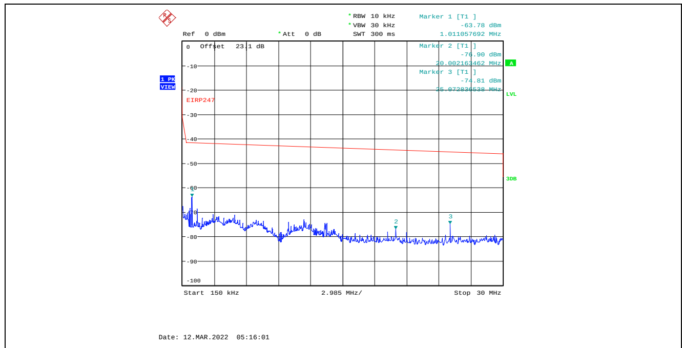
Plot C.2.114. Conducted Spurious Emissions in Restricted Frequency Bands, Chain 2 40 MHz Channel Bandwidth, Data Rate 7, Raw Power Setting 22, 2452 MHz, 150 kHz – 30 MHz, Peak Detector
