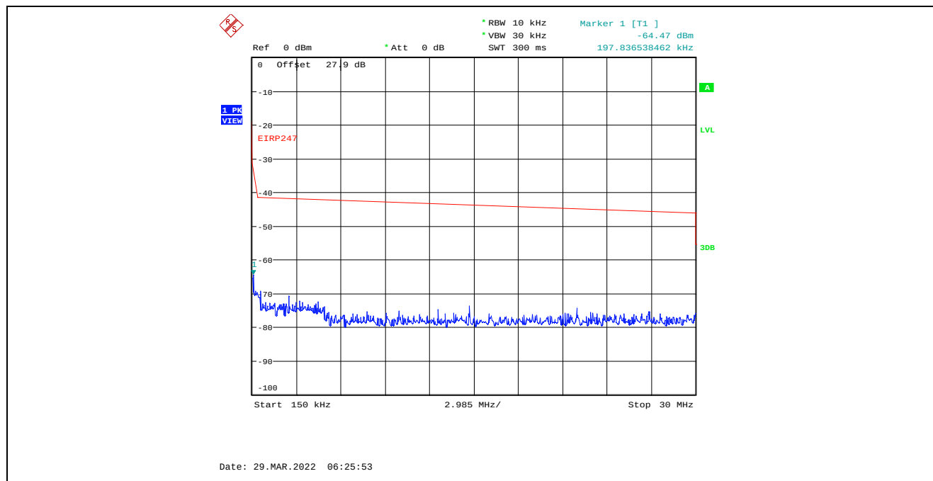
Plot C.4.84. Conducted Spurious Emissions in Restricted Frequency Bands, Chain 2 20 MHz Channel Bandwidth, Data Rate 7, Raw Power Setting 0, 2462 MHz, 150 kHz – 30 MHz, Peak Detector
