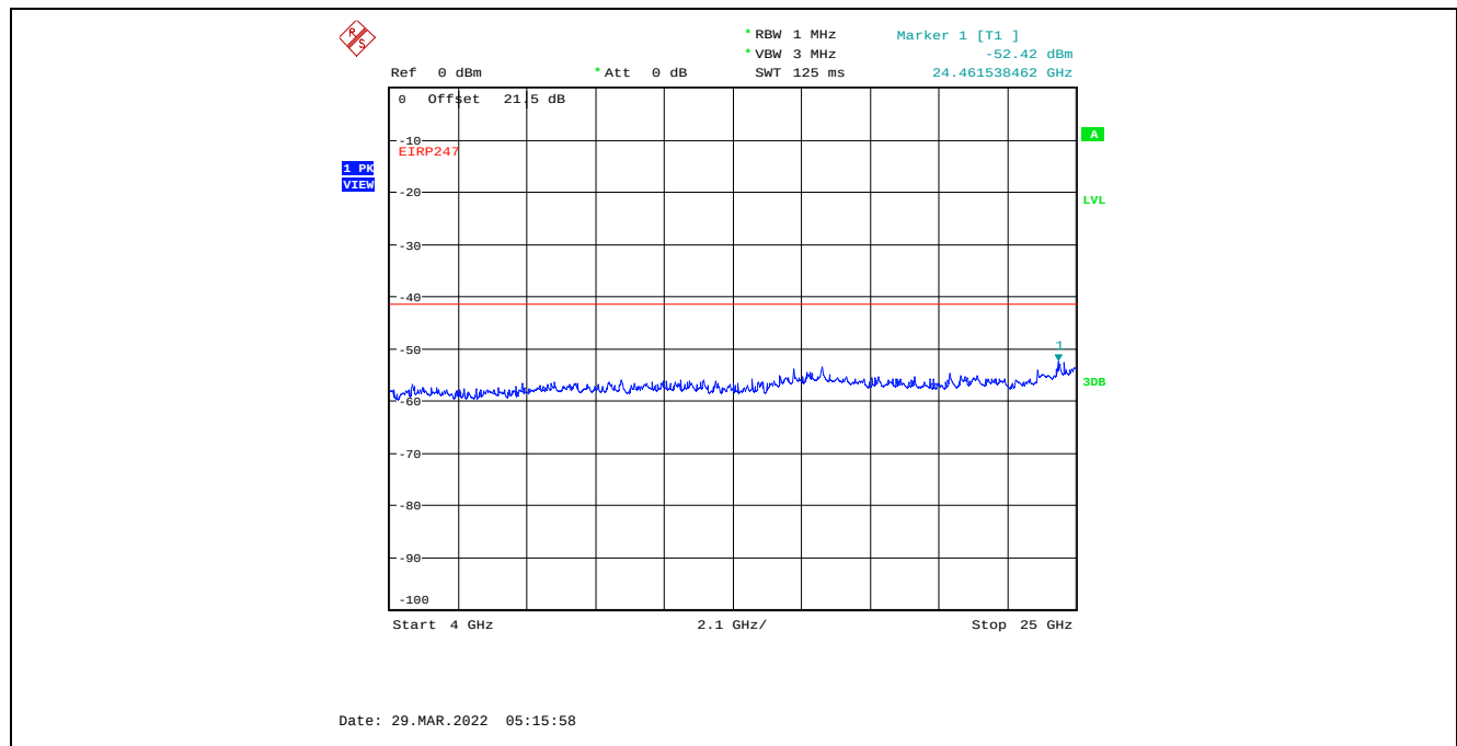
Plot C.3.69. Conducted Spurious Emissions in Restricted Frequency Bands, Chain 1 20 MHz Channel Bandwidth, Data Rate 3, Raw Power Setting 7, 2412 MHz, 4 GHz - 25 GHz, Peak Detector
