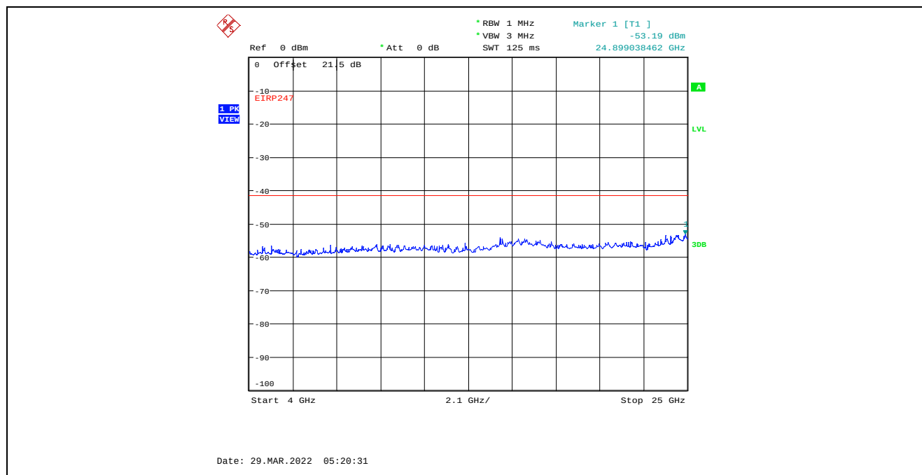
Plot C.4.89. Conducted Spurious Emissions in Restricted Frequency Bands, Chain 1 20 MHz Channel Bandwidth, Data Rate 7, Raw Power Setting 0, 2462 MHz, 4 GHz - 25 GHz, Peak Detector
