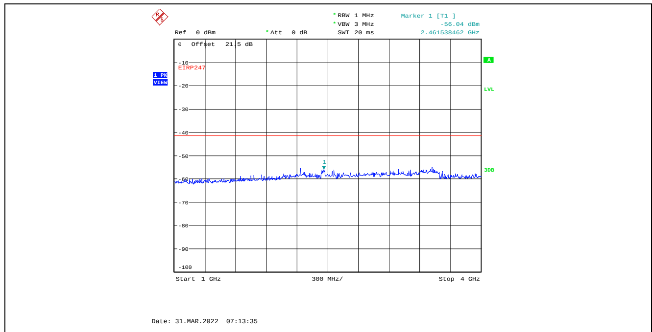
Plot C.4.117. Conducted Spurious Emissions in Restricted Frequency Bands, Chain 1 40 MHz Channel Bandwidth, Data Rate 7, Raw Power Setting 0, 2452 MHz, 1 GHz – 4 GHz, Peak Detector
