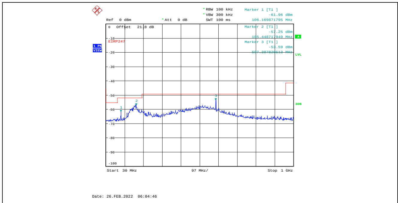
Plot C.2.15. Conducted Spurious Emissions in Restricted Frequency Bands, Chain 1 4 MHz Channel Bandwidth, Data Rate 7, Raw Power Setting 22, 2437 MHz, 30 MHz - 1 GHz, Peak Detector
