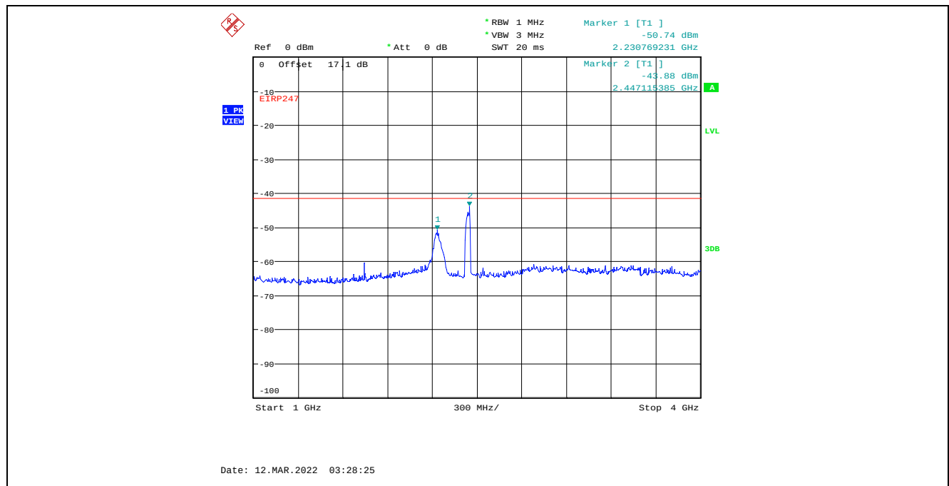
Plot C.1.107. Conducted Spurious Emissions in Restricted Frequency Bands, Chain 1 40 MHz Channel Bandwidth, Data Rate 3, Raw Power Setting 22, 2437 MHz, 1 GHz – 4 GHz, Peak Detector
