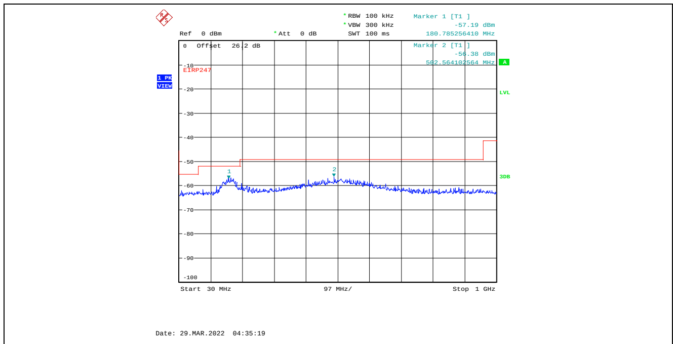
Plot C.3.66. Conducted Spurious Emissions in Restricted Frequency Bands, Chain 2 20 MHz Channel Bandwidth, Data Rate 3, Raw Power Setting 7, 2412 MHz, 30 MHz - 1 GHz, Peak Detector
