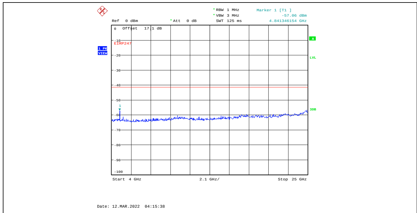
Plot C.2.110. Conducted Spurious Emissions in Restricted Frequency Bands, Chain 2 40 MHz Channel Bandwidth, Data Rate 7, Raw Power Setting 24, 2437 MHz, 4 GHz - 25 GHz, Peak Detector
