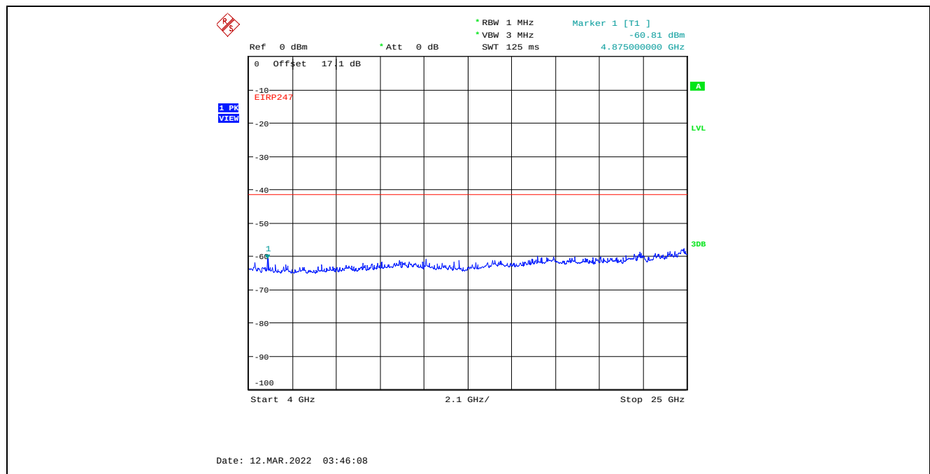
Plot C.1.120. Conducted Spurious Emissions in Restricted Frequency Bands, Chain 2 40 MHz Channel Bandwidth, Data Rate 3, Raw Power Setting 15, 2452 MHz, 4 GHz - 25 GHz, Peak Detector
