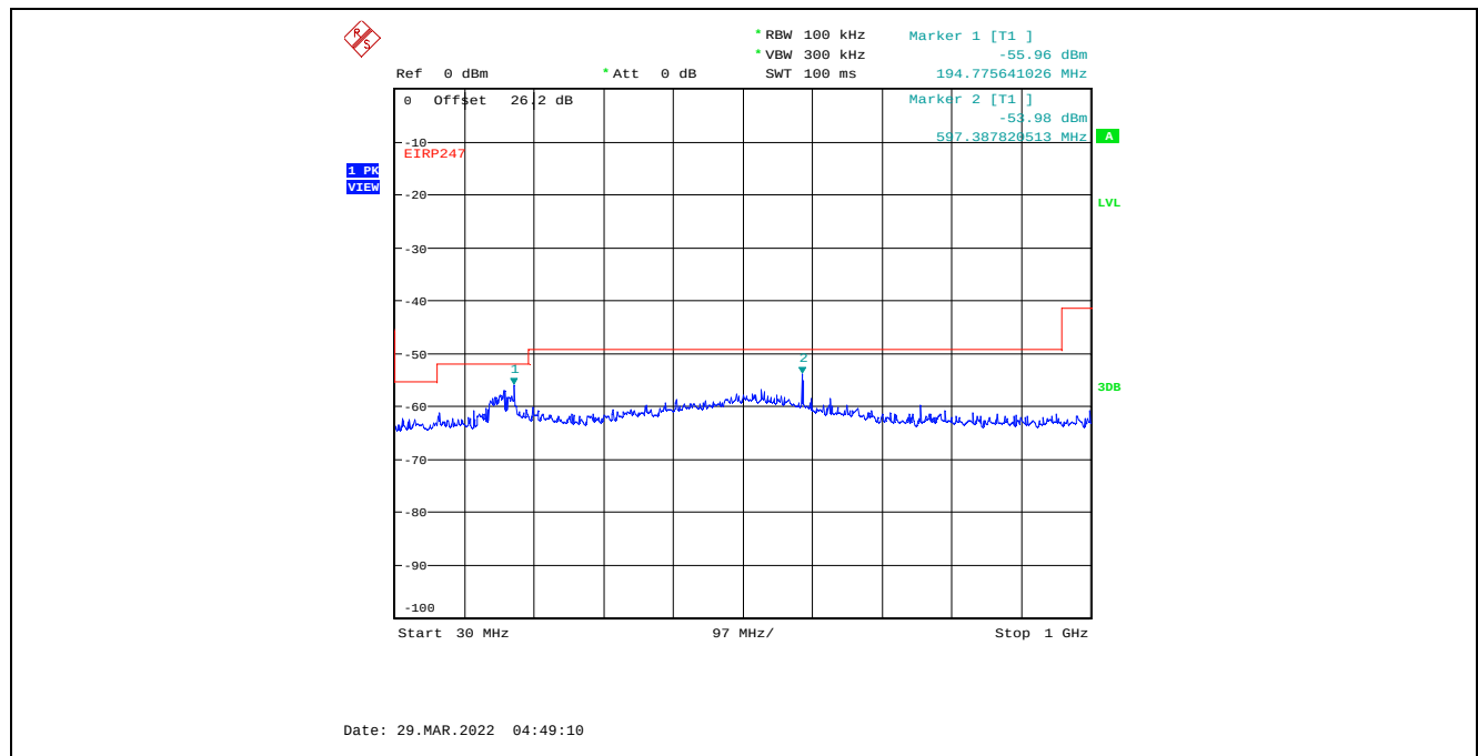
Plot C.3.75. Conducted Spurious Emissions in Restricted Frequency Bands, Chain 1 20 MHz Channel Bandwidth, Data Rate 3, Raw Power Setting 7, 2437 MHz, 30 MHz - 1 GHz, Peak Detector
