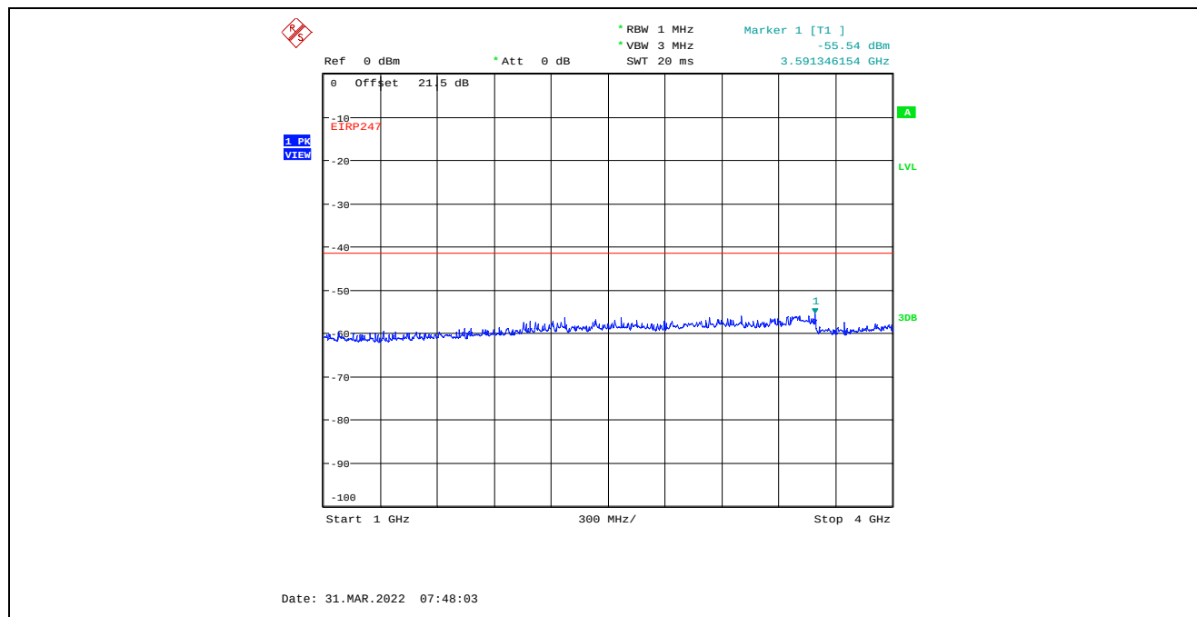
Plot C.4.98. Conducted Spurious Emissions in Restricted Frequency Bands, Chain 2 40 MHz Channel Bandwidth, Data Rate 7, Raw Power Setting 0, 2422 MHz, 1 GHz – 4 GHz, Peak Detector
