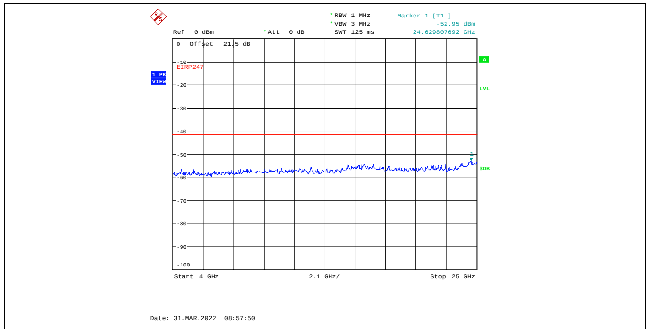
Plot C.4.99. Conducted Spurious Emissions in Restricted Frequency Bands, Chain 1 40 MHz Channel Bandwidth, Data Rate 7, Raw Power Setting 0, 2422 MHz, 4 GHz - 25 GHz, Peak Detector
