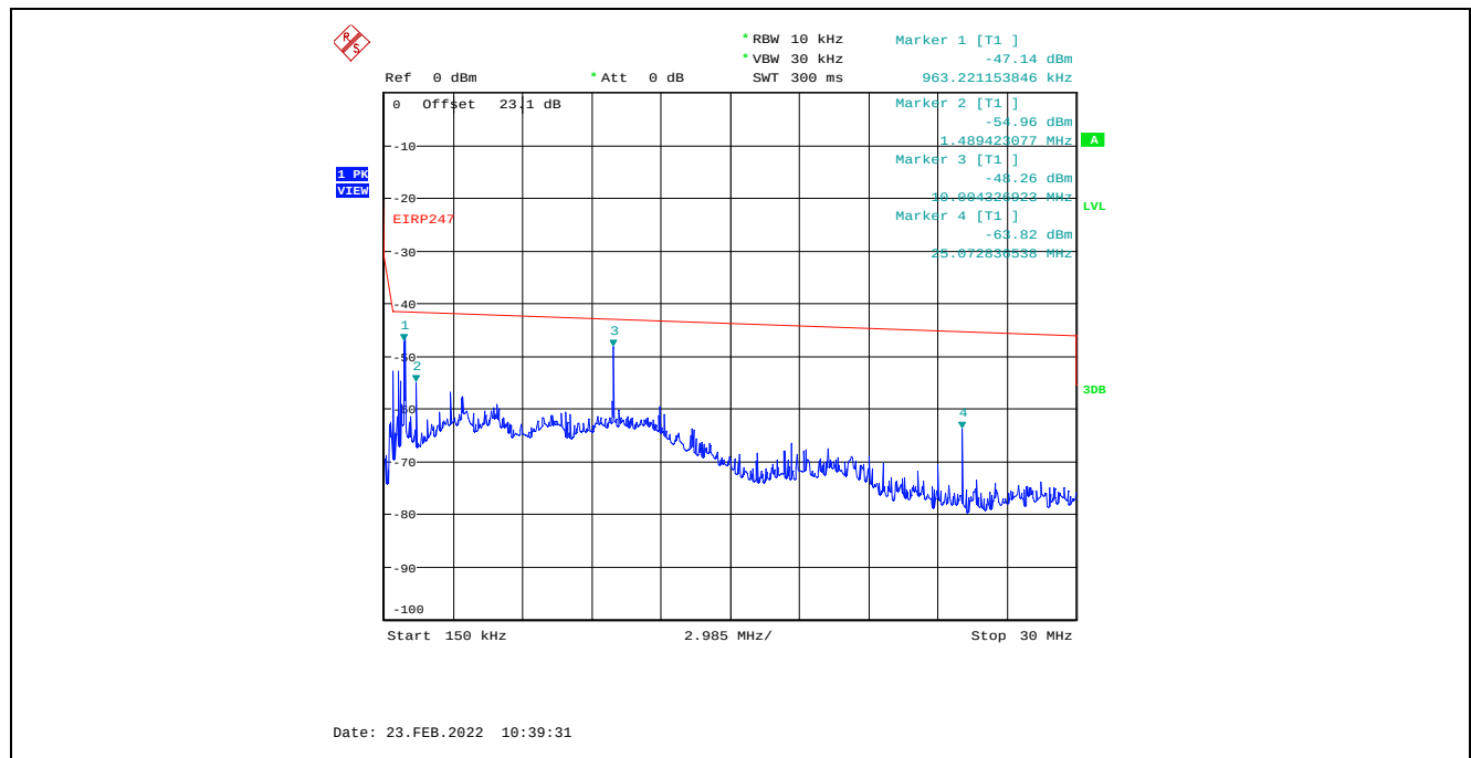
Plot C.1.3. Conducted Spurious Emissions in Restricted Frequency Bands, Chain 1 4 MHz Channel Bandwidth, Data Rate 3, Raw Power Setting 16, 2402 MHz, 150 kHz – 30 MHz, Peak Detector
