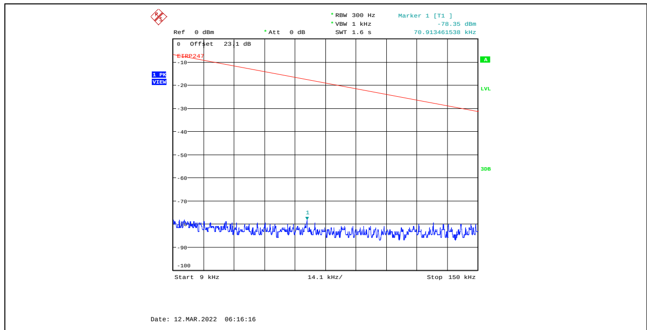
Plot C.1.81. Conducted Spurious Emissions in Restricted Frequency Bands, Chain 1 20 MHz Channel Bandwidth, Data Rate 3, Raw Power Setting 26, 2462 MHz, 9 kHz - 150 kHz, Peak Detector
