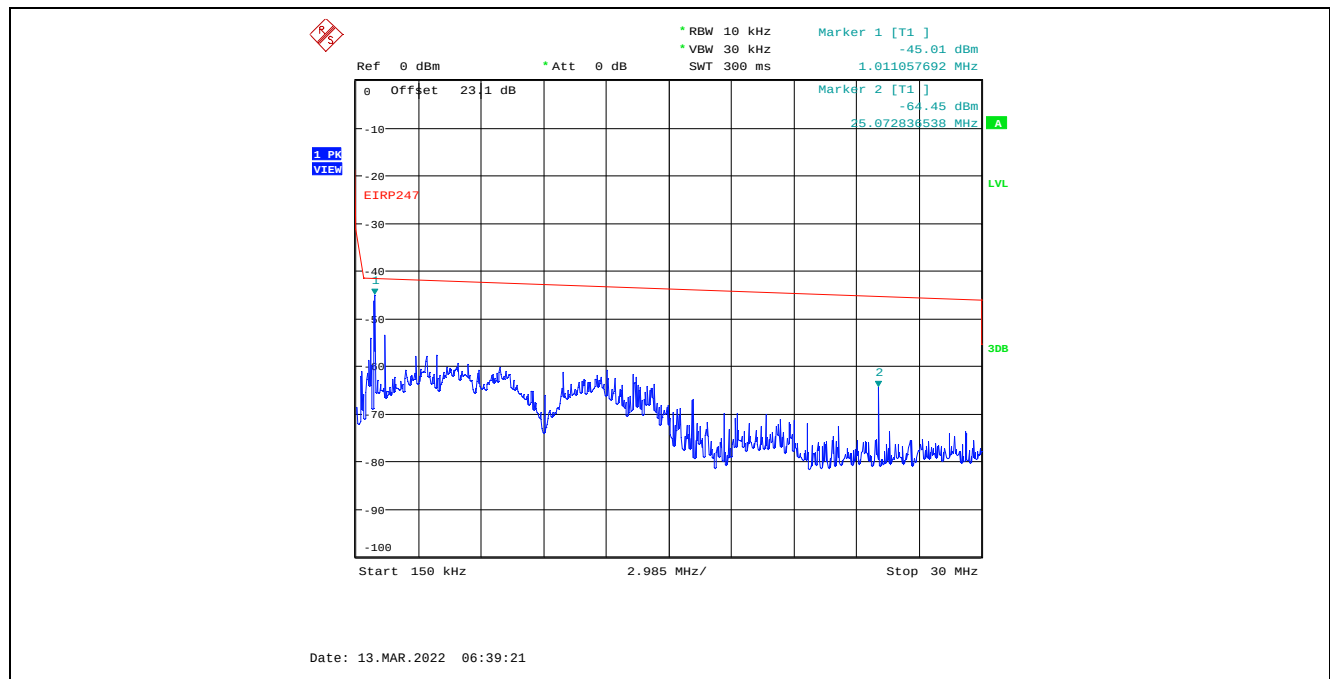
Plot C.2.74. Conducted Spurious Emissions in Restricted Frequency Bands, Chain 2 20 MHz Channel Bandwidth, Data Rate 7, Raw Power Setting 23, 2437 MHz, 150 kHz – 30 MHz, Peak Detector
