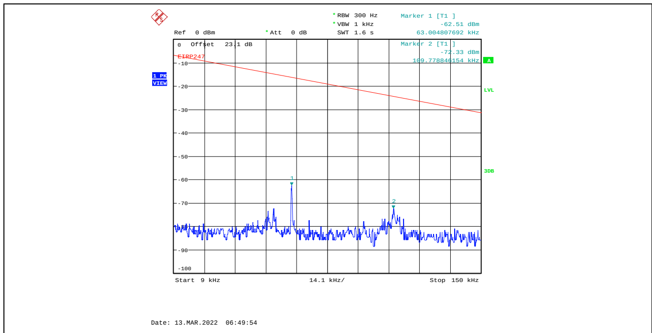
Plot C.2.82. Conducted Spurious Emissions in Restricted Frequency Bands, Chain 2 20 MHz Channel Bandwidth, Data Rate 7, Raw Power Setting 23, 2462 MHz, 9 kHz - 150 kHz, Peak Detector
