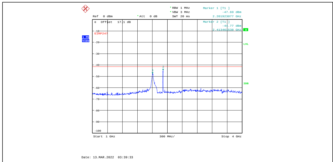
Plot C.1.68. Conducted Spurious Emissions in Restricted Frequency Bands, Chain 2 20 MHz Channel Bandwidth, Data Rate 3, Raw Power Setting 26, 2412 MHz, 1 GHz – 4 GHz, Peak Detector Marker 2 is Fundamental Signal
