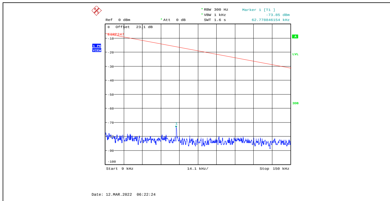
Plot C.1.62. Conducted Spurious Emissions in Restricted Frequency Bands, Chain 2 20 MHz Channel Bandwidth, Data Rate 3, Raw Power Setting 26, 2412 MHz, 9 kHz - 150 kHz, Peak Detector
