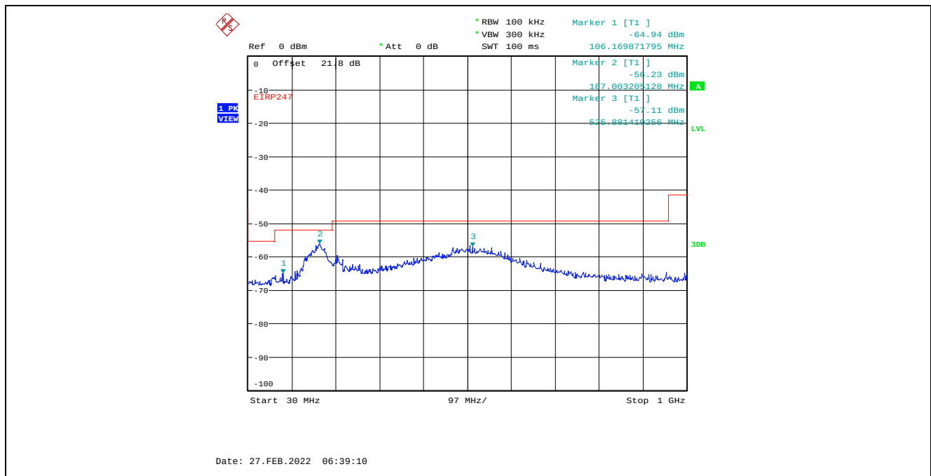
Plot C.2.36. Conducted Spurious Emissions in Restricted Frequency Bands, Chain 2 8 MHz Channel Bandwidth, Data Rate 7, Raw Power Setting 23, 2407 MHz, 30 MHz - 1 GHz, Peak Detector
