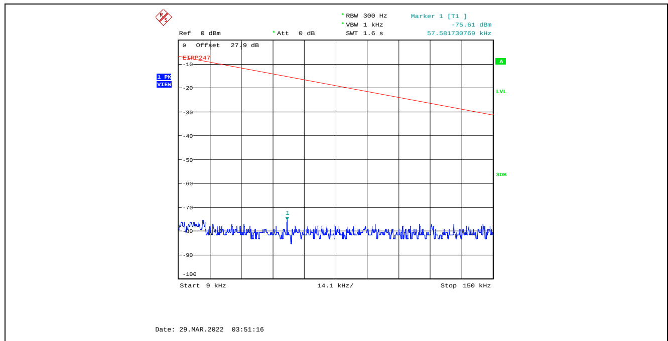
Plot C.3.61. Conducted Spurious Emissions in Restricted Frequency Bands, Chain 1 20 MHz Channel Bandwidth, Data Rate 3, Raw Power Setting 7, 2412 MHz, 9 kHz - 150 kHz, Peak Detector
