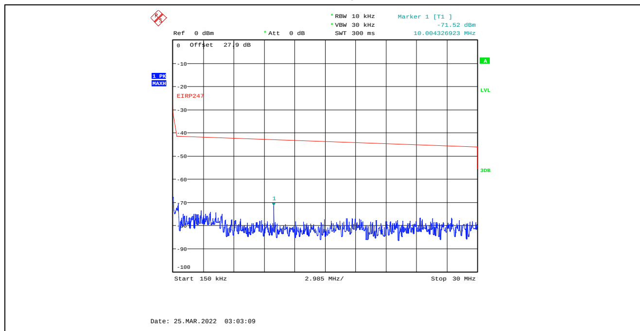
Plot C.3.4. Conducted Spurious Emissions in Restricted Frequency Bands, Chain 2 4 MHz Channel Bandwidth, Data Rate 3, Raw Power Setting 8, 2402 MHz, 150 kHz – 30 MHz, Peak Detector
