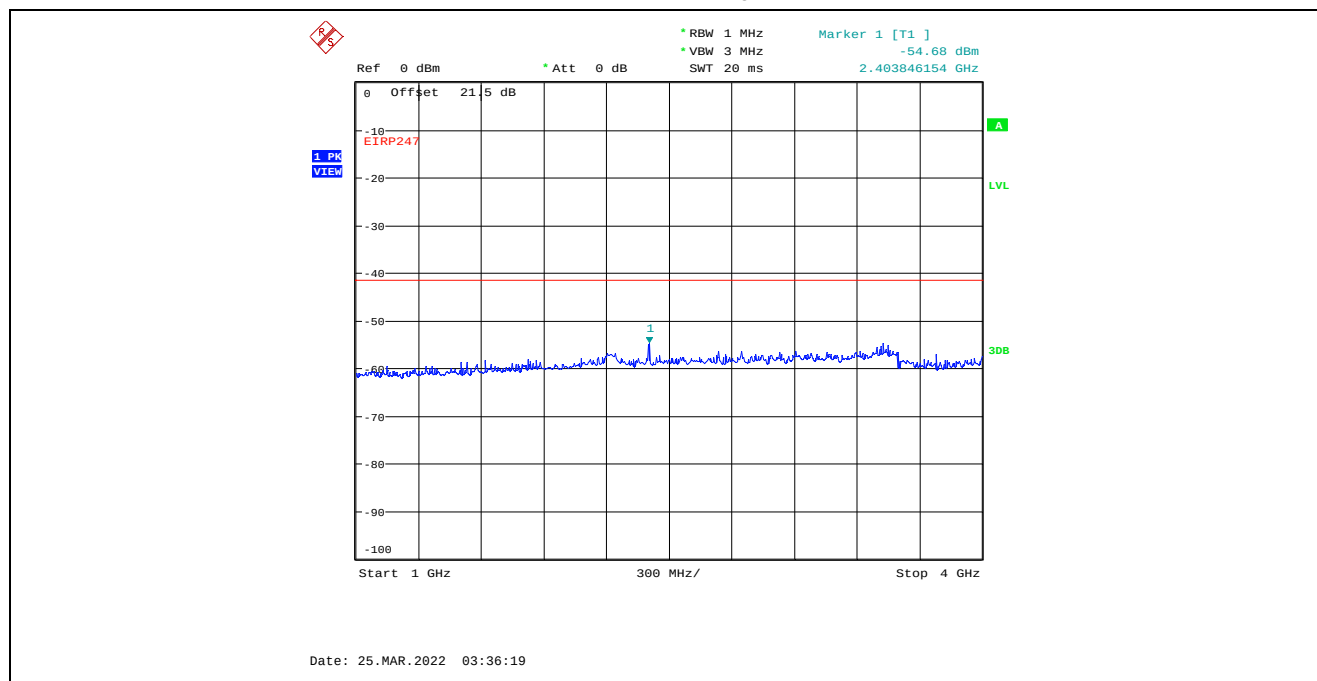
Plot C.3.8. Conducted Spurious Emissions in Restricted Frequency Bands, Chain 1 4 MHz Channel Bandwidth, Data Rate 3, Raw Power Setting 8, 2402 MHz, 1 GHz - 4 GHz, Peak Detector
