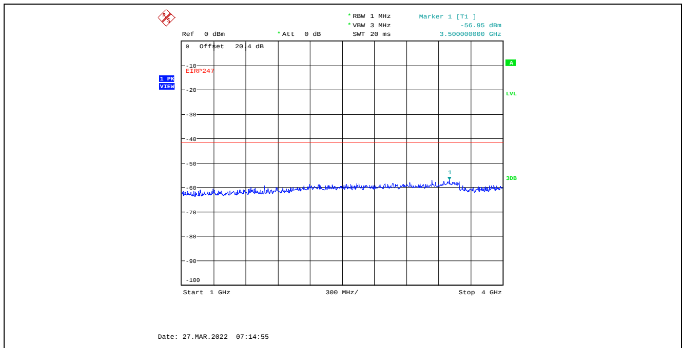
Plot C.4.37. Conducted Spurious Emissions in Restricted Frequency Bands, Chain 1 8 MHz Channel Bandwidth, Data Rate 7, Raw Power Setting 0, 2407 MHz, 1 GHz – 4 GHz, Peak Detector
