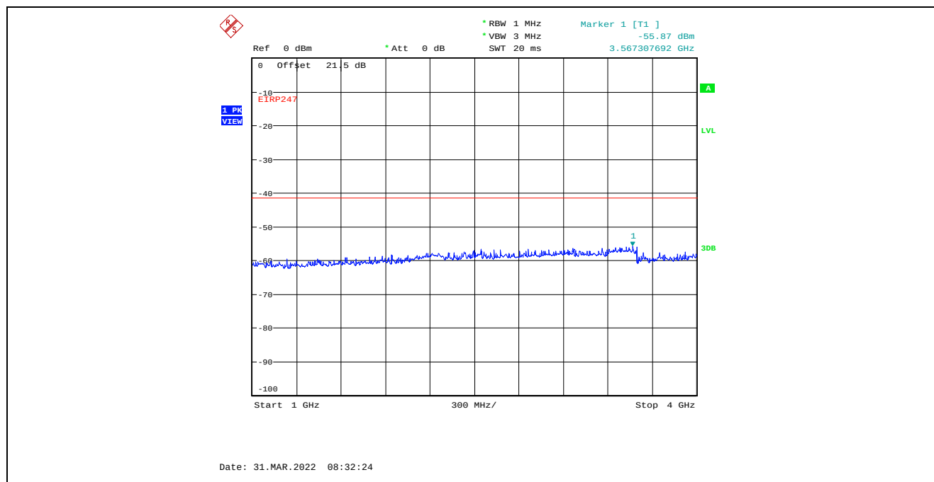
Plot C.3.98. Conducted Spurious Emissions in Restricted Frequency Bands, Chain 2 40 MHz Channel Bandwidth, Data Rate 3, Raw Power Setting 0, 2422 MHz, 1 GHz – 4 GHz, Peak Detector
