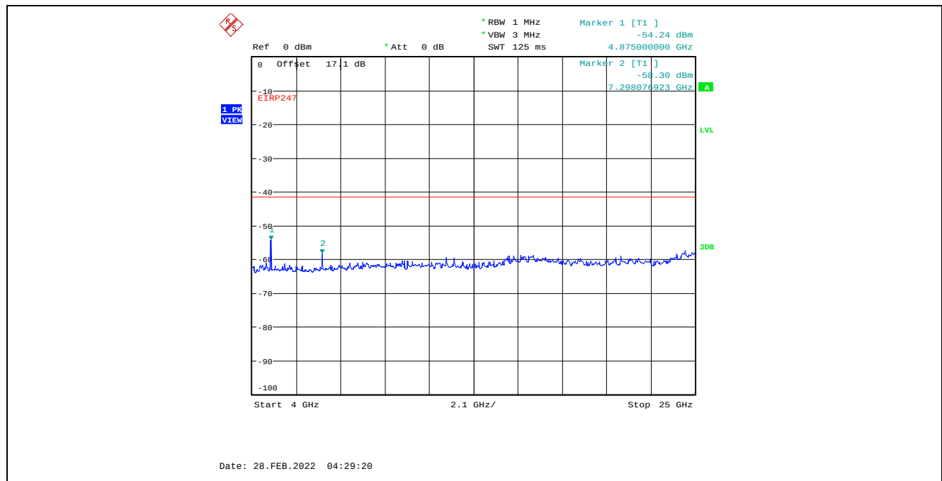
Plot C.2.50. Conducted Spurious Emissions in Restricted Frequency Bands, Chain 2 8 MHz Channel Bandwidth, Data Rate 7, Raw Power Setting 23, 2437 MHz, 4 GHz - 25 GHz, Peak Detector
