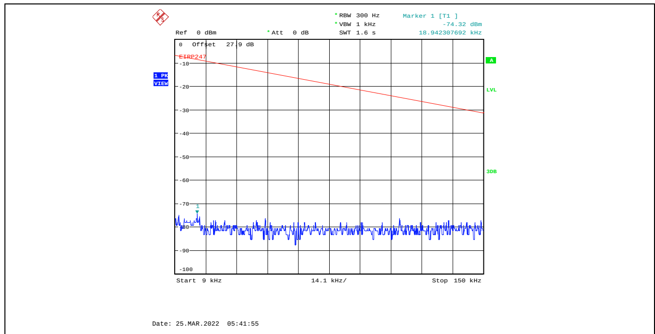
Plot C.4.22. Conducted Spurious Emissions in Restricted Frequency Bands, Chain 2 4 MHz Channel Bandwidth, Data Rate 7, Raw Power Setting 0, 2477 MHz, 9 kHz - 150 kHz, Peak Detector
