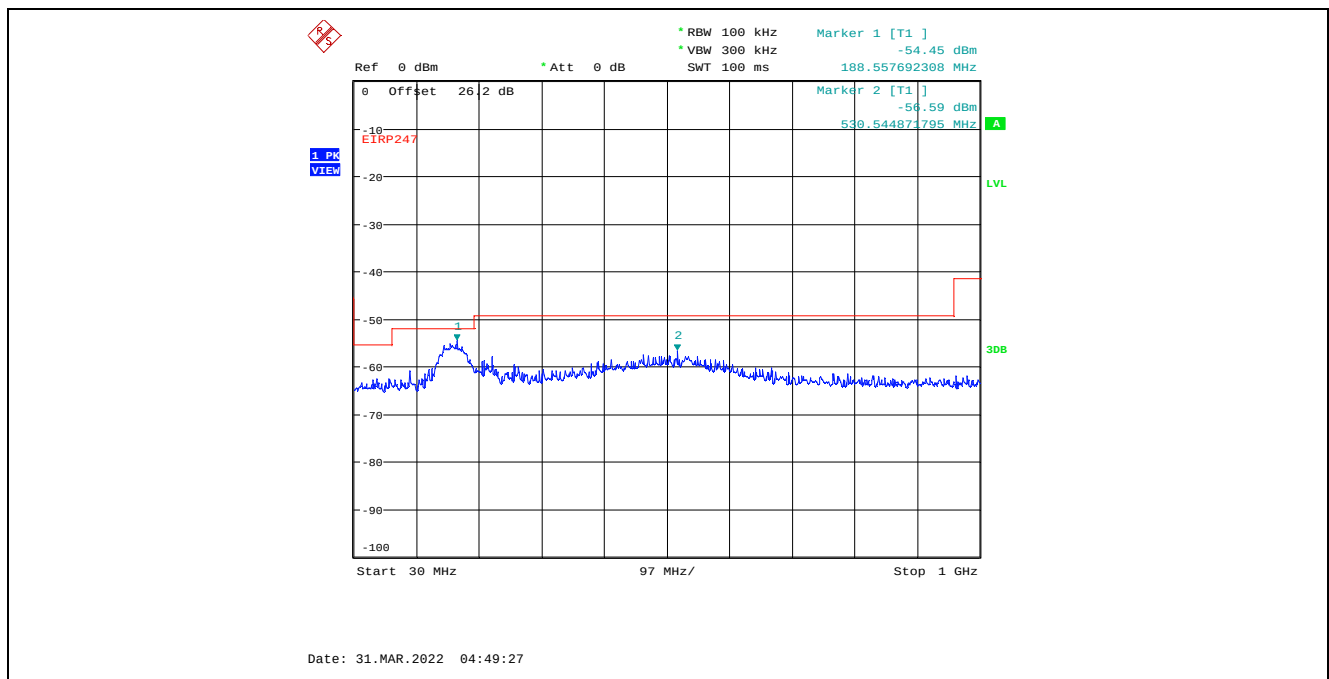
Plot C.4.106. Conducted Spurious Emissions in Restricted Frequency Bands, Chain 2 40 MHz Channel Bandwidth, Data Rate 7, Raw Power Setting 0, 2437 MHz, 30 MHz - 1 GHz, Peak Detector
