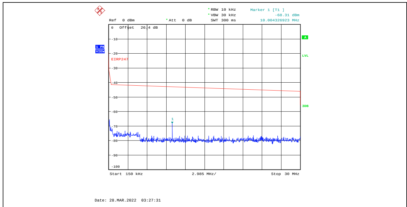
Plot C.4.33. Conducted Spurious Emissions in Restricted Frequency Bands, Chain 1 8 MHz Channel Bandwidth, Data Rate 7, Raw Power Setting 0, 2407 MHz, 150 kHz – 30 MHz, Peak Detector
