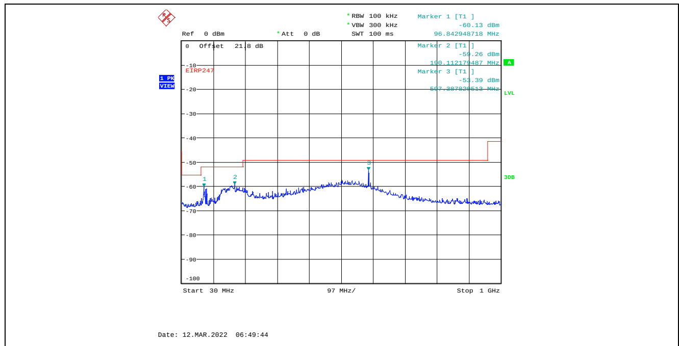
Plot C.1.65. Conducted Spurious Emissions in Restricted Frequency Bands, Chain 1 20 MHz Channel Bandwidth, Data Rate 3, Raw Power Setting 26, 2412 MHz, 30 MHz - 1 GHz, Peak Detector
