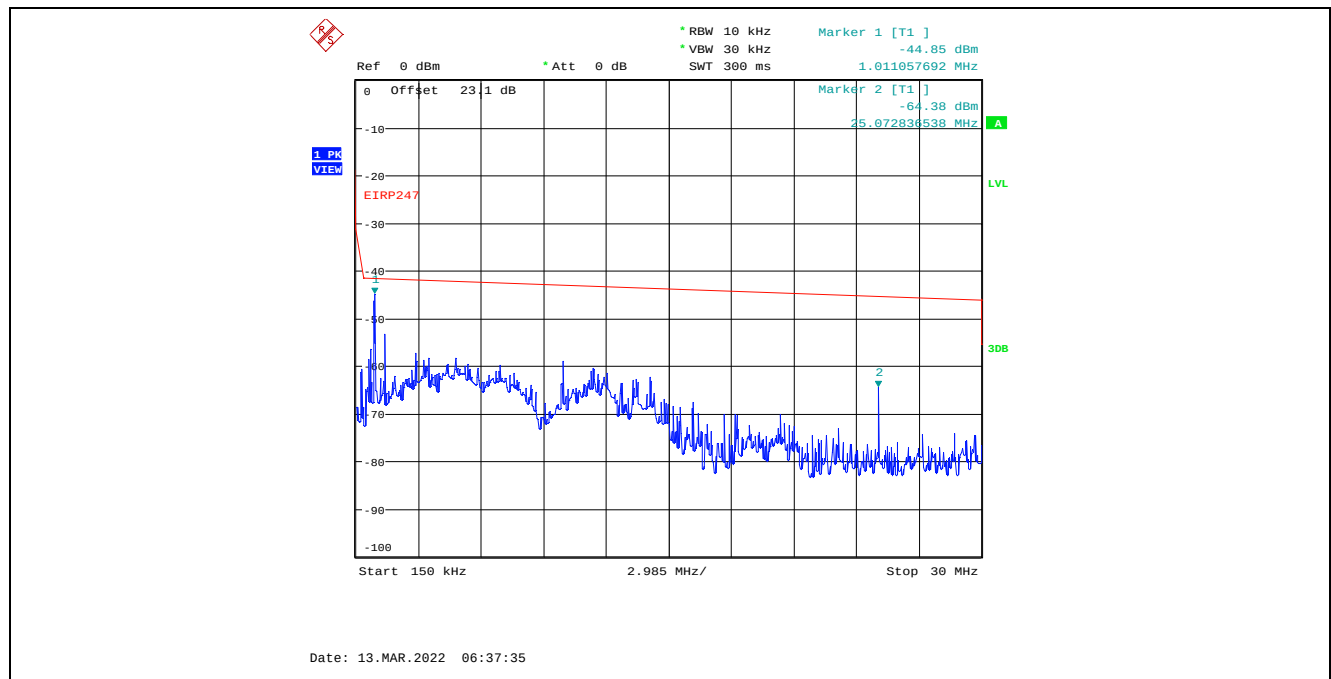
Plot C.2.84. Conducted Spurious Emissions in Restricted Frequency Bands, Chain 2 20 MHz Channel Bandwidth, Data Rate 7, Raw Power Setting 23, 2462 MHz, 150 kHz – 30 MHz, Peak Detector
