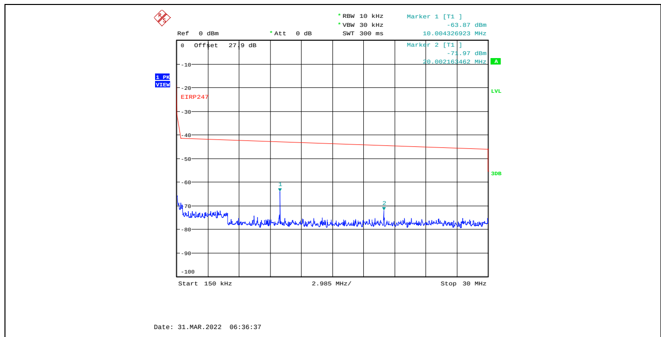
Plot C.4.114. Conducted Spurious Emissions in Restricted Frequency Bands, Chain 2 40 MHz Channel Bandwidth, Data Rate 7, Raw Power Setting 0, 2452 MHz, 150 kHz – 30 MHz, Peak Detector
