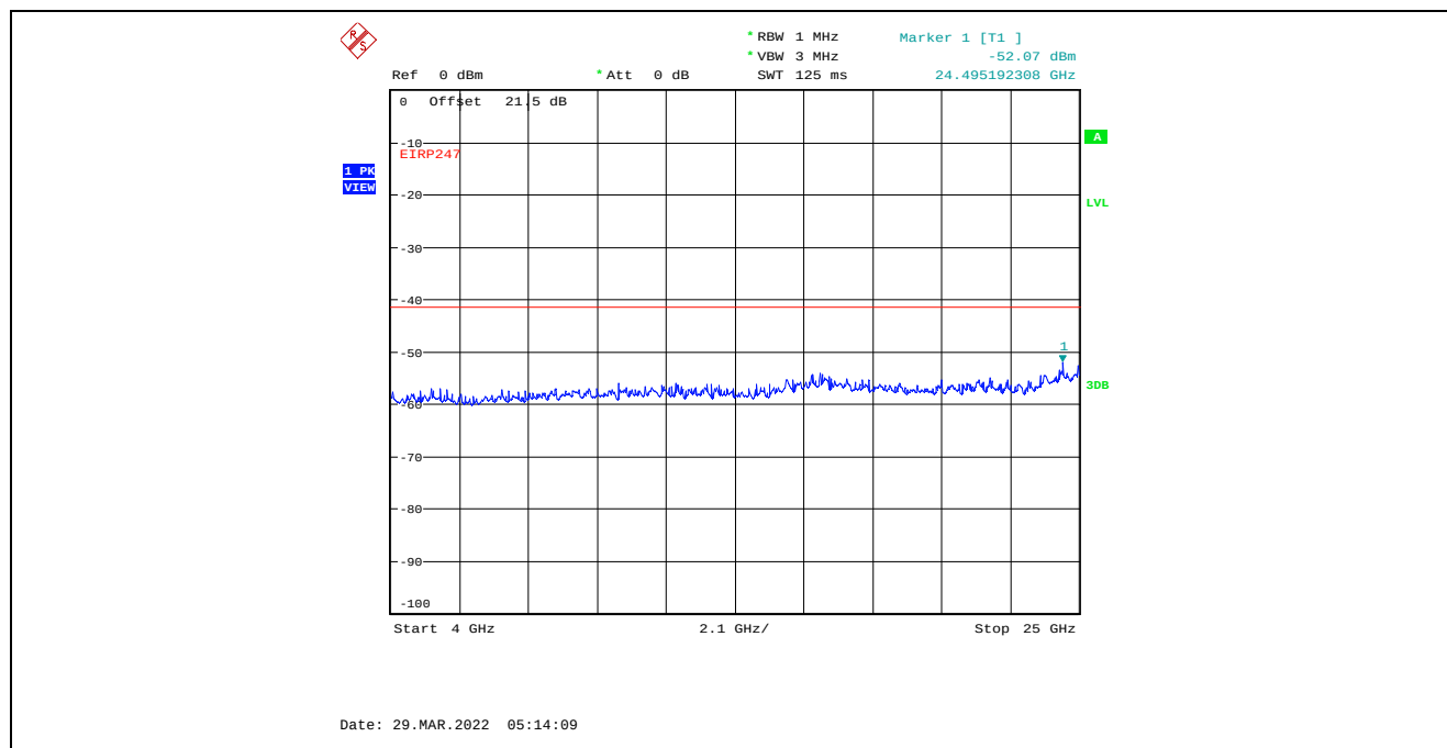
Plot C.3.79. Conducted Spurious Emissions in Restricted Frequency Bands, Chain 1 20 MHz Channel Bandwidth, Data Rate 3, Raw Power Setting 7, 2437 MHz, 4 GHz - 25 GHz, Peak Detector
