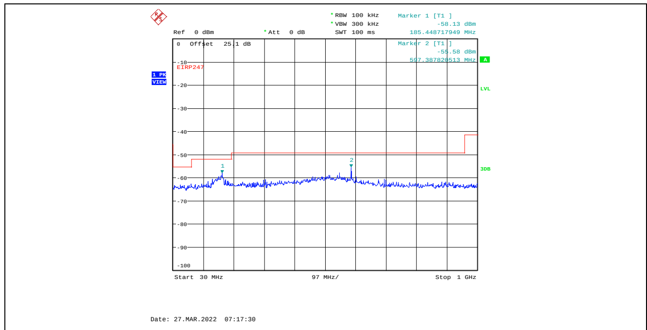
Plot C.4.35. Conducted Spurious Emissions in Restricted Frequency Bands, Chain 1 8 MHz Channel Bandwidth, Data Rate 7, Raw Power Setting 0, 2407 MHz, 30 MHz - 1 GHz, Peak Detector
