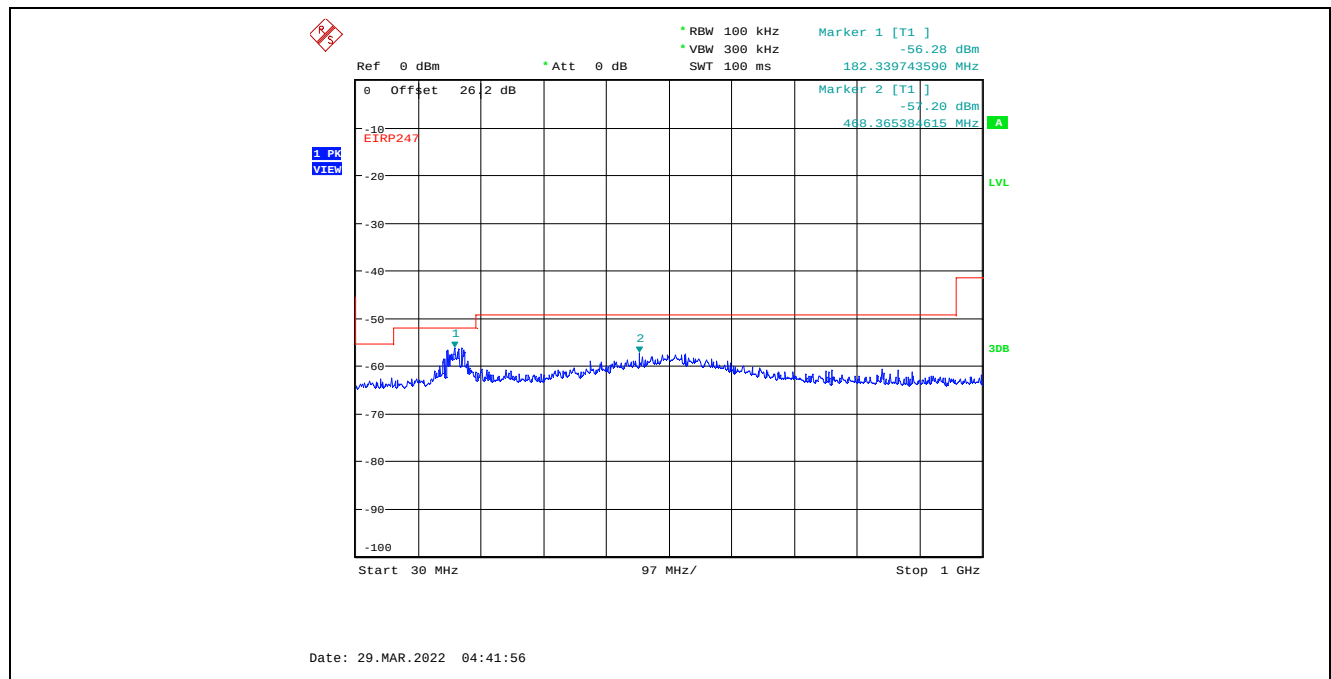
Plot C.3.86. Conducted Spurious Emissions in Restricted Frequency Bands, Chain 2 20 MHz Channel Bandwidth, Data Rate 3, Raw Power Setting 7, 2462 MHz, 30 MHz - 1 GHz, Peak Detector
