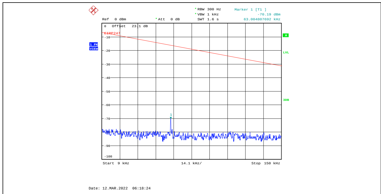
Plot C.1.82. Conducted Spurious Emissions in Restricted Frequency Bands, Chain 2 20 MHz Channel Bandwidth, Data Rate 3, Raw Power Setting 26, 2462 MHz, 9 kHz - 150 kHz, Peak Detector
