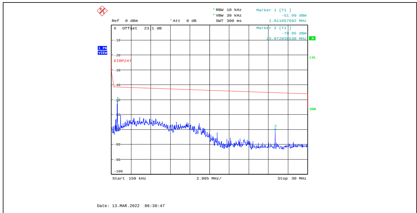
Plot C.2.63. Conducted Spurious Emissions in Restricted Frequency Bands, Chain 1 20 MHz Channel Bandwidth, Data Rate 7, Raw Power Setting 23, 2412 MHz, 150 kHz – 30 MHz, Peak Detector
