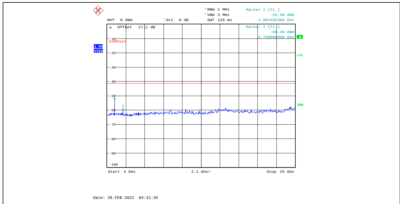
Plot C.2.40. Conducted Spurious Emissions in Restricted Frequency Bands, Chain 2 8 MHz Channel Bandwidth, Data Rate 7, Raw Power Setting 23, 2407 MHz, 4 GHz - 25 GHz, Peak Detector
