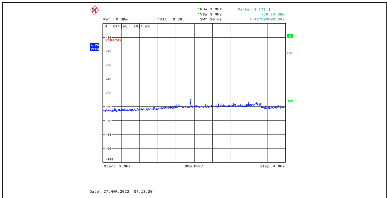
Plot C.4.47. Conducted Spurious Emissions in Restricted Frequency Bands, Chain 1 8 MHz Channel Bandwidth, Data Rate 7, Raw Power Setting 0, 2437 MHz, 1 GHz – 4 GHz, Peak Detector
