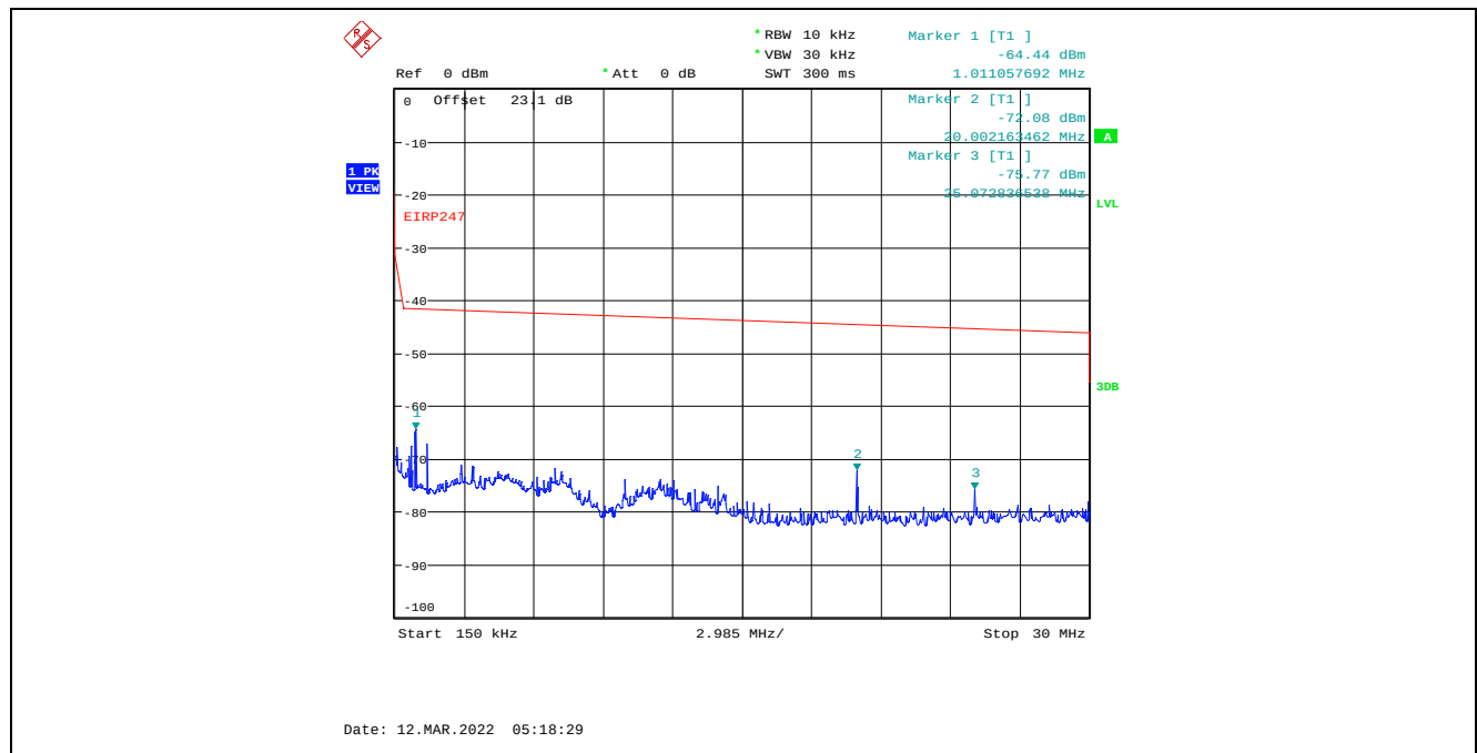
Plot C.2.104. Conducted Spurious Emissions in Restricted Frequency Bands, Chain 2 40 MHz Channel Bandwidth, Data Rate 7, Raw Power Setting 24, 2437 MHz, 150 kHz – 30 MHz, Peak Detector
