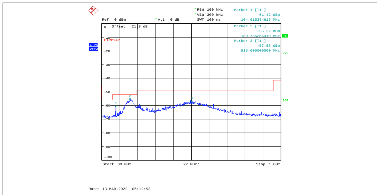
Plot C.2.66. Conducted Spurious Emissions in Restricted Frequency Bands, Chain 2 20 MHz Channel Bandwidth, Data Rate 7, Raw Power Setting 23, 2412 MHz, 30 MHz - 1 GHz, Peak Detector
