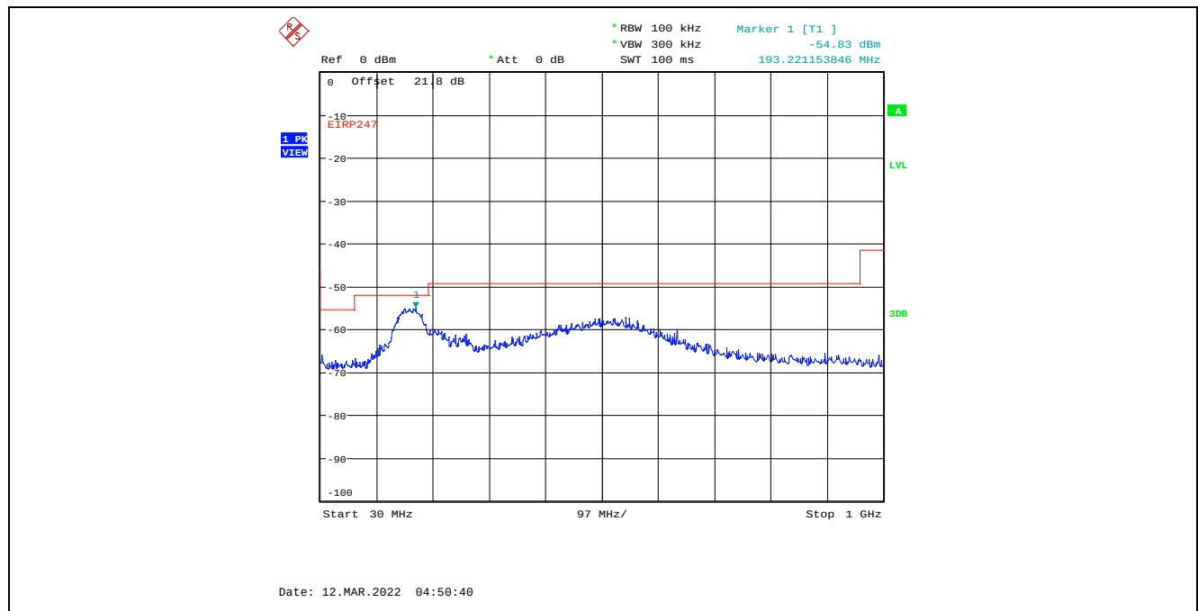
Plot C.2.106. Conducted Spurious Emissions in Restricted Frequency Bands, Chain 2 40 MHz Channel Bandwidth, Data Rate 7, Raw Power Setting 24, 2437 MHz, 30 MHz - 1 GHz, Peak Detector
