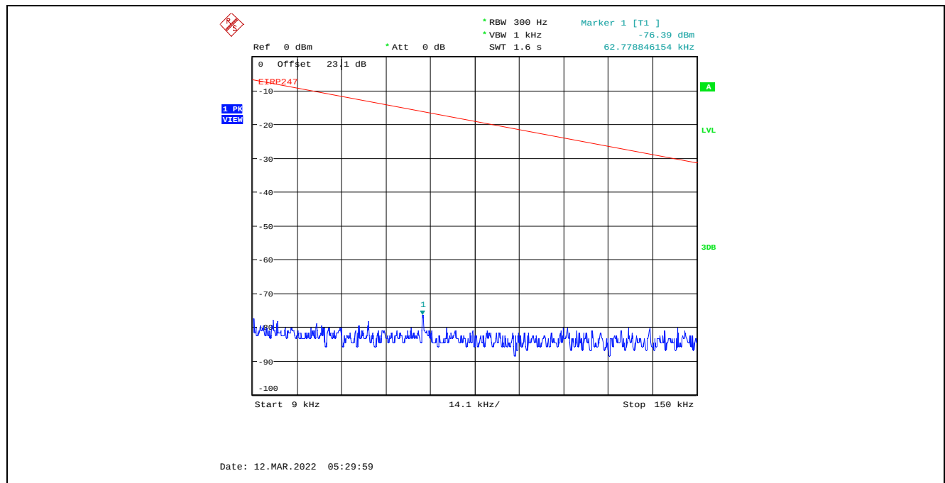
Plot C.2.111. Conducted Spurious Emissions in Restricted Frequency Bands, Chain 1 40 MHz Channel Bandwidth, Data Rate 7, Raw Power Setting 22, 2452 MHz, 9 kHz - 150 kHz, Peak Detector
