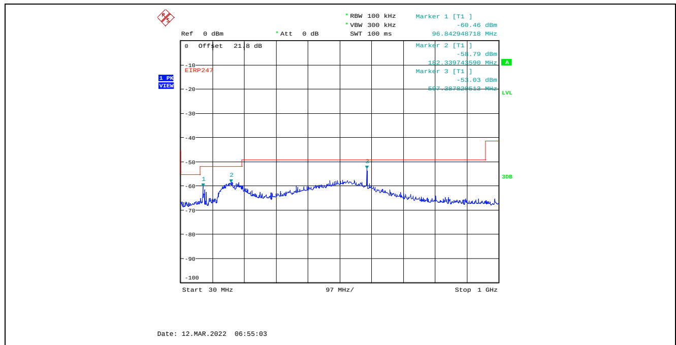
Plot C.1.85. Conducted Spurious Emissions in Restricted Frequency Bands, Chain 1 20 MHz Channel Bandwidth, Data Rate 3, Raw Power Setting 26, 2462 MHz, 30 MHz - 1 GHz, Peak Detector
