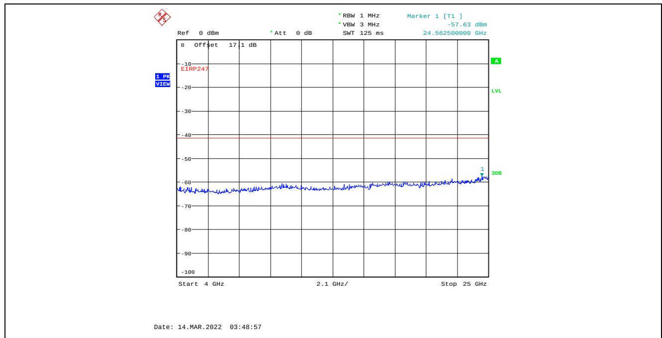
Plot C.1.59. Conducted Spurious Emissions in Restricted Frequency Bands, Chain 1 8 MHz Channel Bandwidth, Data Rate 3, Raw Power Setting 14, 2476 MHz, 4 GHz - 25 GHz, Peak Detector
