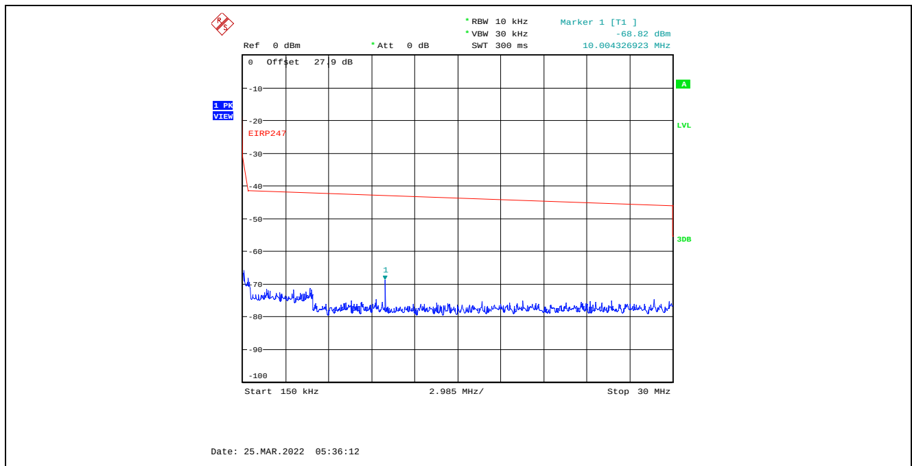
Plot C.4.14. Conducted Spurious Emissions in Restricted Frequency Bands, Chain 2 4 MHz Channel Bandwidth, Data Rate 7, Raw Power Setting 0, 2437 MHz, 150 kHz – 30 MHz, Peak Detector
