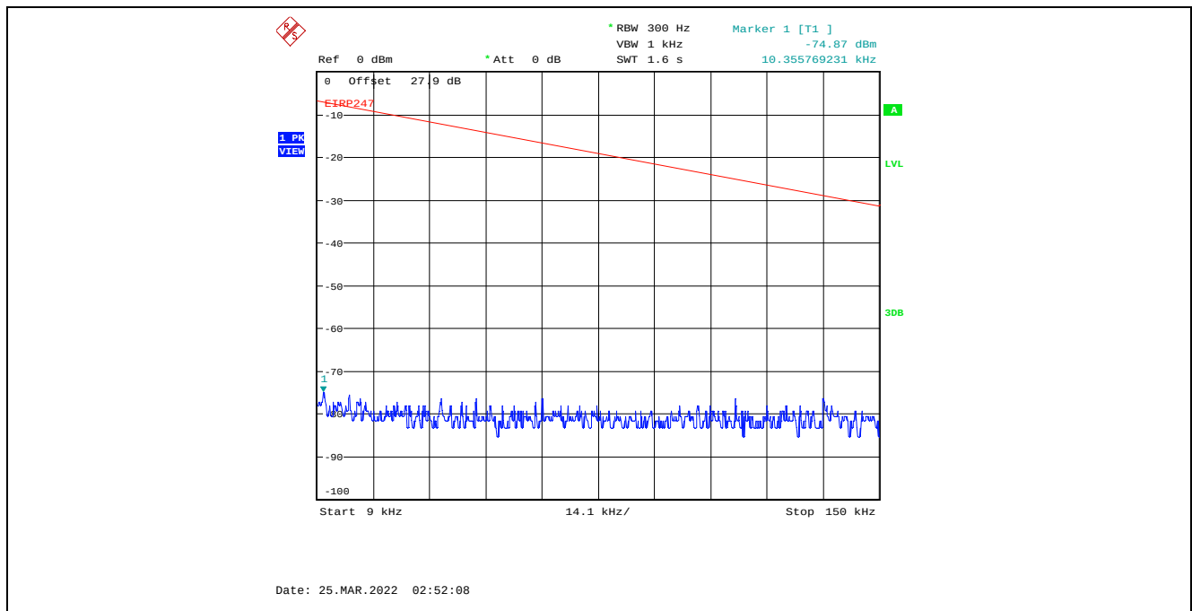
Plot C.3.21. Conducted Spurious Emissions in Restricted Frequency Bands, Chain 1 4 MHz Channel Bandwidth, Data Rate 3, Raw Power Setting 0, 2477 MHz, 9 kHz - 150 kHz, Peak Detector
