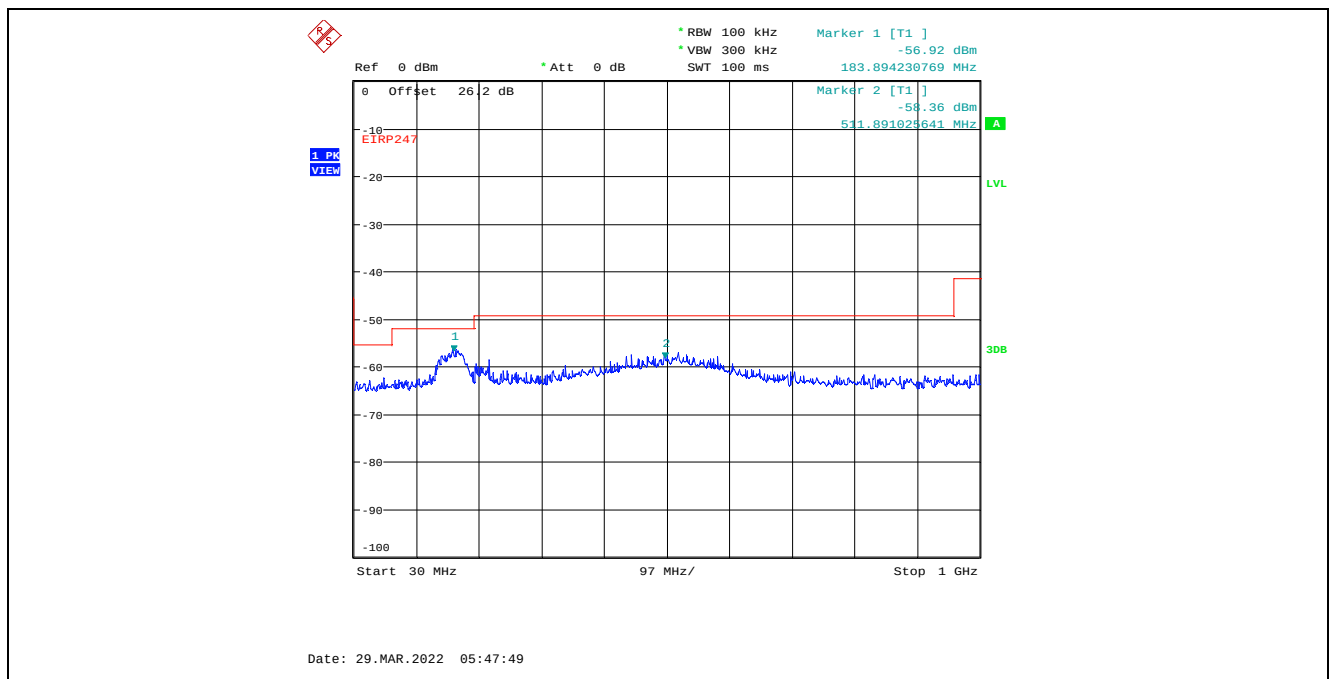
Plot C.4.76. Conducted Spurious Emissions in Restricted Frequency Bands, Chain 2 20 MHz Channel Bandwidth, Data Rate 7, Raw Power Setting 0, 2437 MHz, 30 MHz - 1 GHz, Peak Detector
