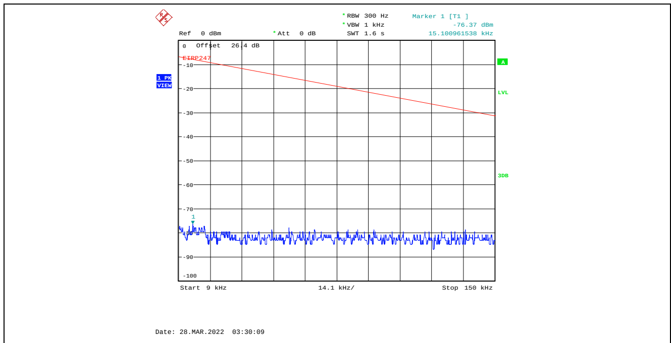
Plot C.4.31. Conducted Spurious Emissions in Restricted Frequency Bands, Chain 1 8 MHz Channel Bandwidth, Data Rate 7, Raw Power Setting 0, 2407 MHz, 9 kHz - 150 kHz, Peak Detector
