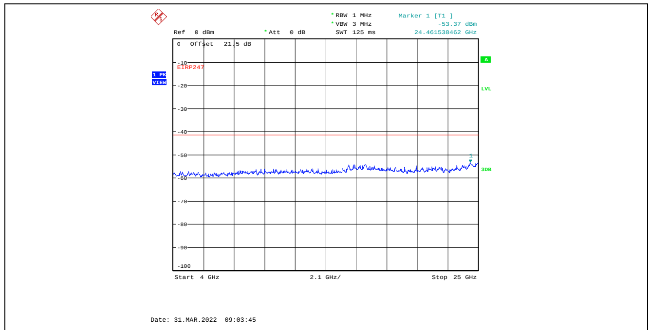
Plot C.3.110. Conducted Spurious Emissions in Restricted Frequency Bands, Chain 2 40 MHz Channel Bandwidth, Data Rate 3, Raw Power Setting 0, 2437 MHz, 4 GHz - 25 GHz, Peak Detector
