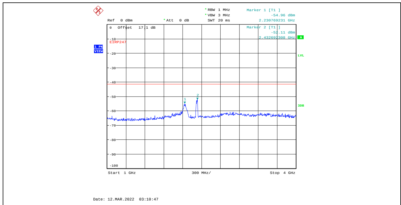
Plot C.1.98. Conducted Spurious Emissions in Restricted Frequency Bands, Chain 2 40 MHz Channel Bandwidth, Data Rate 3, Raw Power Setting 13, 2422 MHz, 1 GHz – 4 GHz, Peak Detector
