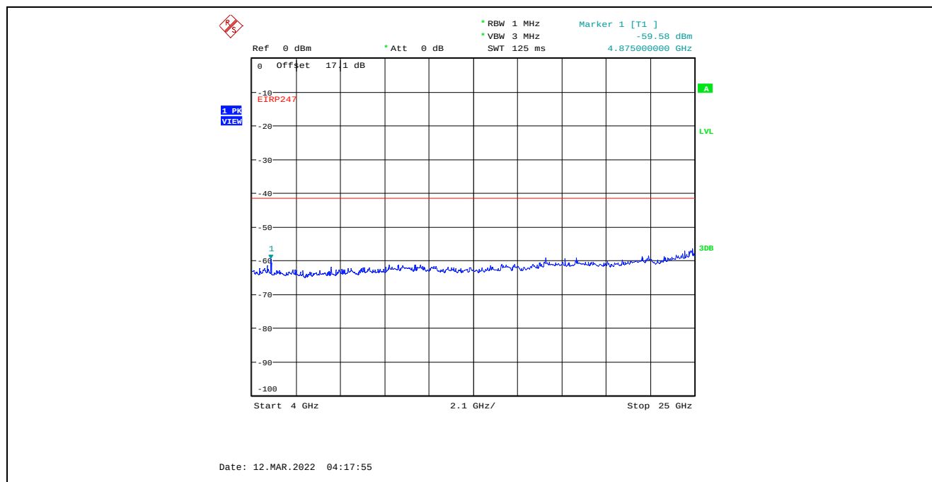
Plot C.2.120. Conducted Spurious Emissions in Restricted Frequency Bands, Chain 2 40 MHz Channel Bandwidth, Data Rate 7, Raw Power Setting 22, 2452 MHz, 4 GHz - 25 GHz, Peak Detector
