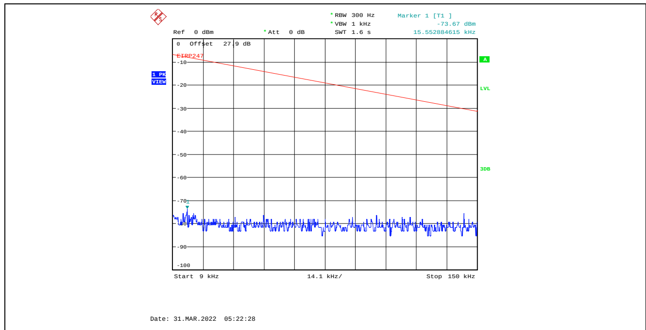
Plot C.3.91. Conducted Spurious Emissions in Restricted Frequency Bands, Chain 1 40 MHz Channel Bandwidth, Data Rate 3, Raw Power Setting 0, 2422 MHz, 9 kHz - 150 kHz, Peak Detector
