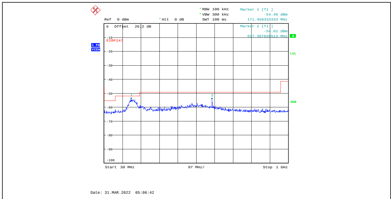
Plot C.4.105. Conducted Spurious Emissions in Restricted Frequency Bands, Chain 1 40 MHz Channel Bandwidth, Data Rate 7, Raw Power Setting 0, 2437 MHz, 30 MHz - 1 GHz, Peak Detector
