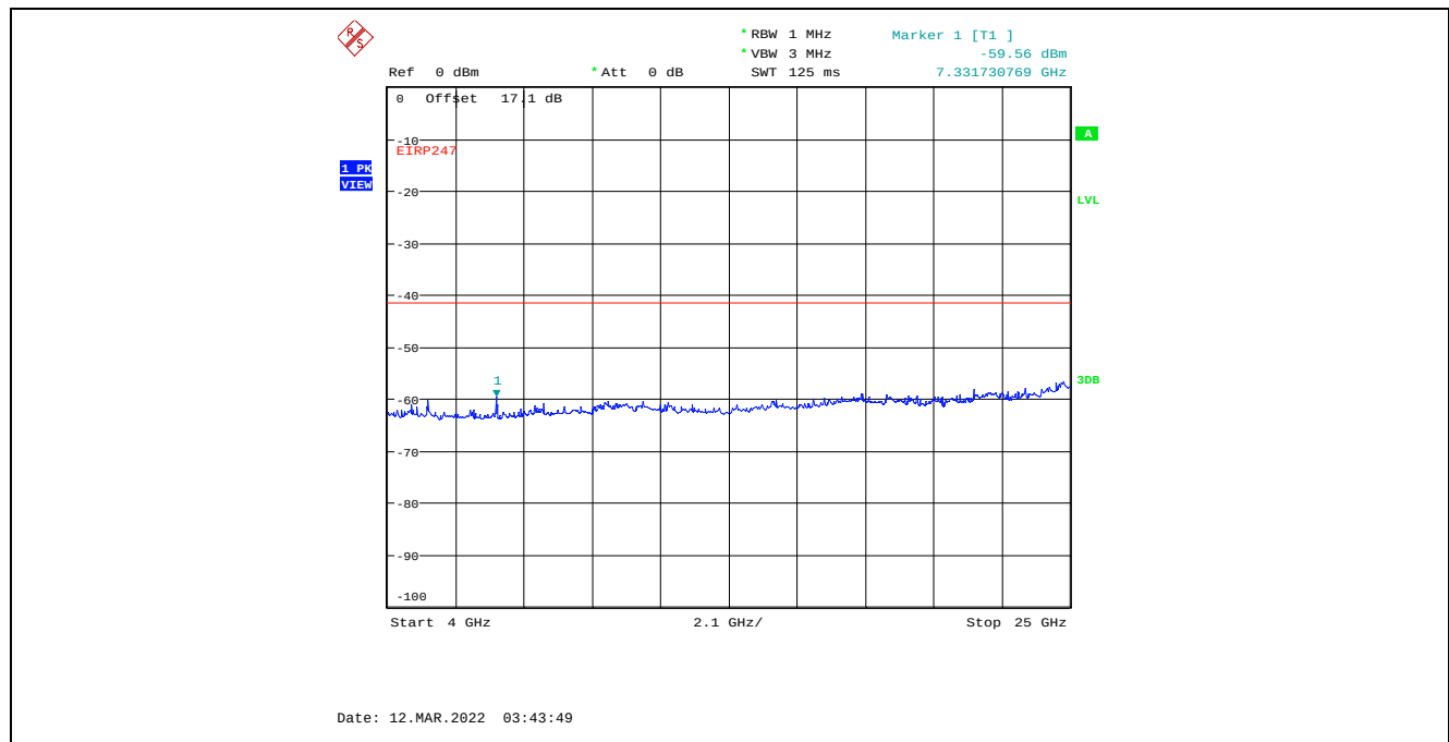
Plot C.1.119. Conducted Spurious Emissions in Restricted Frequency Bands, Chain 1 40 MHz Channel Bandwidth, Data Rate 3, Raw Power Setting 15, 2452 MHz, 4 GHz - 25 GHz, Peak Detector
