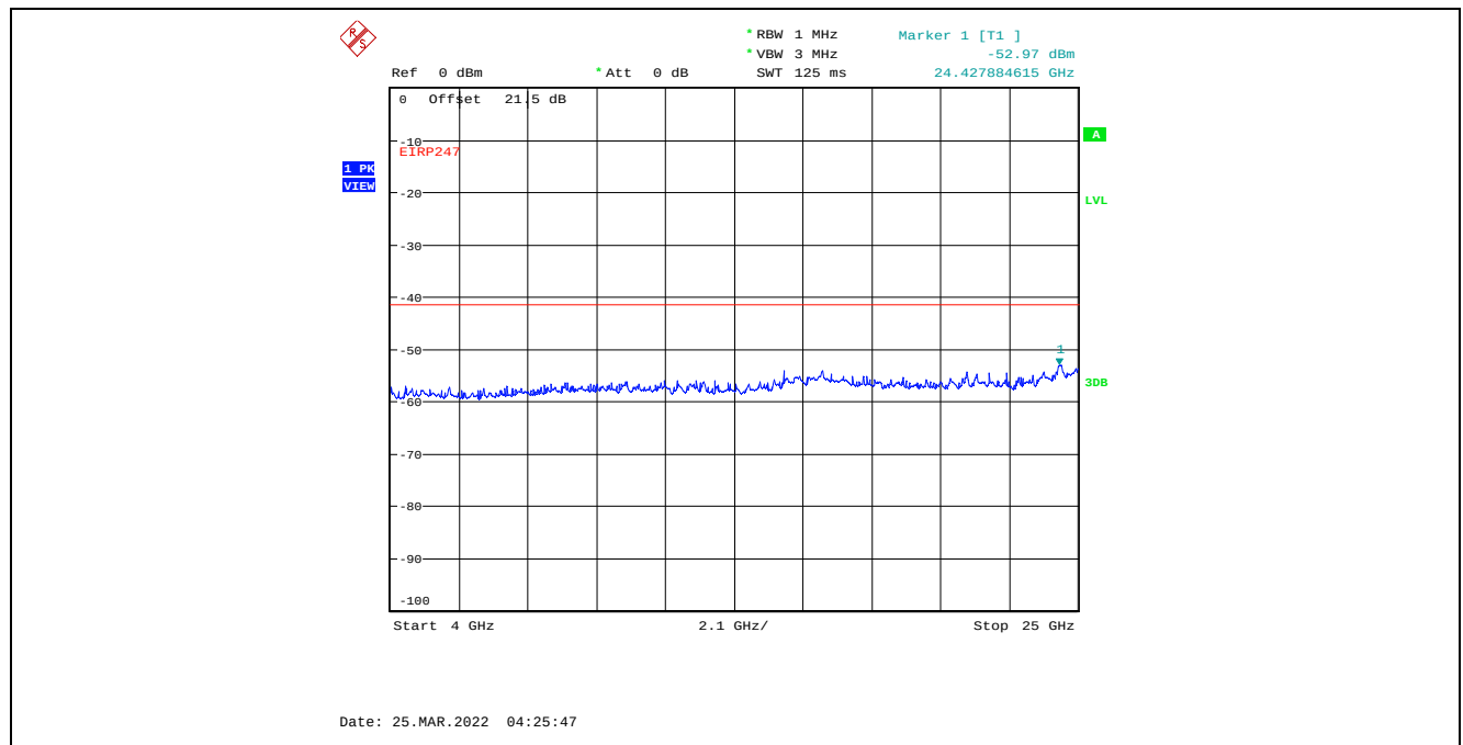
Plot C.4.30. Conducted Spurious Emissions in Restricted Frequency Bands, Chain 2 4 MHz Channel Bandwidth, Data Rate 7, Raw Power Setting 0, 2477 MHz, 4 GHz - 25 GHz, Peak Detector
