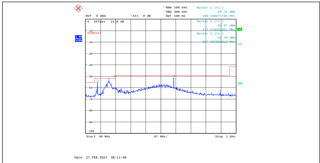
Plot C.2.45. Conducted Spurious Emissions in Restricted Frequency Bands, Chain 1 8 MHz Channel Bandwidth, Data Rate 7, Raw Power Setting 23, 2437 MHz, 30 MHz - 1 GHz, Peak Detector
