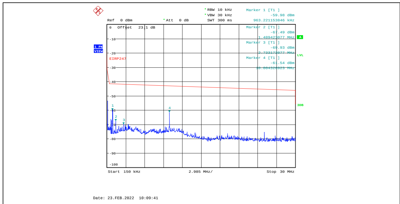
Plot C.1.14. Conducted Spurious Emissions in Restricted Frequency Bands, Chain 2 4 MHz Channel Bandwidth, Data Rate 3, Raw Power Setting 16, 2437 MHz, 150 kHz – 30 MHz, Peak Detector
