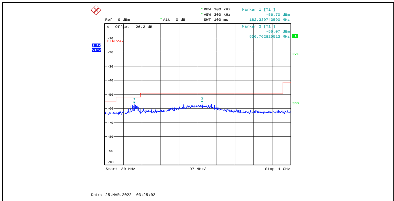
Plot C.3.26. Conducted Spurious Emissions in Restricted Frequency Bands, Chain 2 4 MHz Channel Bandwidth, Data Rate 3, Raw Power Setting 0, 2477 MHz, 30 MHz - 1 GHz, Peak Detector
