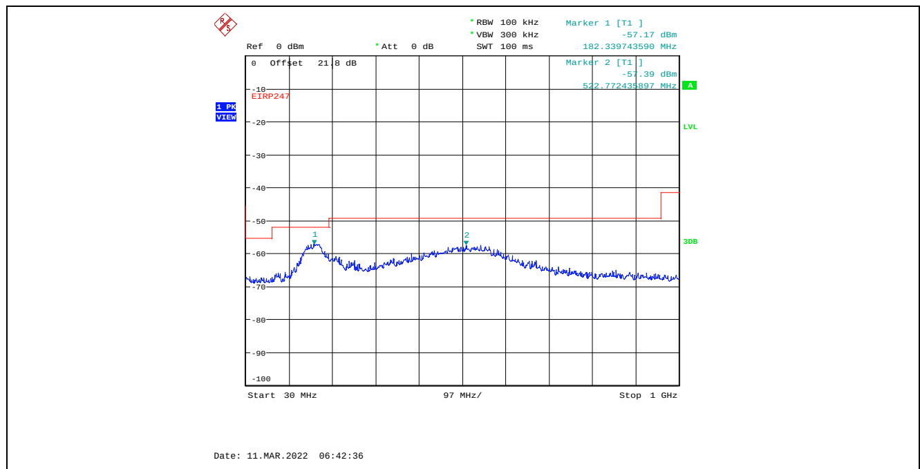
Plot C.1.96. Conducted Spurious Emissions in Restricted Frequency Bands, Chain 2 40 MHz Channel Bandwidth, Data Rate 3, Raw Power Setting 13, 2422 MHz, 30 MHz - 1 GHz, Peak Detector
