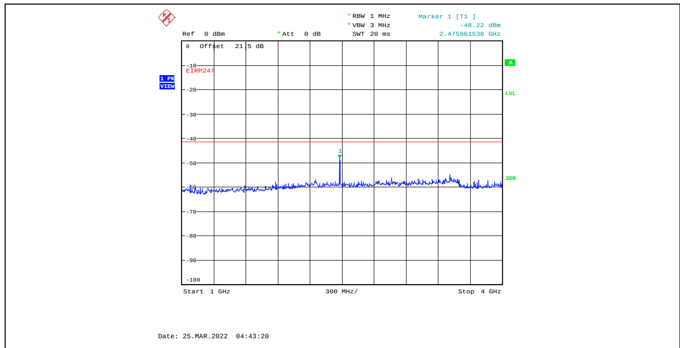
Plot C.4.27. Conducted Spurious Emissions in Restricted Frequency Bands, Chain 1 4 MHz Channel Bandwidth, Data Rate 7, Raw Power Setting 0, 2477 MHz, 1 GHz – 4 GHz, Peak Detector
