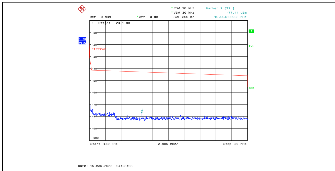
Plot C.1.24. Conducted Spurious Emissions in Restricted Frequency Bands, Chain 2 4 MHz Channel Bandwidth, Data Rate 3, Raw Power Setting 13, 2477 MHz, 150 kHz – 30 MHz, Peak Detector
