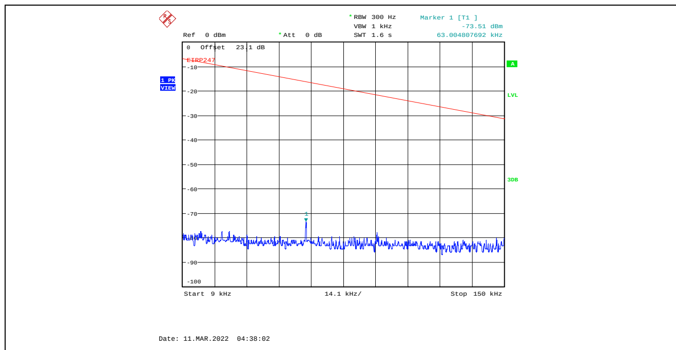
Plot C.1.91. Conducted Spurious Emissions in Restricted Frequency Bands, Chain 1 40 MHz Channel Bandwidth, Data Rate 3, Raw Power Setting 13, 2422 MHz, 9 kHz - 150 kHz, Peak Detector
