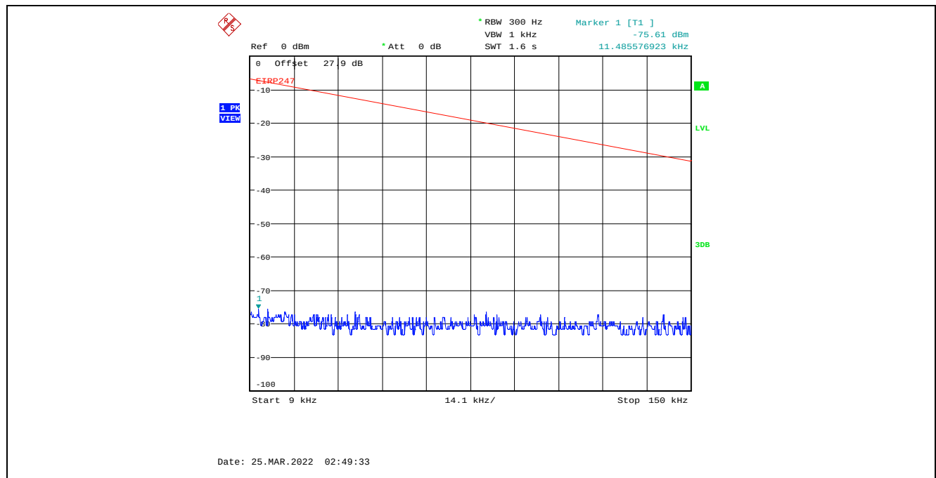
Plot C.3.11. Conducted Spurious Emissions in Restricted Frequency Bands, Chain 1 4 MHz Channel Bandwidth, Data Rate 3, Raw Power Setting 8, 2437 MHz, 9 kHz - 150 kHz, Peak Detector
