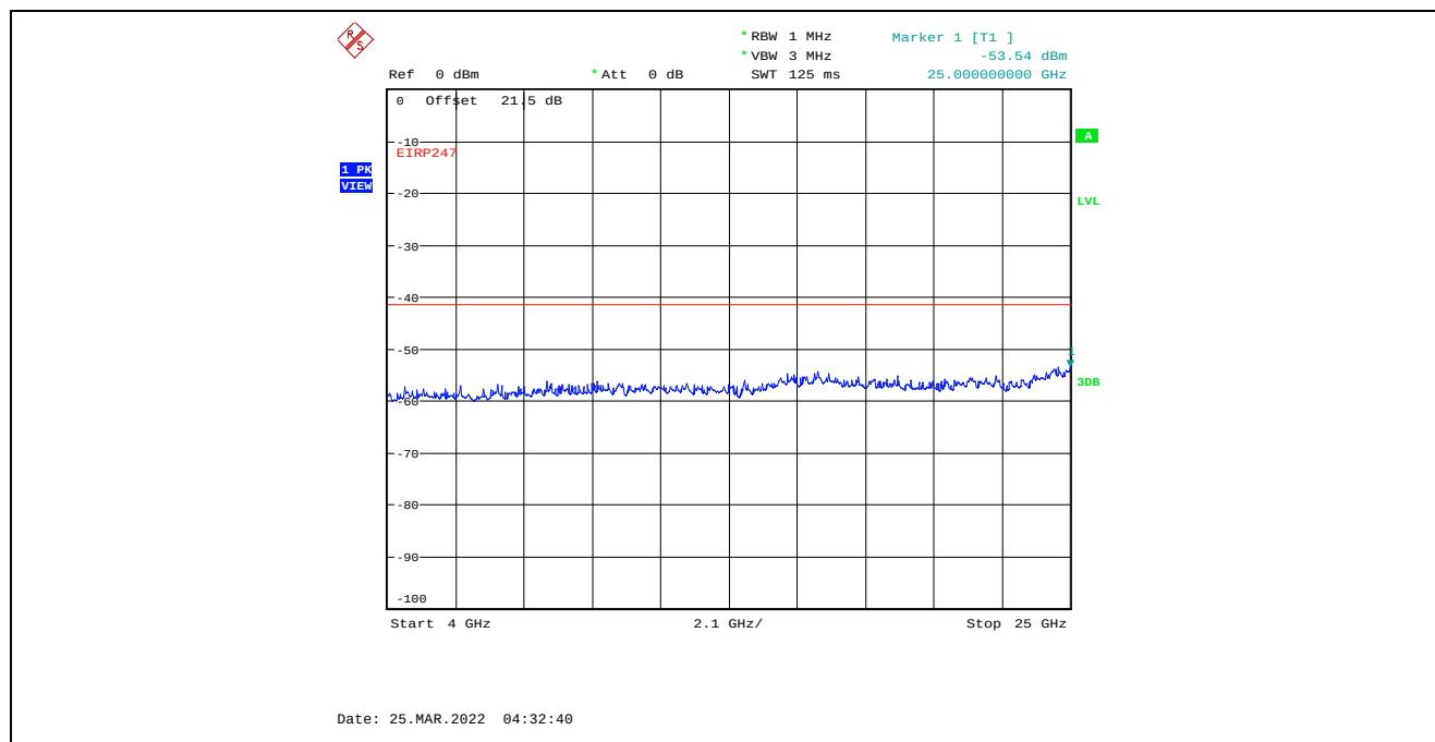
Plot C.4.9. Conducted Spurious Emissions in Restricted Frequency Bands, Chain 2 4 MHz Channel Bandwidth, Data Rate 7, Raw Power Setting 0, 2405 MHz, 4 GHz - 25 GHz, Peak Detector
