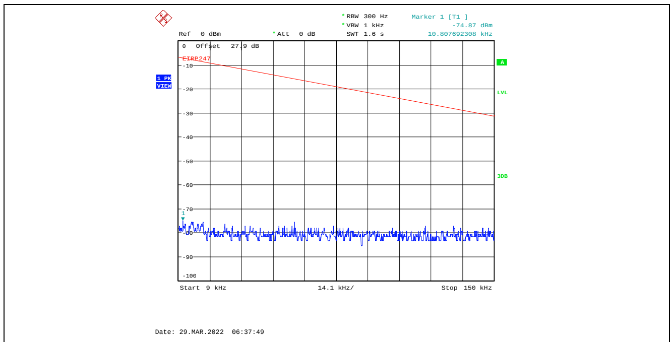
Plot C.4.62. Conducted Spurious Emissions in Restricted Frequency Bands, Chain 2 20 MHz Channel Bandwidth, Data Rate 7, Raw Power Setting 0, 2412 MHz, 9 kHz - 150 kHz, Peak Detector
