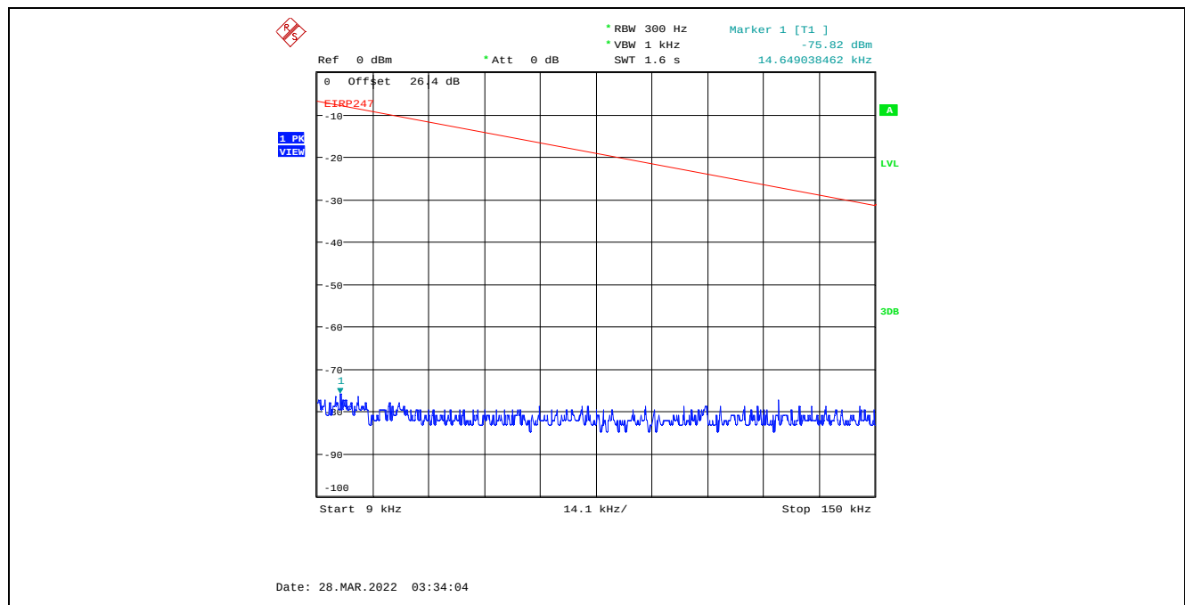
Plot C.4.52. Conducted Spurious Emissions in Restricted Frequency Bands, Chain 2 8 MHz Channel Bandwidth, Data Rate 7, Raw Power Setting 0, 2476 MHz, 9 kHz - 150 kHz, Peak Detector
