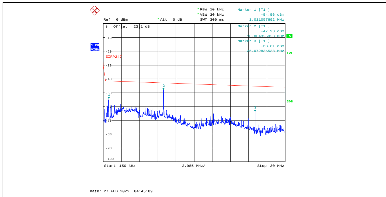
Plot C.1.34. Conducted Spurious Emissions in Restricted Frequency Bands, Chain 2 8 MHz Channel Bandwidth, Data Rate 3, Raw Power Setting 21, 2407 MHz, 150 kHz – 30 MHz, Peak Detector
