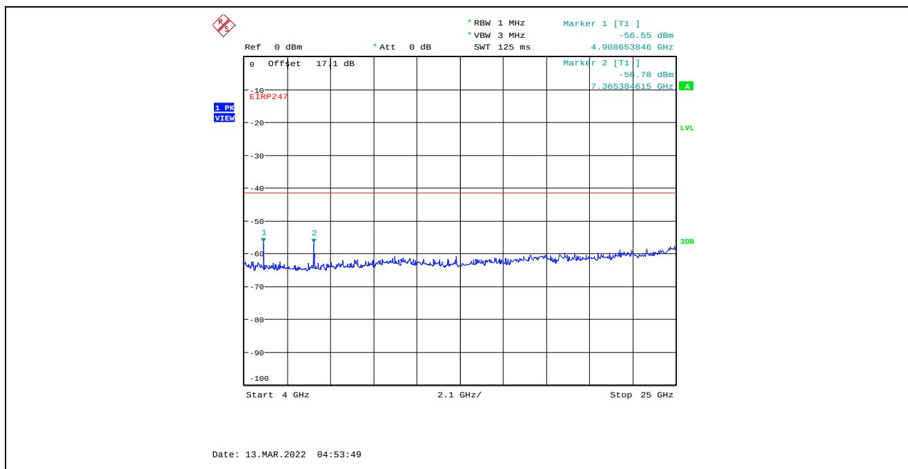
Plot C.2.90. Conducted Spurious Emissions in Restricted Frequency Bands, Chain 2 20 MHz Channel Bandwidth, Data Rate 7, Raw Power Setting 23, 2462 MHz, 4 GHz - 25 GHz, Peak Detector
