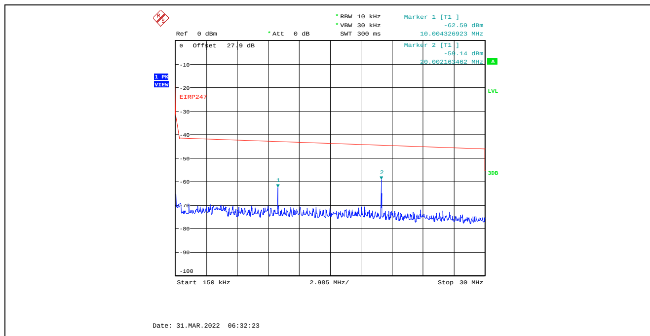
Plot C.3.114. Conducted Spurious Emissions in Restricted Frequency Bands, Chain 2 40 MHz Channel Bandwidth, Data Rate 3, Raw Power Setting 0, 2452 MHz, 150 kHz – 30 MHz, Peak Detector
