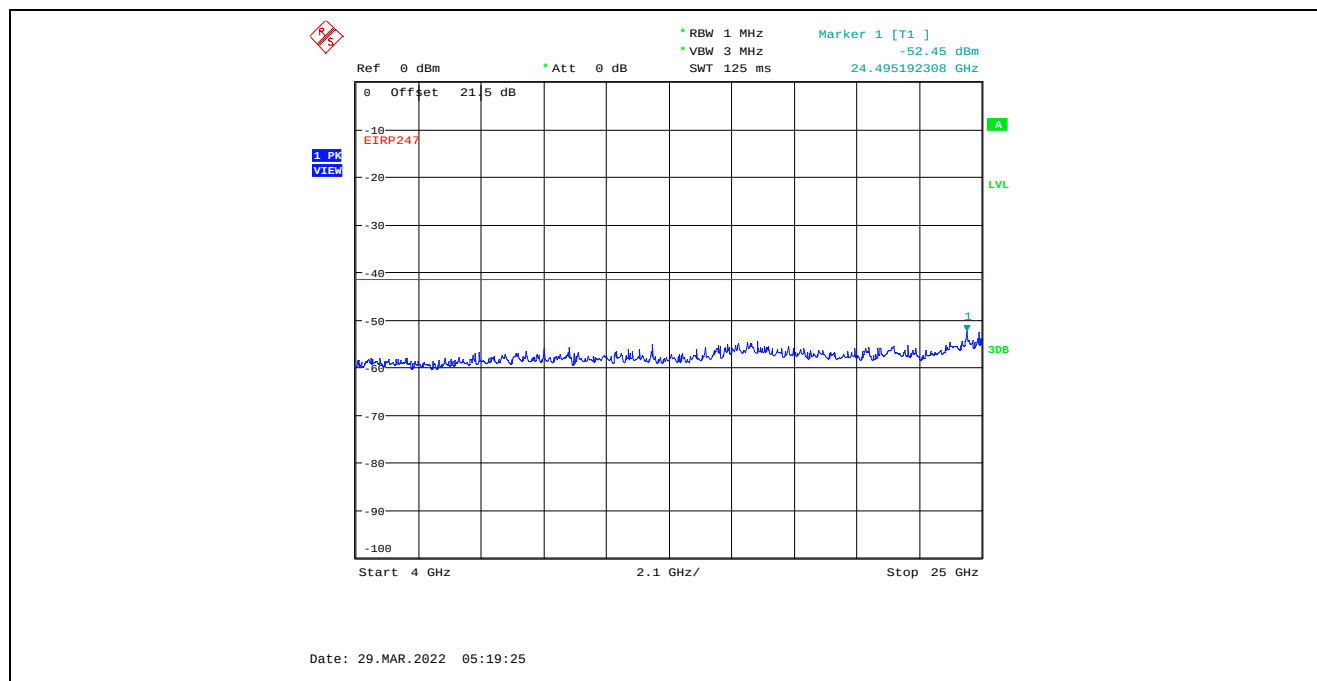
Plot C.4.79. Conducted Spurious Emissions in Restricted Frequency Bands, Chain 1 20 MHz Channel Bandwidth, Data Rate 7, Raw Power Setting 0, 2437 MHz, 4 GHz - 25 GHz, Peak Detector
