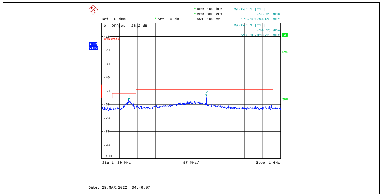
Plot C.3.85. Conducted Spurious Emissions in Restricted Frequency Bands, Chain 1 20 MHz Channel Bandwidth, Data Rate 3, Raw Power Setting 7, 2462 MHz, 30 MHz - 1 GHz, Peak Detector
