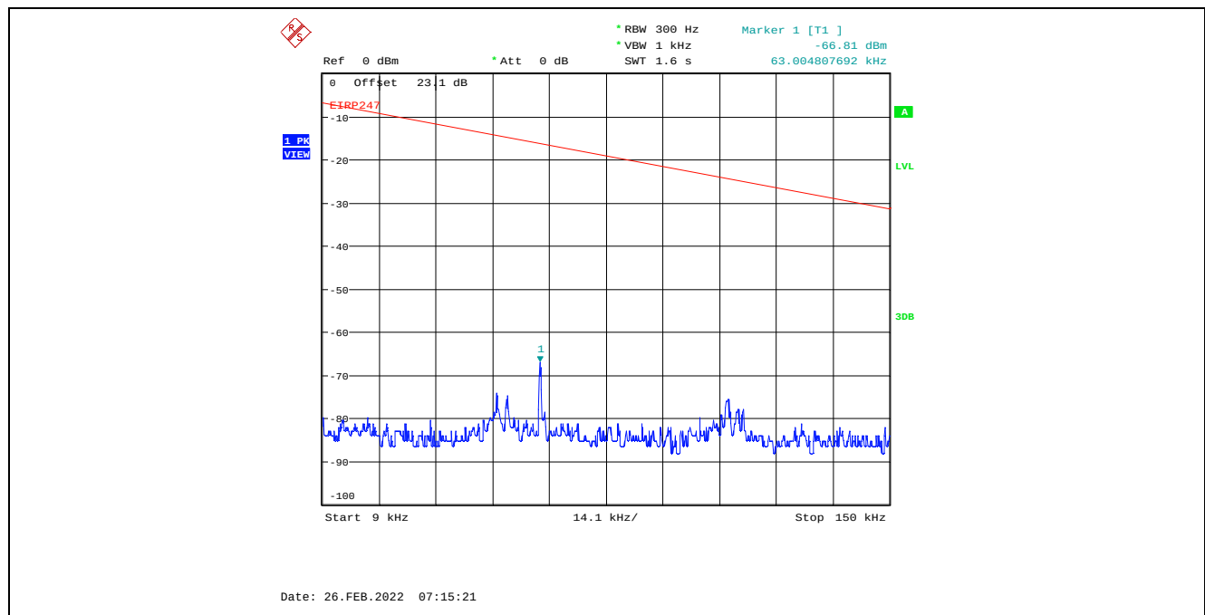
Plot C.2.12. Conducted Spurious Emissions in Restricted Frequency Bands, Chain 2 4 MHz Channel Bandwidth, Data Rate 7, Raw Power Setting 22, 2437 MHz, 9 kHz - 150 kHz, Peak Detector
