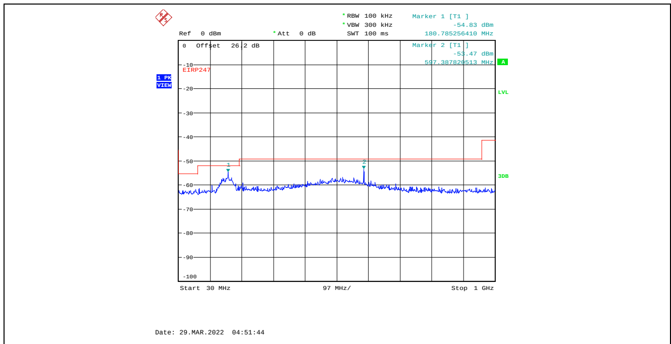
Plot C.3.65. Conducted Spurious Emissions in Restricted Frequency Bands, Chain 1 20 MHz Channel Bandwidth, Data Rate 3, Raw Power Setting 7, 2412 MHz, 30 MHz - 1 GHz, Peak Detector
