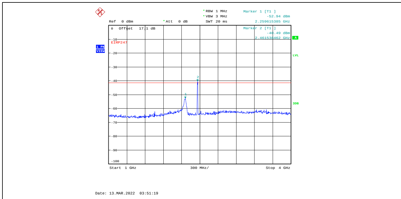
Plot C.1.88. Conducted Spurious Emissions in Restricted Frequency Bands, Chain 2 820 MHz Channel Bandwidth, Data Rate 3, Raw Power Setting 26, 2462 MHz, 1 GHz – 4 GHz, Peak Detector Marker 2 is Fundamental Signal
