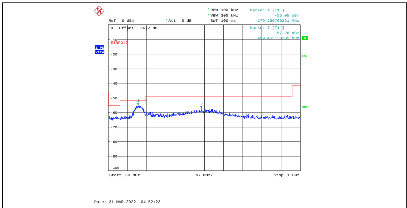
Plot C.4.96. Conducted Spurious Emissions in Restricted Frequency Bands, Chain 1 40 MHz Channel Bandwidth, Data Rate 7, Raw Power Setting 0, 2422 MHz, 30 MHz - 1 GHz, Peak Detector
