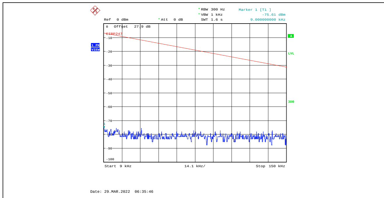
Plot C.4.82. Conducted Spurious Emissions in Restricted Frequency Bands, Chain 2 20 MHz Channel Bandwidth, Data Rate 7, Raw Power Setting 0, 2462 MHz, 9 kHz - 150 kHz, Peak Detector
