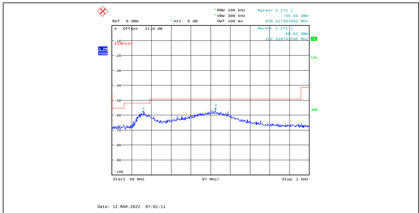
Plot C.1.76. Conducted Spurious Emissions in Restricted Frequency Bands, Chain 2 20 MHz Channel Bandwidth, Data Rate 3, Raw Power Setting 26, 2437 MHz, 30 MHz - 1 GHz, Peak Detector
