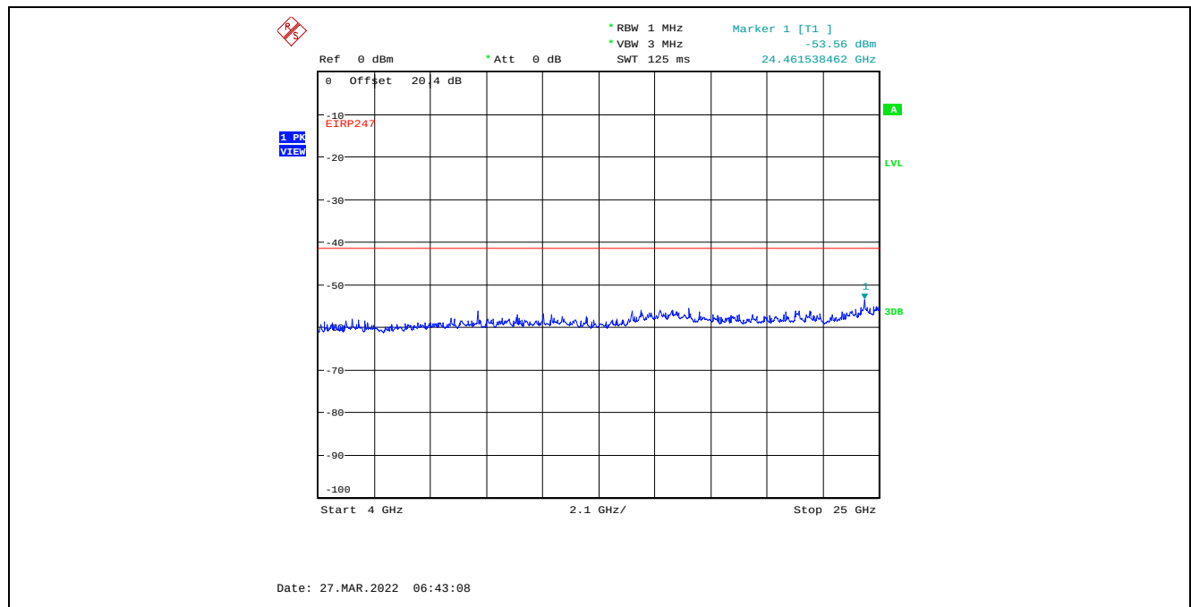
Plot C.3.50. Conducted Spurious Emissions in Restricted Frequency Bands, Chain 2 8 MHz Channel Bandwidth, Data Rate 3, Raw Power Setting 6, 2437 MHz, 4 GHz - 25 GHz, Peak Detector
