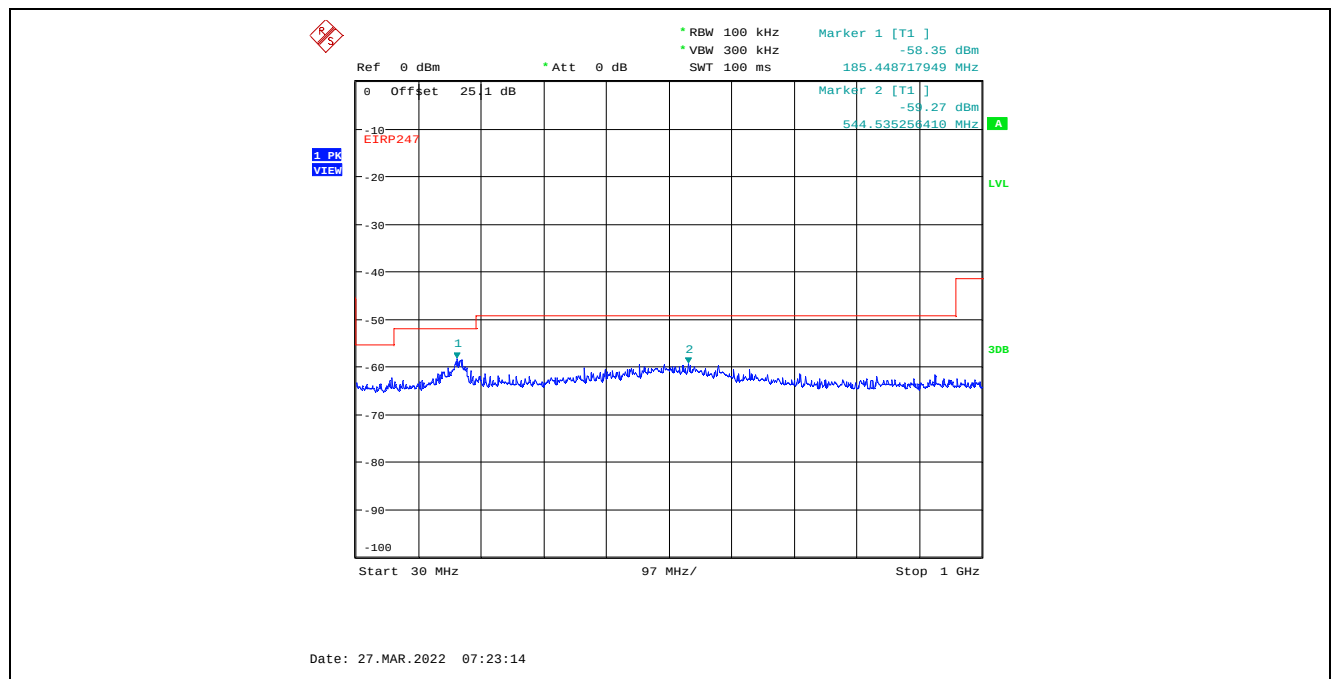
Plot C.4.56. Conducted Spurious Emissions in Restricted Frequency Bands, Chain 2 8 MHz Channel Bandwidth, Data Rate 7, Raw Power Setting 0, 2476 MHz, 30 MHz - 1 GHz, Peak Detector
