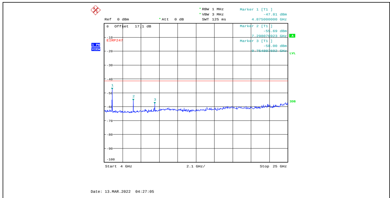
Plot C.1.79. Conducted Spurious Emissions in Restricted Frequency Bands, Chain 1 20 MHz Channel Bandwidth, Data Rate 3, Raw Power Setting 26, 2437 MHz, 4 GHz - 25 GHz, Peak Detector
