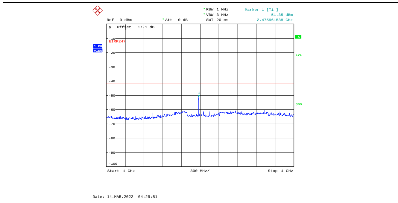
Plot C.2.58. Conducted Spurious Emissions in Restricted Frequency Bands, Chain 2 8 MHz Channel Bandwidth, Data Rate 7, Raw Power Setting 12, 2476 MHz, 1 GHz – 4 GHz, Peak Detector
