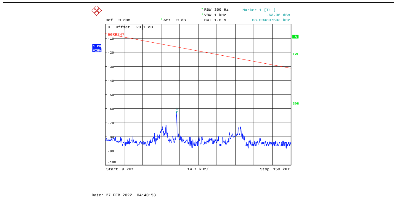
Plot C.1.32. Conducted Spurious Emissions in Restricted Frequency Bands, Chain 2 8 MHz Channel Bandwidth, Data Rate 3, Raw Power Setting 21, 2407 MHz, 9 kHz - 150 kHz, Peak Detector
