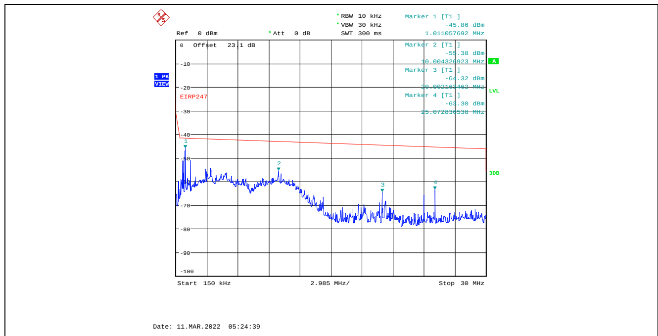
Plot C.1.94. Conducted Spurious Emissions in Restricted Frequency Bands, Chain 2 40 MHz Channel Bandwidth, Data Rate 3, Raw Power Setting 13, 2422 MHz, 150 kHz – 30 MHz, Peak Detector
