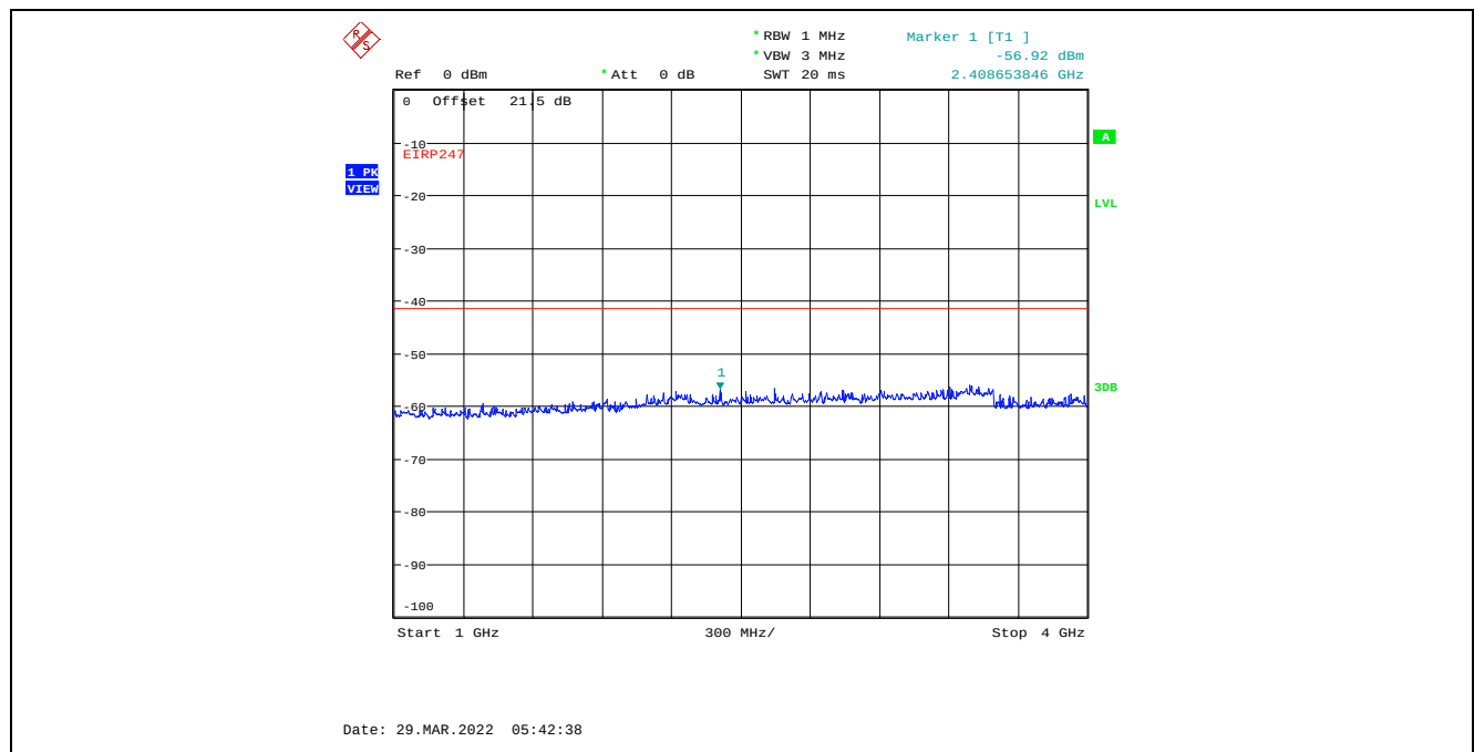
Plot C.4.68. Conducted Spurious Emissions in Restricted Frequency Bands, Chain 2 20 MHz Channel Bandwidth, Data Rate 7, Raw Power Setting 0, 2412 MHz, 1 GHz – 4 GHz, Peak Detector
