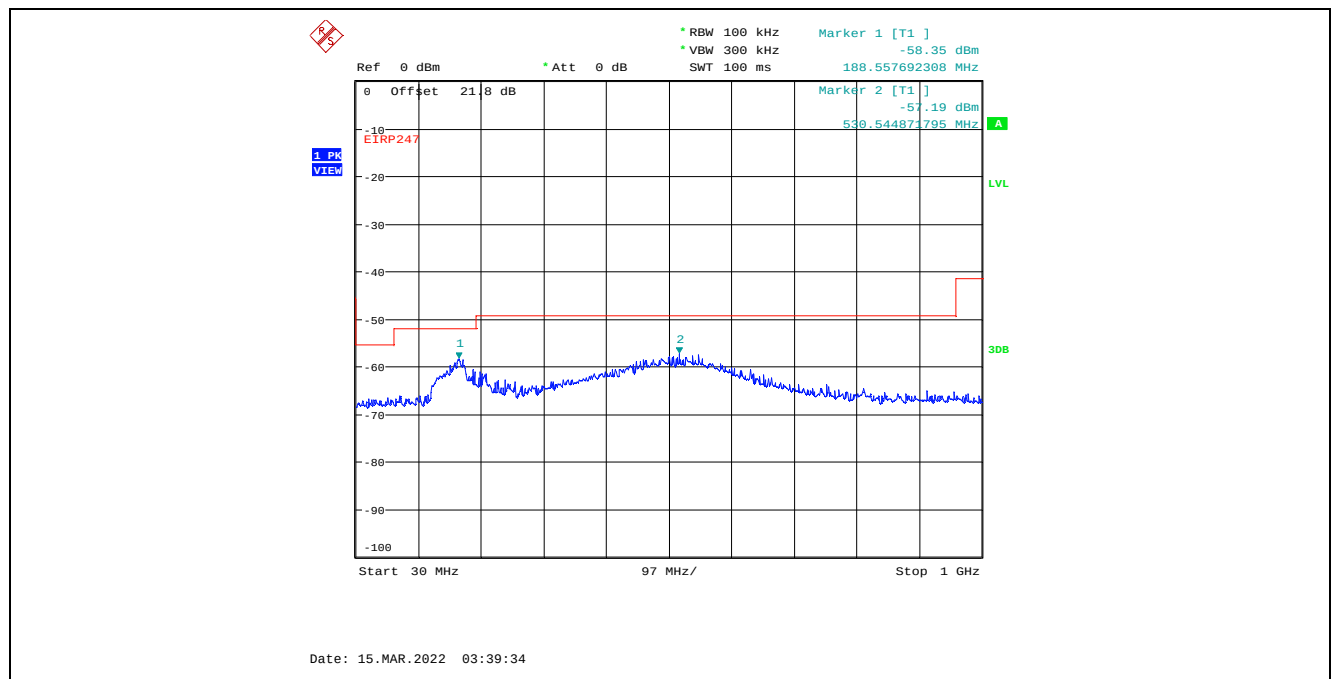
Plot C.2.26. Conducted Spurious Emissions in Restricted Frequency Bands, Chain 2 4 MHz Channel Bandwidth, Data Rate 7, Raw Power Setting 20, 2477 MHz, 30 MHz - 1 GHz, Peak Detector
