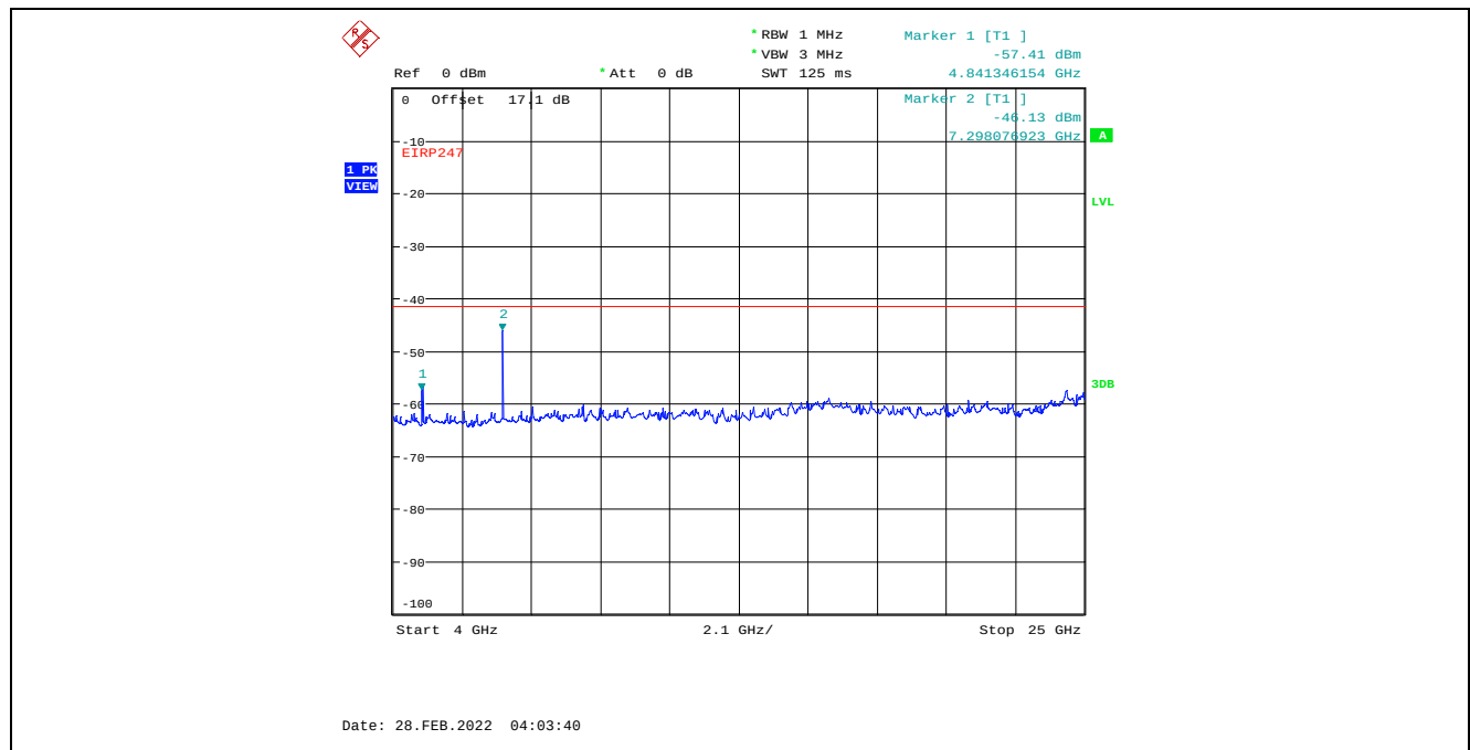
Plot C.1.49. Conducted Spurious Emissions in Restricted Frequency Bands, Chain 1 8 MHz Channel Bandwidth, Data Rate 3, Raw Power Setting 21, 2437 MHz, 4 GHz - 25 GHz, Peak Detector
