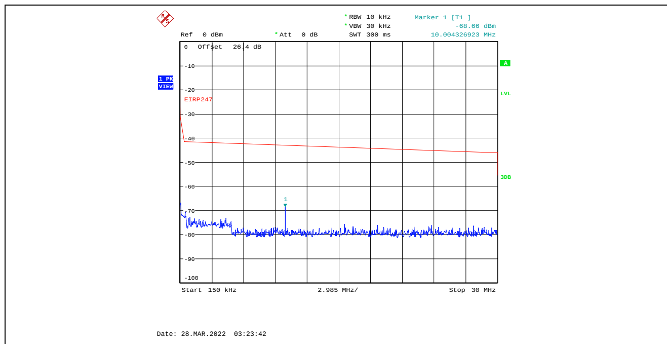
Plot C.4.53. Conducted Spurious Emissions in Restricted Frequency Bands, Chain 1 8 MHz Channel Bandwidth, Data Rate 7, Raw Power Setting 0, 2476 MHz, 150 kHz – 30 MHz, Peak Detector
