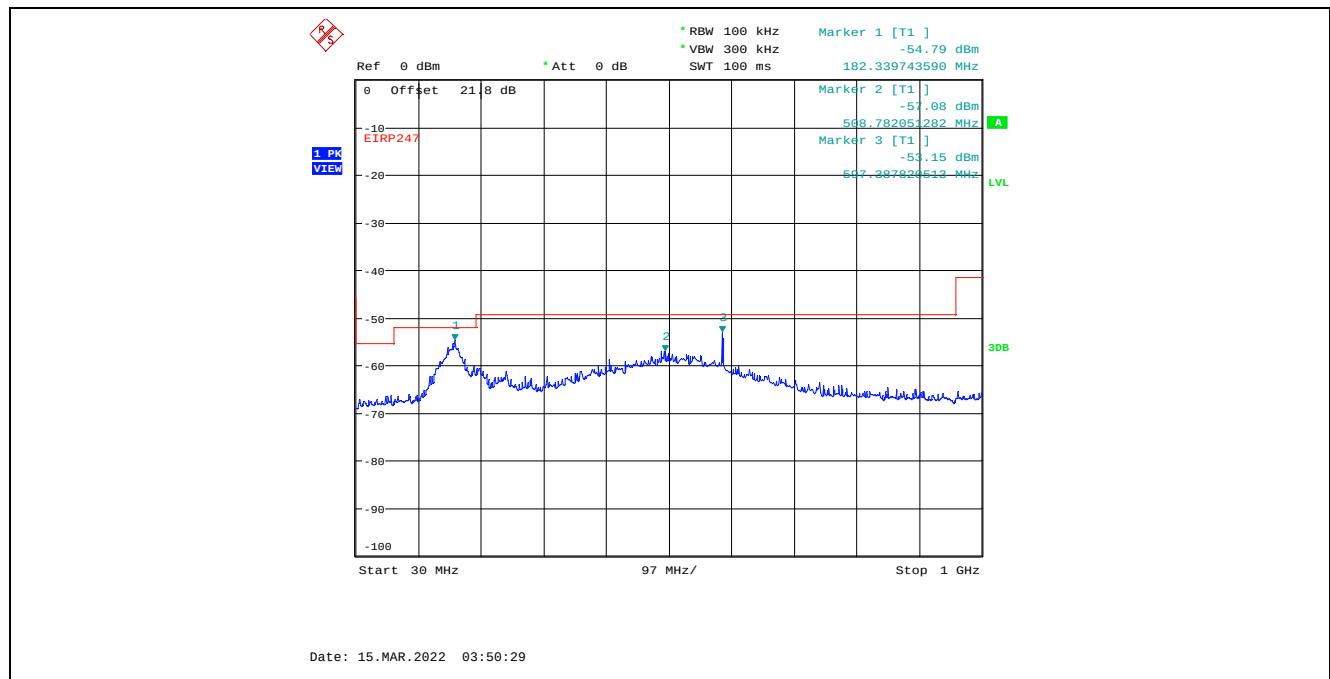
Plot C.1.25. Conducted Spurious Emissions in Restricted Frequency Bands, Chain 1 4 MHz Channel Bandwidth, Data Rate 3, Raw Power Setting 13, 2477 MHz, 30 MHz - 1 GHz, Peak Detector
