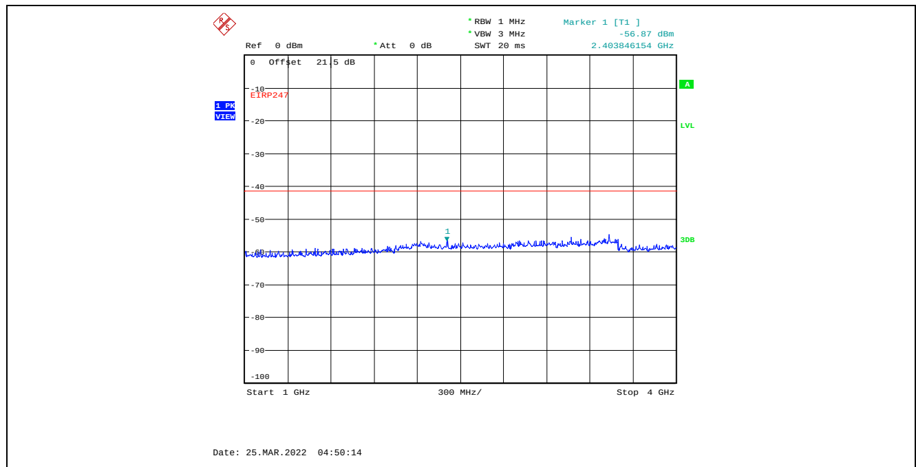
Plot C.4.8. Conducted Spurious Emissions in Restricted Frequency Bands, Chain 1 4 MHz Channel Bandwidth, Data Rate 7, Raw Power Setting 0, 2405 MHz, 1 GHz - 4 GHz, Peak Detector
