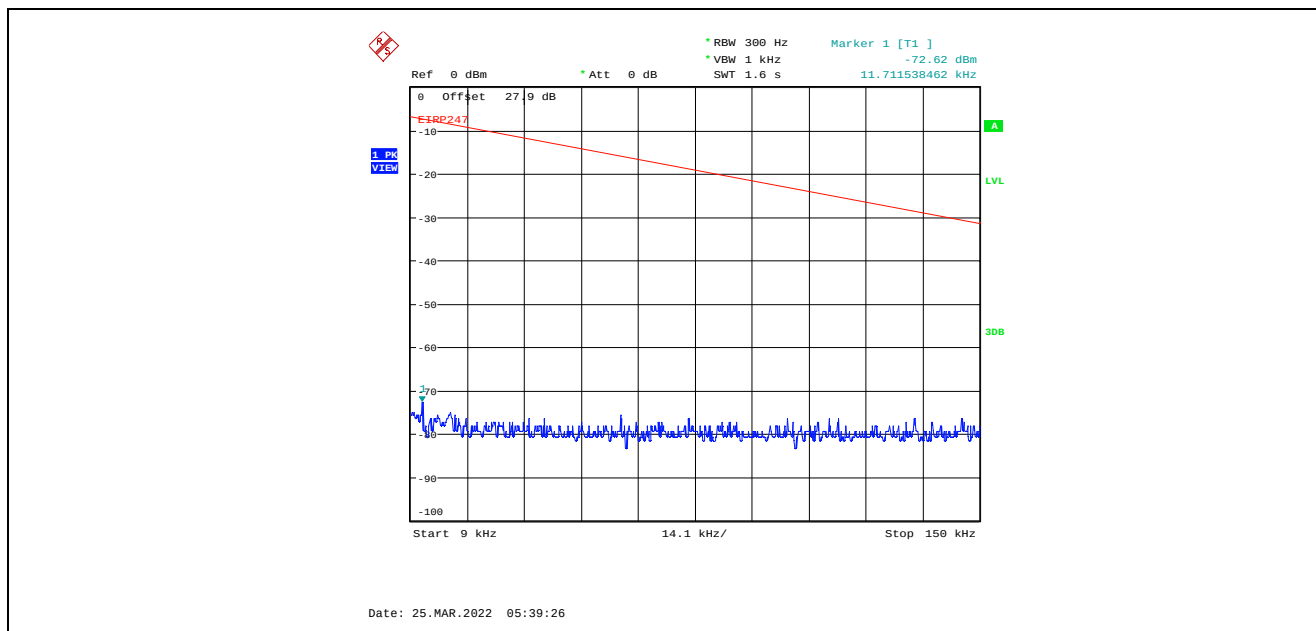
Plot C.4.2. Conducted Spurious Emissions in Restricted Frequency Bands, Chain 2 4 MHz Channel Bandwidth, Data Rate 7, Raw Power Setting 0, 2405 MHz, 9 kHz - 150 kHz, Peak Detector
