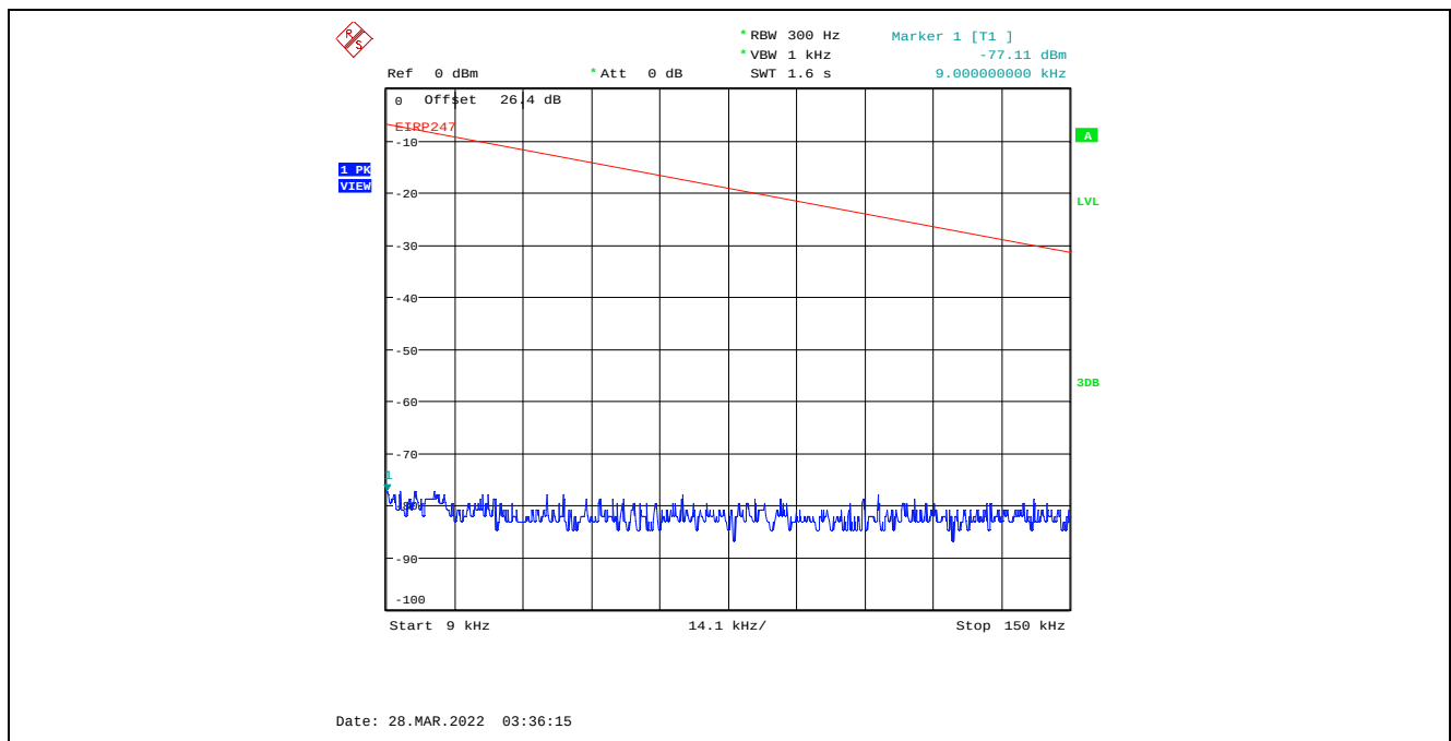
Plot C.4.32. Conducted Spurious Emissions in Restricted Frequency Bands, Chain 2 8 MHz Channel Bandwidth, Data Rate 7, Raw Power Setting 0, 2407 MHz, 9 kHz - 150 kHz, Peak Detector
