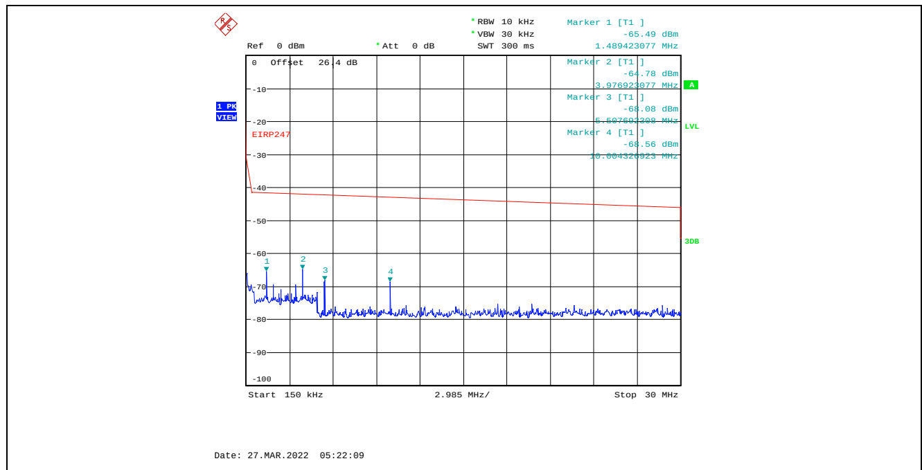
Plot C.3.44. Conducted Spurious Emissions in Restricted Frequency Bands, Chain 2 8 MHz Channel Bandwidth, Data Rate 3, Raw Power Setting 6, 2437 MHz, 150 kHz – 30 MHz, Peak Detector
