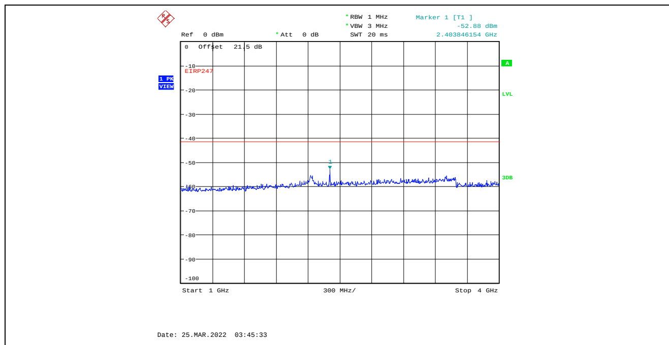
Plot C.3.7. Conducted Spurious Emissions in Restricted Frequency Bands, Chain 1 4 MHz Channel Bandwidth, Data Rate 3, Raw Power Setting 8, 2402 MHz, 1 GHz - 4 GHz, Peak Detector
