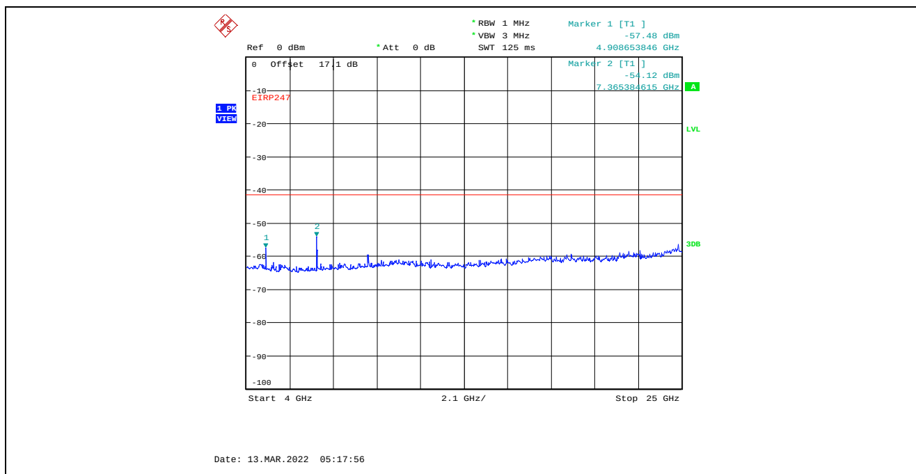
Plot C.2.89. Conducted Spurious Emissions in Restricted Frequency Bands, Chain 1 20 MHz Channel Bandwidth, Data Rate 7, Raw Power Setting 23, 2462 MHz, 4 GHz - 25 GHz, Peak Detector
