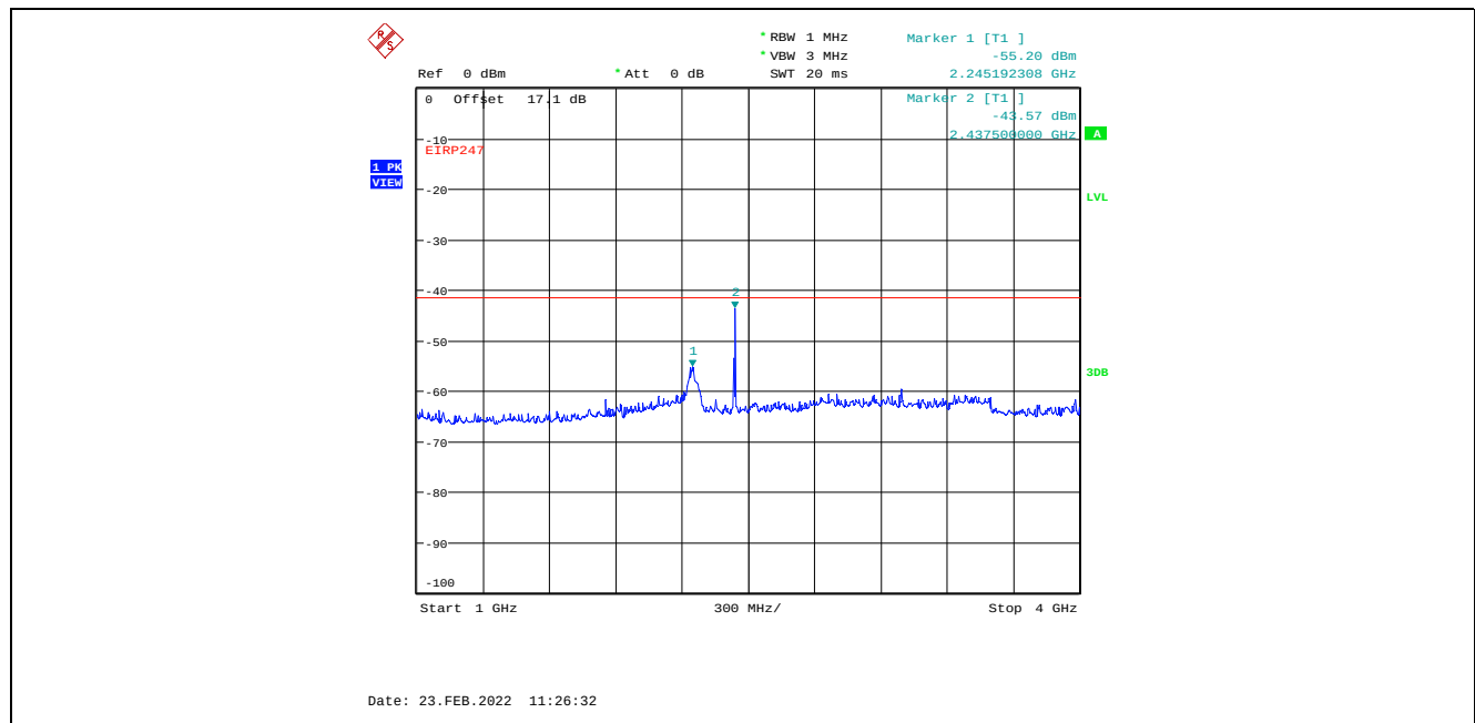
Plot C.1.18. Conducted Spurious Emissions in Restricted Frequency Bands, Chain 2 4 MHz Channel Bandwidth, Data Rate 3, Raw Power Setting 16, 2437 MHz, 1 GHz – 4 GHz, Peak Detector Marker 2 is Fundamental Signal
