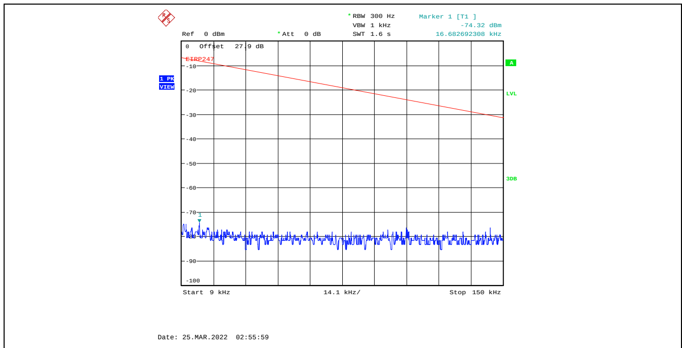
Plot C.3.22. Conducted Spurious Emissions in Restricted Frequency Bands, Chain 2 4 MHz Channel Bandwidth, Data Rate 3, Raw Power Setting 0, 2477 MHz, 9 kHz - 150 kHz, Peak Detector
