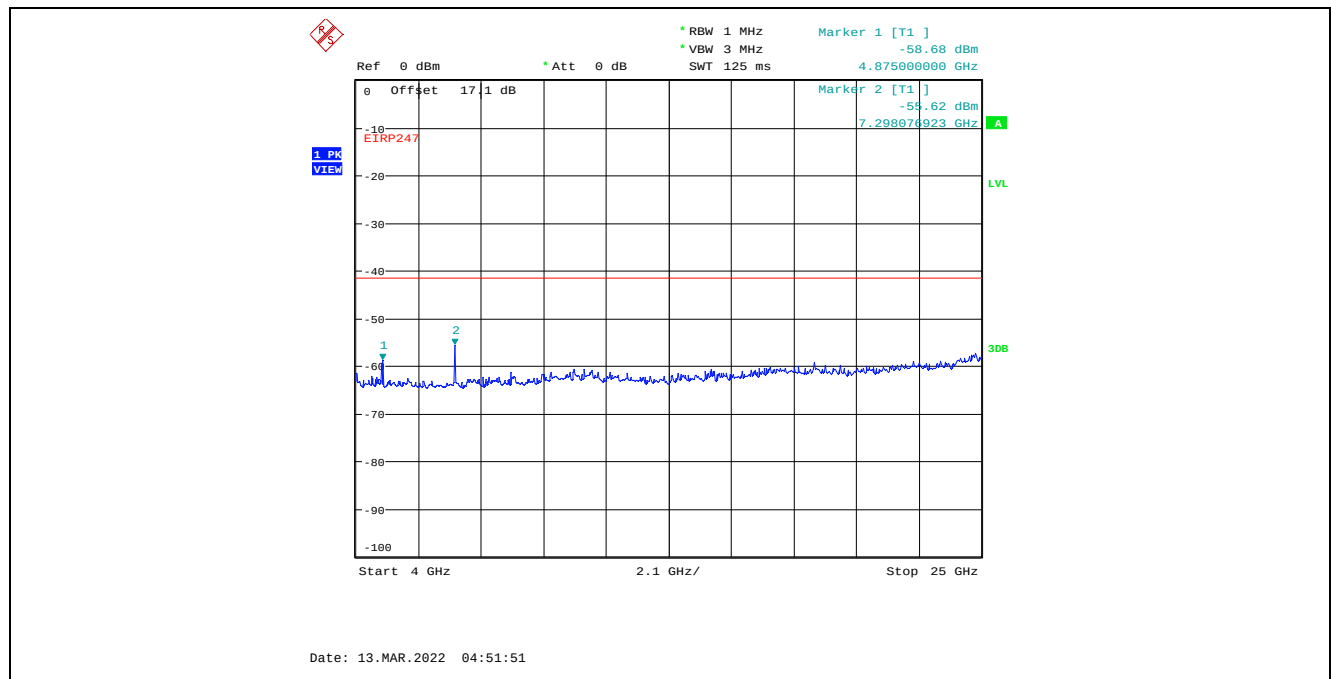
Plot C.2.80. Conducted Spurious Emissions in Restricted Frequency Bands, Chain 2 20 MHz Channel Bandwidth, Data Rate 7, Raw Power Setting 23, 2437 MHz, 4 GHz - 25 GHz, Peak Detector
