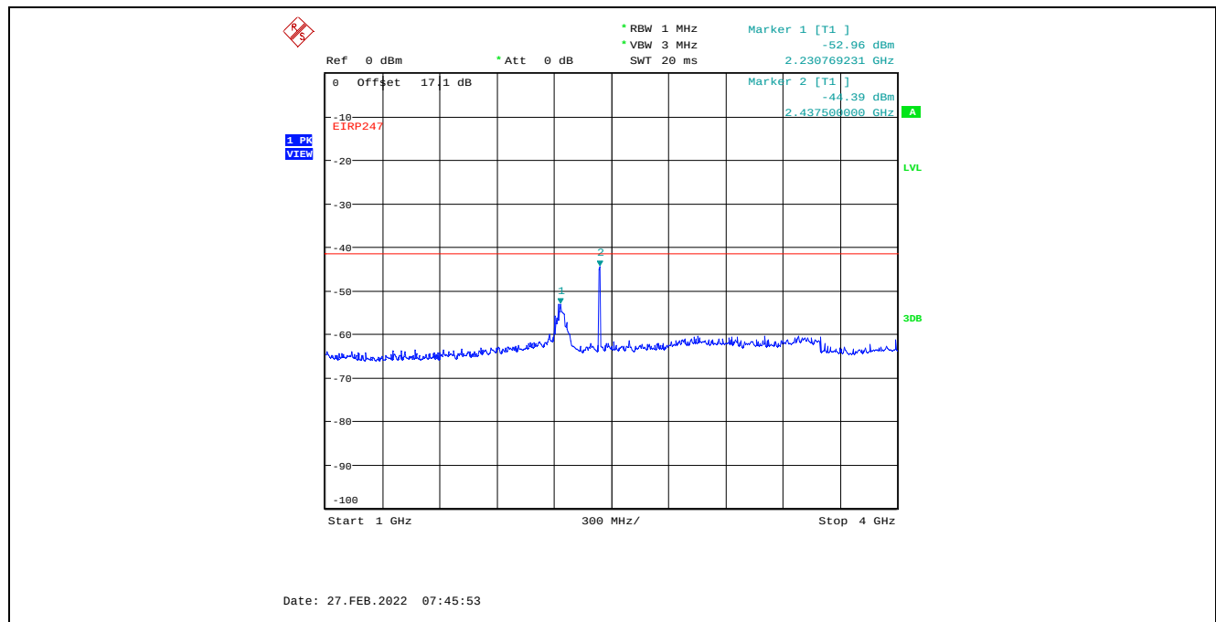
Plot C.2.47. Conducted Spurious Emissions in Restricted Frequency Bands, Chain 1 8 MHz Channel Bandwidth, Data Rate 7, Raw Power Setting 23, 2437 MHz, 1 GHz – 4 GHz, Peak Detector
