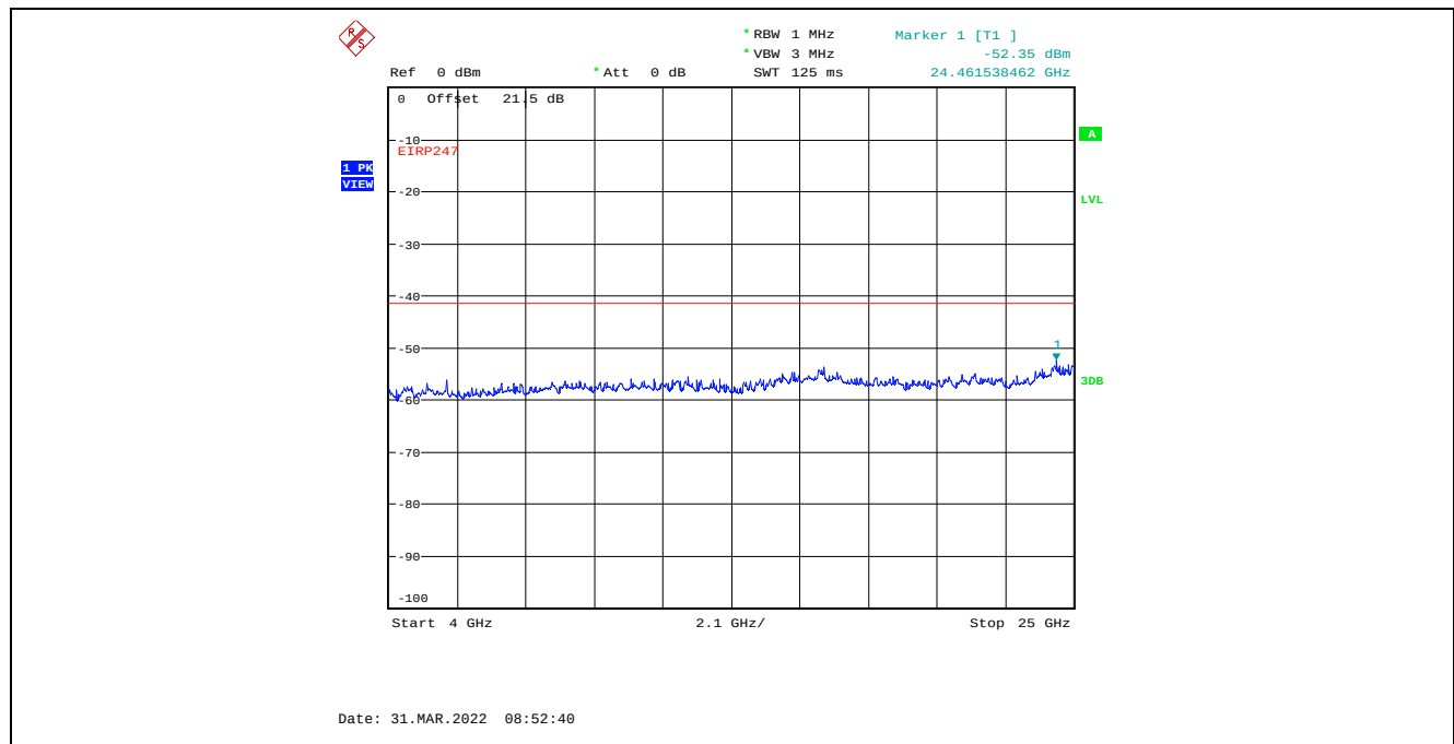
Plot C.3.119. Conducted Spurious Emissions in Restricted Frequency Bands, Chain 1 40 MHz Channel Bandwidth, Data Rate 3, Raw Power Setting 0, 2452 MHz, 4 GHz - 25 GHz, Peak Detector
