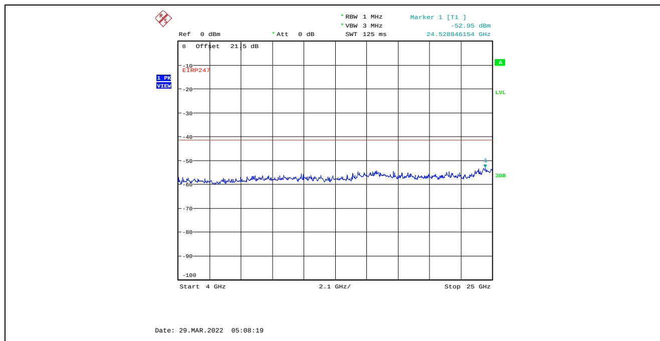
Plot C.3.80. Conducted Spurious Emissions in Restricted Frequency Bands, Chain 2 20 MHz Channel Bandwidth, Data Rate 3, Raw Power Setting 7, 2437 MHz, 4 GHz - 25 GHz, Peak Detector
