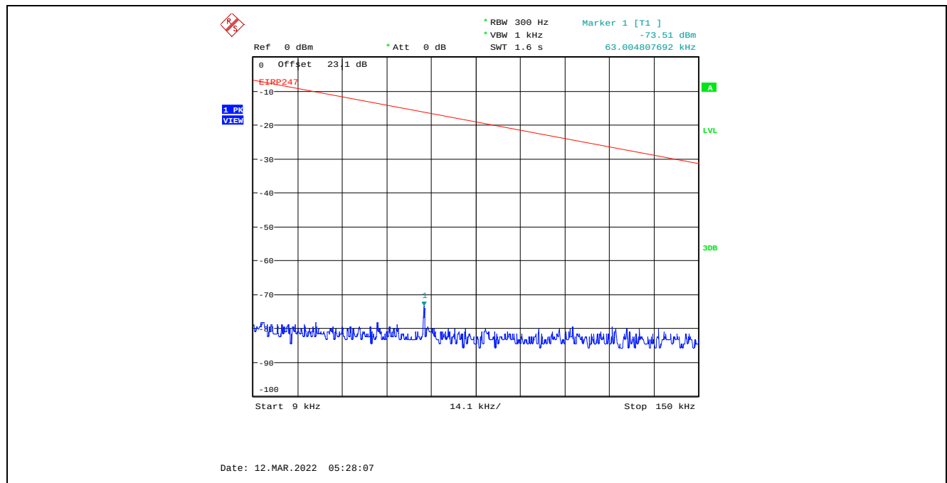
Plot C.2.112. Conducted Spurious Emissions in Restricted Frequency Bands, Chain 2 40 MHz Channel Bandwidth, Data Rate 7, Raw Power Setting 22, 2452 MHz, 9 kHz - 150 kHz, Peak Detector
