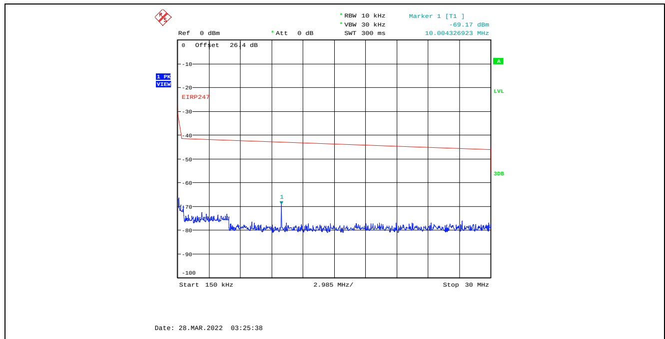
Plot C.4.43. Conducted Spurious Emissions in Restricted Frequency Bands, Chain 1 8 MHz Channel Bandwidth, Data Rate 7, Raw Power Setting 0, 2437 MHz, 150 kHz – 30 MHz, Peak Detector
