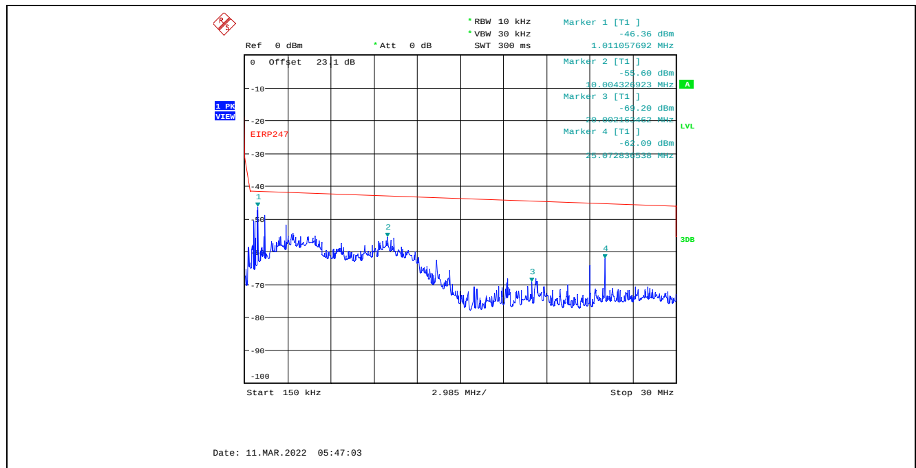
Plot C.1.113. Conducted Spurious Emissions in Restricted Frequency Bands, Chain 1 40 MHz Channel Bandwidth, Data Rate 3, Raw Power Setting 15, 2452 MHz, 150 kHz – 30 MHz, Peak Detector
