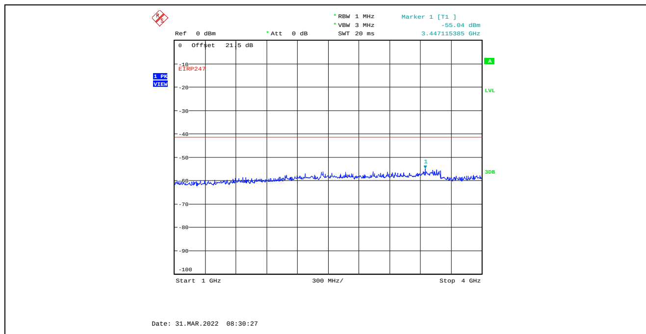
Plot C.3.108. Conducted Spurious Emissions in Restricted Frequency Bands, Chain 2 40 MHz Channel Bandwidth, Data Rate 3, Raw Power Setting 0, 2437 MHz, 1 GHz – 4 GHz, Peak Detector
