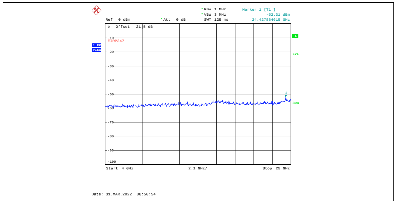
Plot C.3.109. Conducted Spurious Emissions in Restricted Frequency Bands, Chain 1 40 MHz Channel Bandwidth, Data Rate 3, Raw Power Setting 0, 2437 MHz, 4 GHz - 25 GHz, Peak Detector
