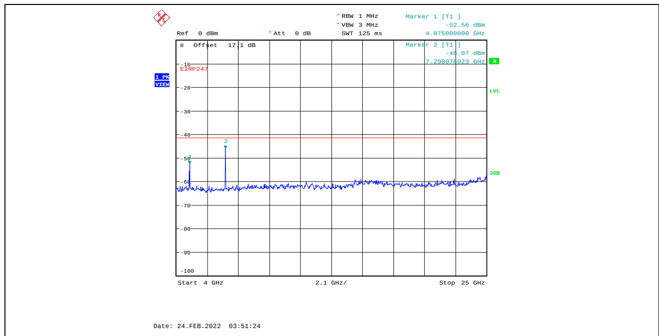
Plot C.1.20. Conducted Spurious Emissions in Restricted Frequency Bands, Chain 2 4 MHz Channel Bandwidth, Data Rate 3, Raw Power Setting 16, 2437 MHz, 4 GHz - 25 GHz, Peak Detector
