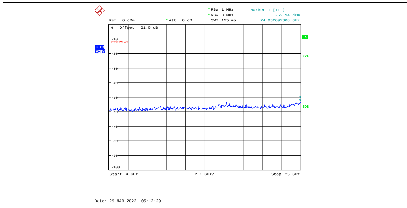
Plot C.3.89. Conducted Spurious Emissions in Restricted Frequency Bands, Chain 1 20 MHz Channel Bandwidth, Data Rate 3, Raw Power Setting 7, 2462 MHz, 4 GHz - 25 GHz, Peak Detector
