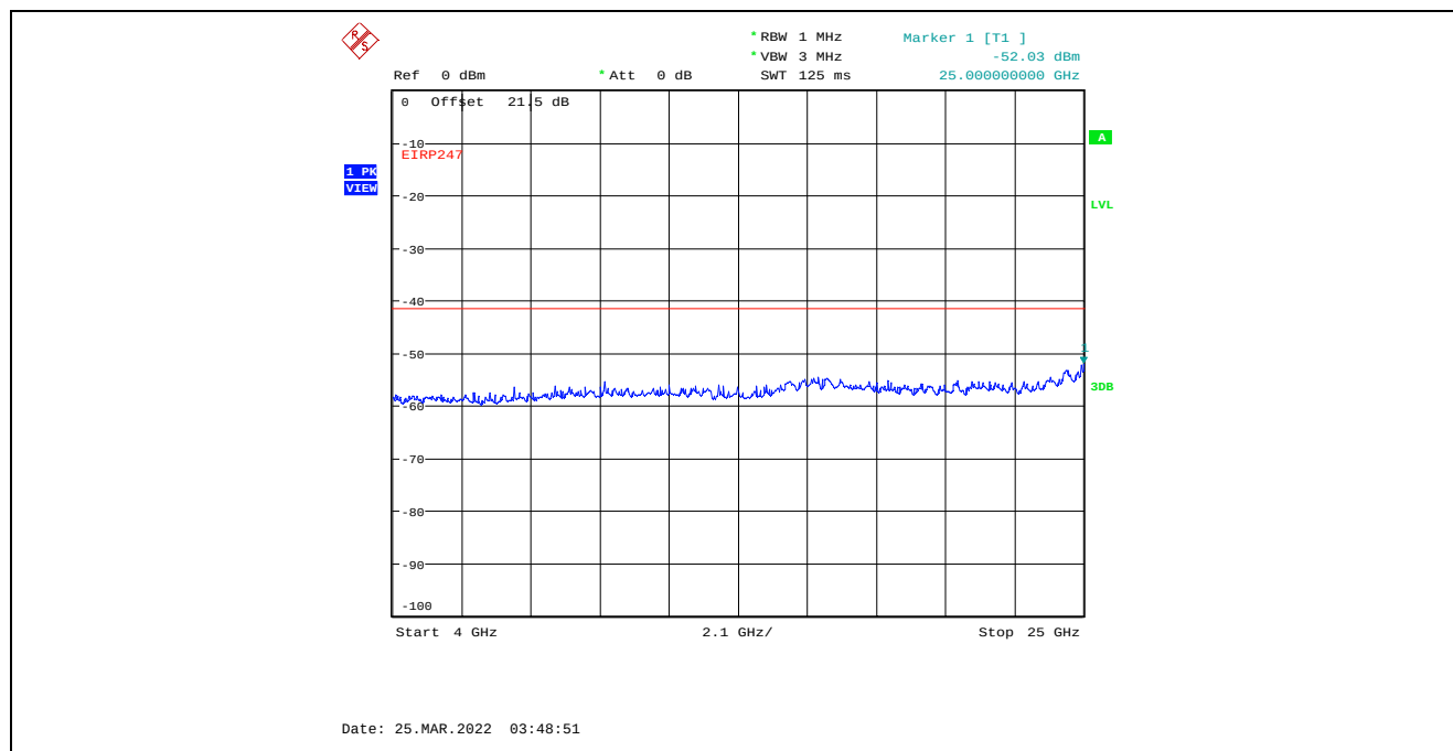
Plot C.3.9. Conducted Spurious Emissions in Restricted Frequency Bands, Chain 2 4 MHz Channel Bandwidth, Data Rate 3, Raw Power Setting 8, 2402 MHz, 4 GHz - 25 GHz, Peak Detector
