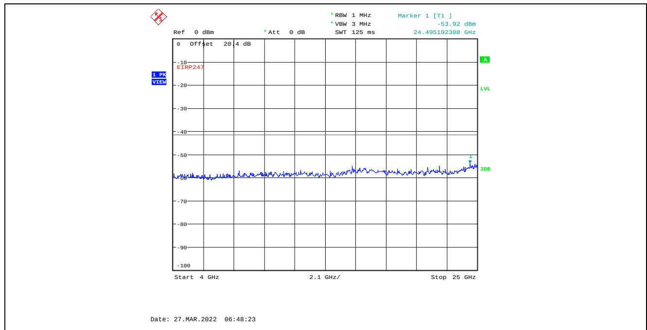
Plot C.4.39. Conducted Spurious Emissions in Restricted Frequency Bands, Chain 1 8 MHz Channel Bandwidth, Data Rate 7, Raw Power Setting 0, 2407 MHz, 4 GHz - 25 GHz, Peak Detector
