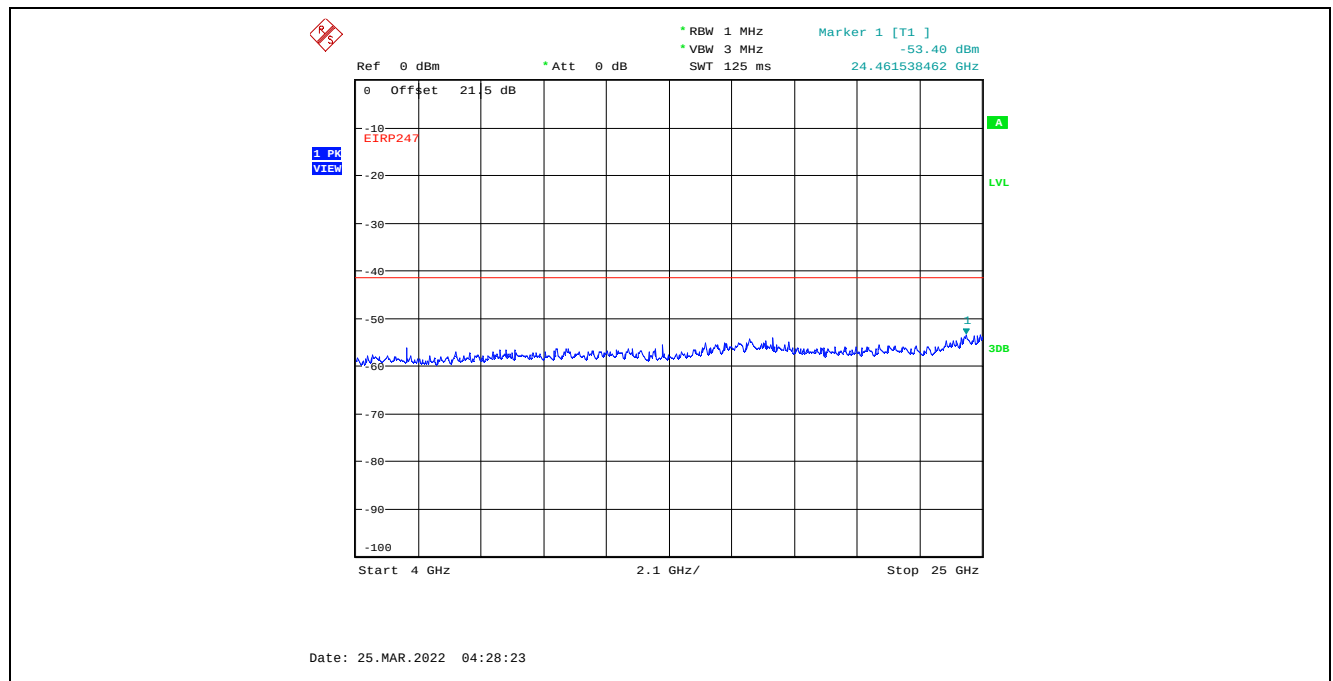
Plot C.4.29. Conducted Spurious Emissions in Restricted Frequency Bands, Chain 1 4 MHz Channel Bandwidth, Data Rate 7, Raw Power Setting 0, 2477 MHz, 4 GHz - 25 GHz, Peak Detector
