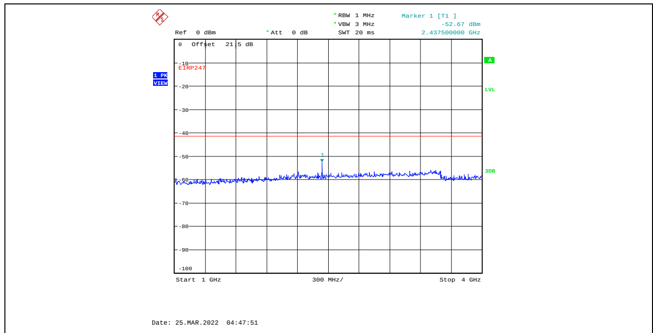
Plot C.4.18. Conducted Spurious Emissions in Restricted Frequency Bands, Chain 2 4 MHz Channel Bandwidth, Data Rate 7, Raw Power Setting 0, 2437 MHz, 1 GHz – 4 GHz, Peak Detector
