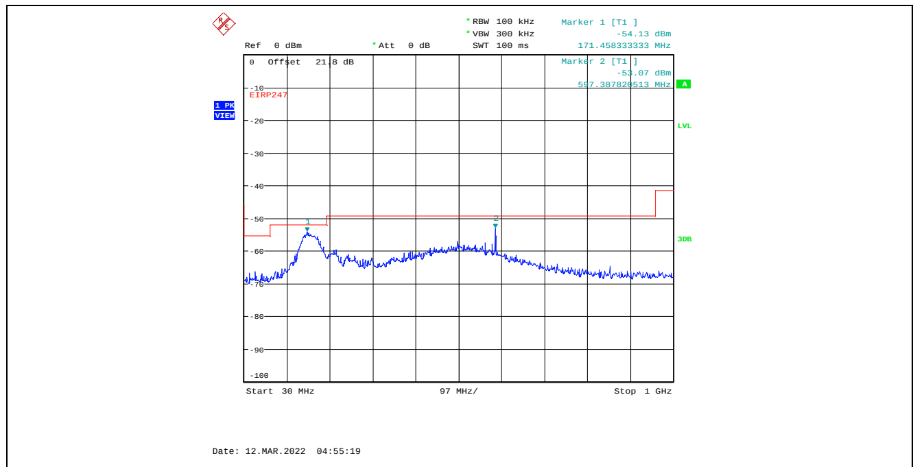
Plot C.2.115. Conducted Spurious Emissions in Restricted Frequency Bands, Chain 1 40 MHz Channel Bandwidth, Data Rate 7, Raw Power Setting 22, 2452 MHz, 30 MHz - 1 GHz, Peak Detector
