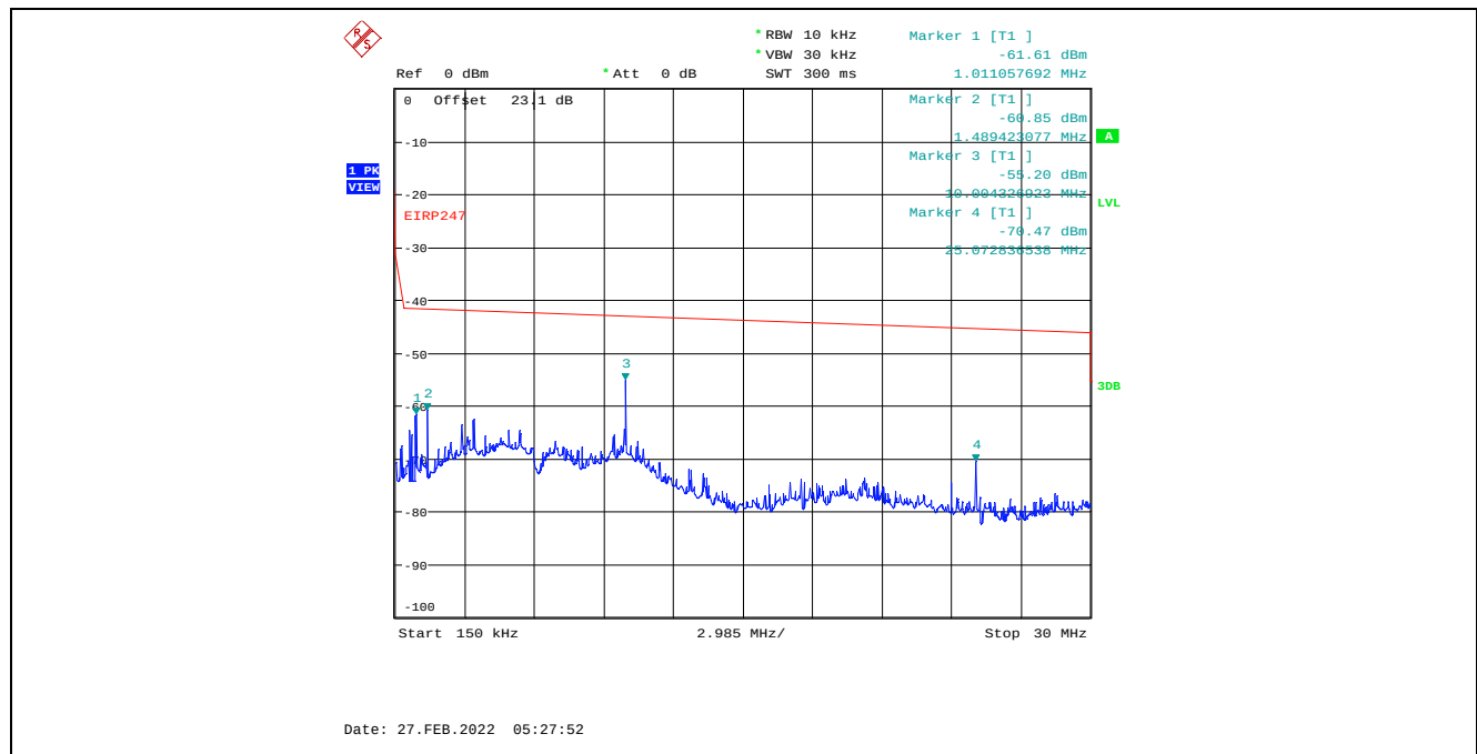
Plot C.1.43. Conducted Spurious Emissions in Restricted Frequency Bands, Chain 1 8 MHz Channel Bandwidth, Data Rate 3, Raw Power Setting 21, 2437 MHz, 150 kHz – 30 MHz, Peak Detector
