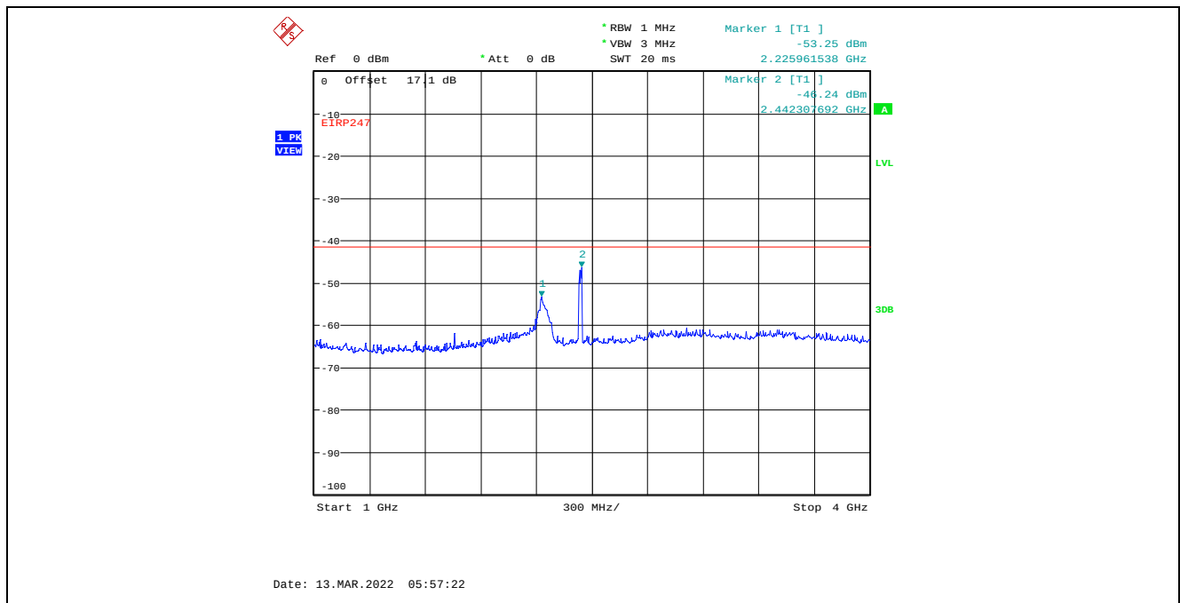
Plot C.2.78. Conducted Spurious Emissions in Restricted Frequency Bands, Chain 2 20 MHz Channel Bandwidth, Data Rate 7, Raw Power Setting 23, 2437 MHz, 1 GHz – 4 GHz, Peak Detector
