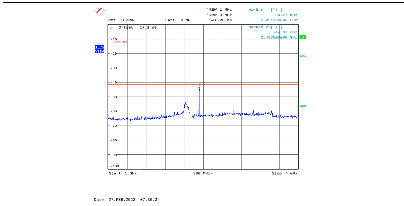
Plot C.2.48. Conducted Spurious Emissions in Restricted Frequency Bands, Chain 2 8 MHz Channel Bandwidth, Data Rate 7, Raw Power Setting 23, 2437 MHz, 1 GHz – 4 GHz, Peak Detector
