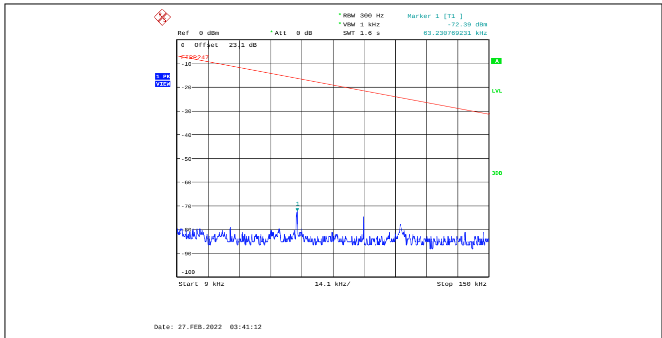
Plot C.1.31. Conducted Spurious Emissions in Restricted Frequency Bands, Chain 1 8 MHz Channel Bandwidth, Data Rate 3, Raw Power Setting 21, 2407 MHz, 9 kHz - 150 kHz, Peak Detector
