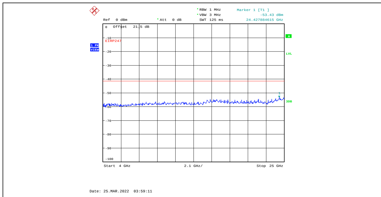
Plot C.3.10. Conducted Spurious Emissions in Restricted Frequency Bands, Chain 2 4 MHz Channel Bandwidth, Data Rate 3, Raw Power Setting 8, 2402 MHz, 4 GHz - 25 GHz, Peak Detector
