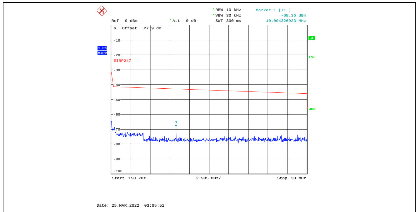
Plot C.3.14. Conducted Spurious Emissions in Restricted Frequency Bands, Chain 2 4 MHz Channel Bandwidth, Data Rate 3, Raw Power Setting 8, 2437 MHz, 150 kHz – 30 MHz, Peak Detector
