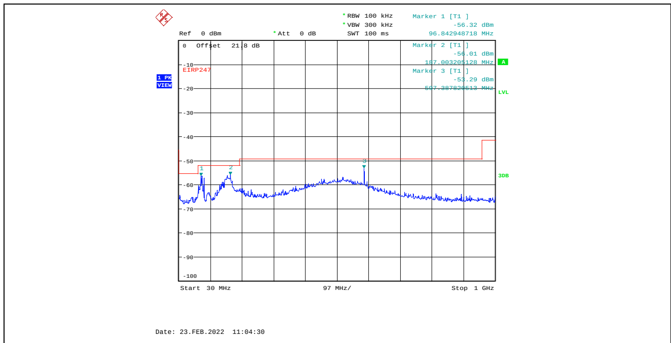
Plot C.1.5. Conducted Spurious Emissions in Restricted Frequency Bands, Chain 1 4 MHz Channel Bandwidth, Data Rate 3, Raw Power Setting 16, 2402 MHz, 30 MHz - 1 GHz, Peak Detector
