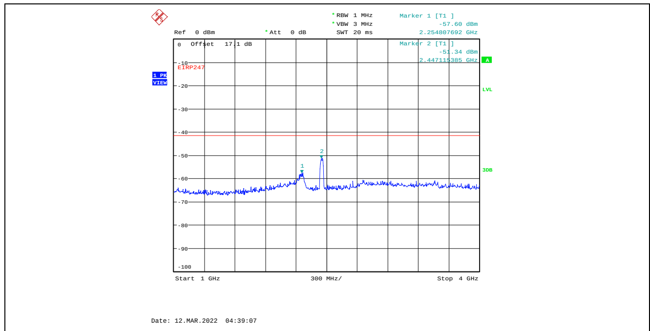
Plot C.2.118. Conducted Spurious Emissions in Restricted Frequency Bands, Chain 2 40 MHz Channel Bandwidth, Data Rate 7, Raw Power Setting 22, 2452 MHz, 1 GHz – 4 GHz, Peak Detector
