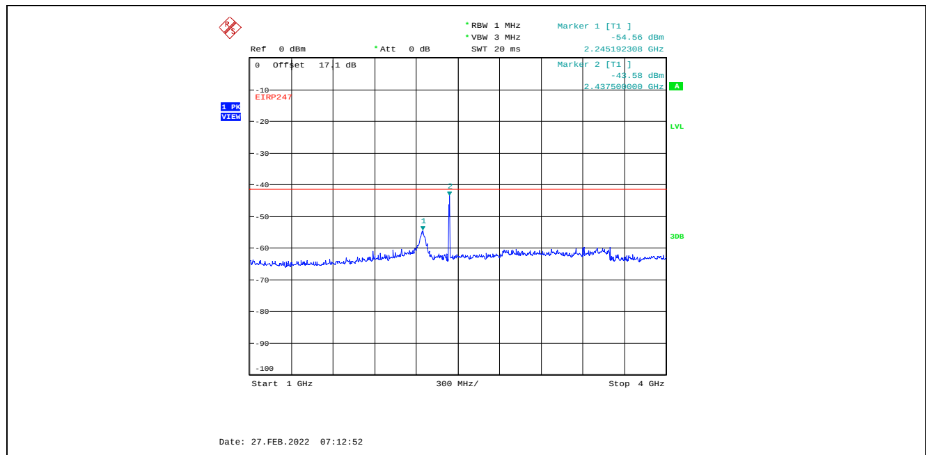
Plot C.1.48. Conducted Spurious Emissions in Restricted Frequency Bands, Chain 2 8 MHz Channel Bandwidth, Data Rate 3, Raw Power Setting 21, 2437 MHz, 1 GHz – 4 GHz, Peak Detector Marker 2 is Fundamental Signal
