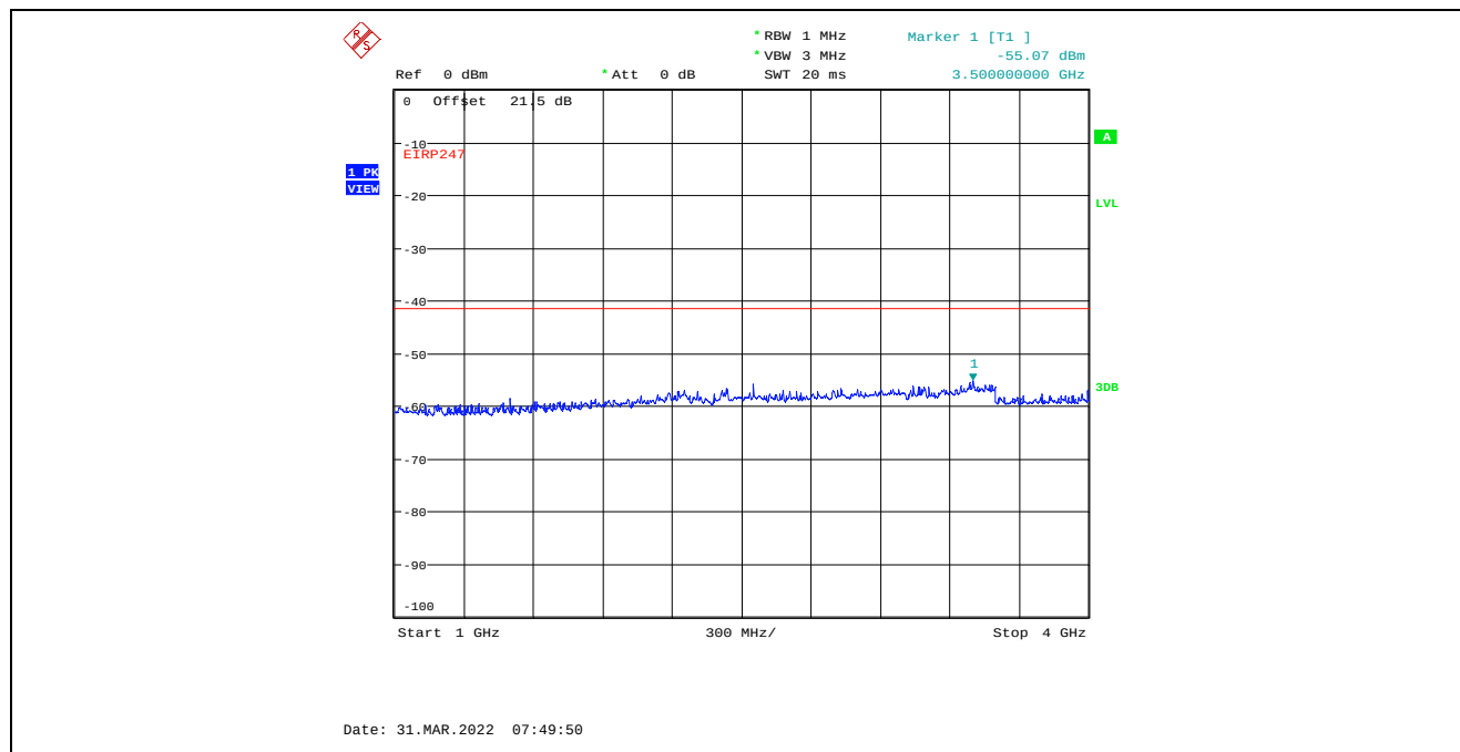
Plot C.4.108. Conducted Spurious Emissions in Restricted Frequency Bands, Chain 2 40 MHz Channel Bandwidth, Data Rate 7, Raw Power Setting 0, 2437 MHz, 1 GHz – 4 GHz, Peak Detector
