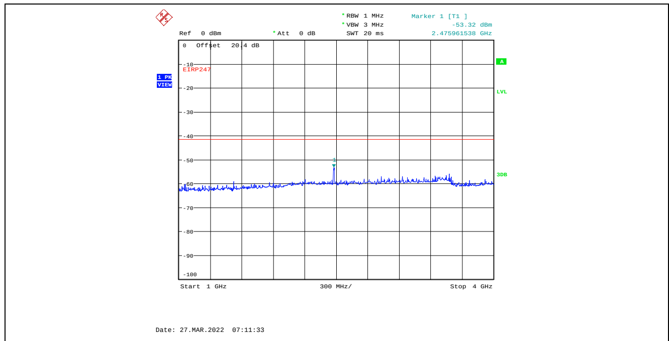
Plot C.4.57. Conducted Spurious Emissions in Restricted Frequency Bands, Chain 1 8 MHz Channel Bandwidth, Data Rate 7, Raw Power Setting 0, 2476 MHz, 1 GHz – 4 GHz, Peak Detector
