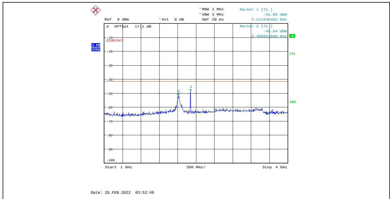
Plot C.1.37. Conducted Spurious Emissions in Restricted Frequency Bands, Chain 1 8 MHz Channel Bandwidth, Data Rate 3, Raw Power Setting 21, 2407 MHz, 1 GHz – 4 GHz, Peak Detector
