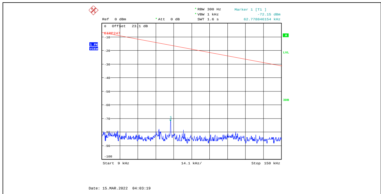
Plot C.1.22. Conducted Spurious Emissions in Restricted Frequency Bands, Chain 2 4 MHz Channel Bandwidth, Data Rate 3, Raw Power Setting 13, 2477 MHz, 9 kHz - 150 kHz, Peak Detector
