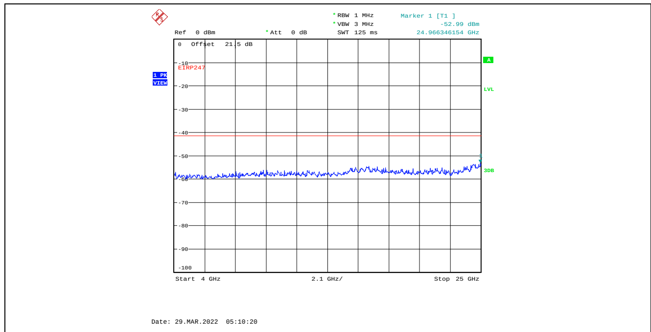
Plot C.3.90. Conducted Spurious Emissions in Restricted Frequency Bands, Chain 2 20 MHz Channel Bandwidth, Data Rate 3, Raw Power Setting 7, 2462 MHz, 4 GHz - 25 GHz, Peak Detector
