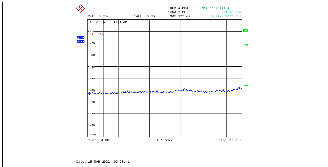
Plot C.1.29. Conducted Spurious Emissions in Restricted Frequency Bands, Chain 1 4 MHz Channel Bandwidth, Data Rate 3, Raw Power Setting 13, 2477 MHz, 4 GHz - 25 GHz, Peak Detector
