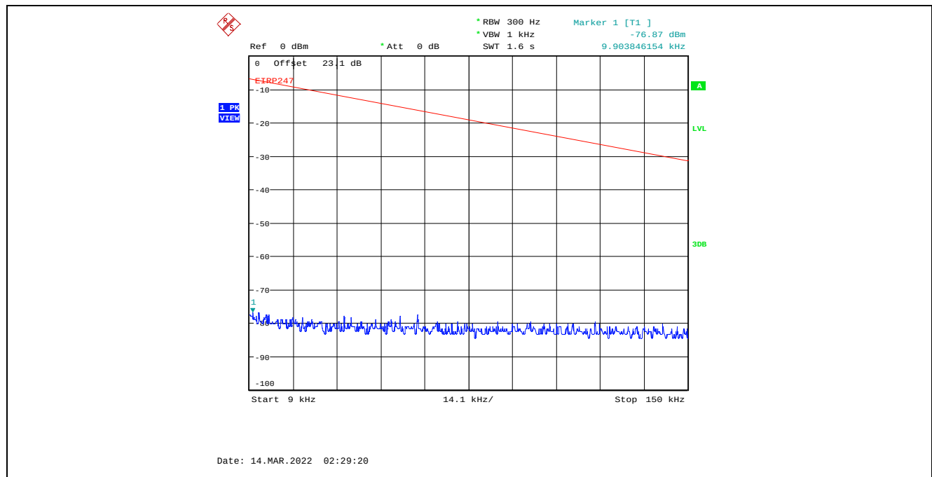
Plot C.2.71. Conducted Spurious Emissions in Restricted Frequency Bands, Chain 1 20 MHz Channel Bandwidth, Data Rate 7, Raw Power Setting 23, 2437 MHz, 9 kHz - 150 kHz, Peak Detector
