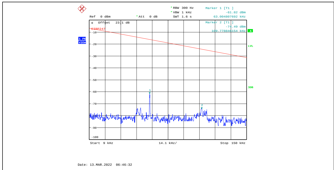
Plot C.2.72. Conducted Spurious Emissions in Restricted Frequency Bands, Chain 2 20 MHz Channel Bandwidth, Data Rate 7, Raw Power Setting 23, 2437 MHz, 9 kHz - 150 kHz, Peak Detector
