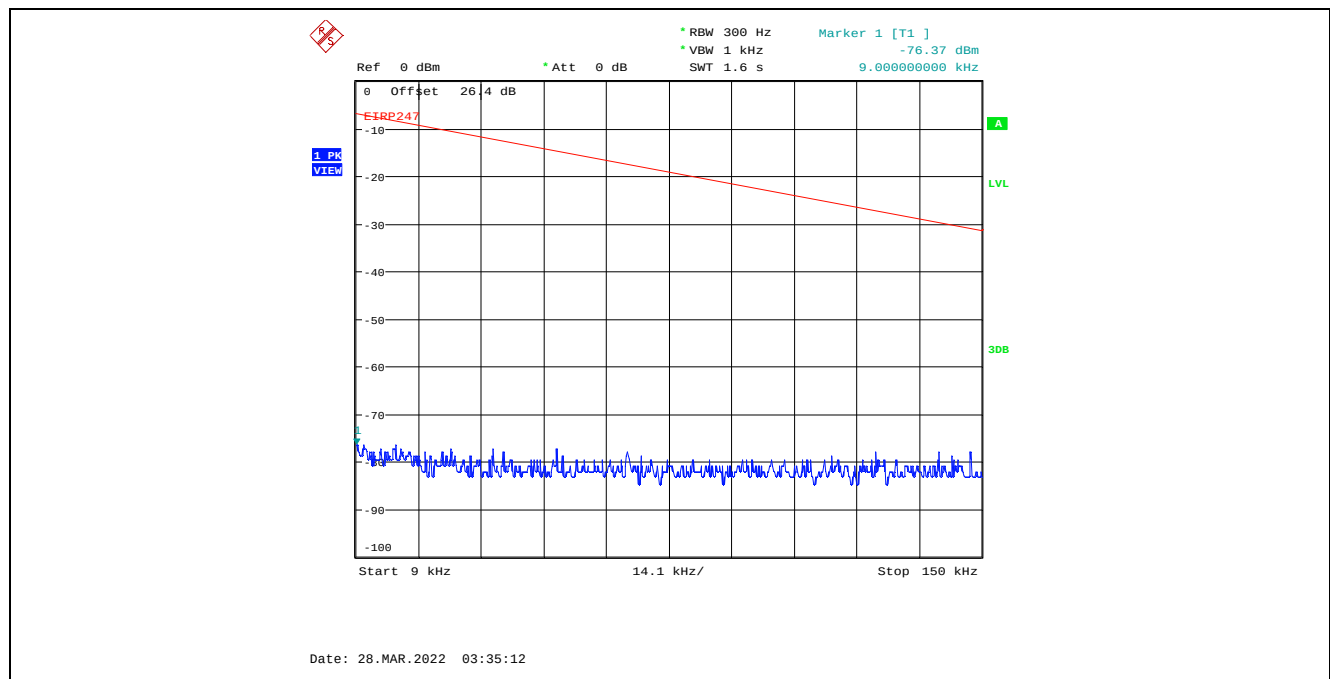
Plot C.4.42. Conducted Spurious Emissions in Restricted Frequency Bands, Chain 2 8 MHz Channel Bandwidth, Data Rate 7, Raw Power Setting 0, 2437 MHz, 9 kHz - 150 kHz, Peak Detector
