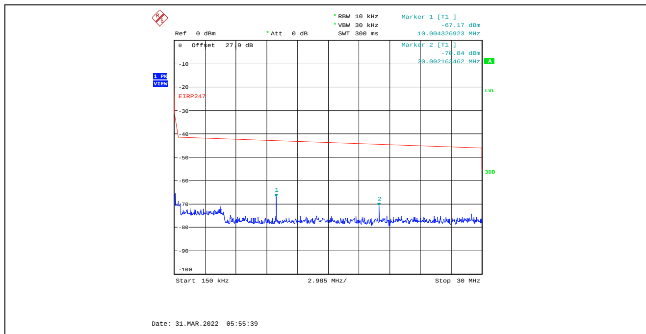
Plot C.3.113. Conducted Spurious Emissions in Restricted Frequency Bands, Chain 1 40 MHz Channel Bandwidth, Data Rate 3, Raw Power Setting 0, 2452 MHz, 150 kHz – 30 MHz, Peak Detector
