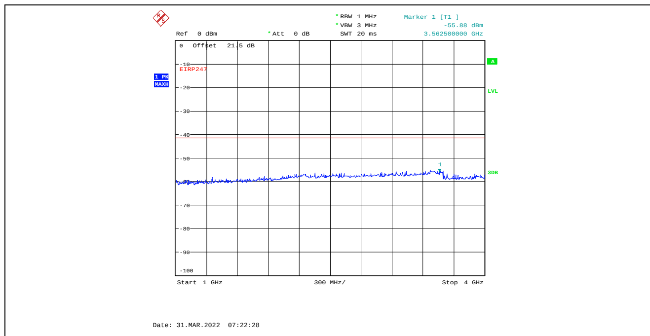
Plot C.4.97. Conducted Spurious Emissions in Restricted Frequency Bands, Chain 1 40 MHz Channel Bandwidth, Data Rate 7, Raw Power Setting 0, 2422 MHz, 1 GHz – 4 GHz, Peak Detector
