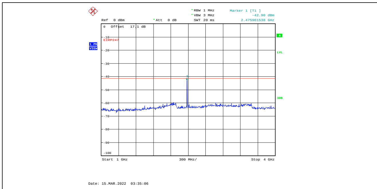
Plot C.2.28. Conducted Spurious Emissions in Restricted Frequency Bands, Chain 2 4 MHz Channel Bandwidth, Data Rate 7, Raw Power Setting 20, 2477 MHz, 1 GHz – 4 GHz, Peak Detector Marker 1 is Fundamental Signal
