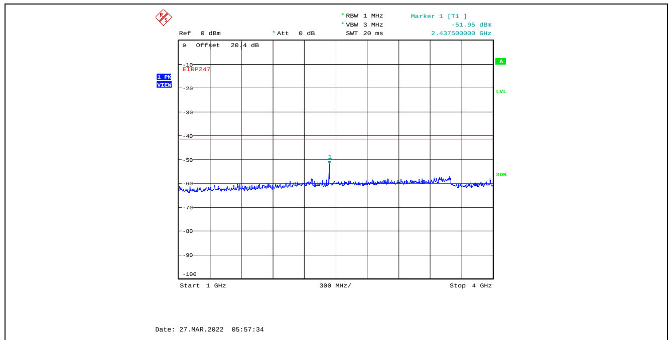
Plot C.3.48. Conducted Spurious Emissions in Restricted Frequency Bands, Chain 2 8 MHz Channel Bandwidth, Data Rate 3, Raw Power Setting 6, 2437 MHz, 1 GHz – 4 GHz, Peak Detector
