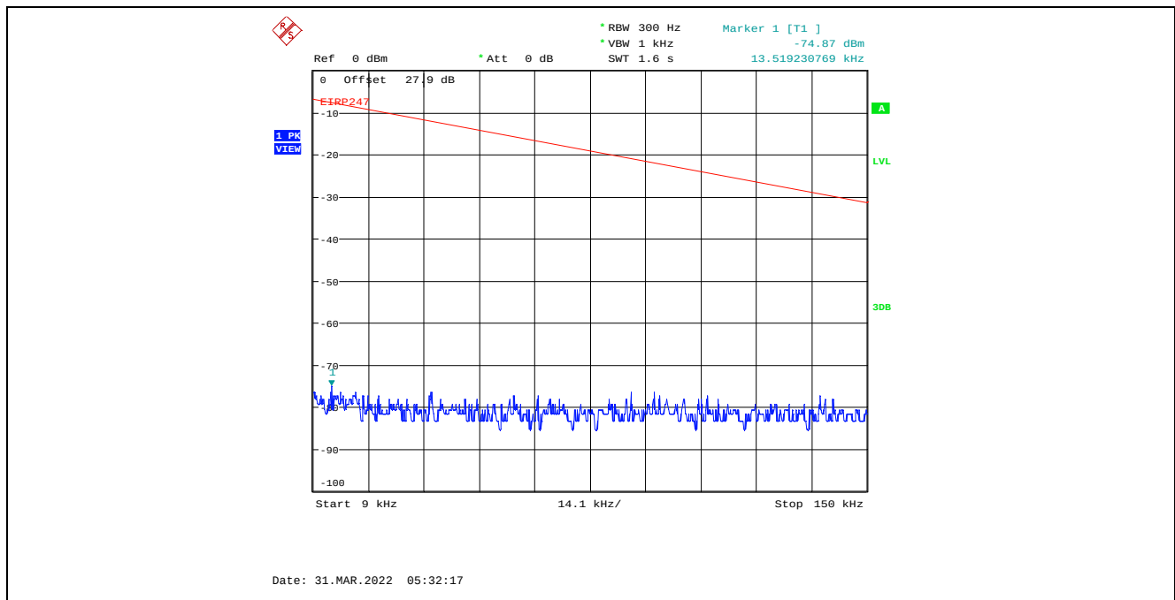
Plot C.4.111. Conducted Spurious Emissions in Restricted Frequency Bands, Chain 1 40 MHz Channel Bandwidth, Data Rate 7, Raw Power Setting 0, 2452 MHz, 9 kHz - 150 kHz, Peak Detector
