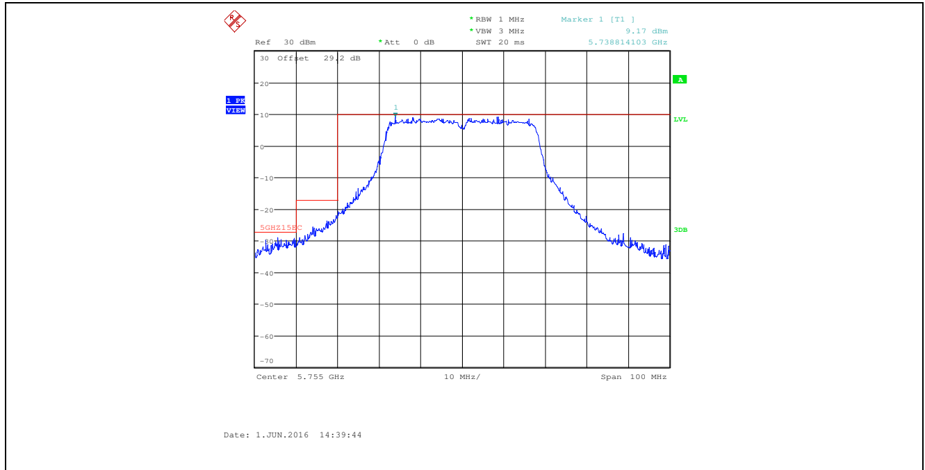
Plot 5.3.4.1.18. Band-Edge Conducted Emissions, 802.11an HT40, 135 Mbps, Ch 151, 5755 MHz, PCDAC Power 40, ANT 1 Offset = 29.16dB = 27.16dB Insertion Loss + 2dBi EUT antenna gain
