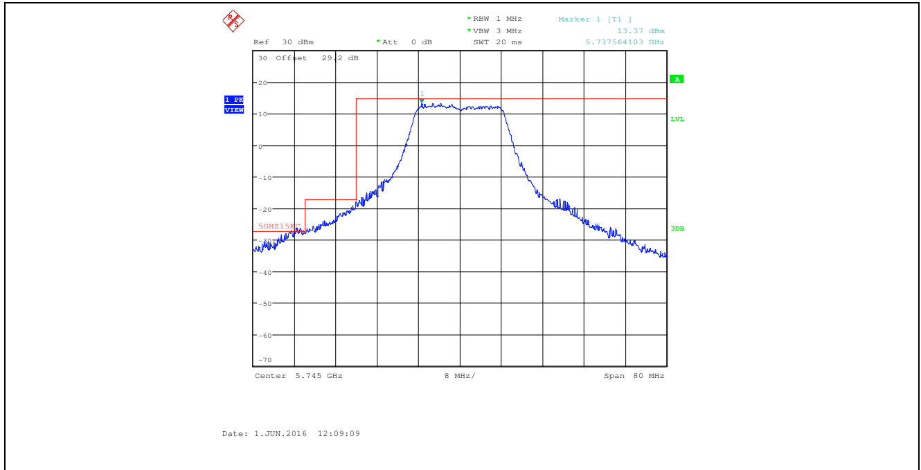
Plot 5.3.4.1.14. Band-Edge Conducted Emissions, 802.11an HT20, 65 Mbps, Ch 149, 5745 MHz, PCDAC Power 40, ANT 2 Offset = 29.16dB = 27.16dB Insertion Loss + 2dBi EUT antenna gain
