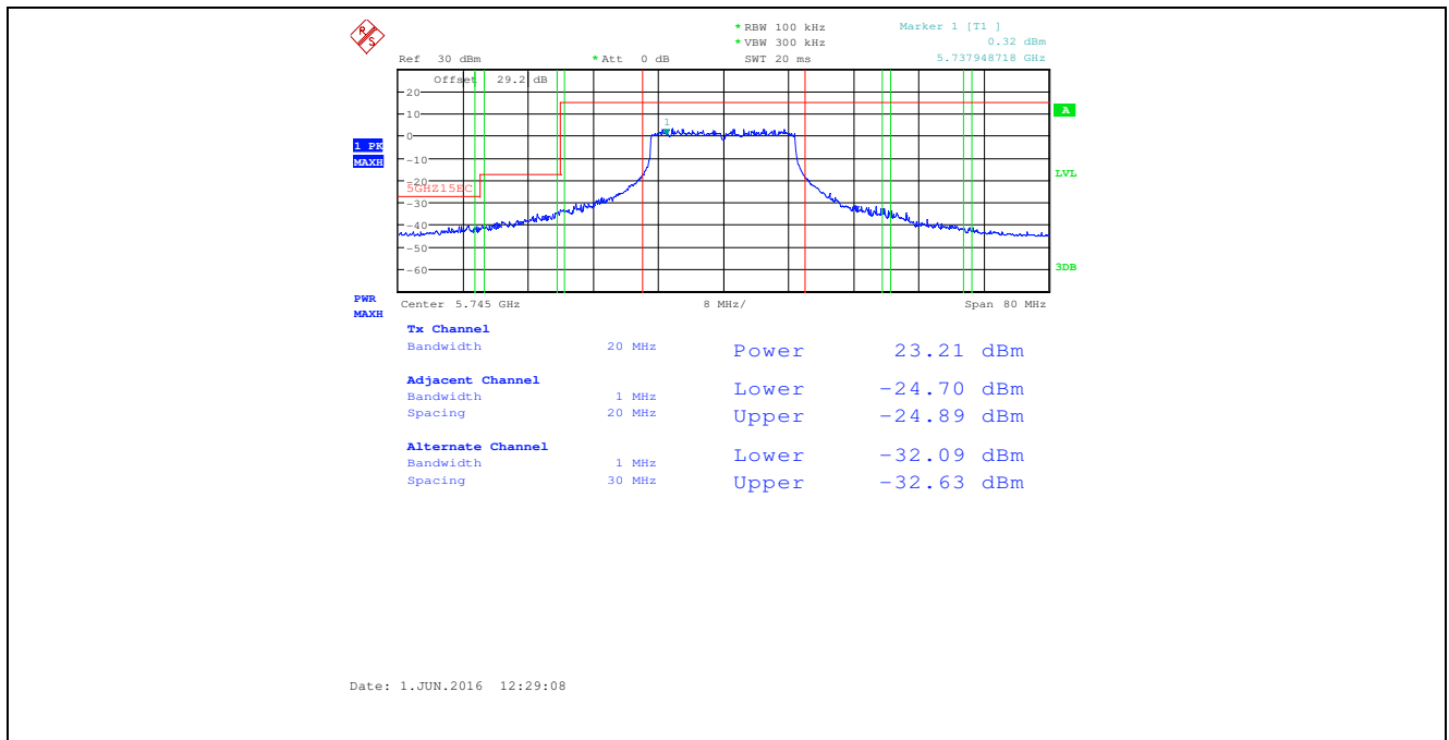
Plot 5.3.4.1.15. Band-Edge Conducted Emissions, 802.11an HT20, 65 Mbps, Ch 149, 5745 MHz, PCDAC Power 40, ANT 2 Offset = 29.16dB = 27.16dB Insertion Loss + 2dBi EUT antenna gain, Integration Method
