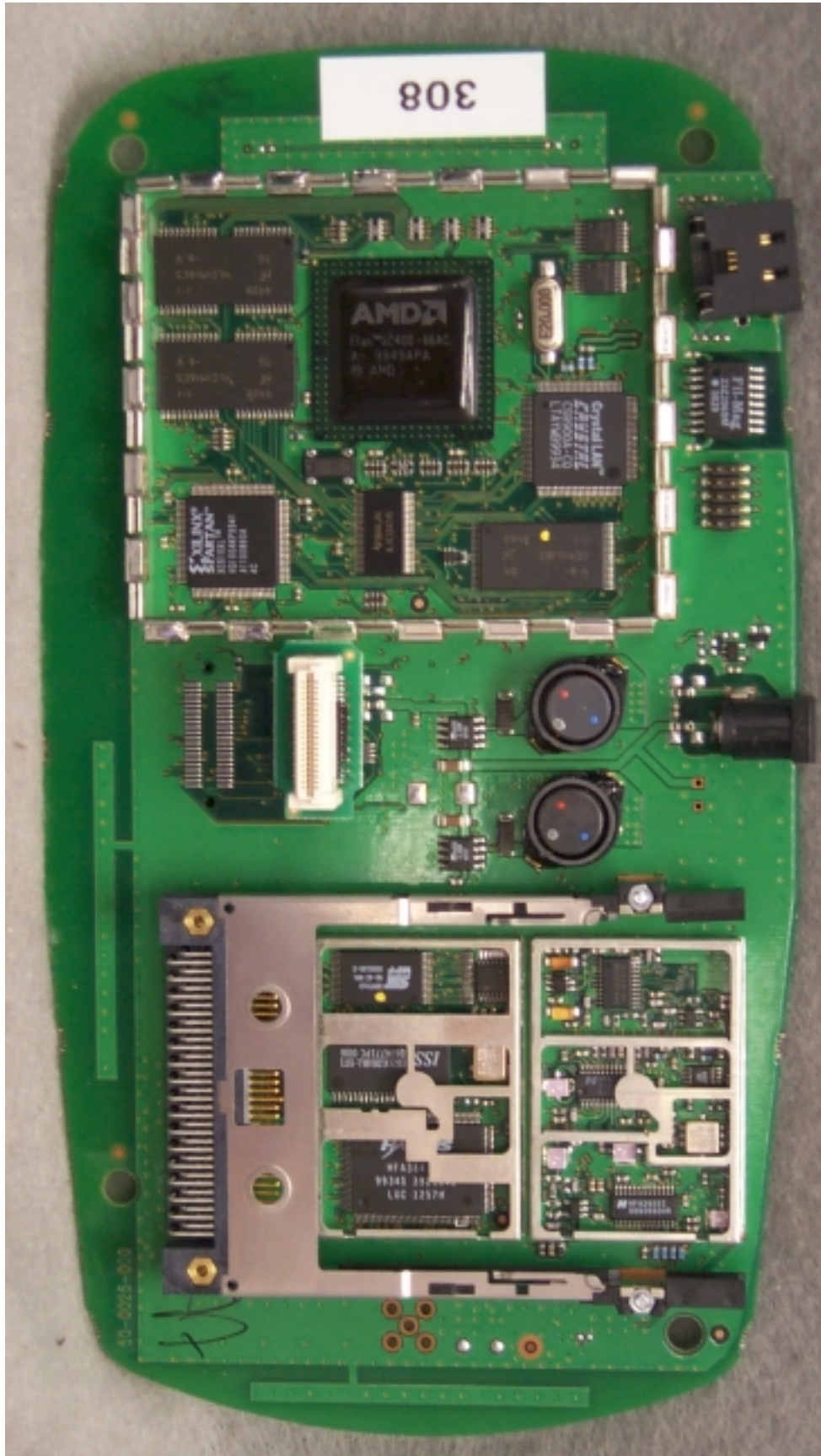
Photo 7. EUT, Top View of Board with Shields Removed
