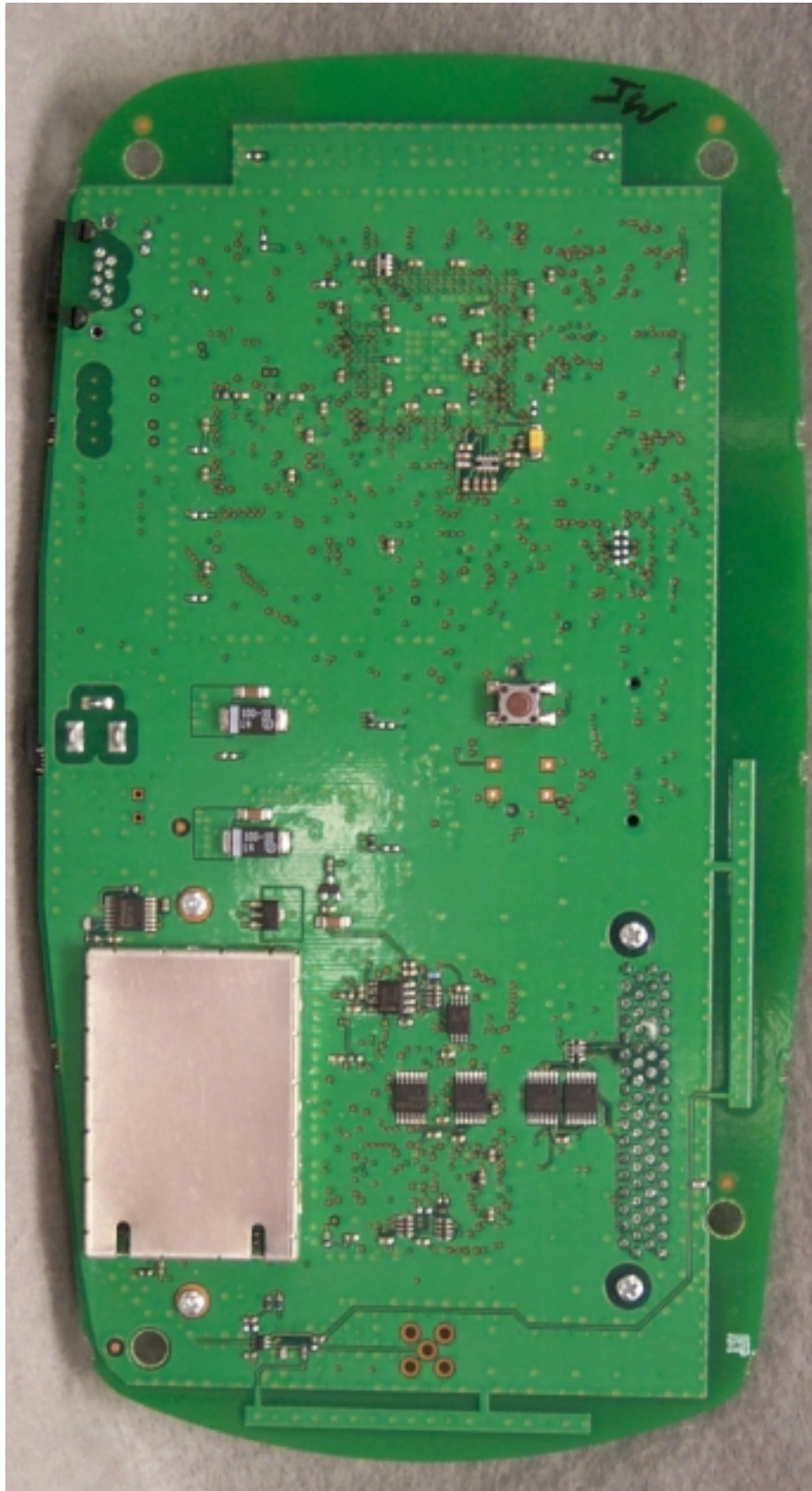
Photo 8. EUT, Bottom View of Board
