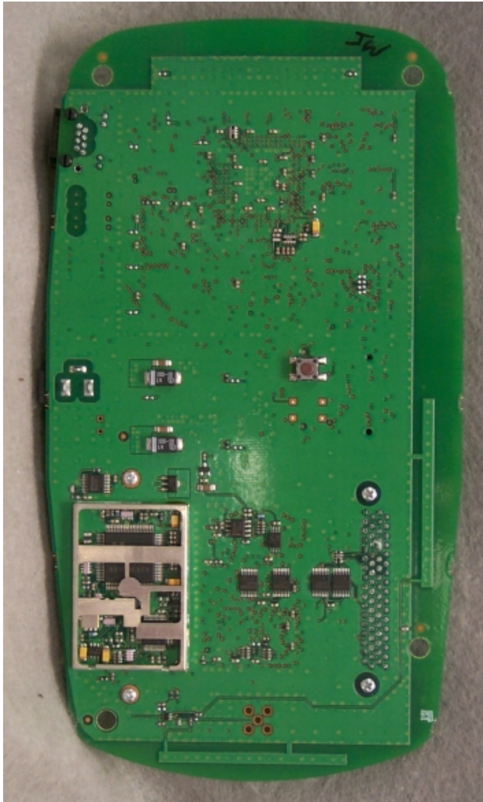
Photo 9. EUT, Bottom View of Board with Shields Removed
