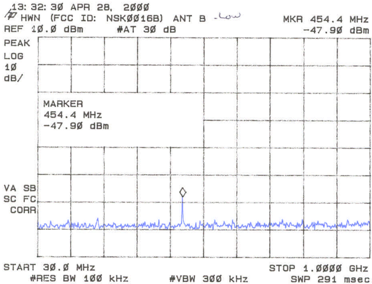
Figure 4m Antenna Conducted Spurious Emissions 15.247(c) (Antenna B - Low)
