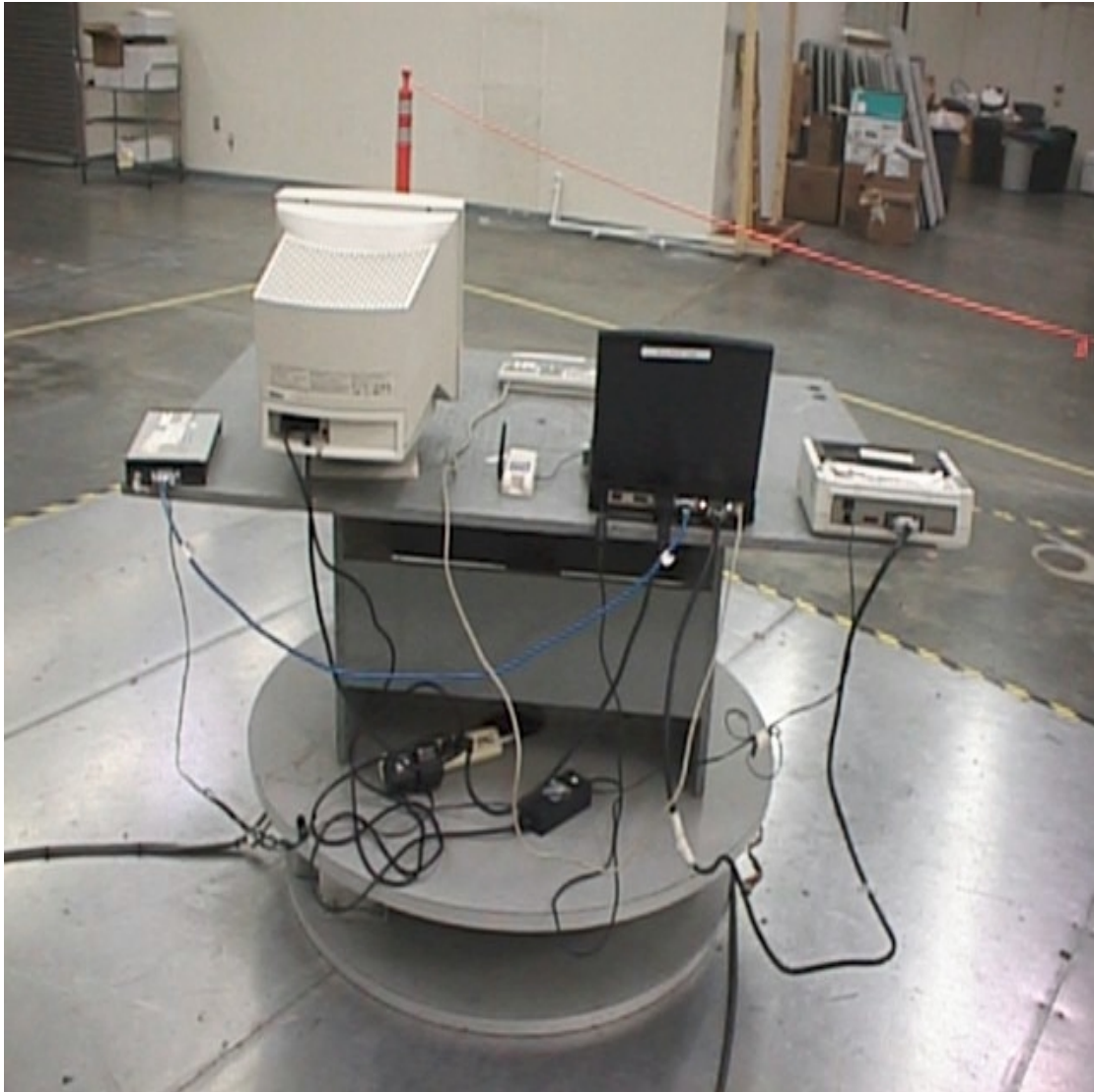
RADIATED EMISSIONS TEST SETUP; BACK SIDE
