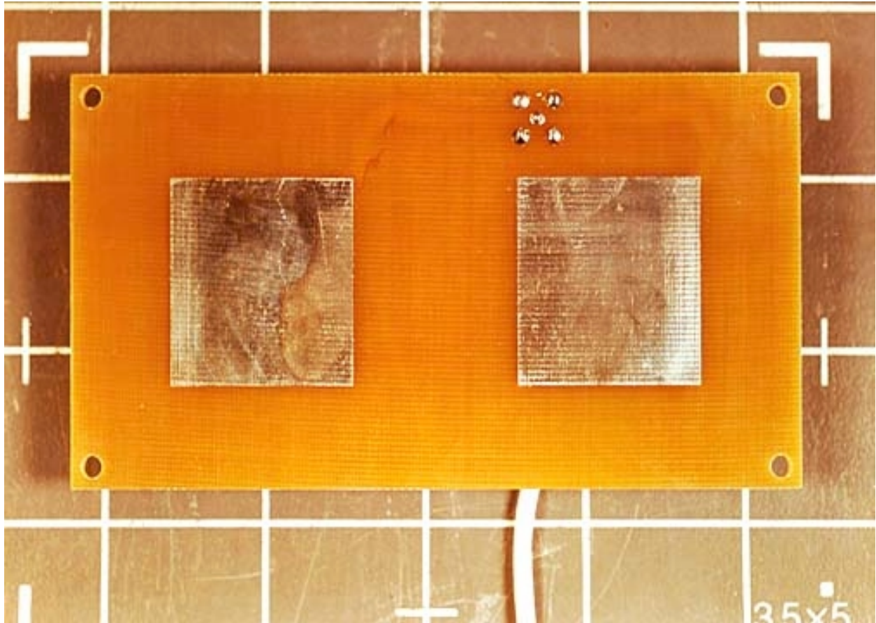
Top PCB in Patch Antenna
