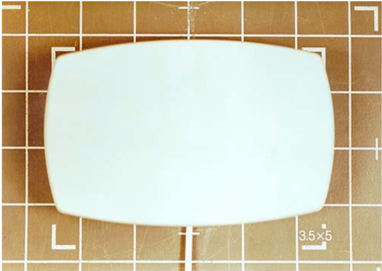
Top Patch Antenna
