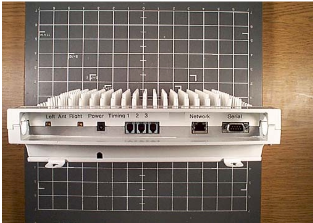
End Showing Ports
