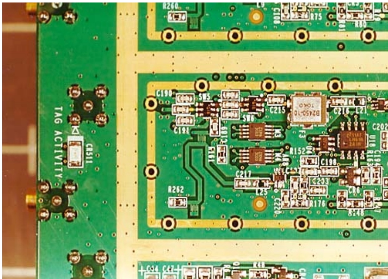
Bottom Front PCB #2 – Top 2
