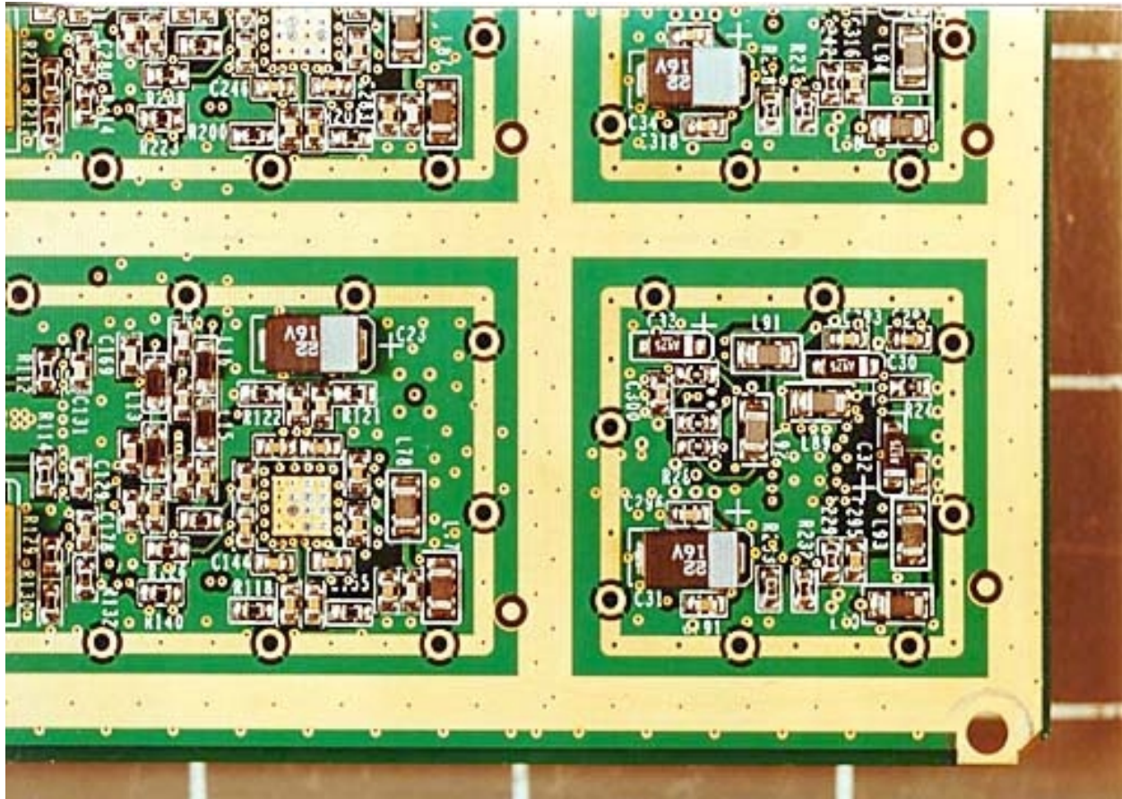
PCB #2 - Back Center 1
