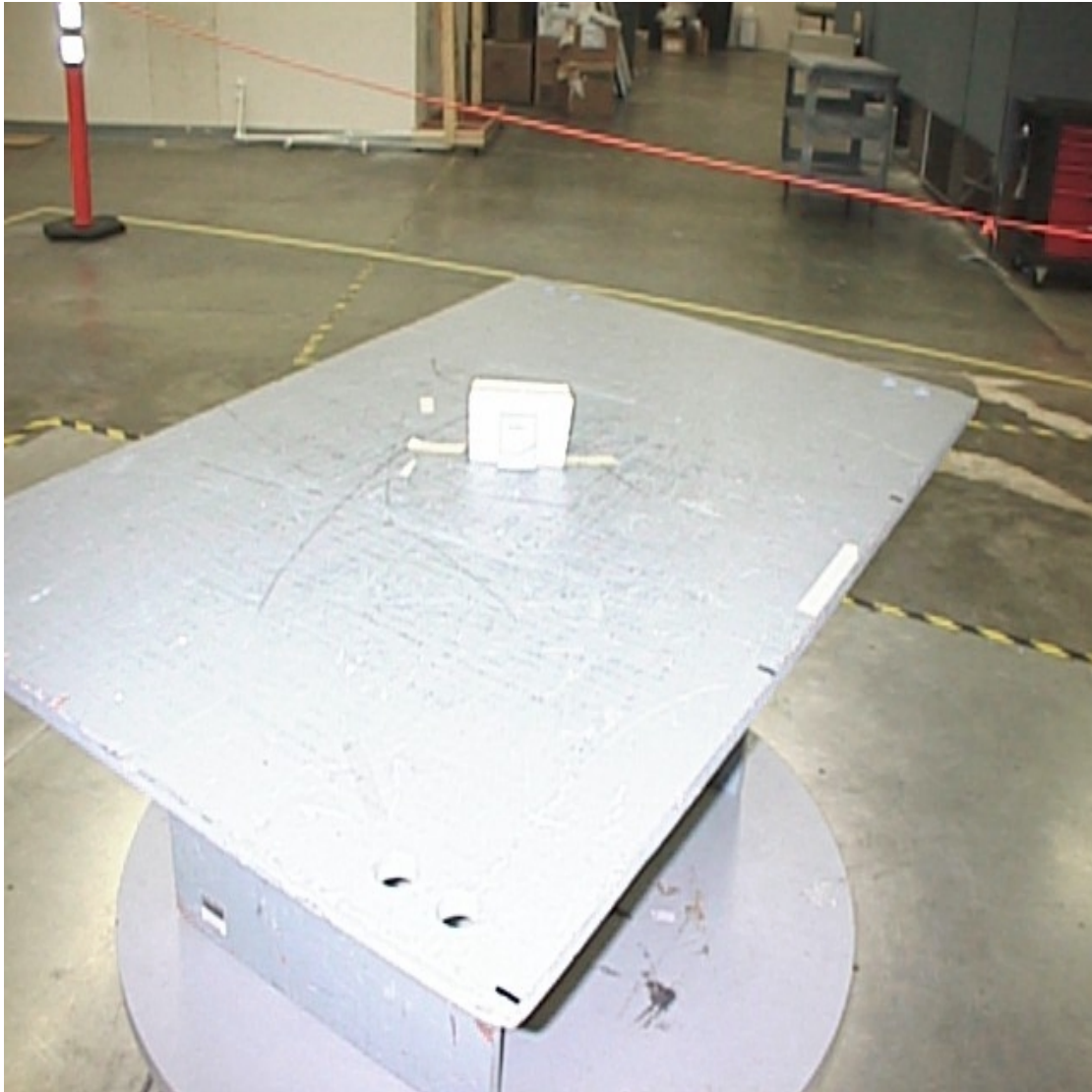
RADIATED EMISSIONS TEST SETUP PHOTO FOR TAG
