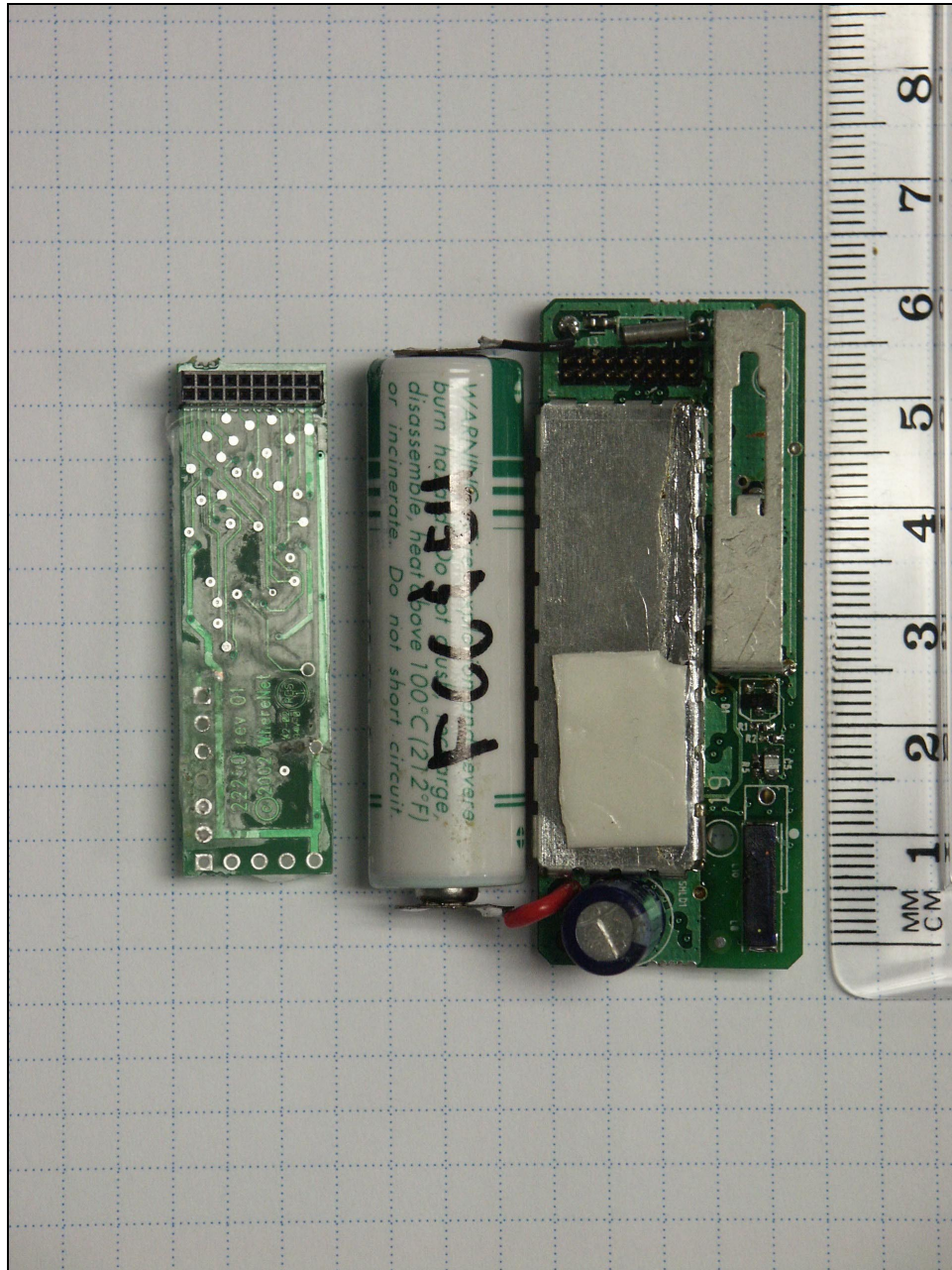
Inside Front PCB 1 and 2
