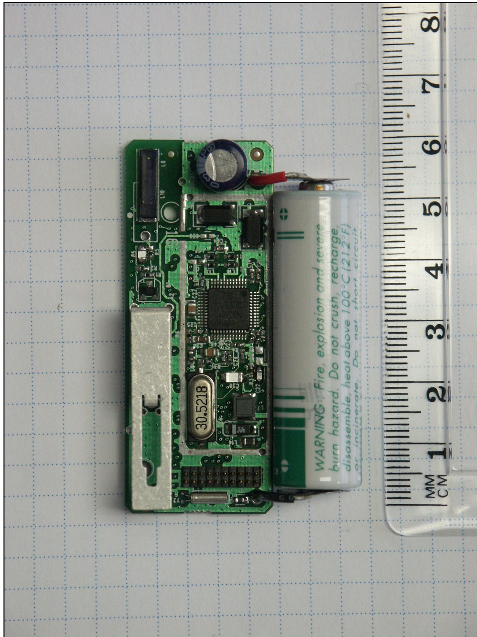
Inside Front PCB 1 without shielding
