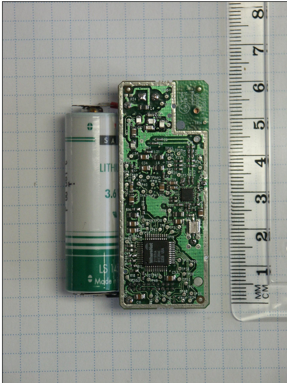
Inside Back PCB 1 without shielding
