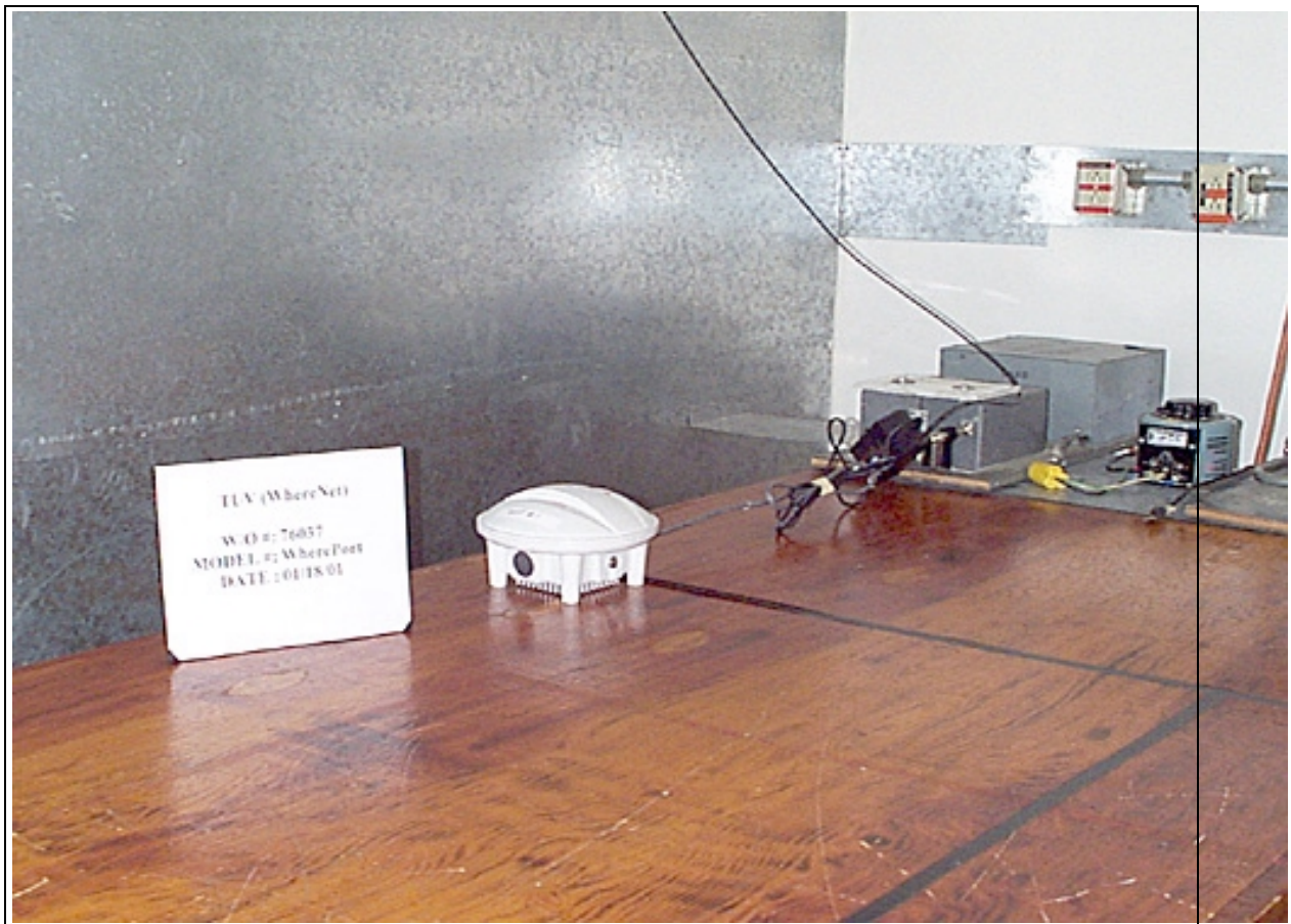
Conducted Emissions
