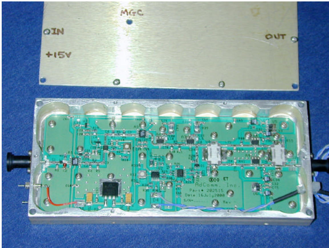
Photo 6 - MGC Amplifier
