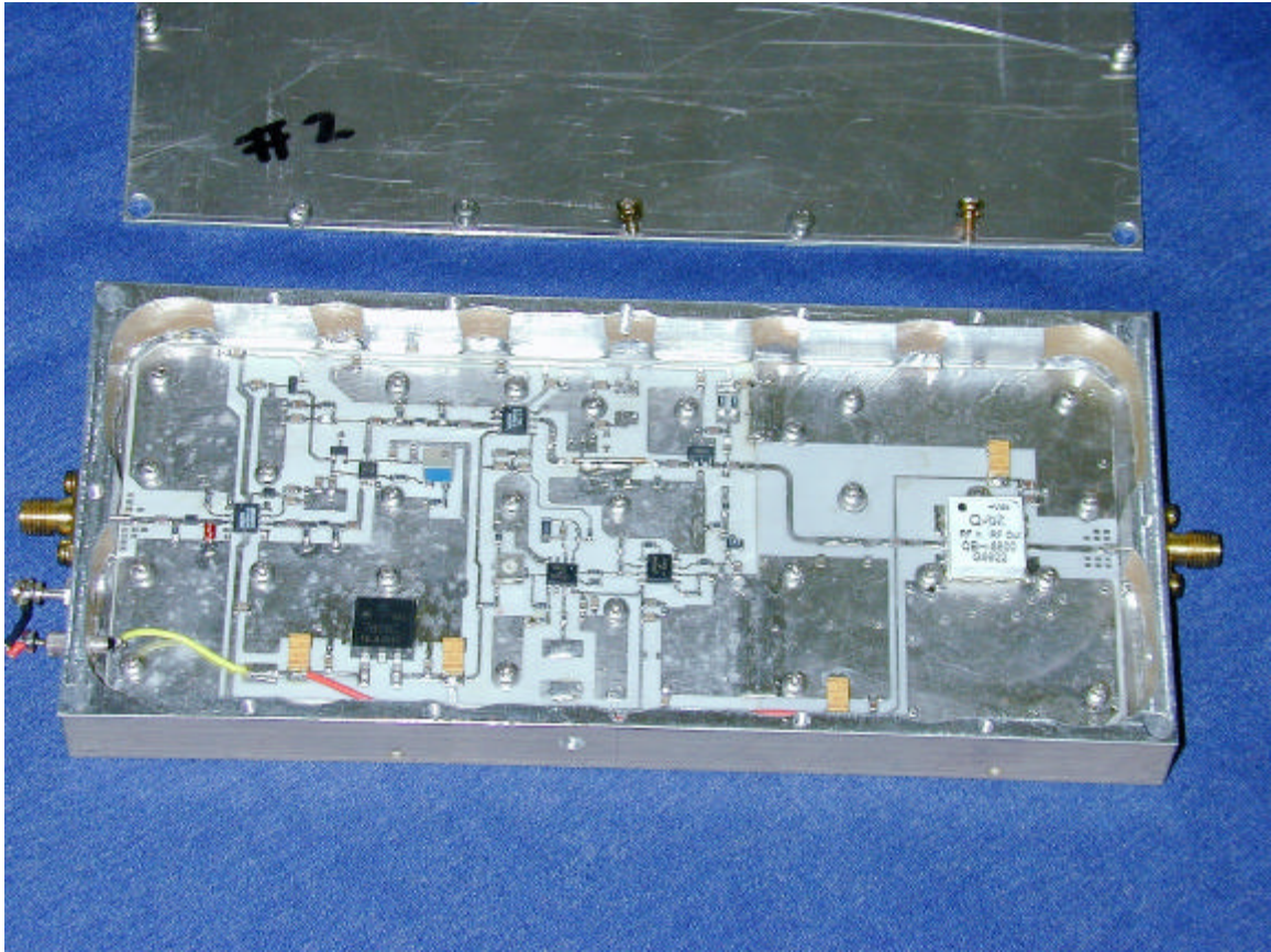
Photo 3 - AGC Amplifier
