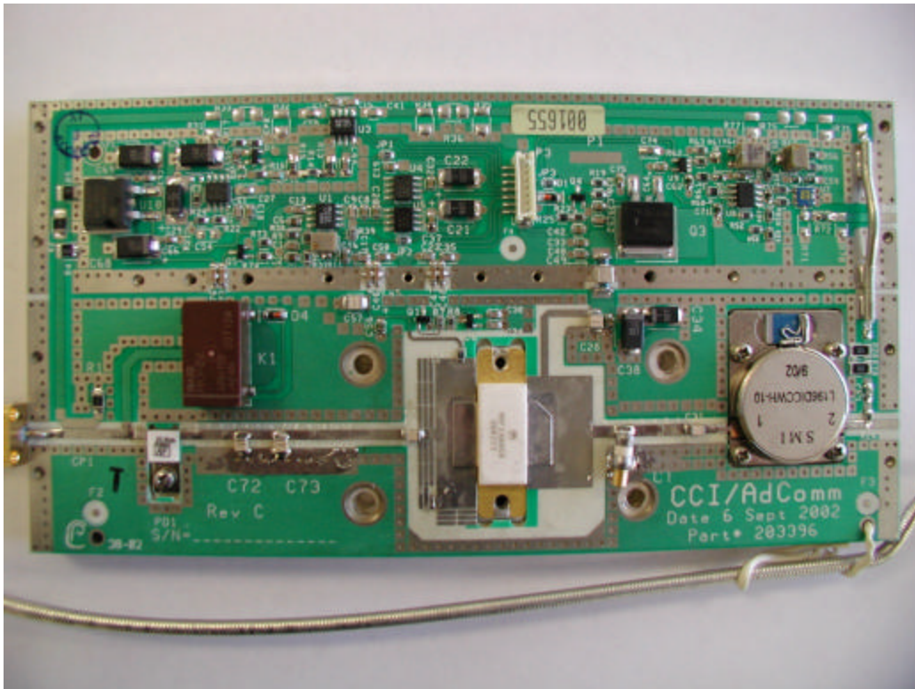
Amplifier Front
