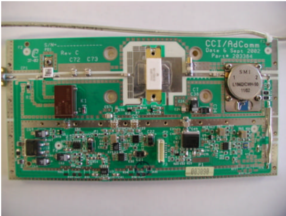
Amplifier B Front
