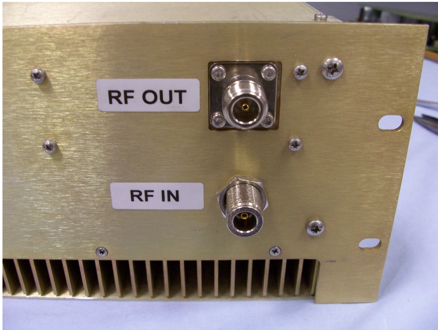
RF CONNECTORS
