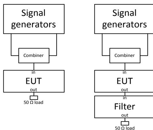
Figure 3.6-1: Setup diagrams
