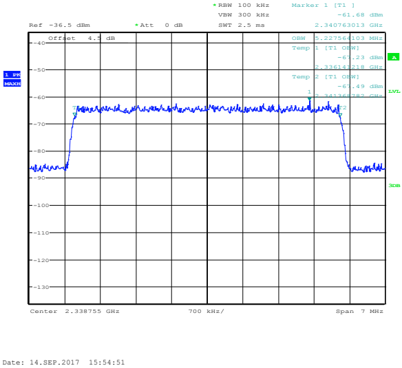
Figure 8.1-3: 99 % bandwidth on high band, input
