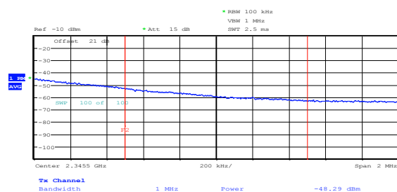
Figure 8.4-7: Spurious emissions at the upper band edge at 2.345 GHz, configuration without external filter
