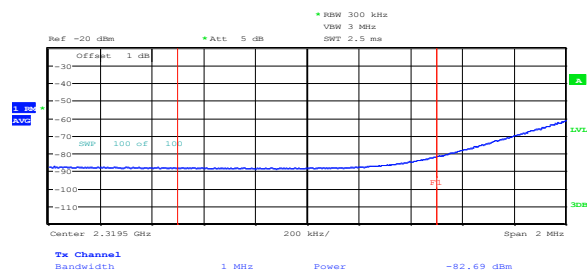
Figure 8.4-1: Spurious emissions at the lower band edge at 2.32 GHz, configuration with external filter
