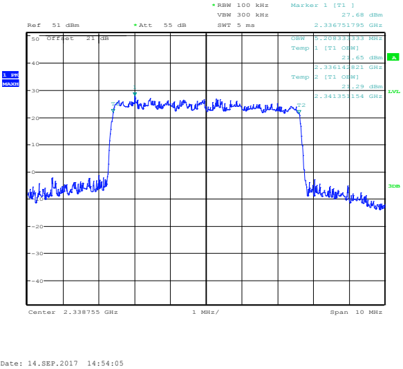
Figure 8.1-4: 99 % bandwidth on high band, output
