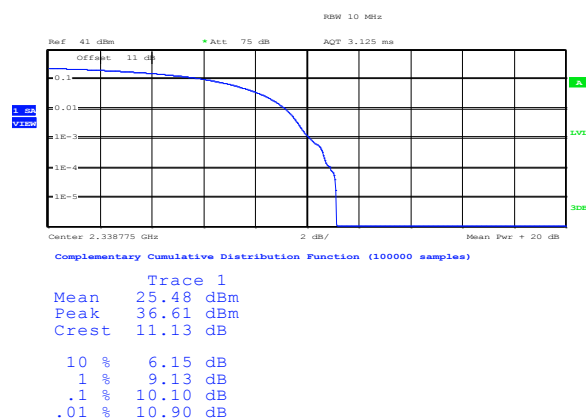
Figure 8.3-2: PAPR on high band
