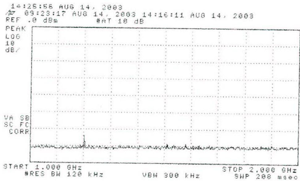
Figure 5.2. Emissions measured at 3 meters in anechoic chamber, 1000-2000 MHz. (top) Receiver plus ambient (bottom) Ambient
