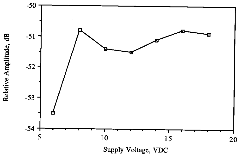
Figure 6.2. Relative emission at "fundamental" vs. supply voltage.
