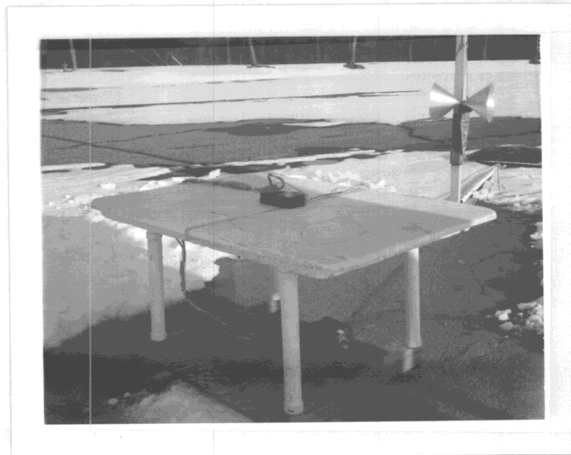
Figure 5.4. DUT on the open-site test table showing the overall view the site.
