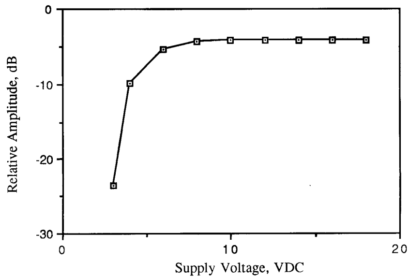
Figure 6.4. Relative emission at 134 kHz vs. supply voltage.
