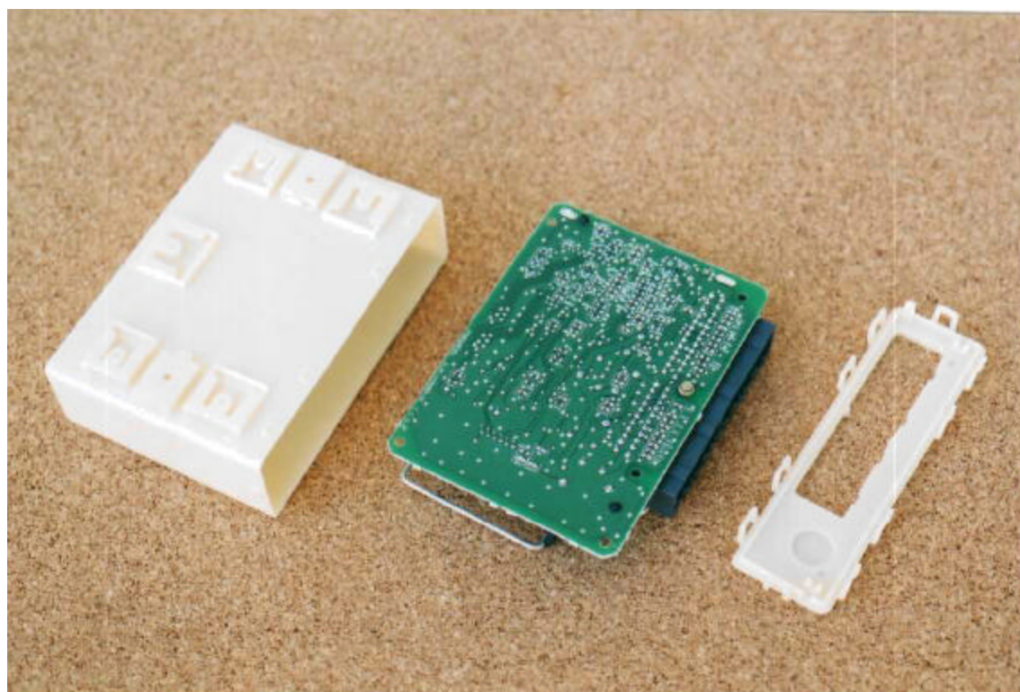
Disassembled DUT, PN: 1L1T-15K602-AE
