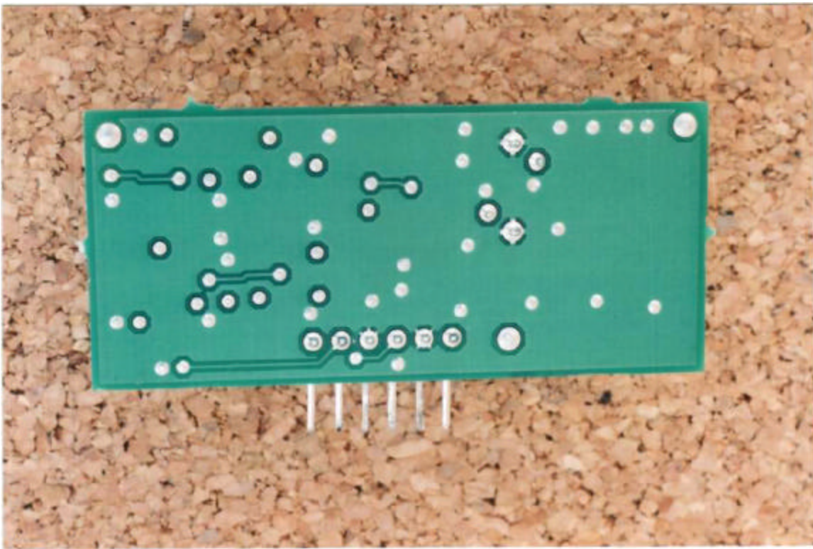
Receiver RF Board. Same used on all versions
