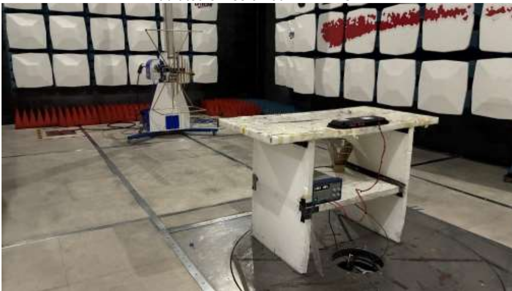
Radiated emission 30 MHz – 1 GHz
