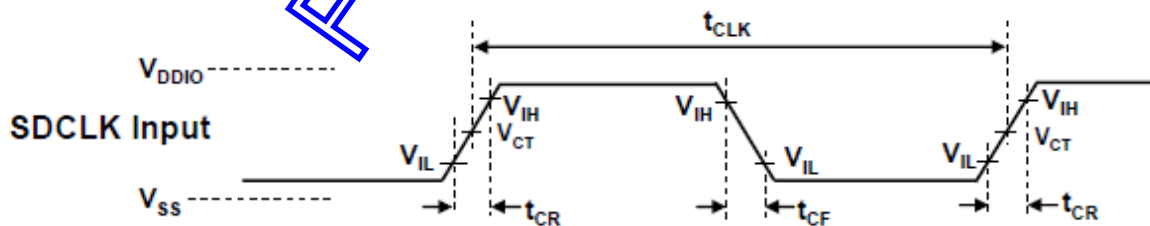
Figure 20. SDR12 、SDR25、SDR50 and SDR104 mode clock signal timing
