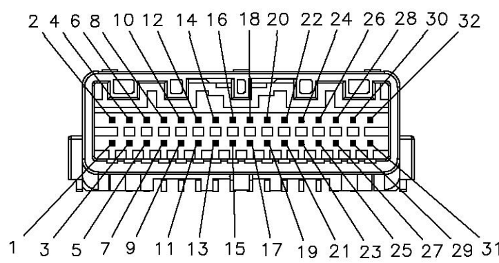
32 WAY MDL MAIN CONNECTOR (NCB00053-A, BOARD SIDE)
