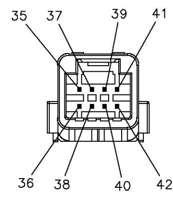
8-WAY CONNECTOR (PCB00111-A, BOARD SIDE)
