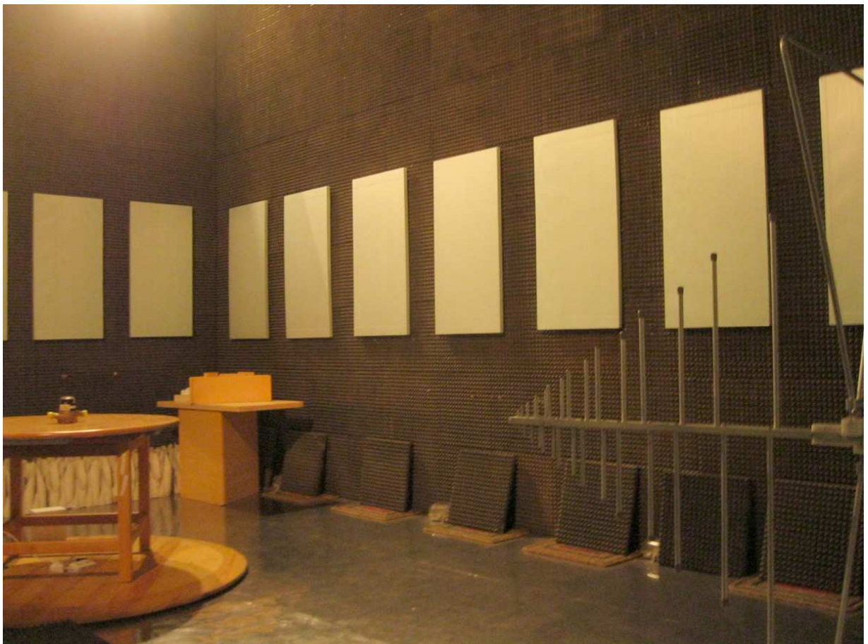
Figure 2.5.2 Radiated measurement
