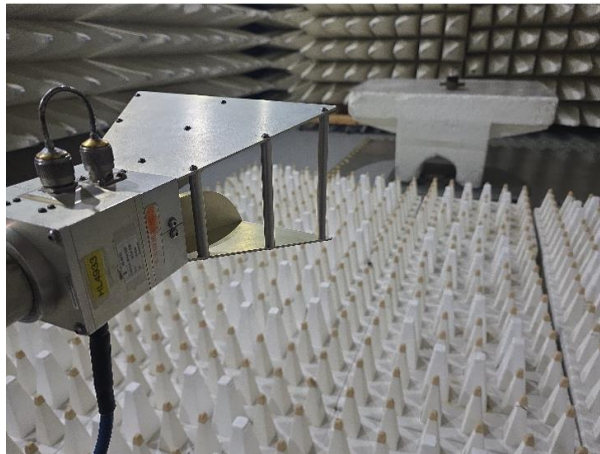
External Antenna
