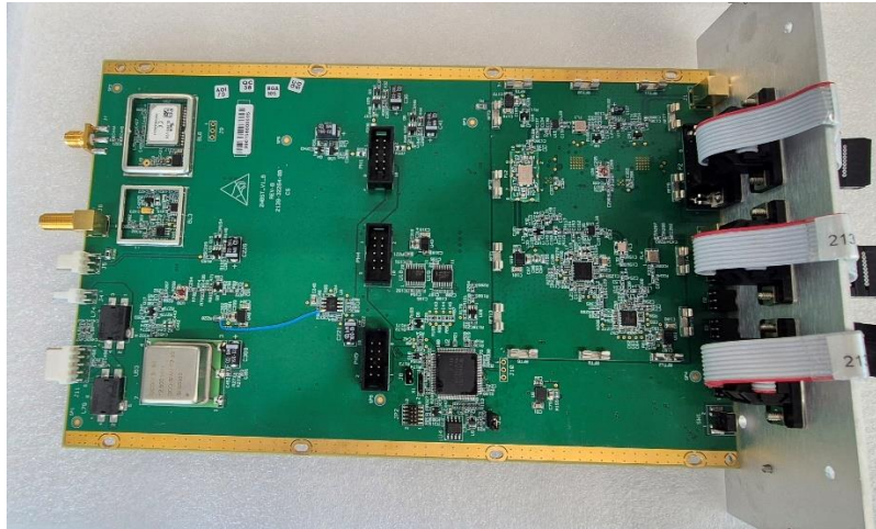
PCB CS side
