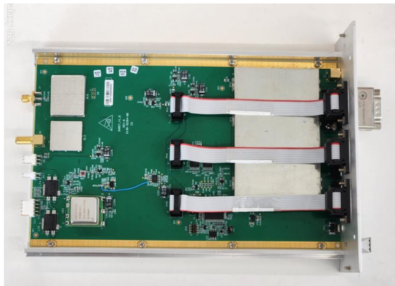
Galaxy Base Station V1- RF transceiver internal view
