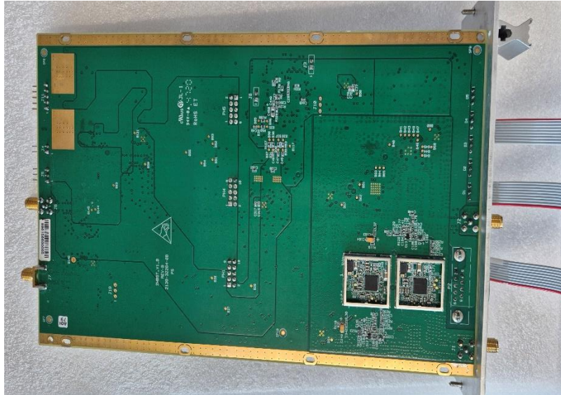
PCB PS side
