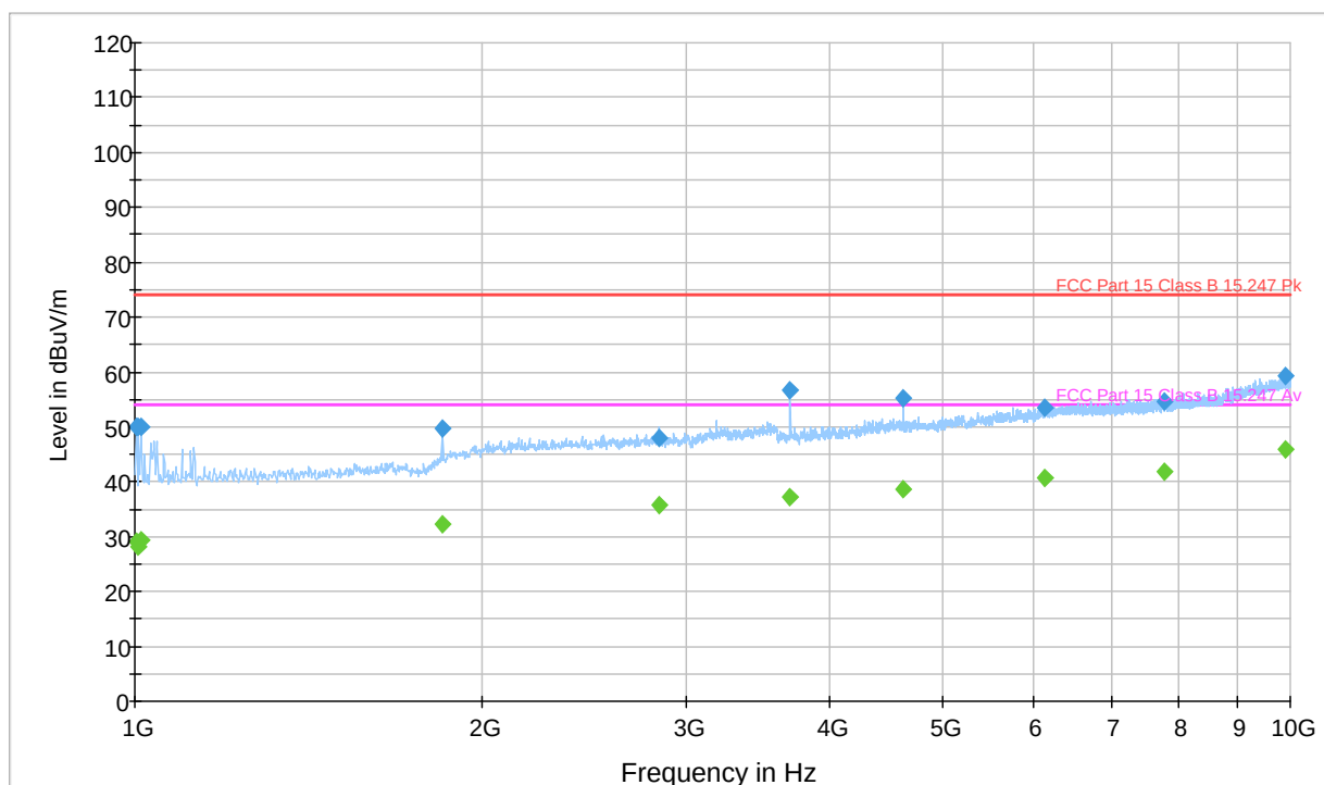
Plot 3.2.4 Radiated emission measurements from 1000 MHz to 10000 MHz at the 923.546 MHz carrier frequency (BPSK)
