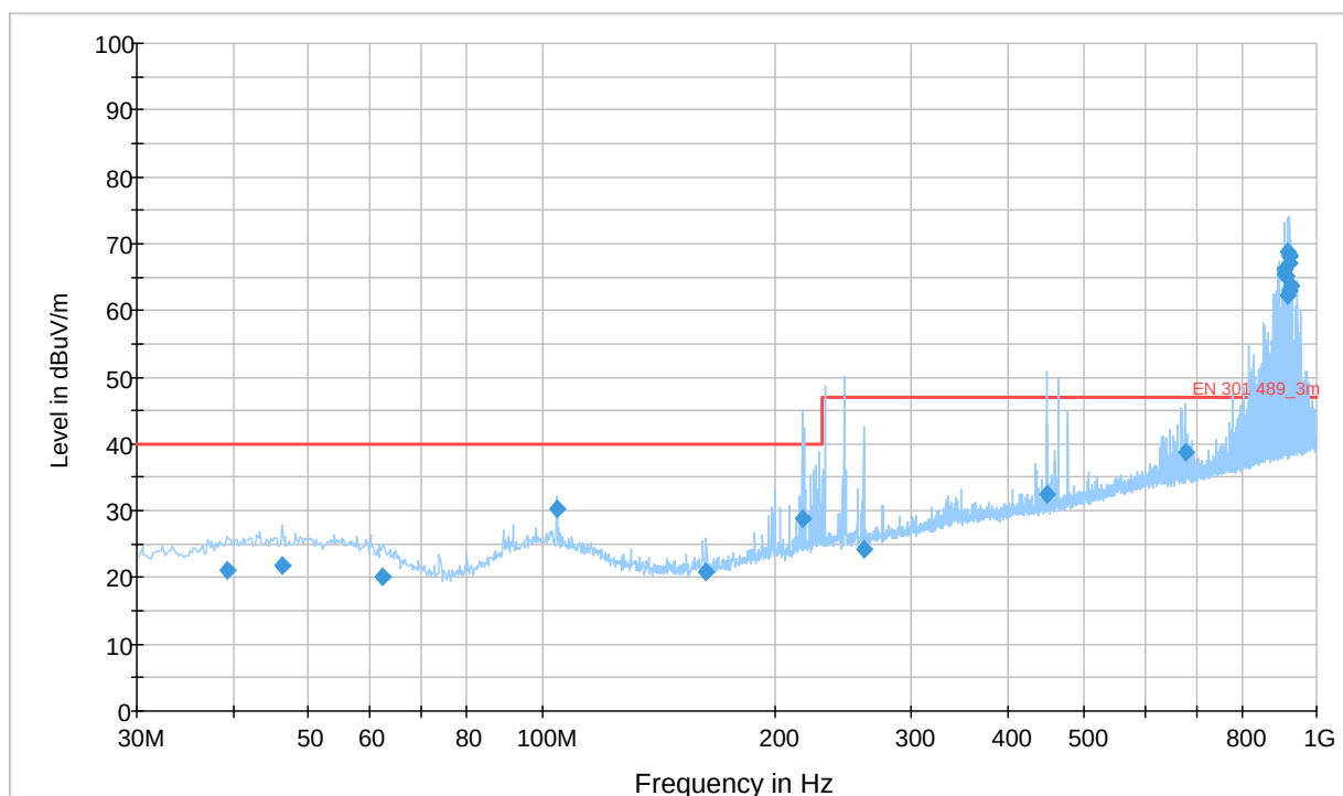
Plot 3.2.5 Radiated emission measurements from 30 MHz to 1000 MHz at the 916.3 MHz carrier frequency (BPSK)
