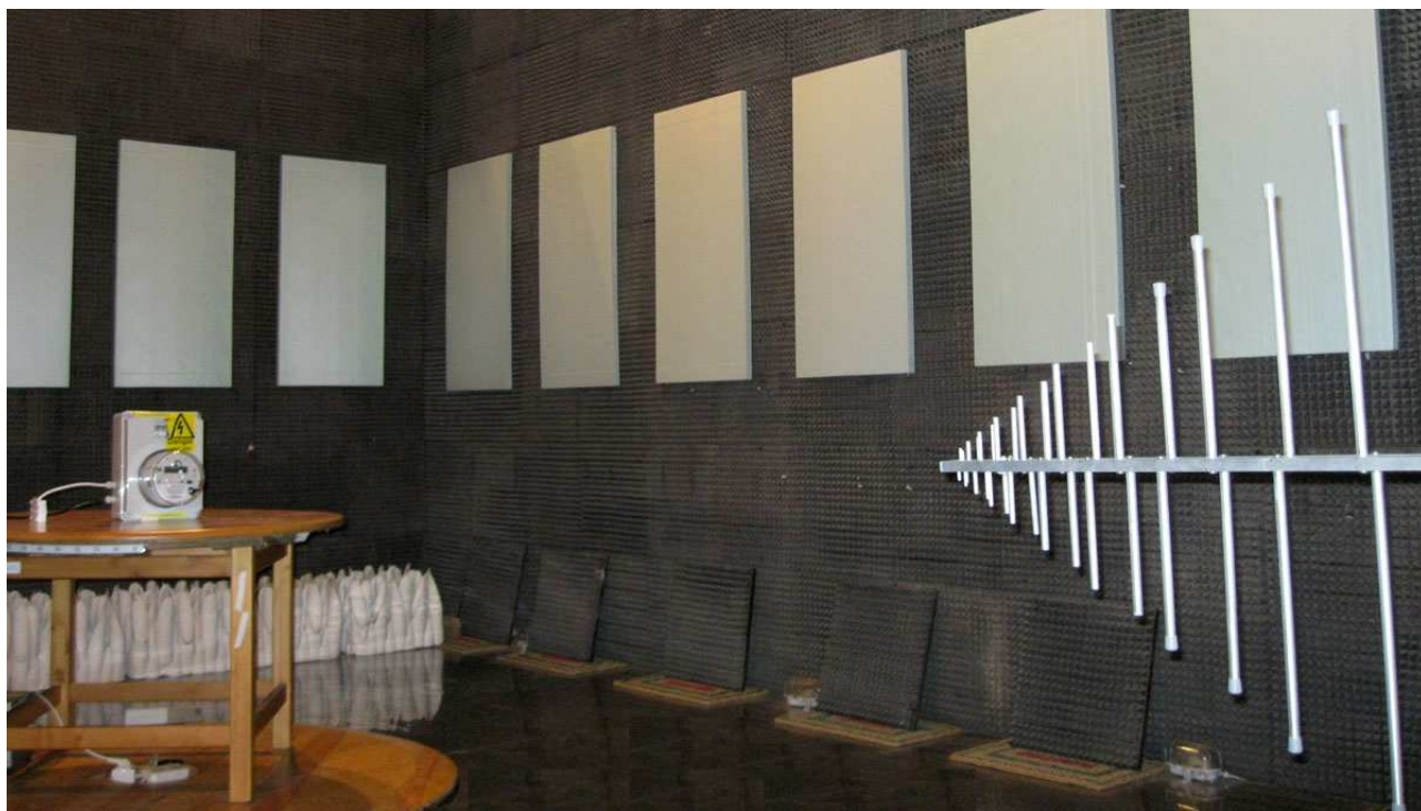
Figure 2.5.2 Radiated measurement
