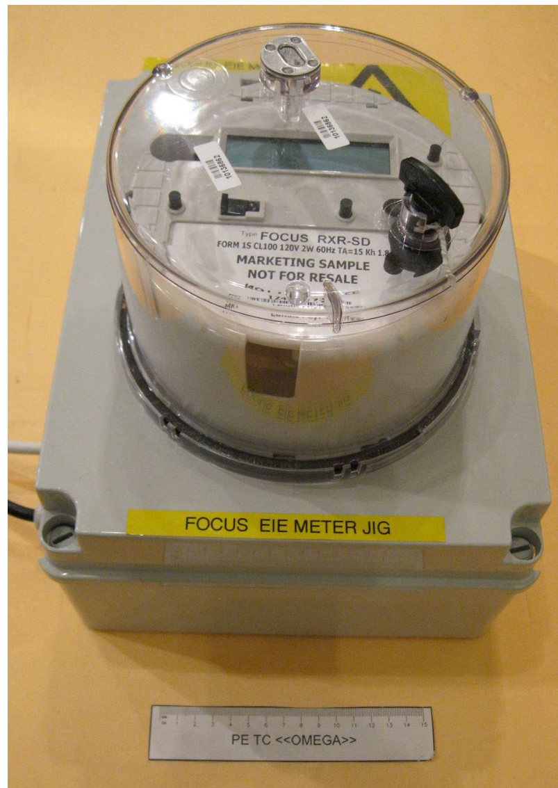
Figure 1.3.2 Front view 2
