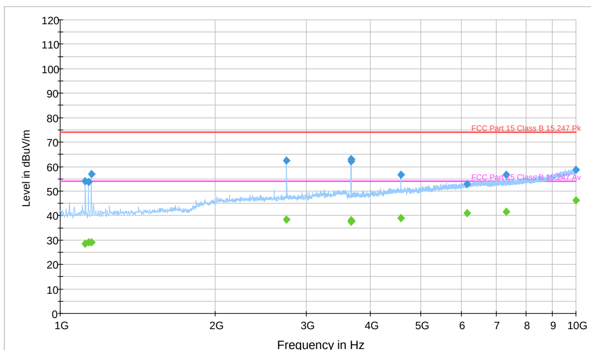
Plot 3.2.2 Radiated emission measurements from 1 GHz to 10 GHz at the 916.3 MHz carrier frequency (FSK) FCC CFR 47 part 15.209 1-18 GHz
