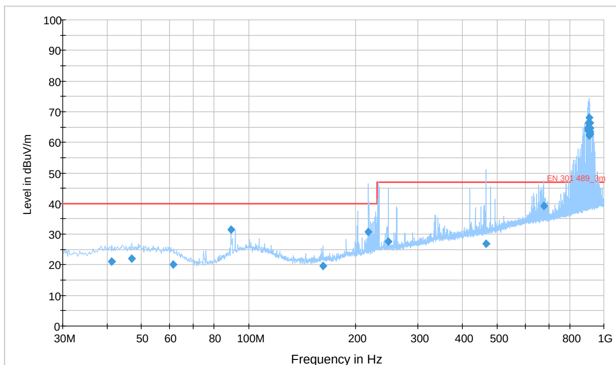
Plot 3.2.7 Radiated emission measurements from 30 MHz to 1000 MHz at the 905.43 MHz carrier frequency (BPSK)
