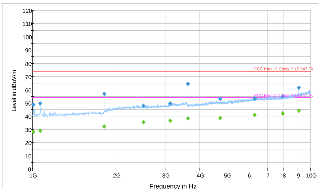
Plot 3.2.8 Radiated emission measurements from 1000 MHz to 10000 MHz at the 905.43 MHz carrier frequency (BPSK)
