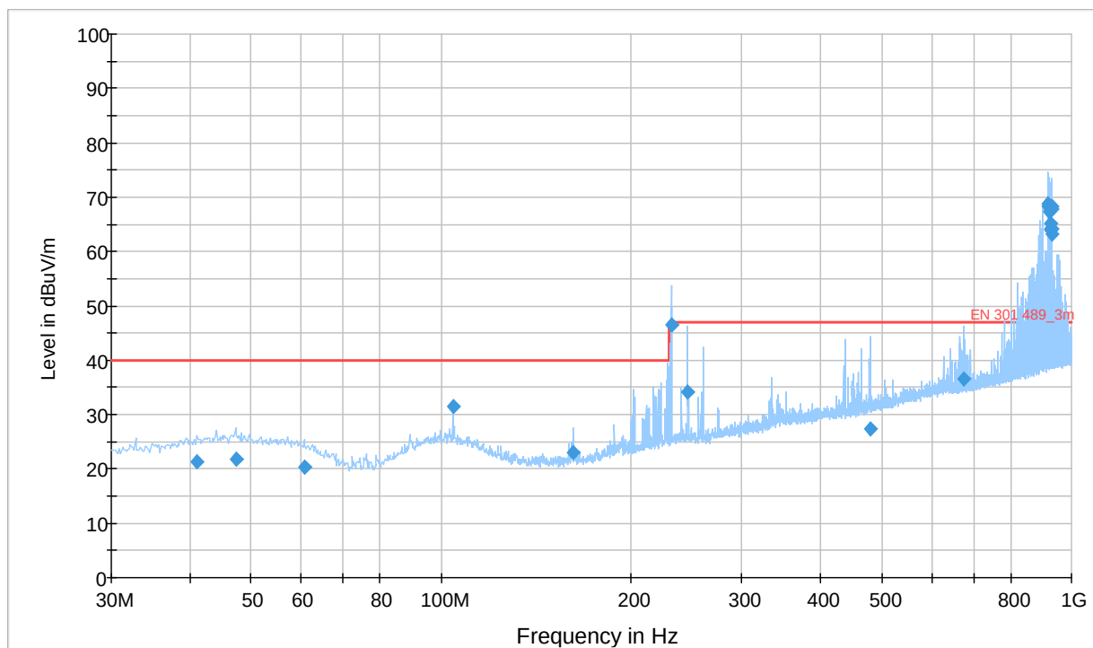
Plot 3.2.3 Radiated emission measurements from 30 MHz to 1000 MHz at the 923.546 MHz carrier frequency (BPSK)
