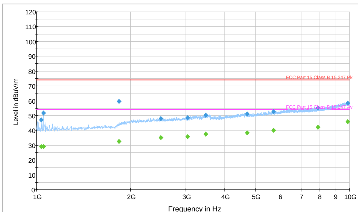
Plot 3.2.6 Radiated emission measurements from 1000 MHz to 10000 MHz at the 916.3 MHz carrier frequency (BPSK)
