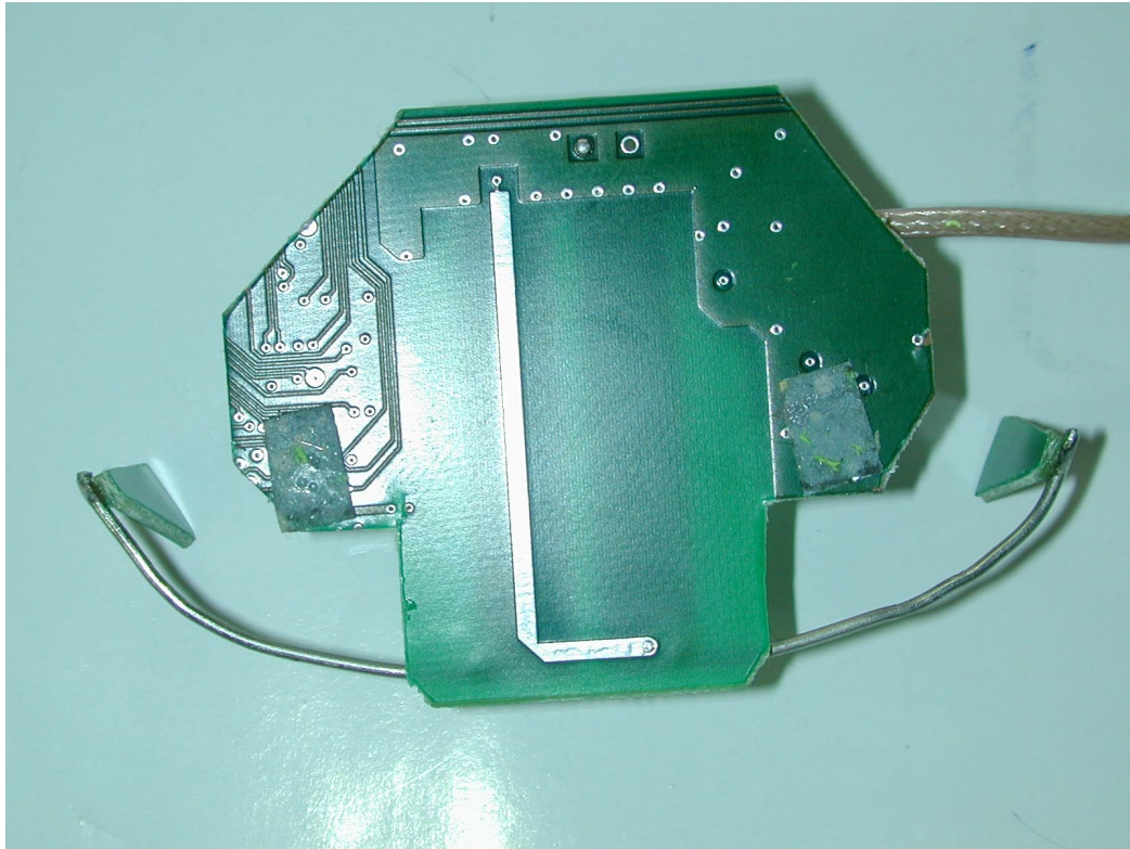
Photograph No.5 FP100HH handheld reader Antenna second side view
