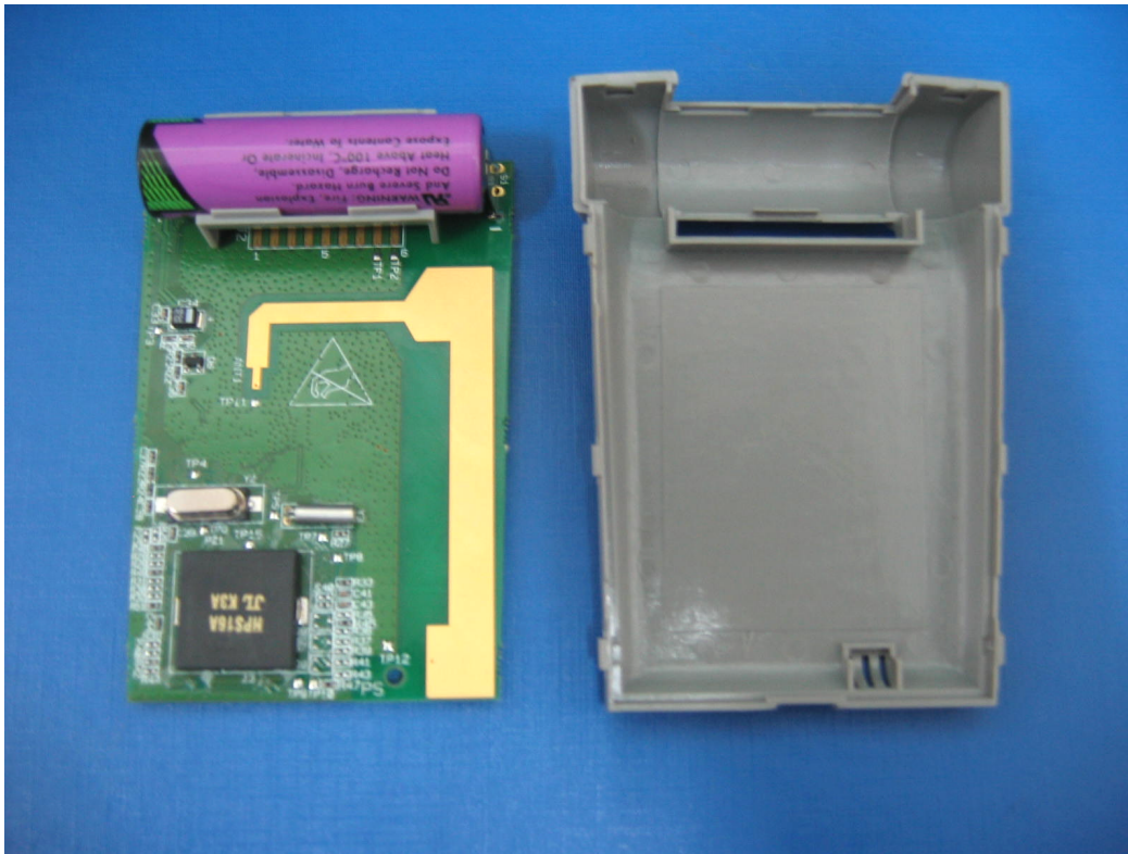
Photograph No.2 FP101TA mobile transponder Internal second side view
