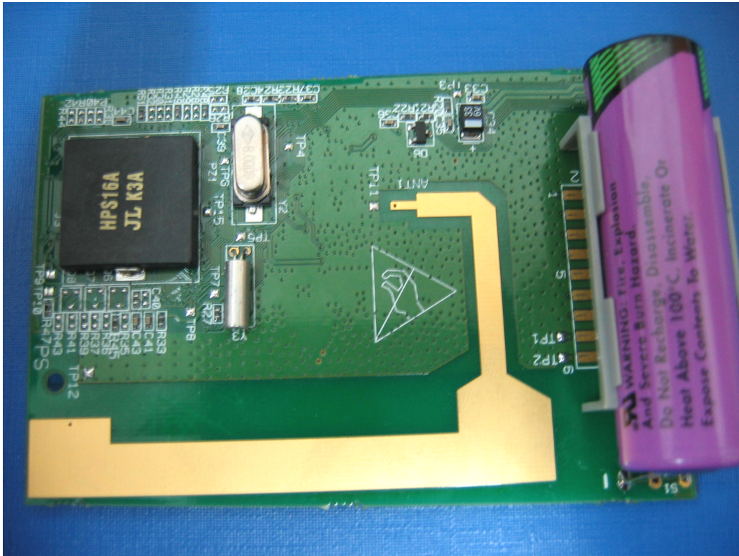
Photograph No.4 FP101TA mobile transponder PCB second side view
