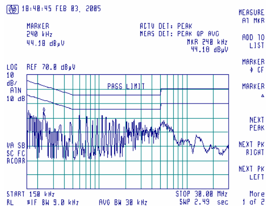
Plot 9.1.2 Conducted emission measurements
