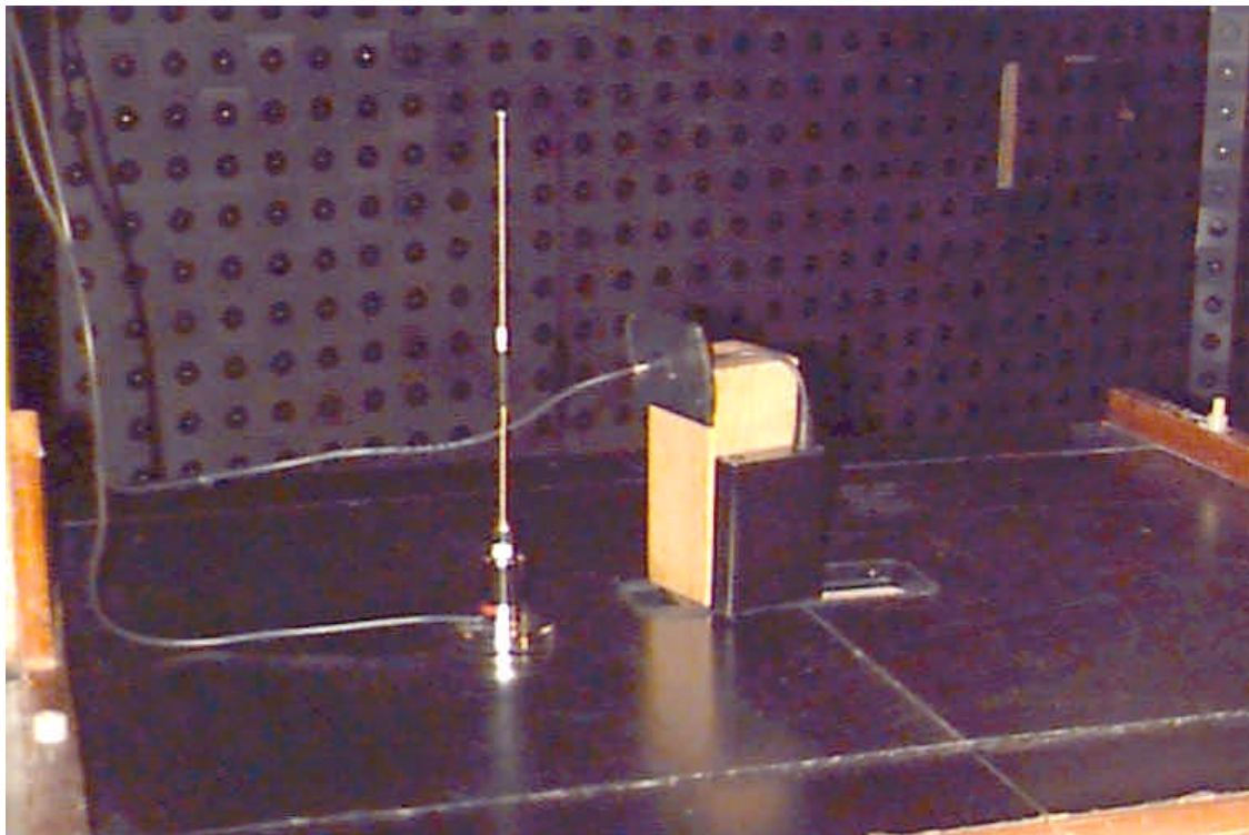
Setup for radiated spurious emission measurements
