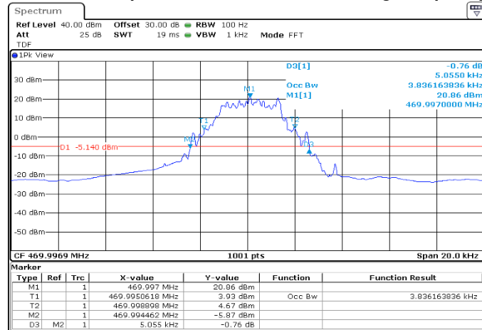
Plot 7.3.3 Occupied bandwidth test result at high frequency
