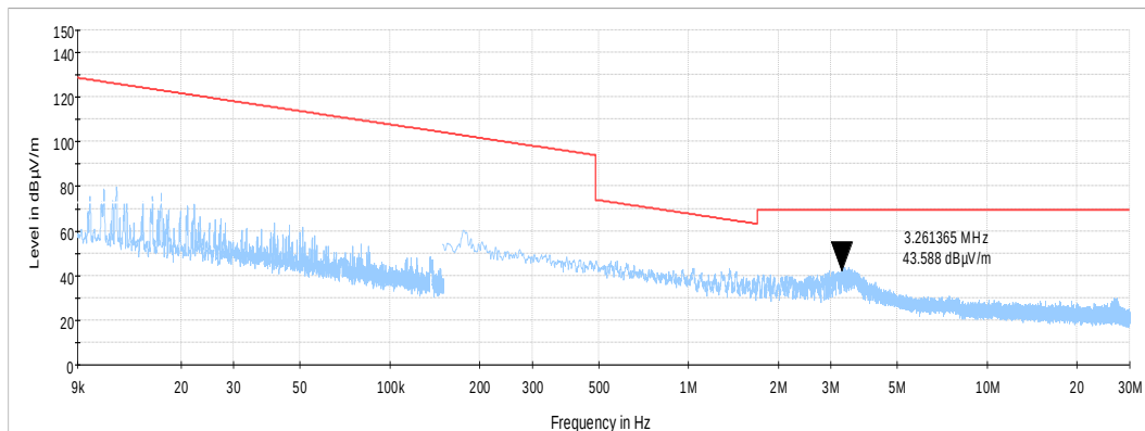
Plot 7.5.5 Radiated emission measurements in 9 kHz - 30 MHz range
