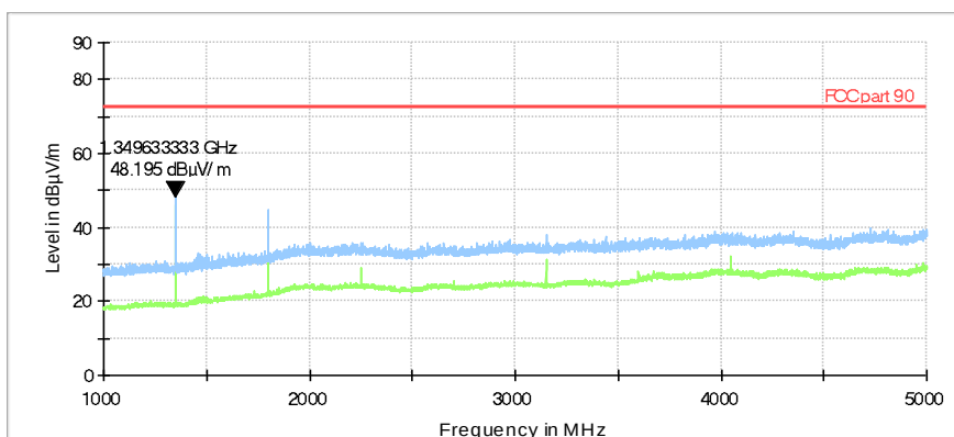
Plot 7.5.14 Radiated emission measurements in 1000 – 5000 MHz range
