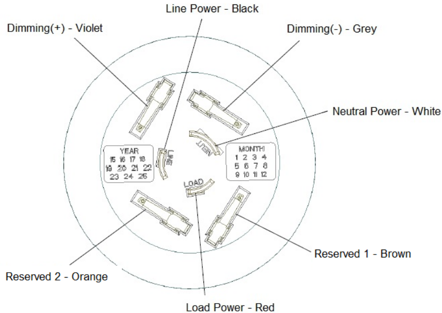
Figure 4 - LCU NEMA 7-Pin Contact Interface
