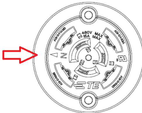
Figure 1 - Top view of the NEMA receptacle showing the North direction
