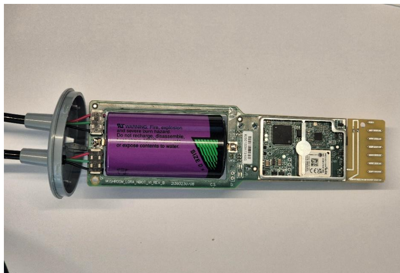
Top side without shield
