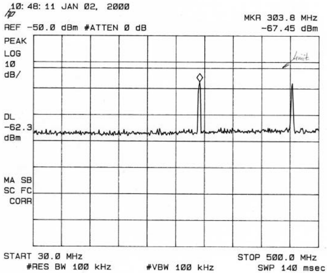
Plot 4.4.5 Spurious emissions
