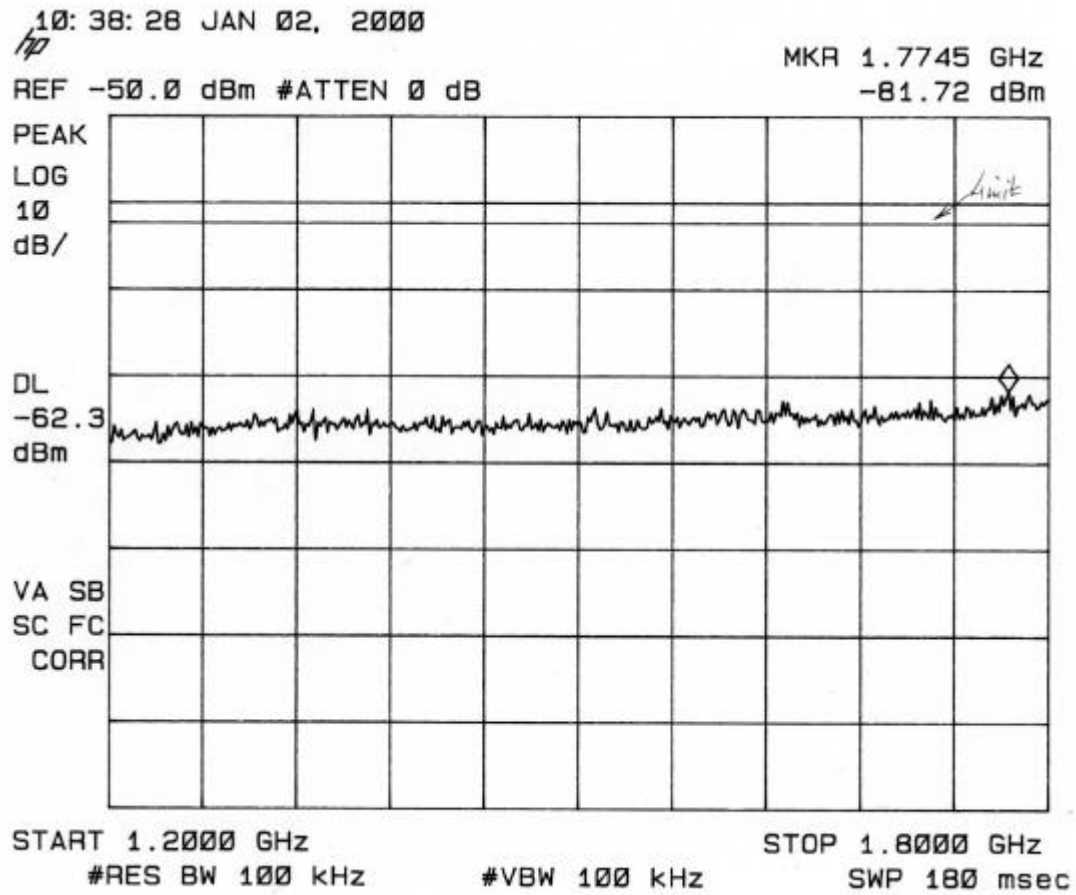
Plot 4.4.8 Spurious emissions
