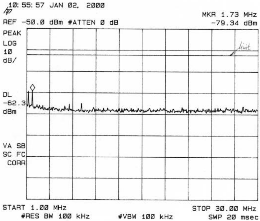
Plot 4.4.4 Spurious emissions
