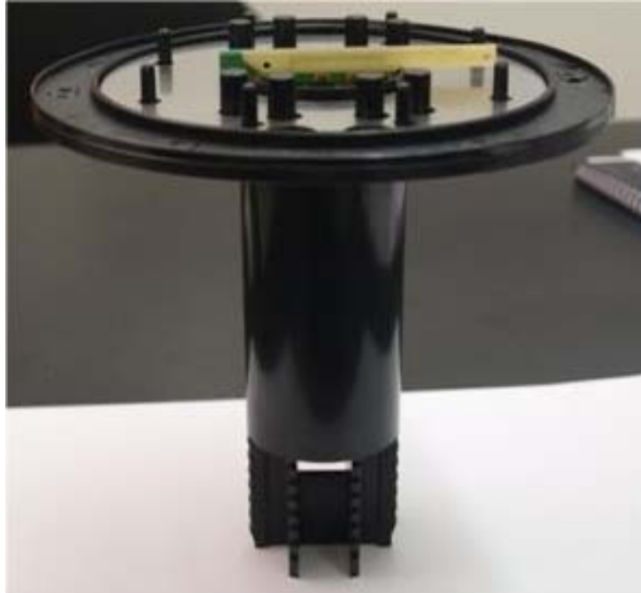
Photograph No.1 Booster 2 with cover removed and integrated printed OMNI antenna
