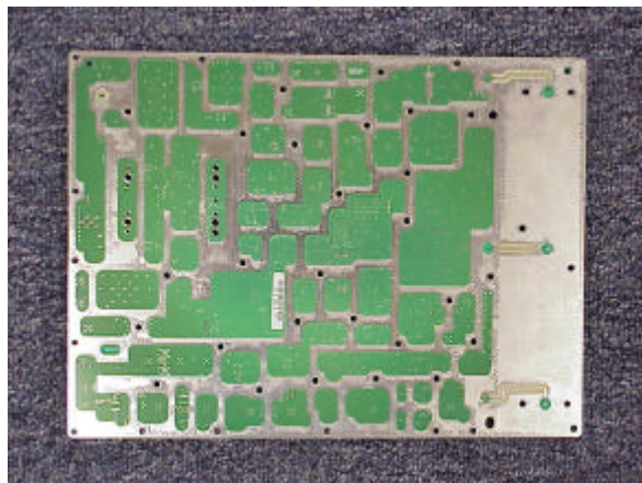
Board Back
