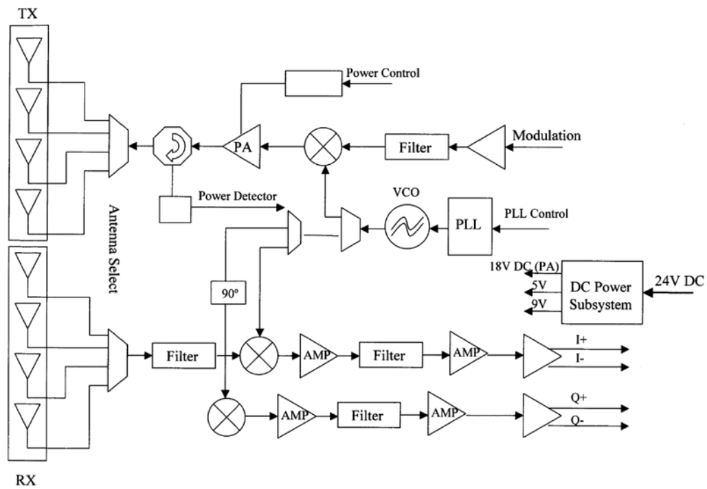
WJSR22XX Block diagram
