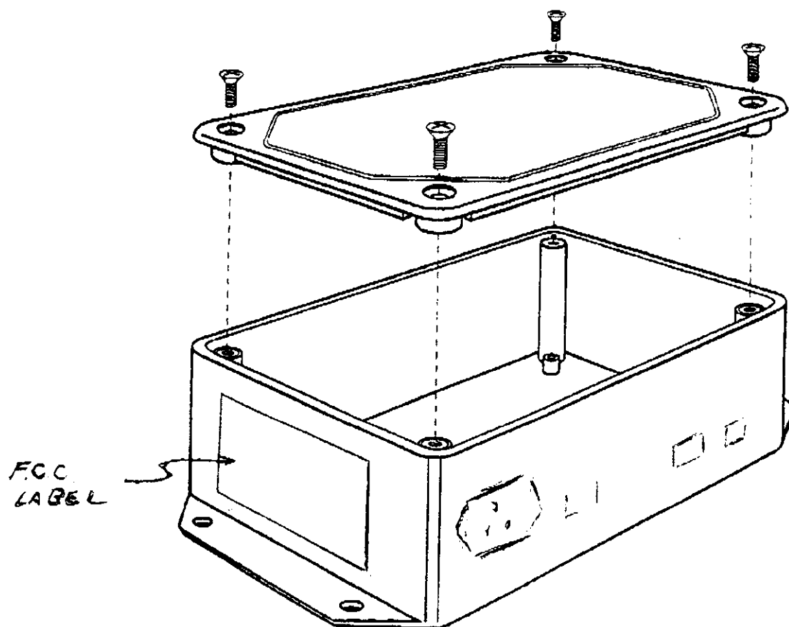
COLLECTOR BASE HOUSING
