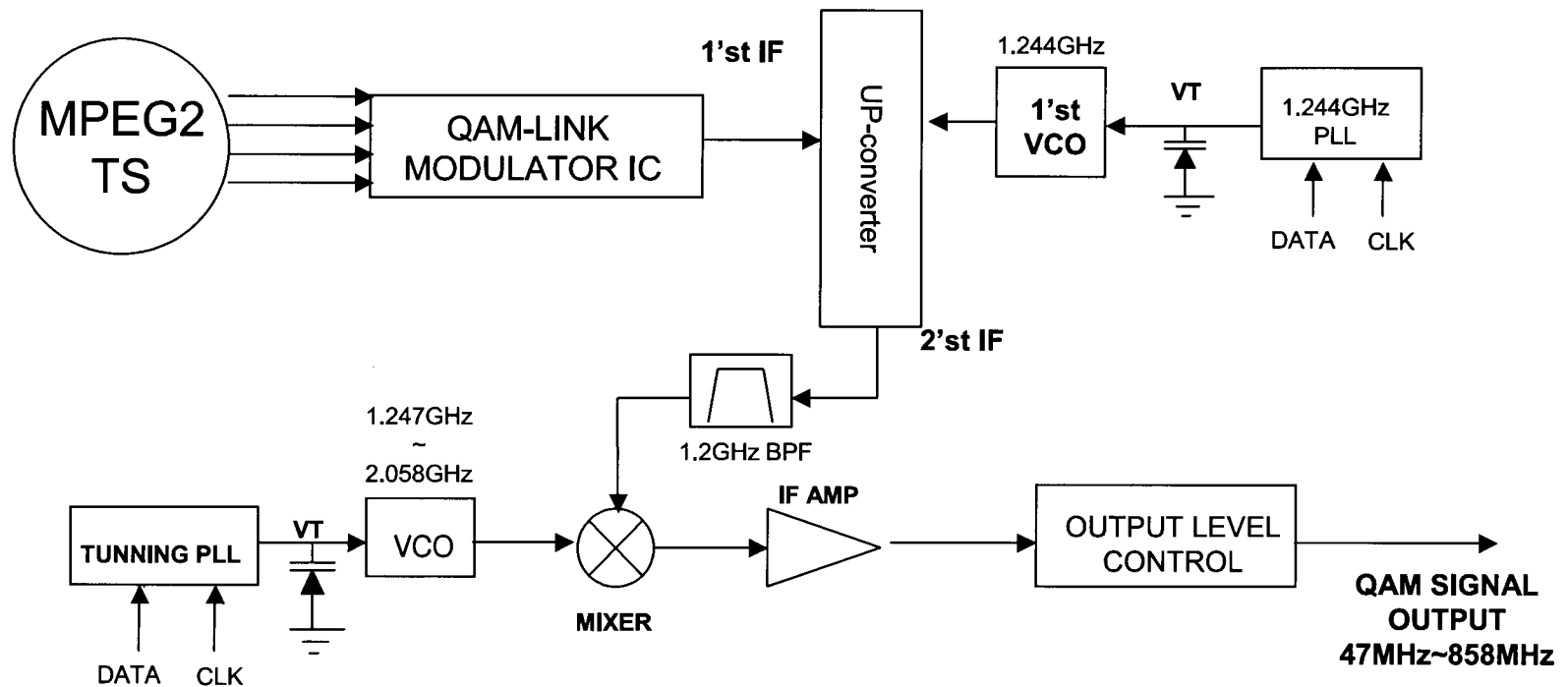
CIRCUIT DIAGRAM NO HST-K2000K
