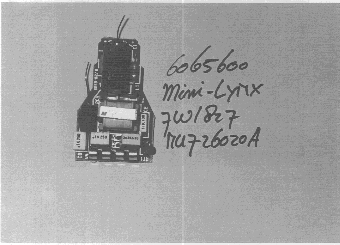
Figure 1-2 interior photograph of the Mini-Lux 7W/827
