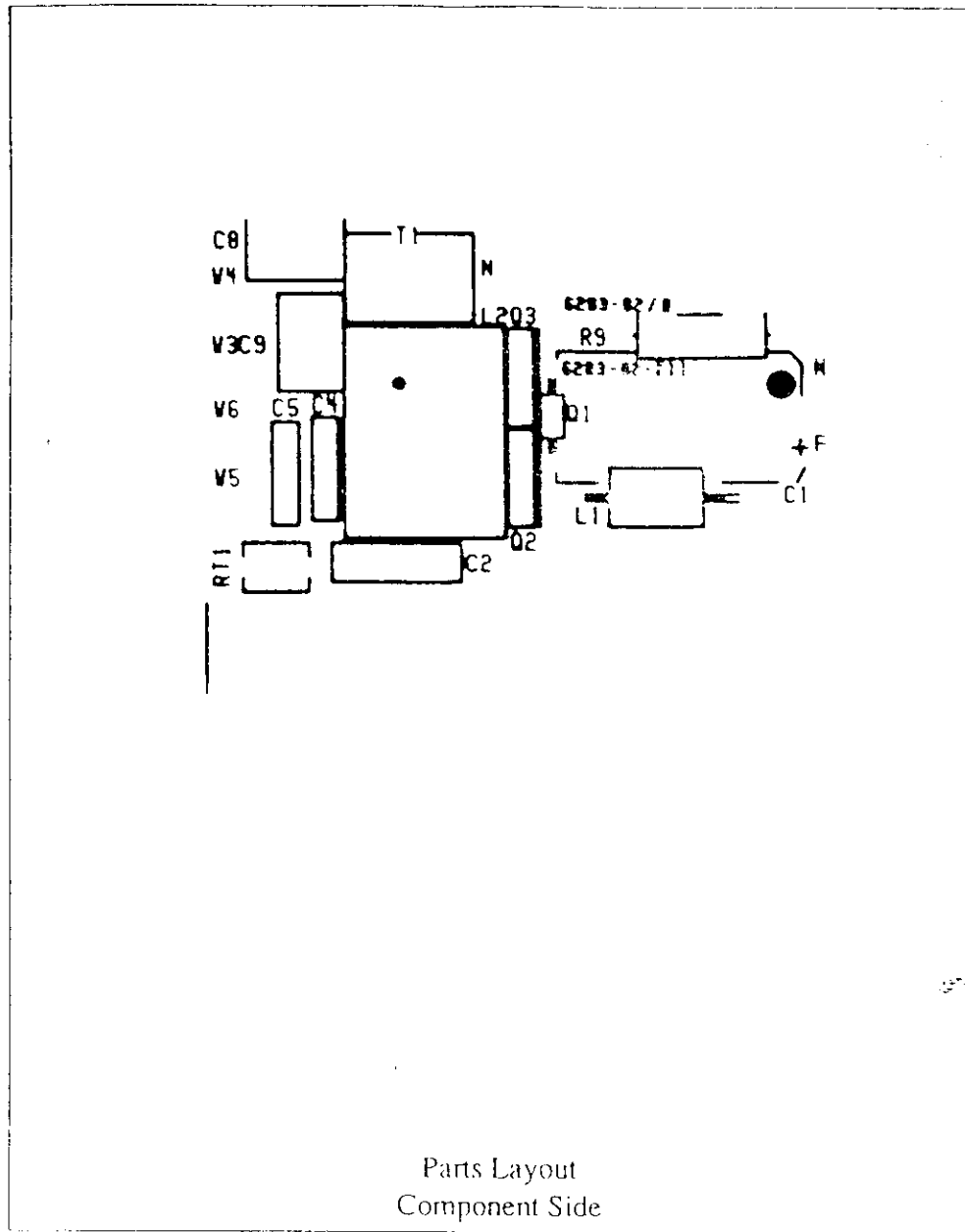
Figure 6.1 Parts layout drawings of the Mini-Lynx 11W/728
