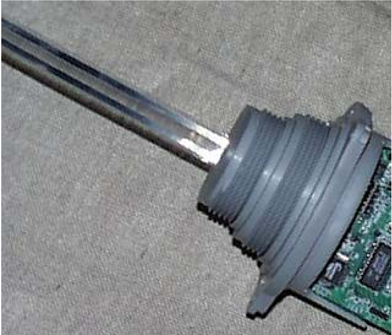
Figure 2: Photograph of outside chassis – base (also showing flat cable)
