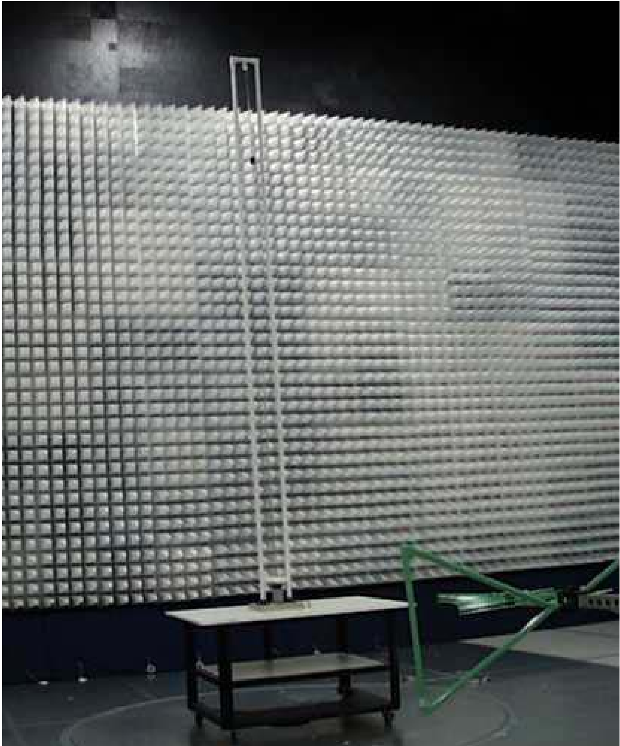
Figure 1: Photograph of radiated emissions setup
