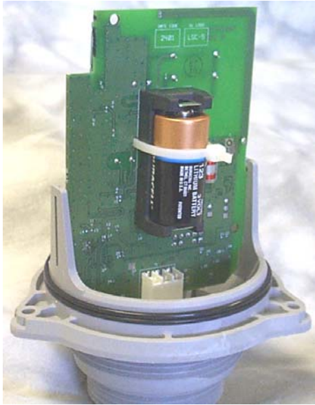
Figure 1. Radar Monitor without Cover (Replacing the Battery)
